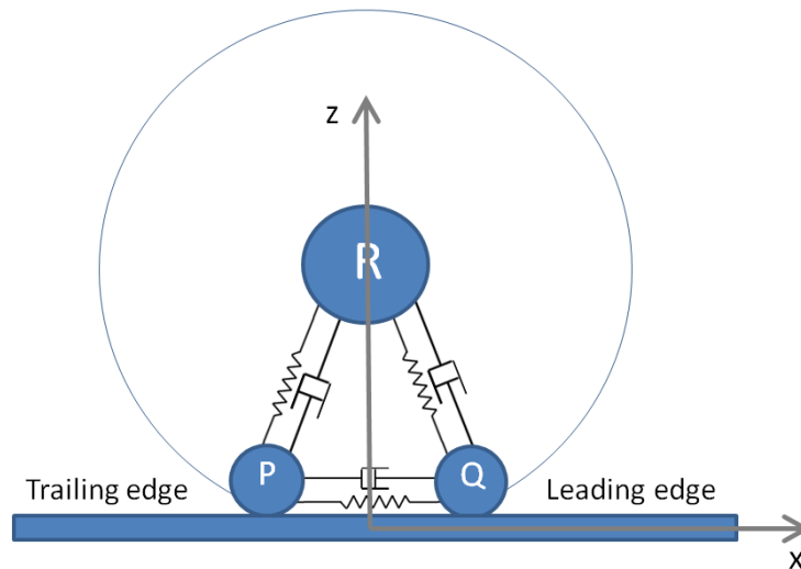
Figure 14. x-z coordinate for a triangle mass-spring-damper system.
