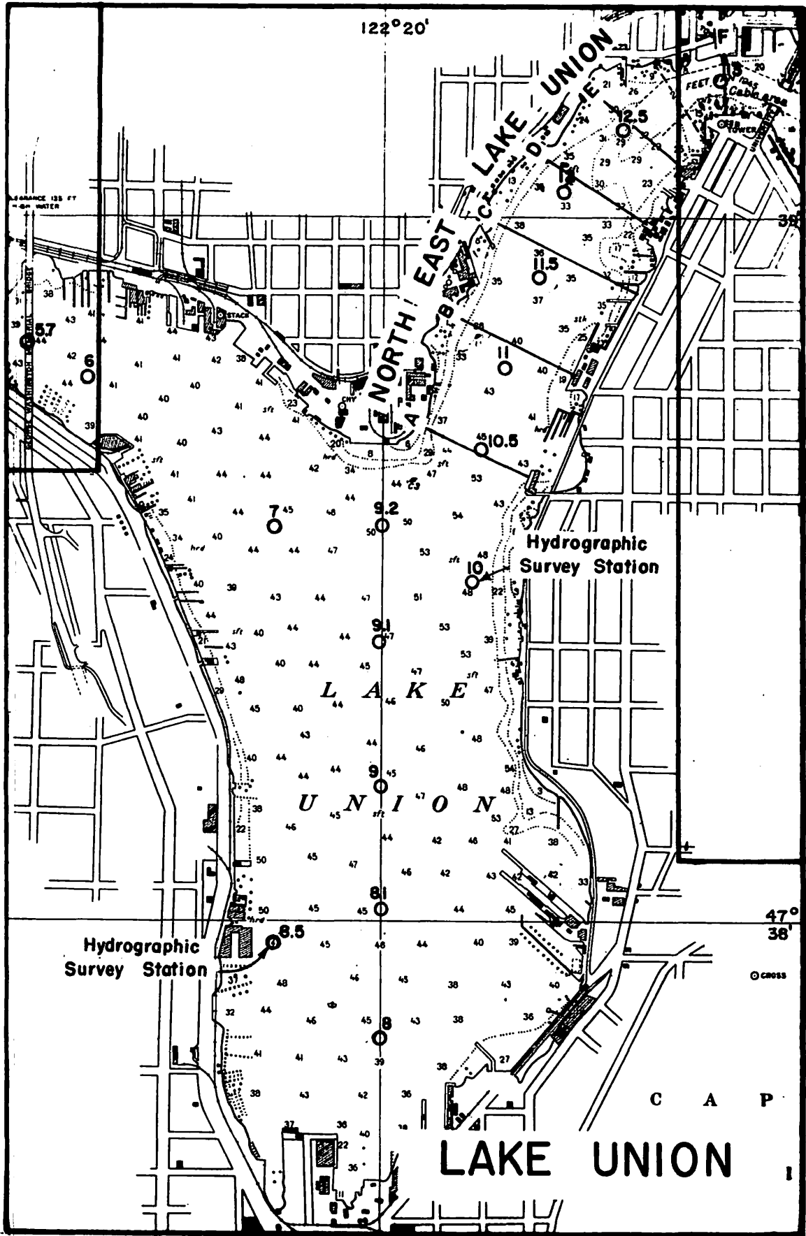
FIGURE 9. Lake Union Showing Survey Stations 6 to 13 and Indicating Locations of Cross Sectional Areas A to F of the North-east Branch of Lake Union. (Base Chart U.S.C.&G.S. Chart 6447)
