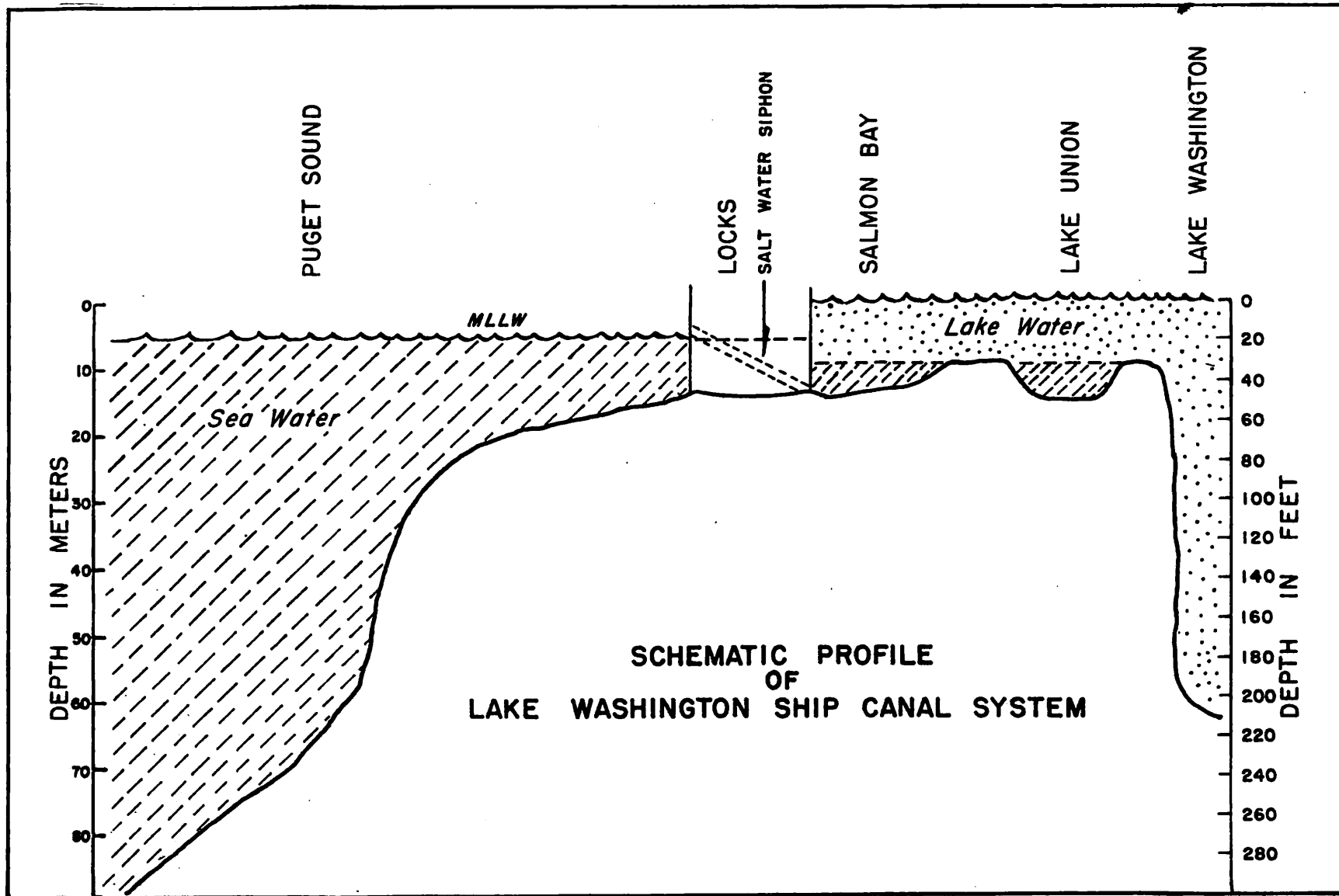
FIGURE 3. Schematic Profile of the Ship Canal.
