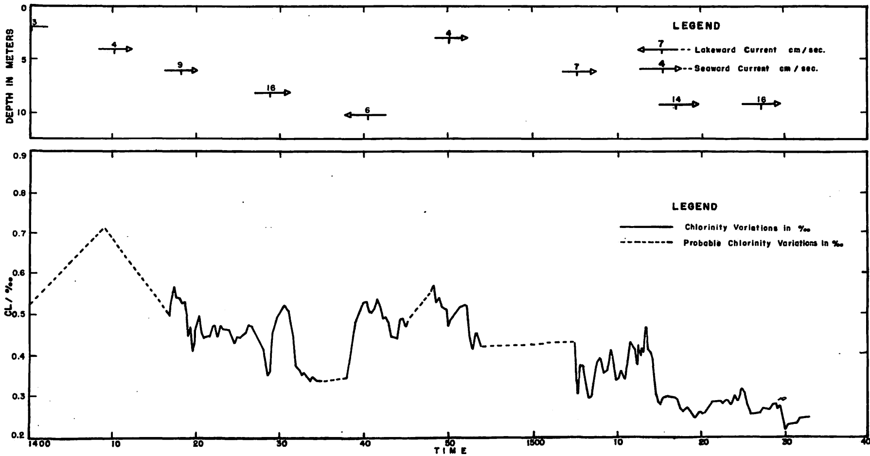
FIGURE 6b. Continuous Chlorinity (‰) Variation at 8 m. and Current Velocities (cm./sec.) at Different Times and Depths in Fremont Canal 1400-1540 (zone +8 time) 16 July 1953.
