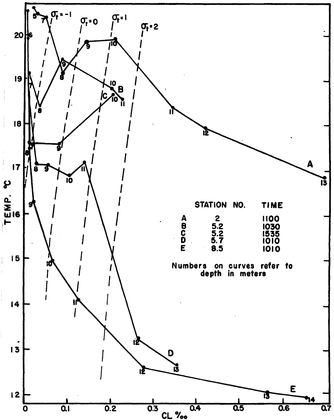
FIGURE 8. Temperature-Chlorinity Diagram Indicating the Source Water in Fremont Canal 16 July 1953.
