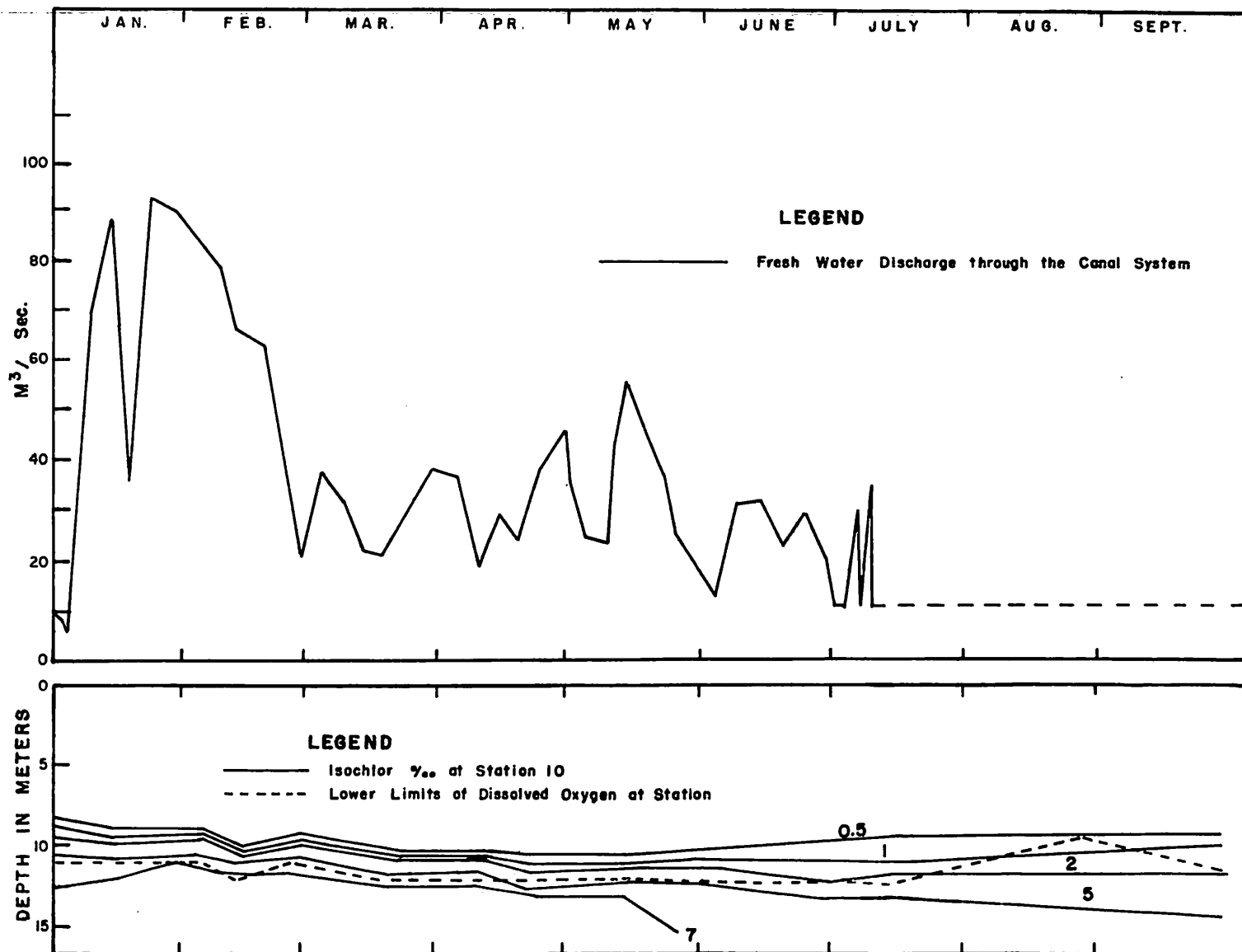
FIGURE 10c. Chlorinity (‰) Variation at Station 10 in Lake Union and Fresh-Water Discharge (m. 3 /sec.) Through the Canal 1953.
