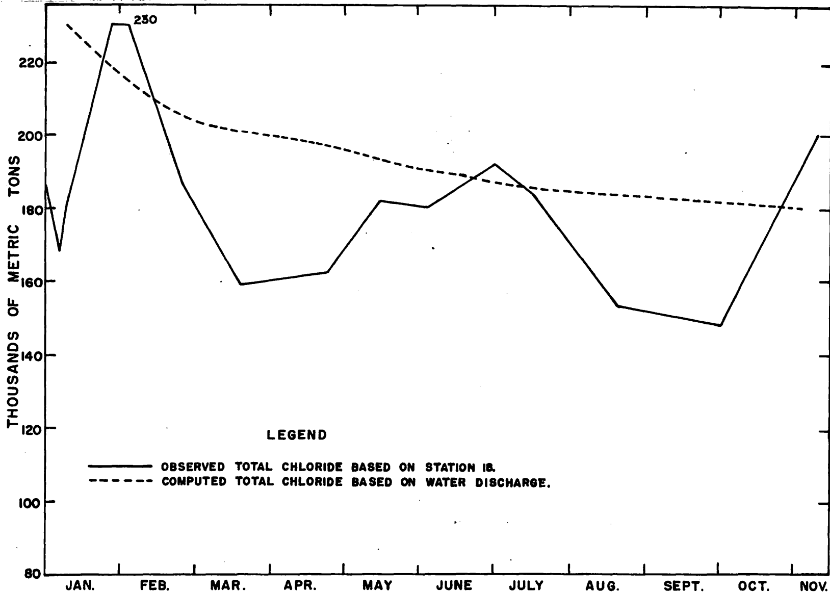
FIGURE 19b. Total Chloride (metric tons) in Lake Washington (Station 18) 1953.
