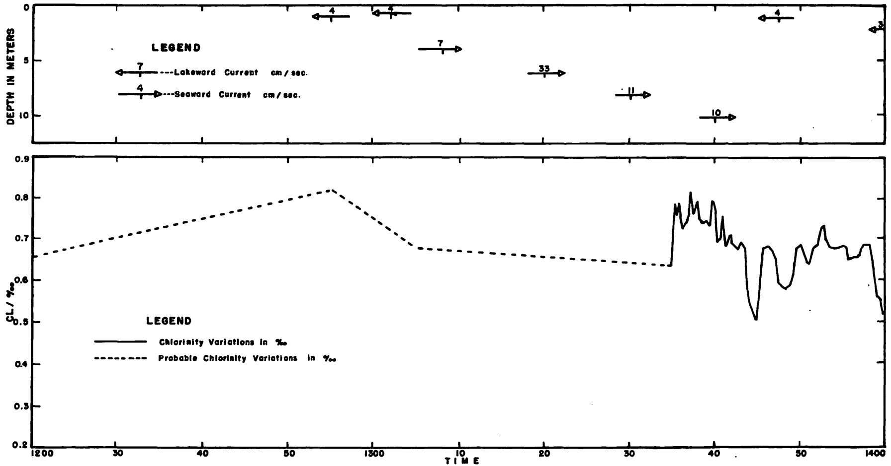
FIGURE 6a. Continuous Chlorinity (‰) Variation at 8 m. and Current Velocities (cm./sec.) at Different Times and Depths in Fremont Canal 1200-1400 (zone +8 time) 16 July 1953.
