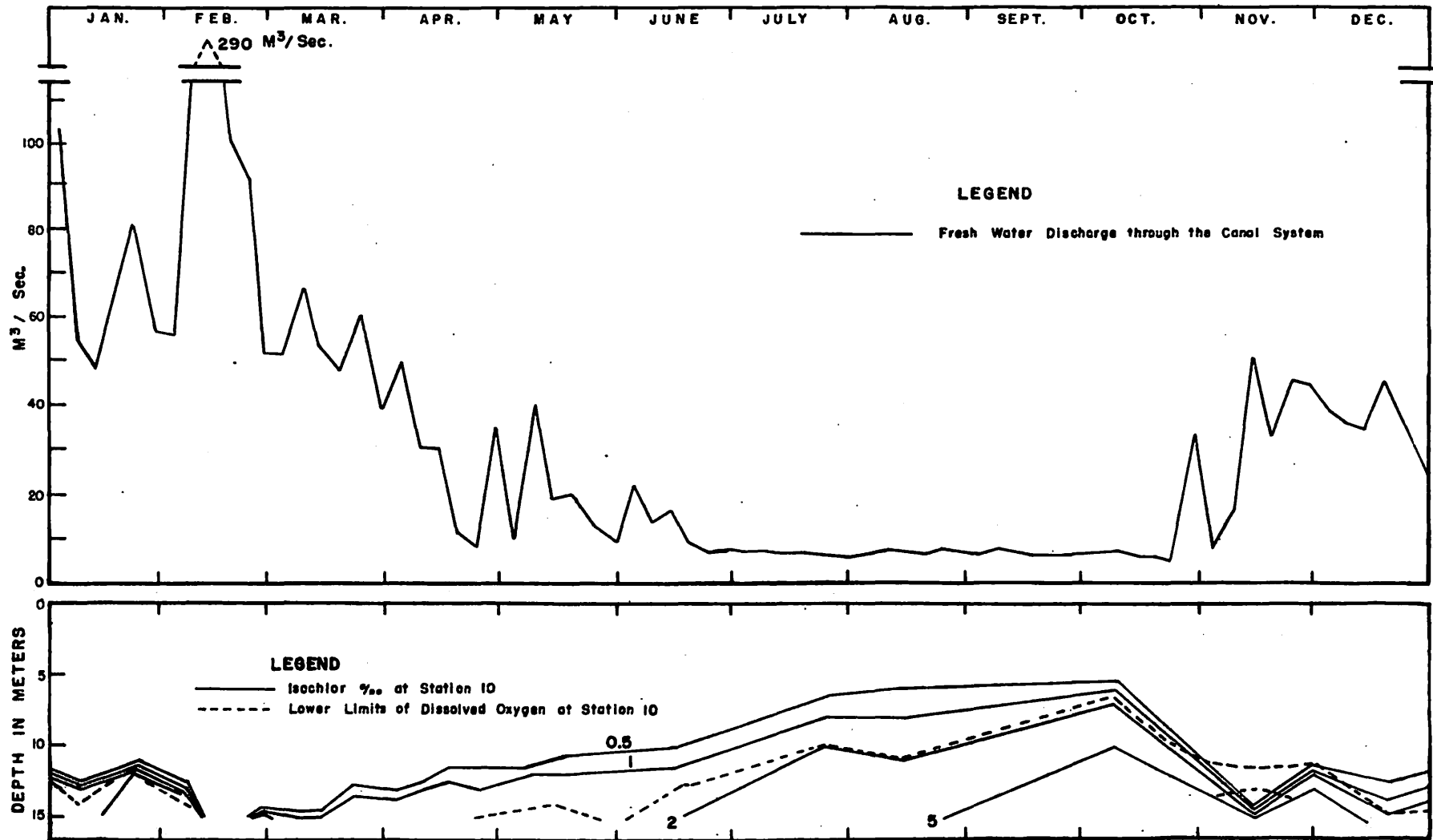
FIGURE 10a. Chlorinity (‰) Variation at Station 10 in Lake Union and Fresh-Water Discharge (m. 3 /sec.) Through the Canal 1951.
