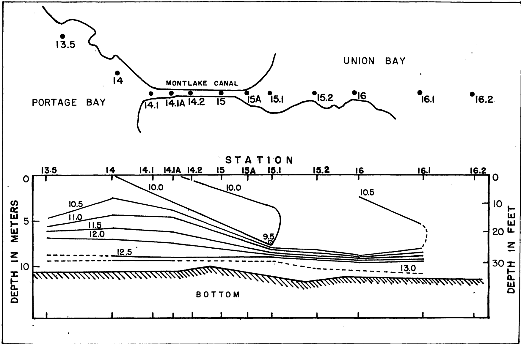
FIGURE 15. Temperature ( ^{\circ} C.) Profile of Montlake Canal (Stations 13.5 to 16.1) 21 November 1952.
