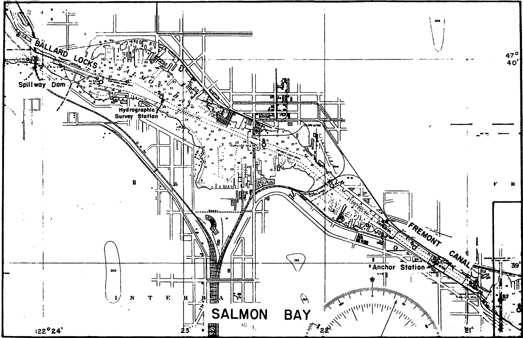
FIGURE 5. Ballard Locks to Lake Union Showing Survey Stations 1 to 6. (Base Chart U. S. C. & G. S. Chart 6447)
