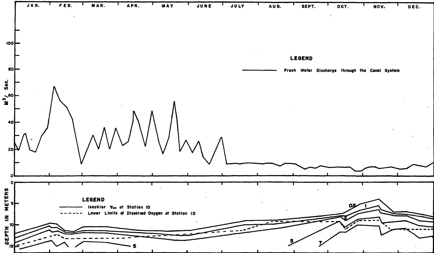
FIGURE 10b. Chlorinity (‰) Variation at Station 10 in Lake Union and Fresh-Water Discharge ( m.^3/sec. ) Through the Canal 1952.
