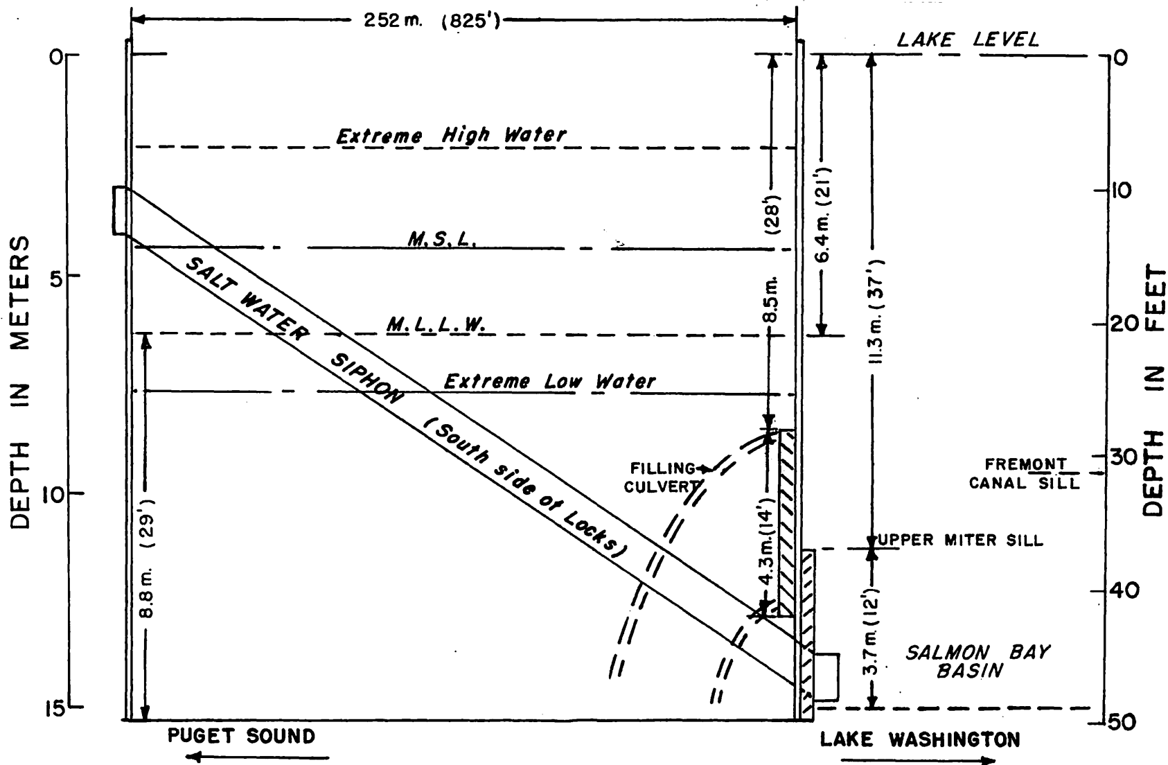
FIGURE 4. Diagram of the Large Lock Showing the Depth of the Filling Culvert and Upper Miter Sill in Relation to Lake Level and the Various Sea Levels.
