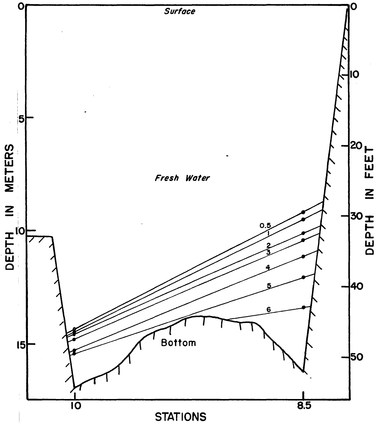
FIGURE 12. Sloping Isochlers ( ^{\circ}/\infty ) in Lake Union Between Station 10 and Station 8.5 14 November 1951.
