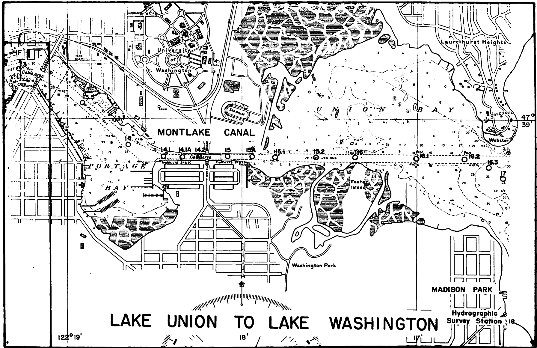
FIGURE 13. Lake Union to Lake Washington Showing Survey Stations 13 to 18. (Base Chart U. S. C. & G. S. Chart 6447)
