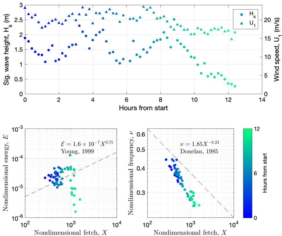
Figure 5.1: Preliminary analysis of SWIFT buoy observations during katabatic wind event in Terra Nova Bay polynya. Upper panel shows time series of significant wave height (circles) and wind speed at 1-m (triangles). Bottom plots show comparison of nondimensional fetch with nondimensional wave parameters compared to classic open water scalings [dashed lines; Young, 1999 ; Donelan et al., 1985 ]. Colors show hours since beginning of deployment.
