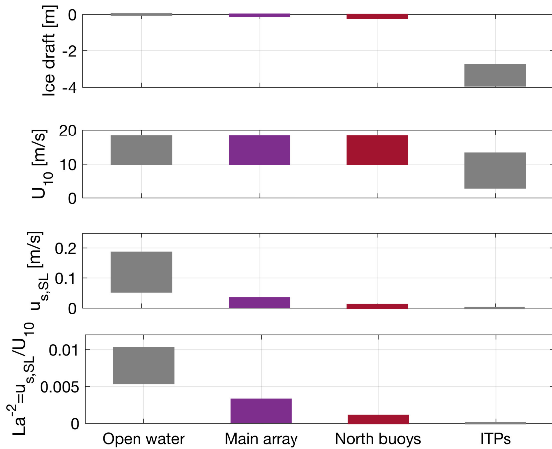
Figure 3.9: Comparison of ice, wind, and wave forcings observed in open water, during the 10-14 Oct event, and under thick ice observed by ITPs [ Jackson et al. , 2012; Timmermans , 2015]. Observations during the 10-14 Oct 2015 event are separated out into the main array and northern SWIFT buoys, in purple and red respectively.
