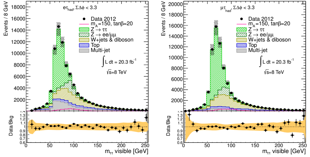
Figure 7.6: The invariant mass of the lepton and the hadronic tau, after the cut on \Sigma\Delta\phi . The shaded bands indicate the total systematic uncertainty.
