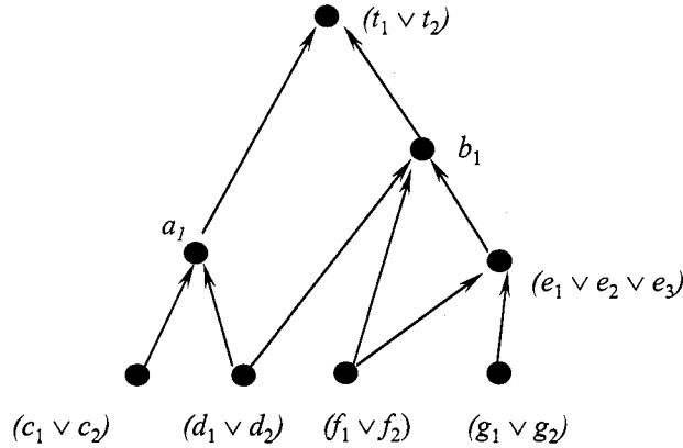
Figure 5.2: A simple pebbling graph to illustrate branch sequence generation
