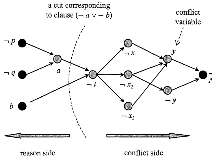
Figure 4.1: A conflict graph
