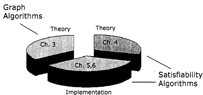
Figure 1.1: The three applications of proof complexity explored in this work
