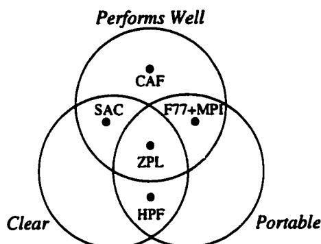
Figure 5.11: Summary of the MG Experiments. This Venn diagram summarizes the MG implementations used in this study. When comparing the implementations in terms of clarity, portability, and performance, they naturally fall into distinct groups. These groups are mapped to the Venn diagram directly.
