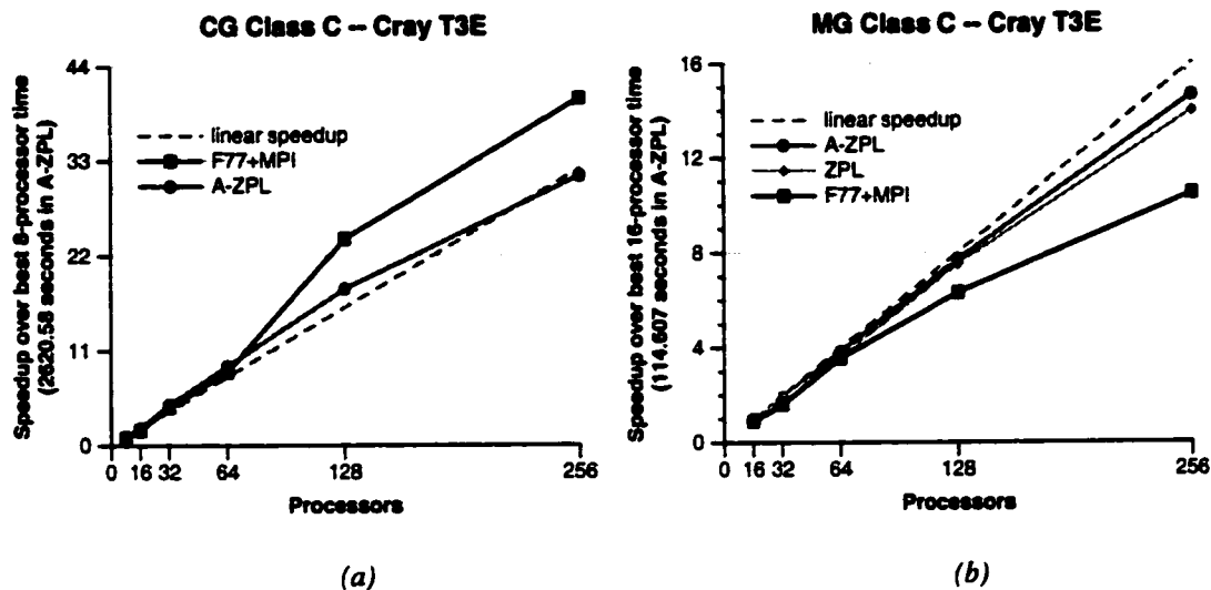
Figure 6.11: Performance for Sparse CG and MG Benchmarks. These graphs show speedup curves for class C of the NAS CG and MG benchmarks on the Cray T3E. Note that there is not enough memory to run these problem sizes on small processor sets. Thus, the speedups for each graph are computed using the fastest execution time on the smallest number of processors (indicated in the y-axis label).
