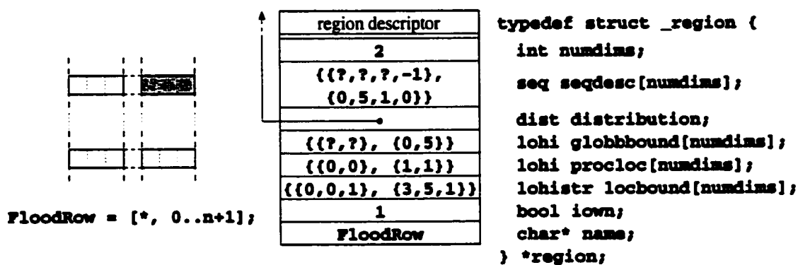
Figure 4.7: The Region Descriptor. This figure shows a flooded row region and the region descriptor for the processor owning the shaded portion of its indices. The fields are as follows: numdims —the rank of the region; seqdesc —the region’s defining sequence descriptors; distribution —a reference to the region’s distribution descriptor; globbound[] —the lowest and highest indices represented by the region in each dimension; procloc[] —the processor coordinates owning these lowest and highest indices; locbound[] —the bounds and stride that define the processor’s local indices; iown —a boolean flag indicating whether or not the processor owns a piece of the region; name —the name of the region, for debugging purposes.
