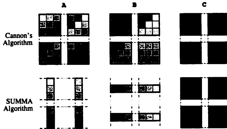
Figure 3.9: 2D Matrix Multiplication Memory Accesses. This illustration shows the approximate amount of memory touched per processor in each iteration of Cannon's Algorithm and the SUMMA algorithm. The SUMMA algorithm has a smaller memory footprint due to the fact that it refers to a single column of A and row of B in each iteration using a flood. In contrast, Cannon's algorithm has to read all of A and B's elements to perform shifts and its elementwise multiplications. Both algorithms touch all elements of C, so there is no difference there.
