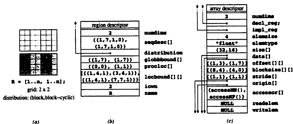
Figure 4.17: Proposed Block-Cyclic Distribution Implementation. (a) A square region that is distributed to a 2 \times 2 processor grid using a blocked distribution for the first dimension and a block-cyclic distribution for the second. The unshaded indices indicate those that would be owned by the second processor in the grid. (b) The region descriptor that describes the unshaded indices. Note that an extra dimension has been added to the traditional local bounds field so that the bounds of each block owned by the processor can be described. The iown field has been changed from a boolean to an indicator of the number of distinct blocks owned by this processor. (c) The array descriptor for an array of floats declared using this region. Several of the fields (the data size, data and origin pointers, offsets, block sizes, and strides) have had an extra dimension added so that the memory layout of each block owned by the processor can be described.
