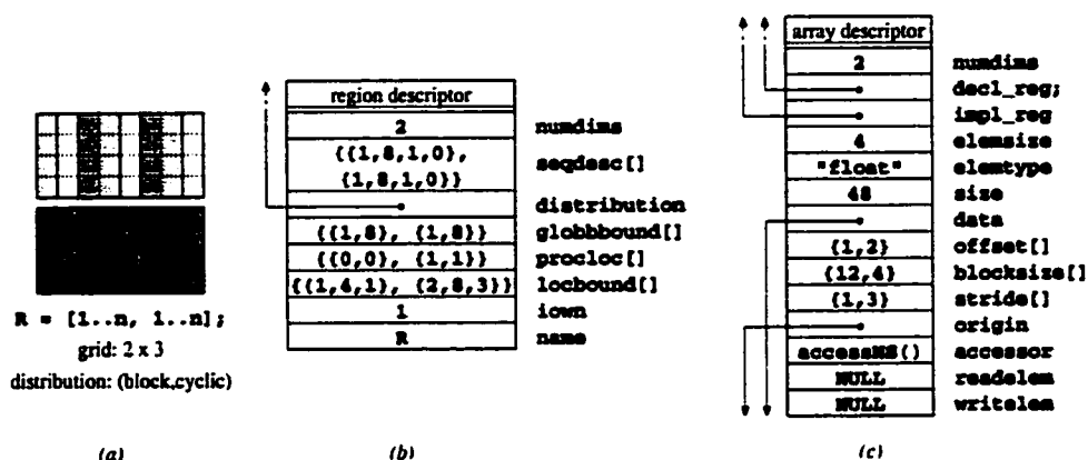
Figure 4.15: Proposed Cyclic Distribution Implementation. (a) A square region that is distributed to a 2 \times 3 processor grid using a blocked distribution for the first dimension and a cyclic distribution for the second. The unshaded indices indicate those that would be owned by the second processor in the grid. (b) The region descriptor that describes the unshaded indices. Note that the local bounds in the second dimension are strided by 3 to capture the cyclic striding. Furthermore, the region's upper processor location is processor 1 rather than processor 2 since it holds the highest index. (c) The array descriptor for an array of floats declared using this region. As usual, the offsets are set so that the lowest local index—(1,2)—maps to the origin. The blocksize is also set as though this was a normal 3 \times 4 block of data. However, the stride is set to 3 in the second dimension to compress the strided indices down to consecutive data values. A traditional accessor function can be used to access these values, provided that it uses the stride in the second dimension.
