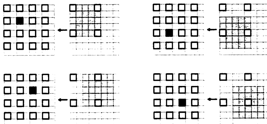
Figure 5.5: MG's interp Stencil. This figure shows a 2D illustration of MG's interp stencil. For each of the four applications of the stencil shown, the grey element on the right-hand side of the assignment indicates the value being written, and the grey box on the right-hand side shows the extent of each 3 \times 3 stencil. Note that a different set of neighboring values are referenced for each application, based on the relative alignment between the fine and coarse grid values. These values are averaged in MG's interp stencil.
