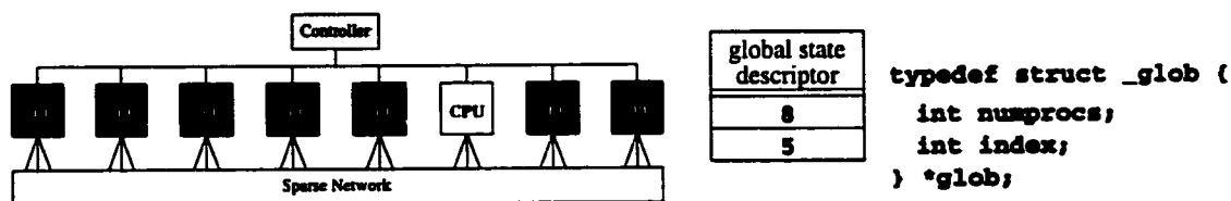
Figure 4.3: The Global State Descriptor. This figure shows the CTA machine model and the global state descriptor that describes the processor shown in white. The numprocs field describes the number of processors in use by the program, and the index field describes the unique ID of the processor storing the descriptor.
