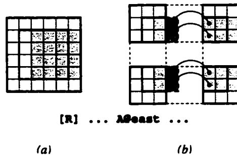
Figure 3.6: The @ Operator in Parallel. (a) The global view of an @-reference. The shaded area will be read for the indices in the center outlined area. (b) The local view of an @-reference. The processors on the left are missing a column of values, so these are sent from the processors on the right using point-to-point communication.
