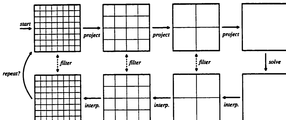
Figure 5.1: The Multigrid Method. This diagram shows a simple overview of the multigrid method. The original discrete problem is projected repeatedly to create coarser and coarser approximations to the original problem. That problem is then solved and the result is interpolated back down the hierarchy, filtering along the way against the original approximations. The entire cycle may then be repeated to improve the solution.
