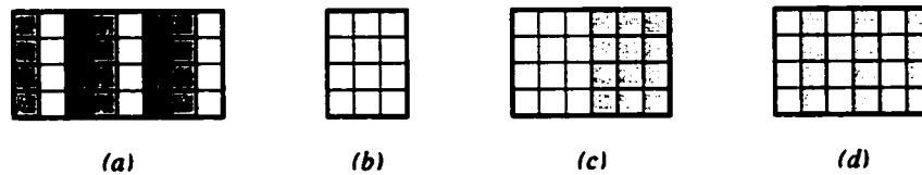
Figure 4.16: Fluff Allocation for Cyclic Distributions. (a) An array whose columns are distributed cyclically. (b) A processor's dense allocation of the unshaded values from part a, assuming that no fluff is required. (c) The fluff allocation for an @east reference in which the fluff values are placed to the side of the processor's data. Note that the amount of fluff required is equal to the amount of data that the processor owns, due to the cyclic distribution. This allocation has the disadvantage that calculating the address for a fluff value does not match the normal array access idioms since the alignment of an index affects its resulting address. (d) An alternative scheme in which the fluff is interleaved with the actual data. This allows traditional access idioms to be used, but has the disadvantage of spacing a processor's actual values out farther in memory.
