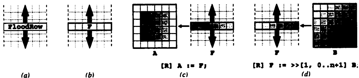
Figure 2.6: Flood Dimensions and Flood Arrays. (a) An illustration of a region whose first dimension is flooded. It represents a single row of values that are conformable to any row. (b) An array F declared using region FloodRow . (c) An assignment from F to A within region R . (d) An assignment from a row of B to F using the flood operator.
