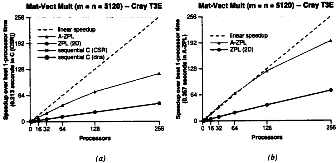
Figure 6.9: Performance for Sparse Matrix-Vector Multiplication. (a) A speedup graph for matrix-vector multiplication comparing the sparse A-ZPL implementation against the dense ZPL implementation and sequential versions in C written using dense arrays and the CSR format. (b) The same comparison, but without the sequential C versions.
