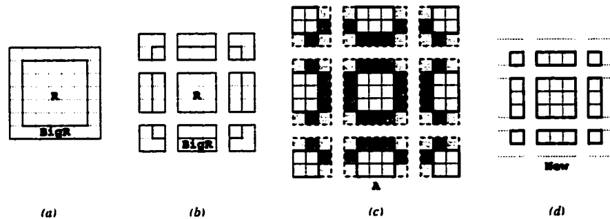
Figure 4.9: Fluff Required by the Jacobi Iteration. (a) The global-view of regions R and BigR for the Jacobi iteration. (b) The blocked distribution of the index space for a 3 \times 3 processor grid. (c) The memory allocated on each processor for array A. White values are normal array values. Dark grey values indicate fluff values required by the processor to store elements transferred for the @-references. Light grey values indicate additional values that are allocated to keep each processor's data rectangular in shape. (d) The memory allocated on each processor for array New. No fluff values are required since it has no @-references within the program.
