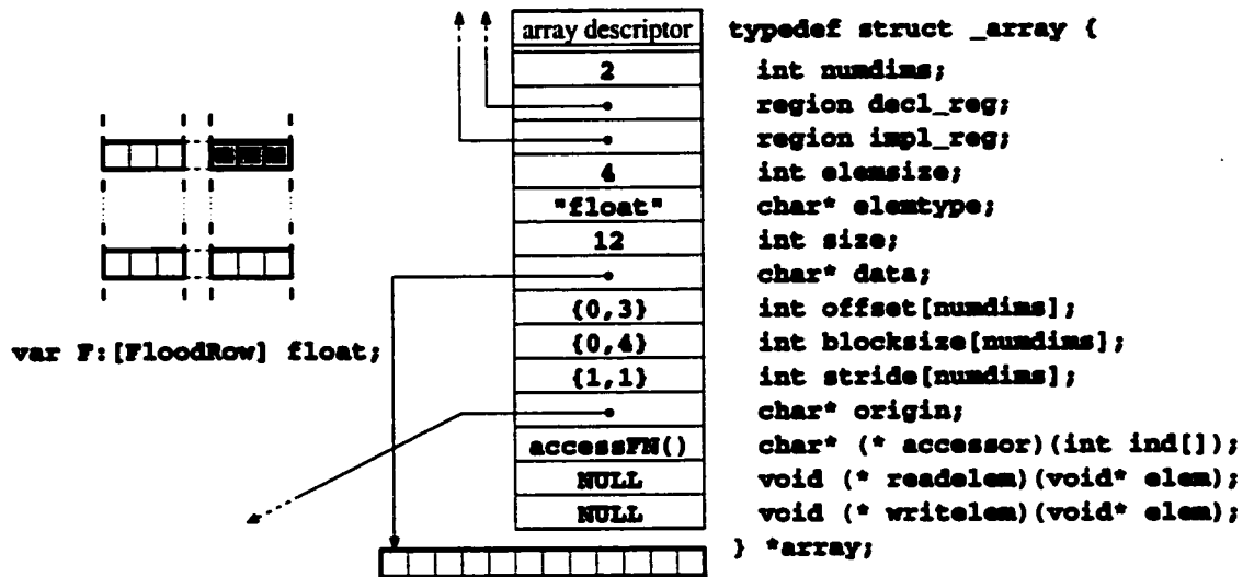
Figure 4.8: The Parallel Array Descriptor. This figure shows the parallel implementation of a flooded row array, and the array descriptor for the processor owning the shaded portion of the array. The fields are as follows: numdims —the rank of the array; decl_reg —the region used to declare the array; impl_reg —the region describing the array’s size once implicit storage is added to it; elemsize —the size of the array’s element type in bytes; elemtype —a string describing the array’s element type; size —the size of the data buffer allocated for the array’s data values; data —a pointer to the array’s data buffer; offset[] —offsets for making global indices zero-based when accessing the array; blocksize[] —multiplicative factors used to scale each dimension of an array’s access; stride[] —divisors used to stride an array’s dimensions; origin —a special pointer used to optimize array accesses; accessor() —a function used to access the array element at a given index; readelem()/writeelem() —functions to read or write the elements of an array, used primary for arrays with non-scalar element types.
