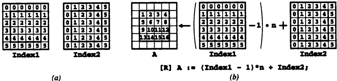
Figure 2.7: The Index Constants. (a) Pictures depicting Index1 and Index2 . BigR and R are indicated by the outlines. (b) A diagram showing the unique numbering of elements in R using Index1 and Index2 .
