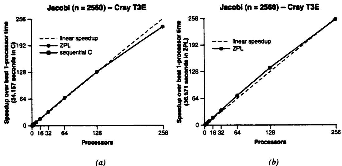
Figure 3.12: Performance of the Jacobi Iteration. (a) The speedup of the ZPL implementation of the Jacobi Iteration as compared to a hand-coded C version. (b) The speedup of the ZPL implementation against itself.
