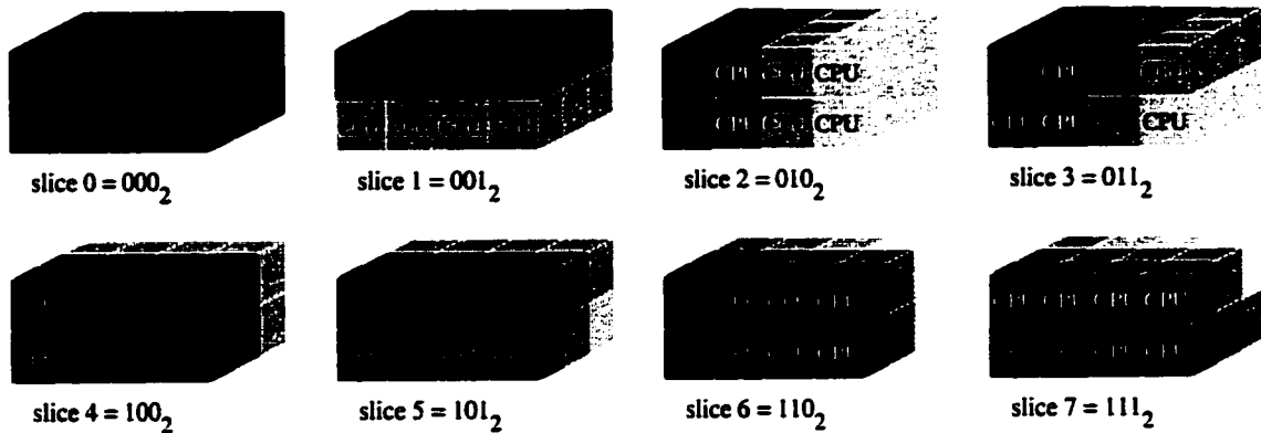
Figure 4.4: Processor Grid Slices in 3D. This figure illustrates the 8 ways of slicing a 3D processor grid and their corresponding slice numbers.
