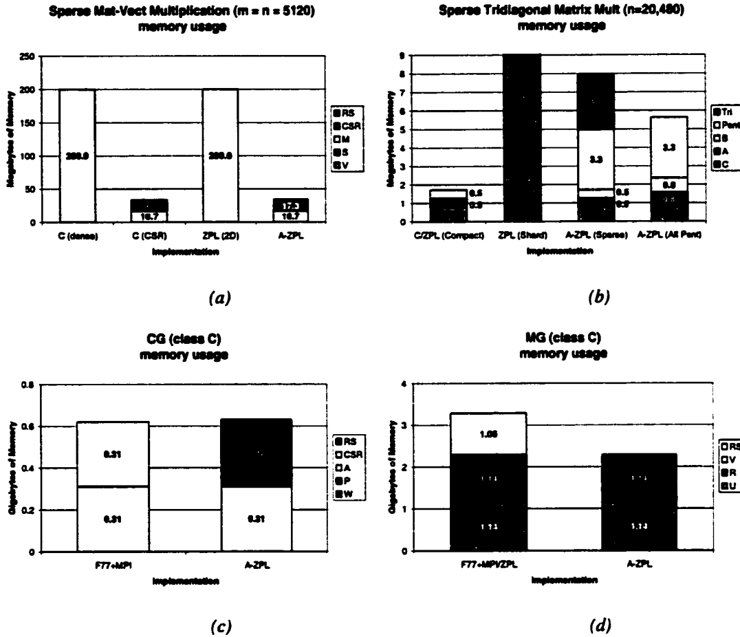
Figure 6.8: Memory Requirements for Sparse Benchmarks. These graphs indicate the memory used by each benchmark’s main data structures when run on a single processor. In general, “RS” indicates the memory required by a sparse region whereas “CSR” indicates the memory used by a hand-coded CSR format. (a) Sparse matrix-vector multiplication as written in C using dense arrays and the CSR format, in ZPL using a dense region, and in A-ZPL using a sparse region. Recall that “M” is the sparse matrix, while “V” and “S” are the input and solution vectors. (b) Sparse tridiagonal matrix multiplication as written in C and ZPL using a compact format, in ZPL using a dense format, and in A-ZPL using two or one sparse regions. “A,” “B,” and “C” are the three matrices. “Tri” and “Pent” are the sparse tridiagonal and pentadiagonal regions as declared in A-ZPL. (c) The CG benchmark as written by NAS in F77+MPI and in A-ZPL using a sparse region. “P” and “W” are vectors, whereas “A” represents the sparse array values. (d) The MG benchmark as written in F77+MPI or ZPL using a dense input array and in A-ZPL using a sparse input array. Recall that “U” and “R” are the two hierarchical arrays and that “V” is the input array.
