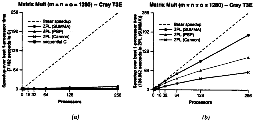
Figure 3.14: Performance of Matrix Multiplications. (a) The speedup of the Cannon, SUMMA, and PSP Matrix Multiplication algorithms as compared to a sequential hand-coded C version. (b) The speedup of the ZPL implementations in isolation.
