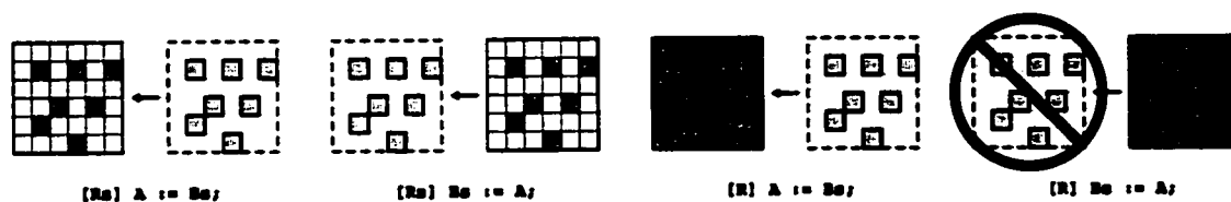
Figure 6.3: Sample Sparse/Dense Assignments. Assume that R and A are dense, and that R_s and B_s are sparse. Note that sparse reads and writes of both arrays are legal, referring only to the elements in the sparsity pattern. Dense reads of sparse arrays are also legal—the IRV is used for values that are not in the sparsity pattern. However, a dense write to a sparse array is not legal due to the fact that a unique memory location is not allocated for each index. These examples extend in the obvious way to statements which refer to multiple sparsity patterns.
