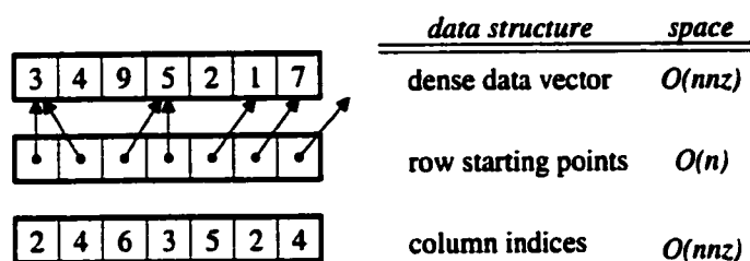
Figure 6.2: The CSR Sparse Array Format. This figure shows the sparse array of Figure 6.1 stored in CSR format. The array's interesting values are stored in a dense vector format. A second vector of integer pointers indicates the starting position of each row of the array. The third vector stores the column index of each value.
