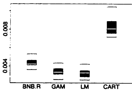
Figure 3.2: Hyperplane
