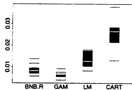
Figure 3.3: Friedman #1
