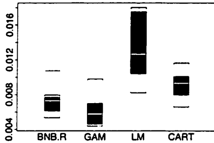
Figure 3.4: Friedman #2
