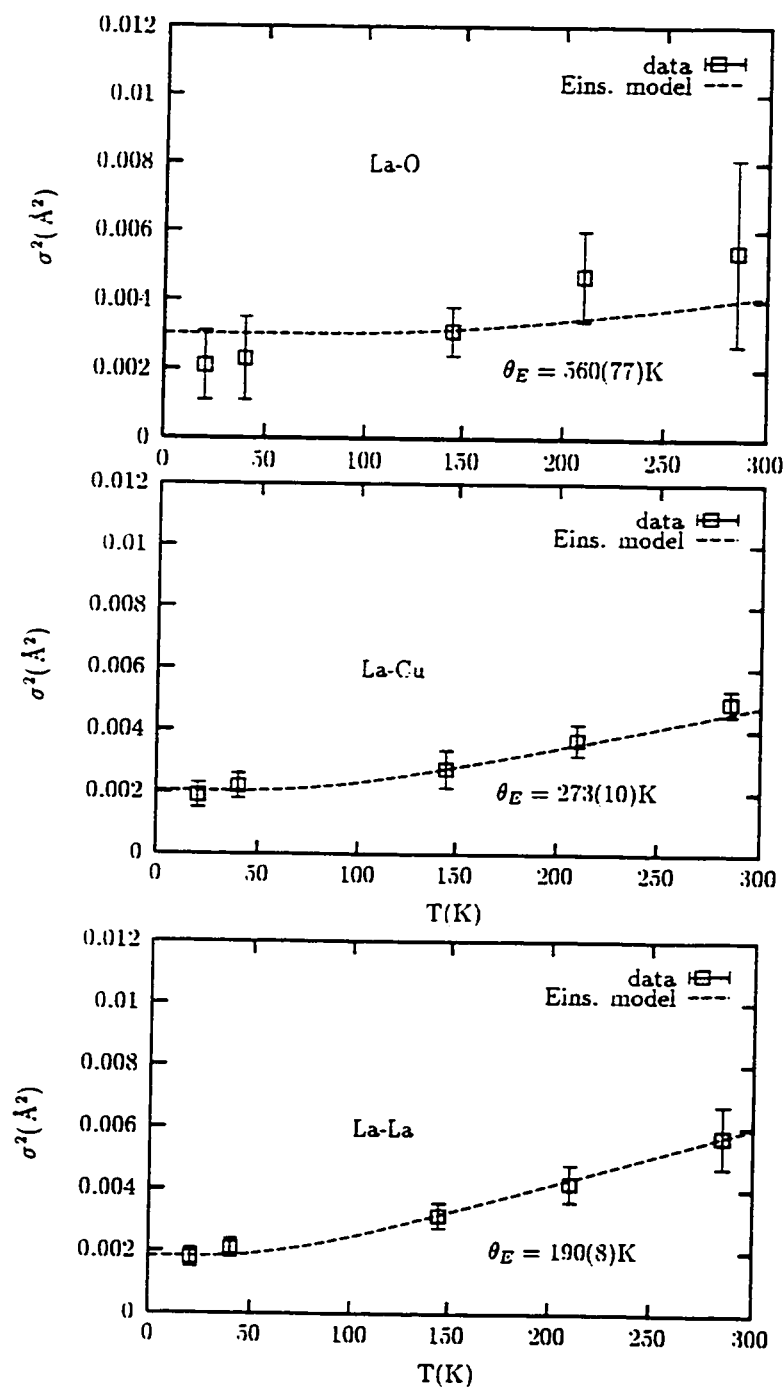
Figure 5.18: Fit results for Debye-Waller factors as obtained for x = 0.15 at temperatures below and above the structural phase transition. Fits to Einstein models also shown with their respective Einstein temperatures.
