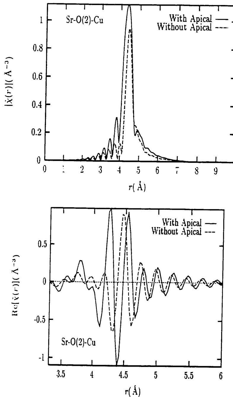
Figure 5.30: FEFF6 calculation of the Sr-O(2)-Cu MS paths at r \sim 4.76 \text{ \AA} with and without the O(2) apical oxygen. Three SS oxygen paths at r \sim 5 \text{ \AA} listed in table 5.11 are also included in both cases. Magnitude (top) and real part (bottom) of the Fourier transform are shown. Atomic positions used correspond to x = 0.1 at 10K.
