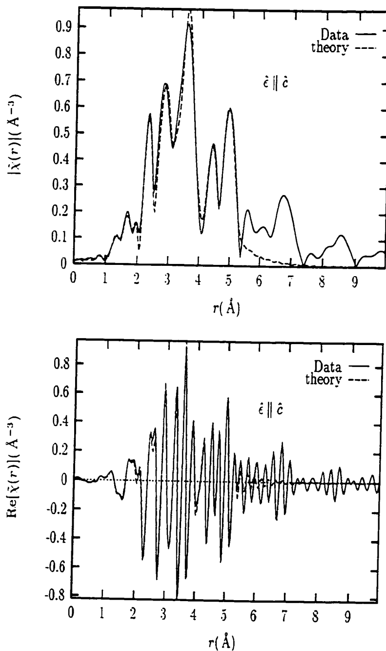
Figure 6.12: Fit results for the x = 0.125 sample at T=10 K. The magnitude (top) and the real part (bottom) of the complex Fourier transform are shown for \hat{\epsilon} \parallel \hat{c}
