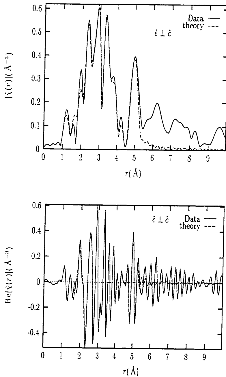
Figure 6.13: Fit results for the x = 0.125 sample at T=10 K. The magnitude (top) and the real part (bottom) of the complex Fourier transform are shown for \hat{\epsilon} \perp \hat{c}
