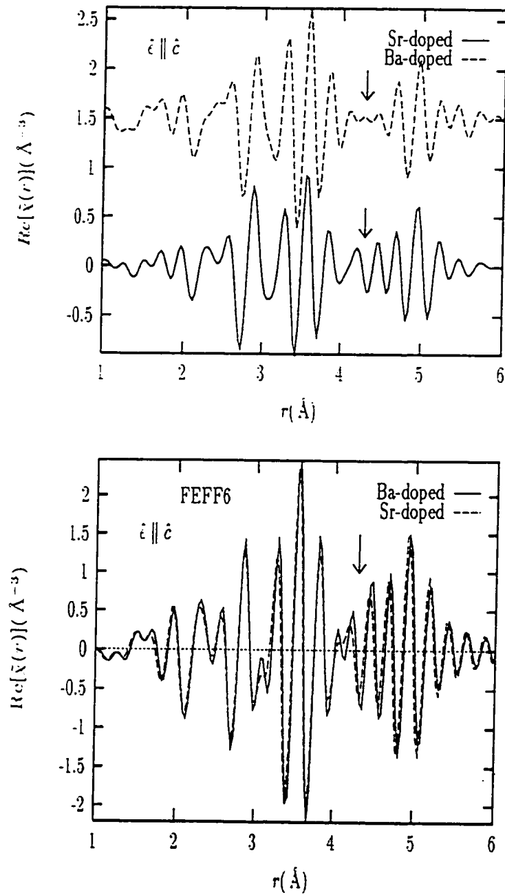
Figure 6.8: Real part of the complex Fourier transforms of Sr-doped ( x = 0.075 , T=20\text{K} ) and Ba-doped ( x = 0.125 , T=10\text{K} ) La K -edge, \hat{c} -polarized XAFS data (top) and their respective FEFF6 calculations (bottom) using the relevant average structures found by diffraction. The FEFF6 calculations are not corrected for thermal or static disorder. The larger than expected disorder in the La-O(2)-Cu MS signal of the Ba-doped sample is evident.
