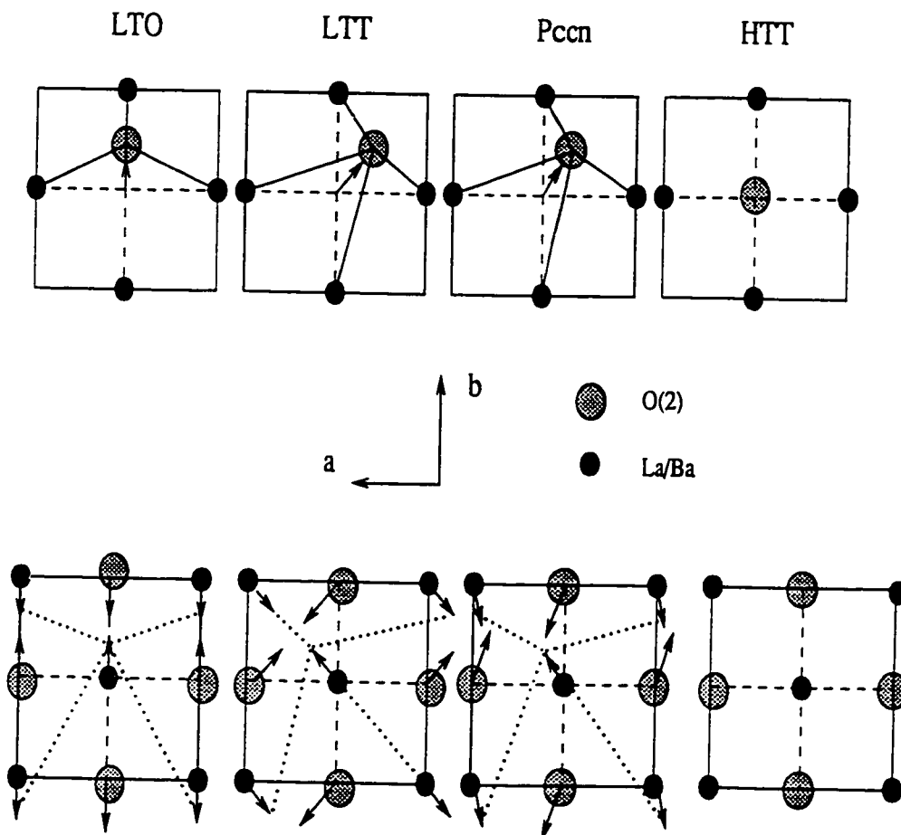
Figure 6.17: Schematic representation of the O(2) and correlated La/Ba atomic displacements in all LTO, LTT, Pccn and HTT phase. The arrows are not drawn to scale; the O(2) displacements (relative to the undistorted HTT phase) being much larger than the La/Ba ones.
