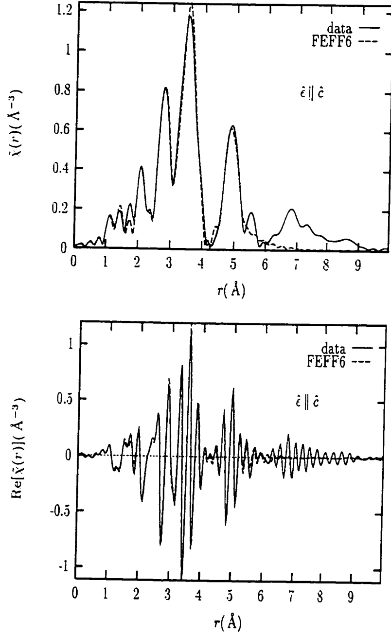
Figure 6.4: Fit results for the x = 0.125 sample at T = 10 K. The magnitude (top) and the real part (bottom) of the complex Fourier transform are shown for \hat{\epsilon} \parallel \hat{c}
