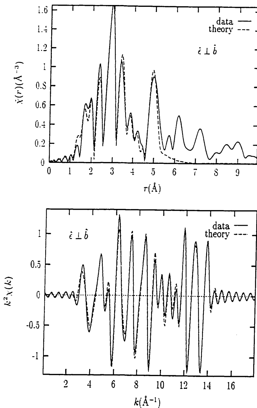
Figure 5.27: Sr K -edge fit results for x = 0.1 , \hat{\epsilon} \perp \hat{b} at T=17\text{K} . Top: Magnitude of the complex Fourier transform; bottom: back Fourier transform of the fitted region of r -space.
