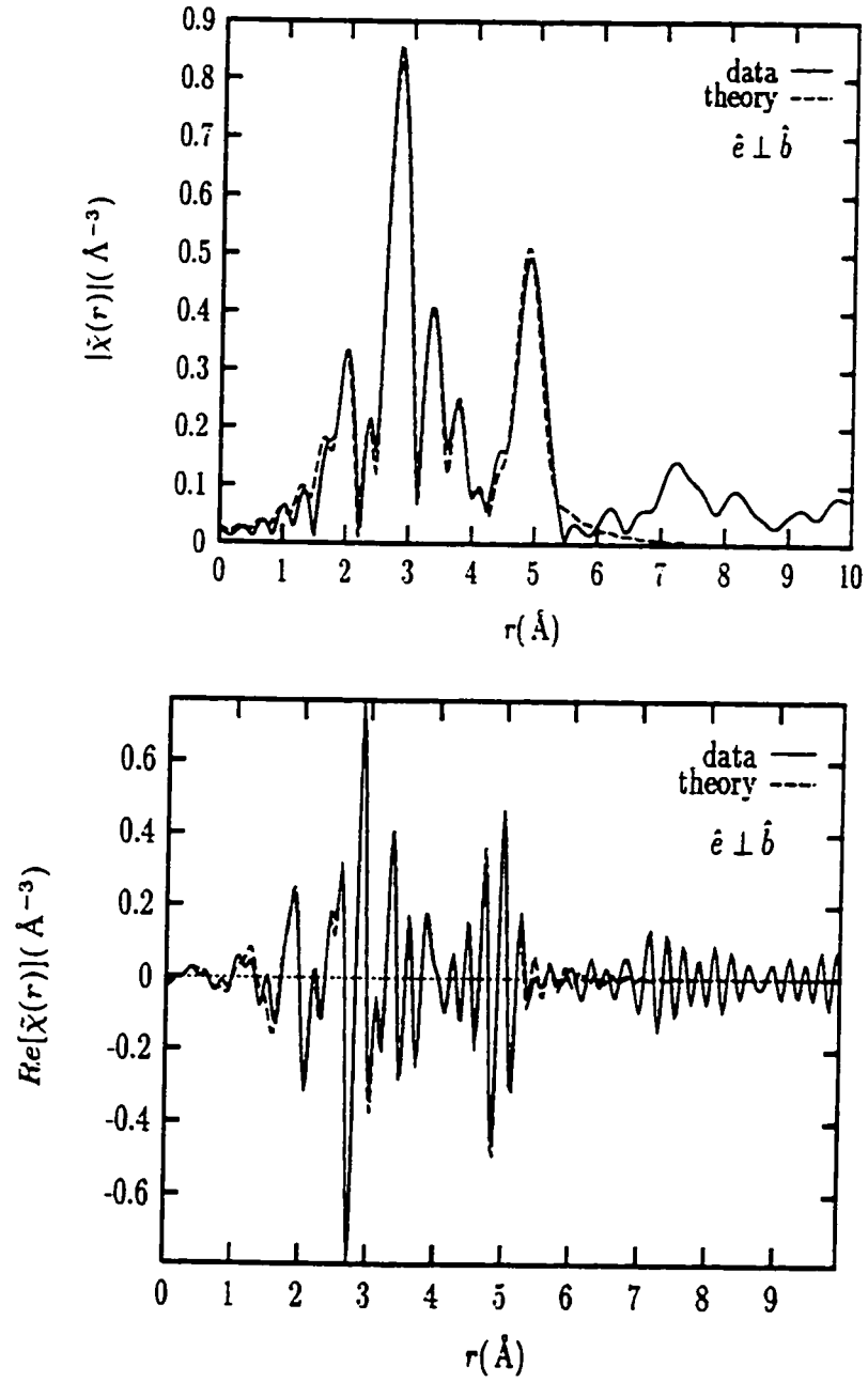
Figure 5.6: Fit results for the x = 0.075 sample at 20 K. The magnitude (top) and the real part (bottom) of the complex Fourier transform are shown for \hat{e} \perp \hat{b}
