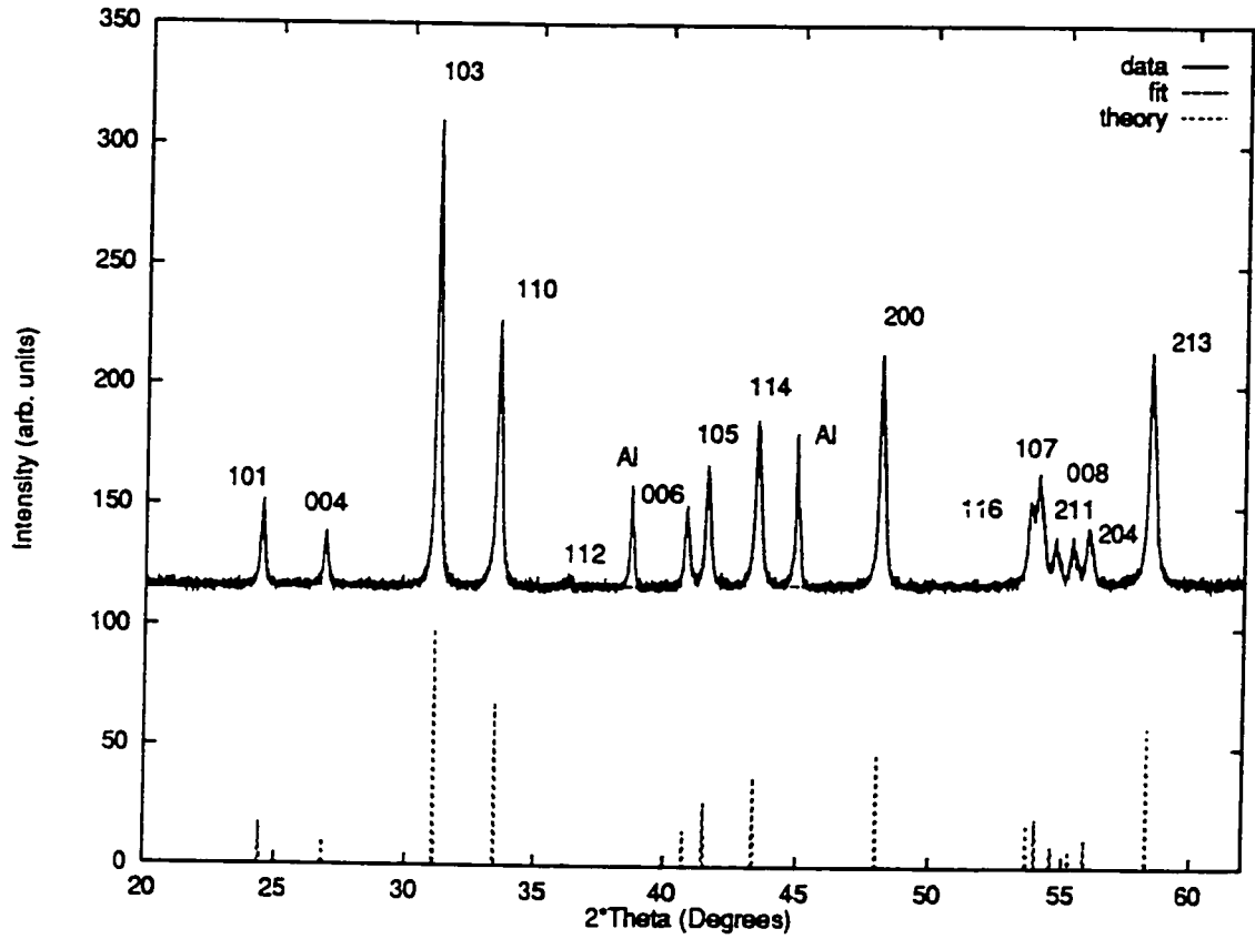
Figure 4.10: Powder diffraction pattern for \text{La}_{1.85}\text{Ba}_{0.15}\text{CuO}_4 at 300K together with the fit obtained by varying the lattice parameters. A theoretical powder pattern is also shown.
