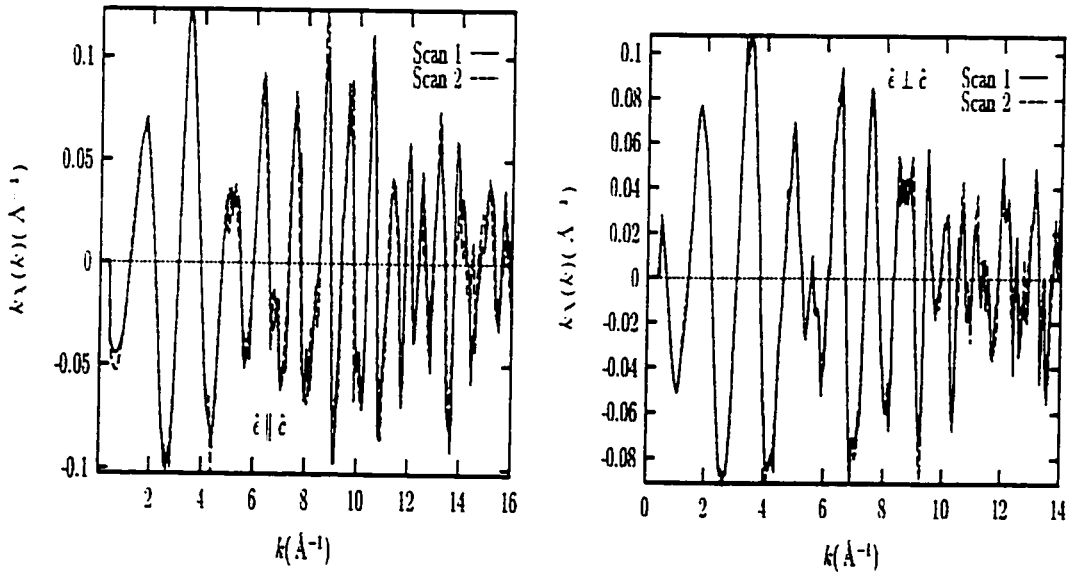
Figure 6.10: k\chi(k) reproducibility data for x = 0.125, 0.15 in \text{La}_{2-x}\text{Ba}_x\text{CuO}_4 at T=10\text{K} . Left: x = 0.125 , \hat{c} -polarization; right: x = 0.15 , in-plane, \hat{a}\hat{a} -polarization
