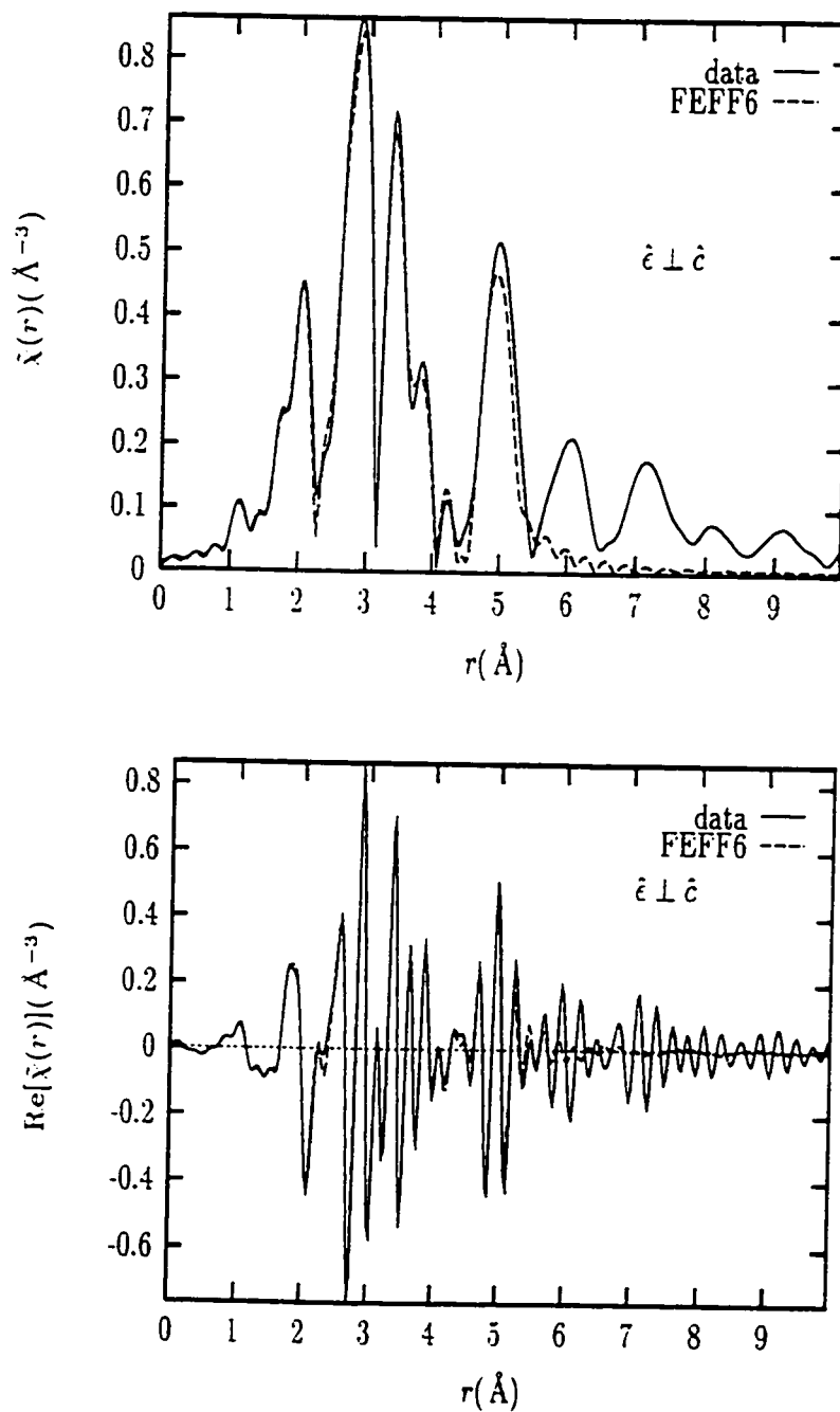
Figure 6.5: Fit results for the x = 0.125 sample at T = 10 K. The magnitude (top) and the real part (bottom) of the complex Fourier transform are shown for \hat{\epsilon} \perp \hat{c}
