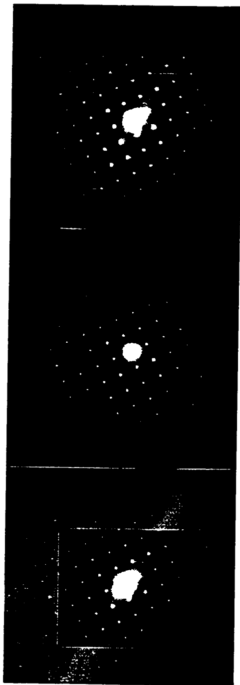
Figure 4.8: Sequence of selected area diffraction patterns at three different temperatures around 200K. From top to bottom: T=181\text{K} , 198\text{K} , 207\text{K} .
