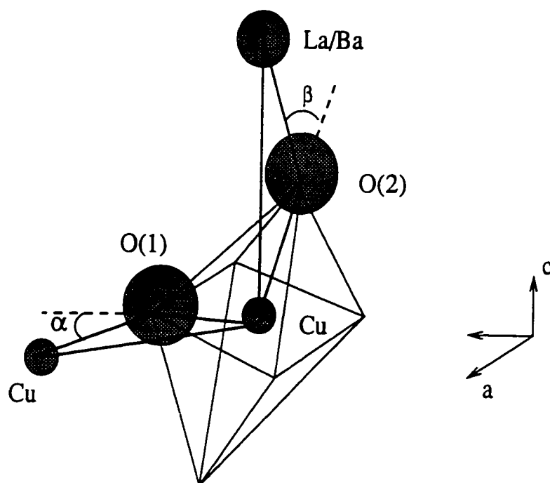
Figure 6.31: Schematic representation of the buckling angles \alpha and \beta determined from MS analysis of Cu-O(1)-Cu and Cu-O(2)-La signals using \widehat{aa} and \widehat{c} polarized Cu K -edge data.
