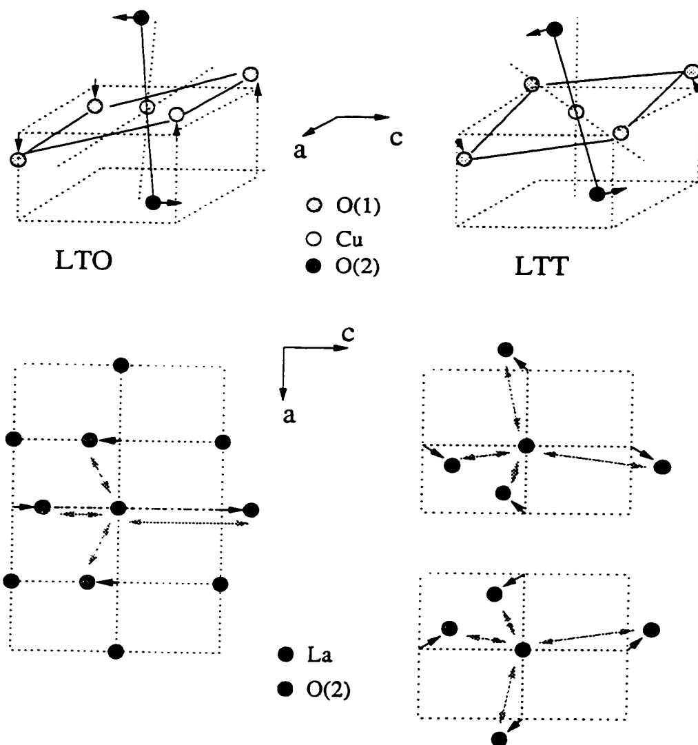
Figure 5.22: Atomic displacements associated with LTO and LTT types of tilts. The LTO tilts result in three different sets of La-O(2) planar distances while they are grouped in two sets of distances in the LTT tilts. The small correlated displacements of the La atoms are not shown. Dynamical fluctuations between the two equivalent LTT configurations will result in the average LTO tilts. Fluctuations between four equivalent LTT configurations will result in the HTT phase.
