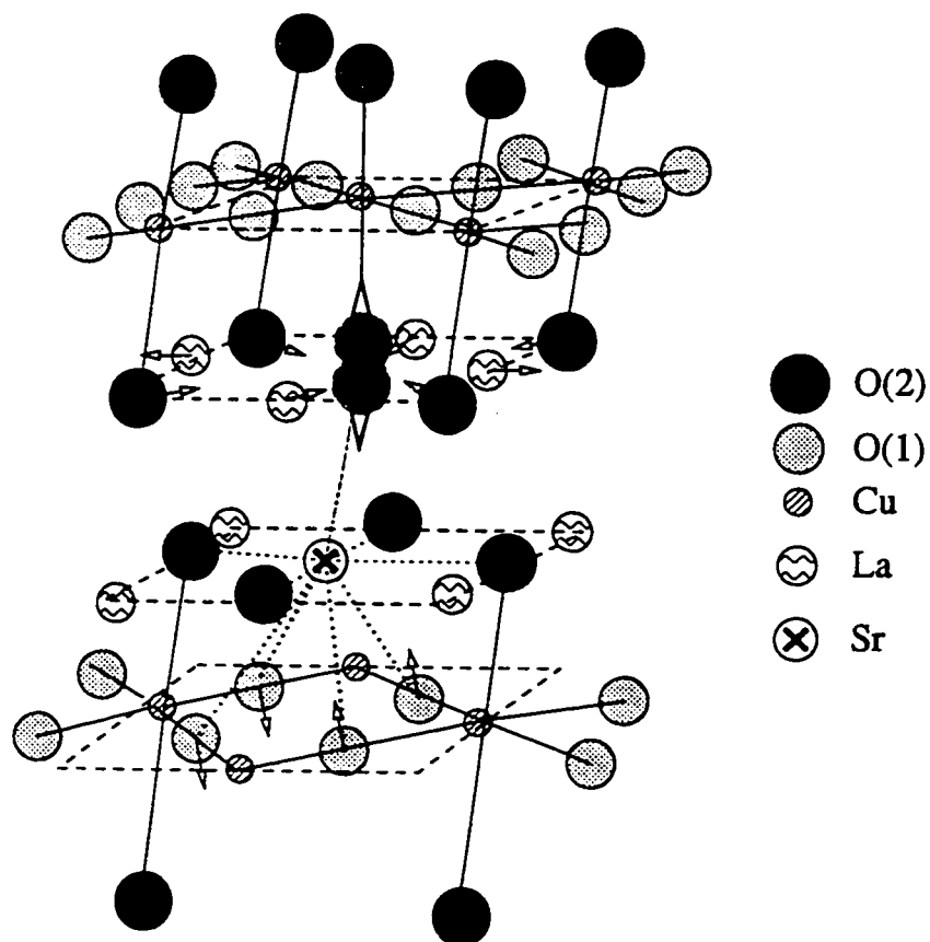
Figure 5.35: Schematic representation of the pattern of atomic displacements induced by Sr substitution in \text{La}_{2-x}\text{Sr}_x\text{CuO}_4 as determined by Sr K -edge XAFS. The arrows are intended as an approximate representation of the orientation of the actual atomic displacements.
