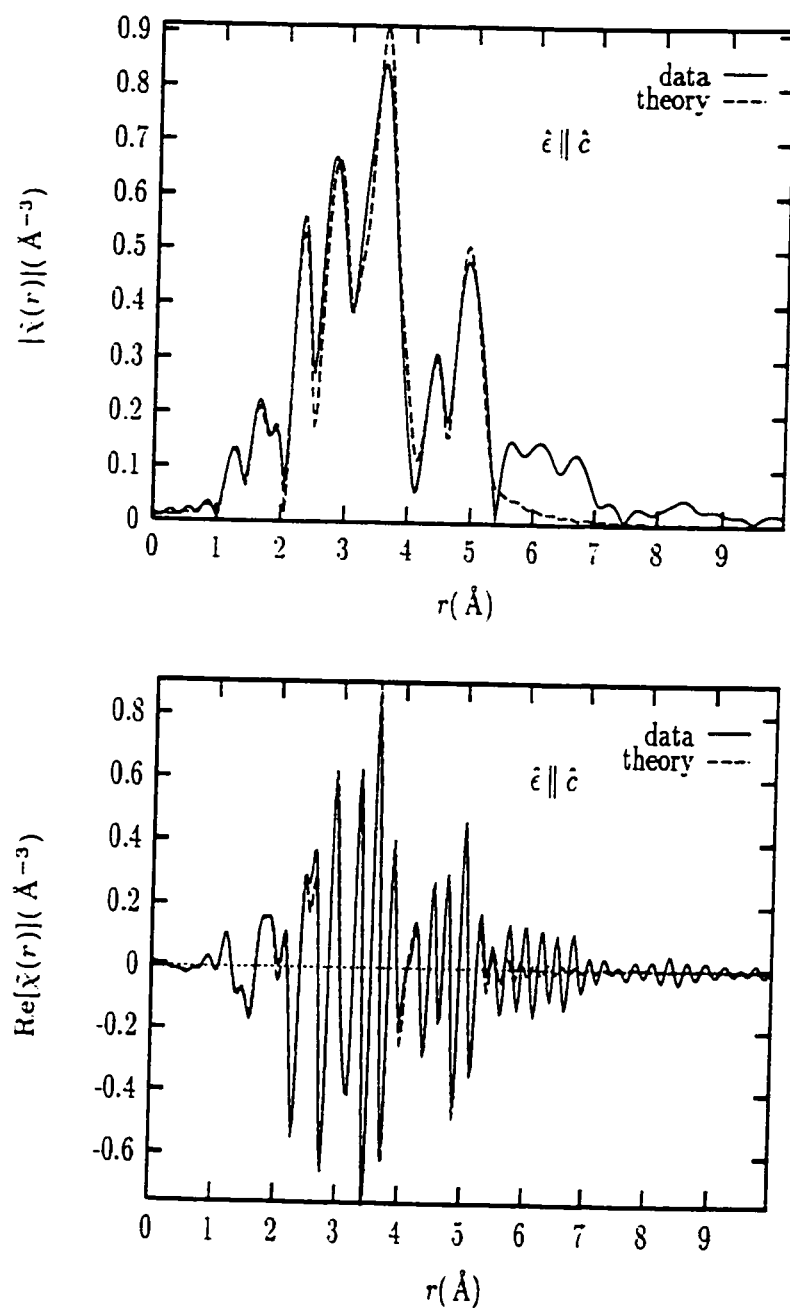
Figure 6.14: Fit results for the x = 0.15 sample at T = 10 K. The magnitude (top) and the real part (bottom) of the complex Fourier transform are shown for \hat{\epsilon} \parallel \hat{c}
