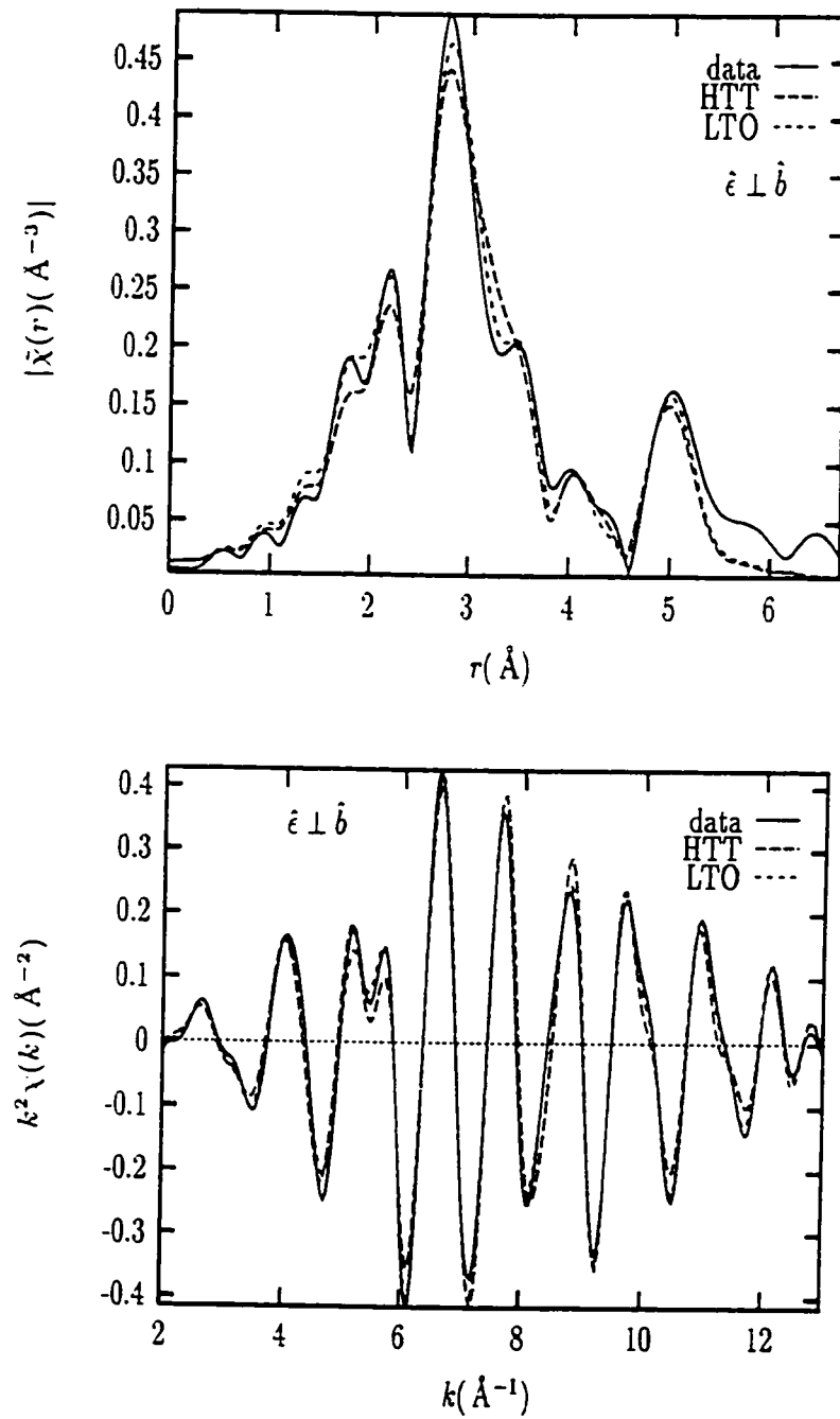
Figure 5.20: Fit results for x = 0.15 at 285K using both LTO and HTT models. LTO \rightarrow HTT phase boundary is at T=200 \pm 10\text{K} Top: magnitude of the complex Fourier transform; bottom: back Fourier transform of the fitted region of r -space. Data corresponds to \hat{\epsilon} \perp \hat{b} polarization.
