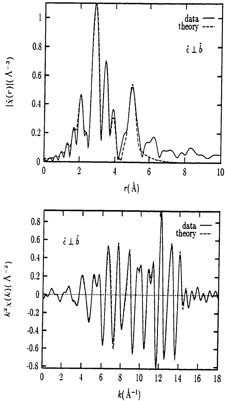
Figure 5.14: La K -edge fit results for x = 0.15 , \hat{\epsilon} \perp \hat{b} at T=20\text{K} . Top: Magnitude of the complex Fourier transform; bottom: back Fourier transform of the fitted region of r -space.
