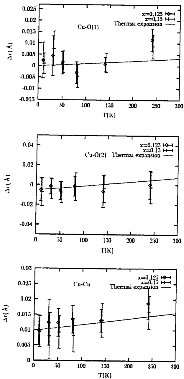
Figure 6.26: Fit results as obtained in the analysis of Cu K -edge polarized XAFS data for x = 0.125, 0.15 . From top to bottom: Cu-O(1), Cu-O(2), Cu-Cu distances. \Delta r is the measured change in distance relative to the diffraction results of Katano et. al [74], listed in tables 6.11 & 6.12. The slope of the thermal expansion lines are from reference 126. x = 0.15 results displaced by 2K for clarity.
