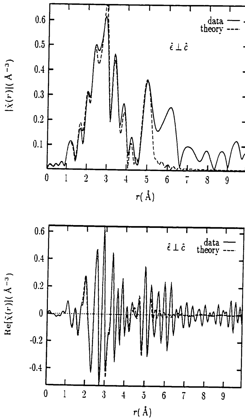
Figure 6.15: Fit results for the x = 0.15 sample at T=10 K. The magnitude (top) and the real part (bottom) of the complex Fourier transform are shown for \hat{\epsilon} \perp \hat{c}
