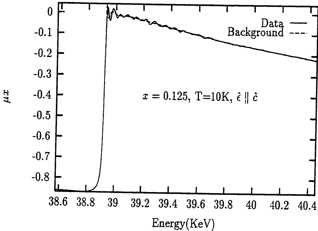
Figure 6.2: La K edge in \text{La}_{1.875}\text{Ba}_{0.125}\text{CuO}_4 at T=10\text{K} , \hat{c} -polarization
