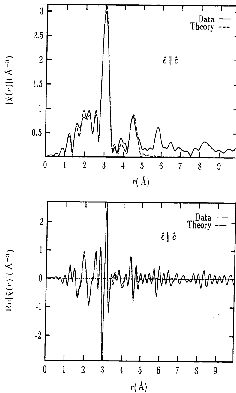
Figure 6.24: Fit results for the x = 0.15 sample at T=10 K. The magnitude (top) and the real part (bottom) of the complex Fourier transform are shown for \hat{\epsilon} \parallel \hat{c}
