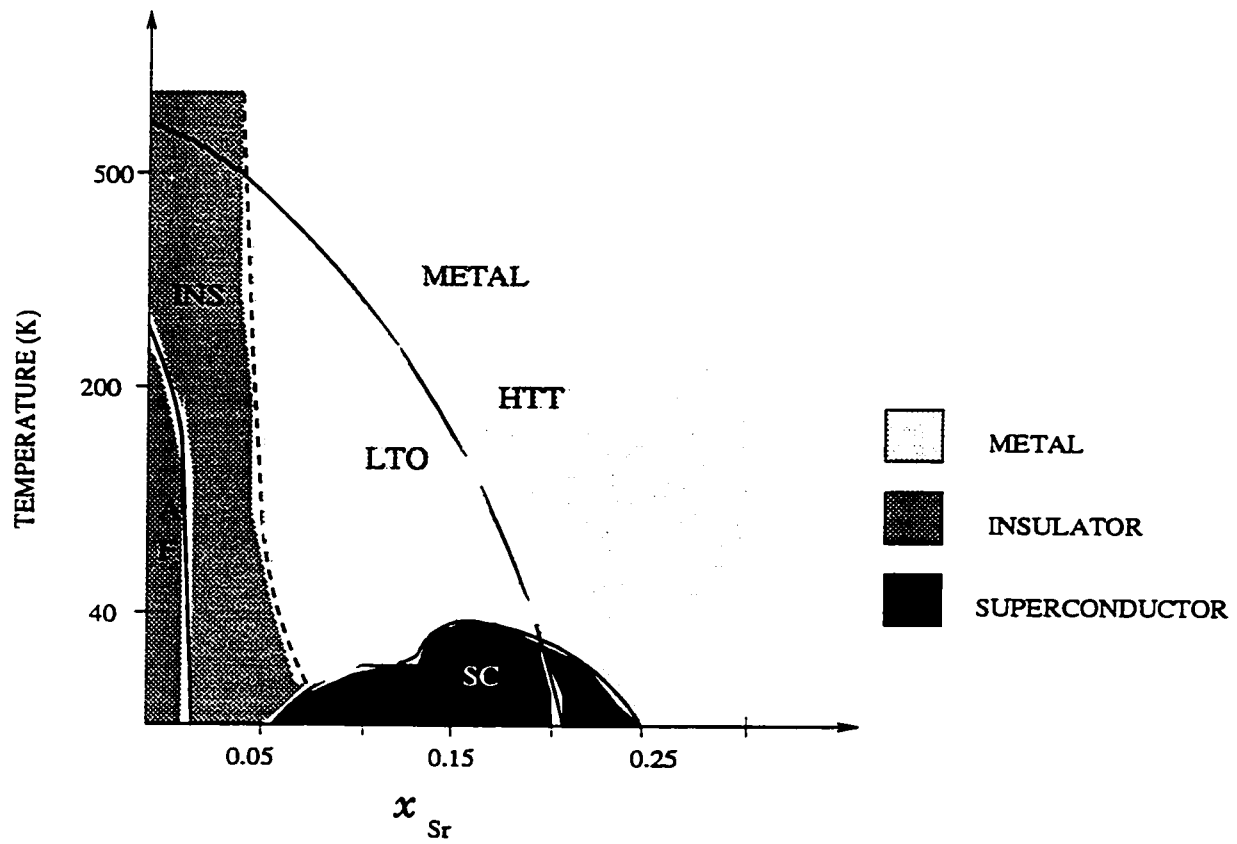
Figure 1.1: Phase diagram of \text{La}_{2-x}\text{Sr}_x\text{CuO}_4 in the temperature-doping plane. AF=Antiferromagnet, LTO and HTT stand for low temperature orthorhombic and high temperature tetragonal, respectively.
