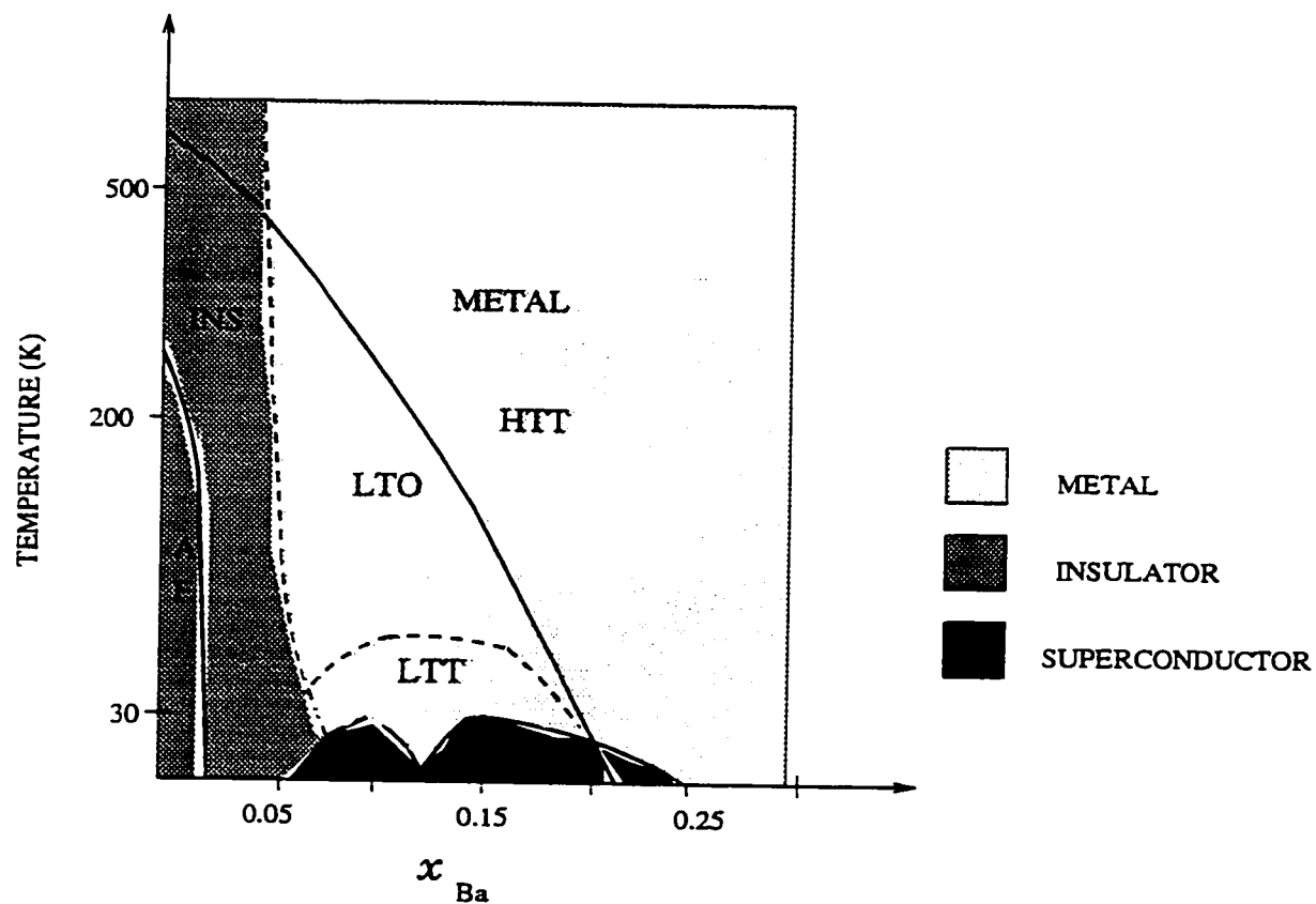
Figure 1.4: Phase diagram of \text{La}_{2-x}\text{Ba}_x\text{CuO}_4 in the temperature-doping plane. AF=Antiferromagnet, LTO, HTT and LTT stand for low temperature orthorhombic, high temperature tetragonal and low temperature tetragonal, respectively.
