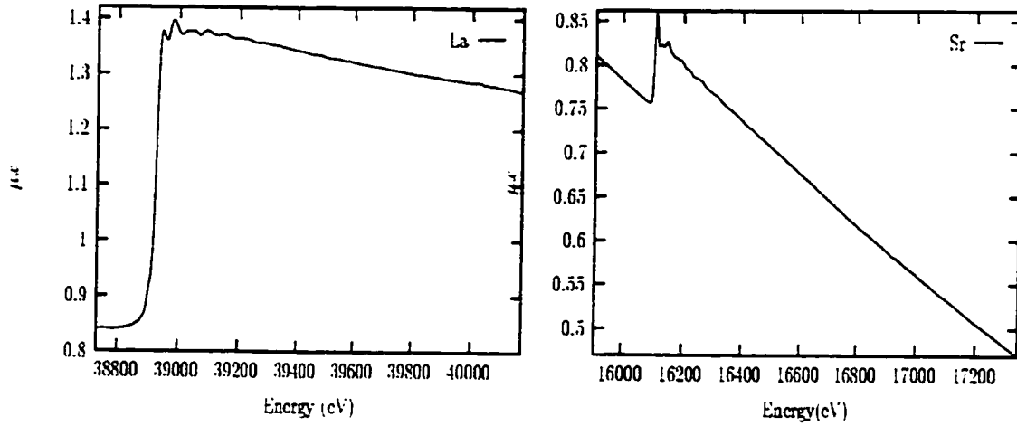
Figure 4.1: La and Sr K -edges in \text{La}_{1.85}\text{Sr}_{0.15}\text{CuO}_4 at T=300\text{K} , \hat{a}\hat{b} -polarization; \Delta\mu x = 0.54, 0.095 , respectively.
