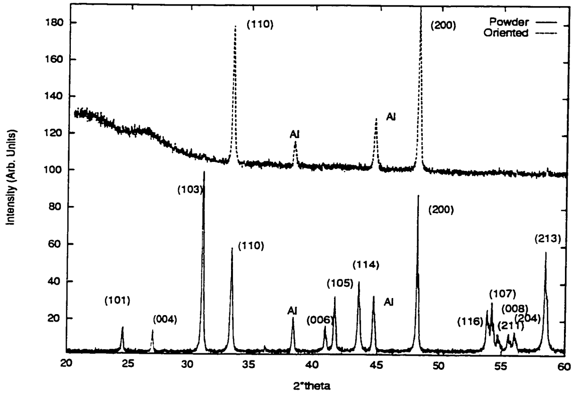
Figure 4.4: X-ray powder diffraction of \text{La}_{1.85}\text{Sr}_{0.15}\text{CuO}_4 before and after alignment.
