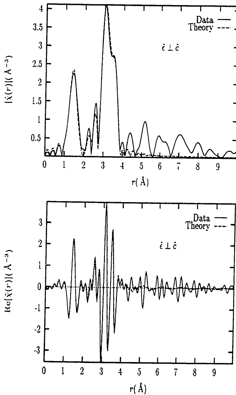
Figure 6.23: Fit results for the x = 0.125 sample at T=10 K. The magnitude (top) and the real part (bottom) of the complex Fourier transform are shown for \hat{\epsilon} \perp \hat{c}
