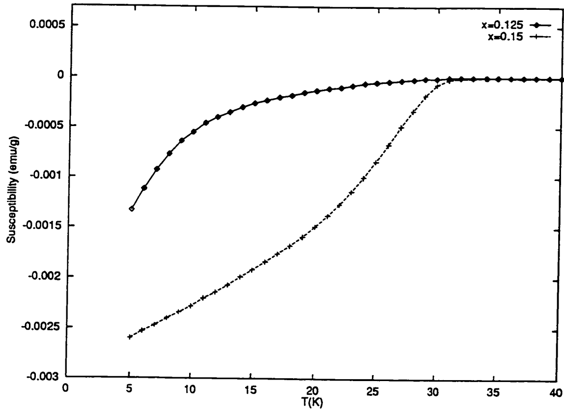
Figure 4.11: Zero field cooled magnetic susceptibility measurements on fine powder ( \sim 10\mu m ) of La_{2-x}Ba_xCuO_4 .
