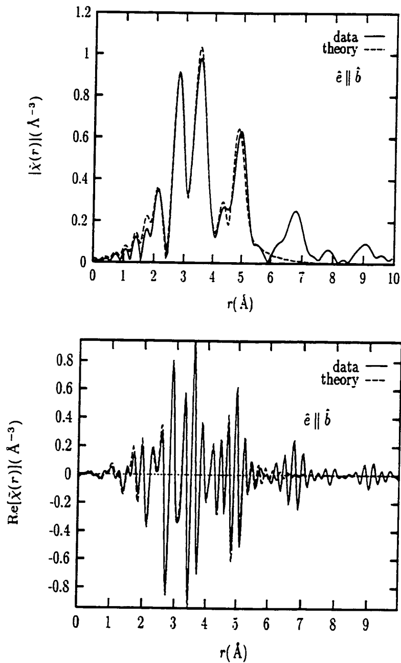
Figure 5.5: Fit results for the x = 0.075 sample at 20 K. The magnitude (top) and the real part (bottom) of the complex Fourier transform are shown for \hat{e} \parallel \hat{b}
