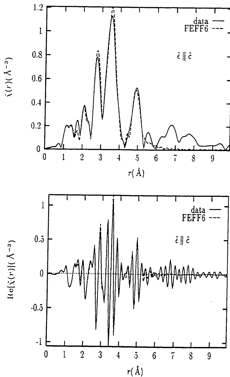
Figure 6.6: Fit results for the x = 0.15 sample at T = 10 K. The magnitude (top) and the real part (bottom) of the complex Fourier transform are shown for \hat{\epsilon} \parallel \hat{c}
