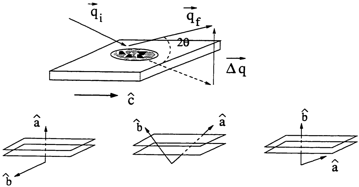
Figure 4.3: Scattering geometry used for checking the degree of magnetic alignment using powder x-ray diffraction.
