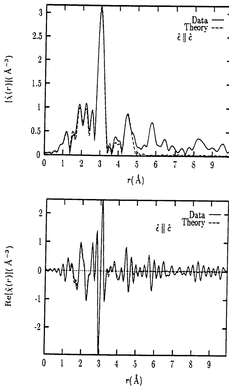
Figure 6.22: Fit results for the x = 0.125 sample at T=10 K. The magnitude (top) and the real part (bottom) of the complex Fourier transform are shown for \hat{\epsilon} \parallel \hat{c}
