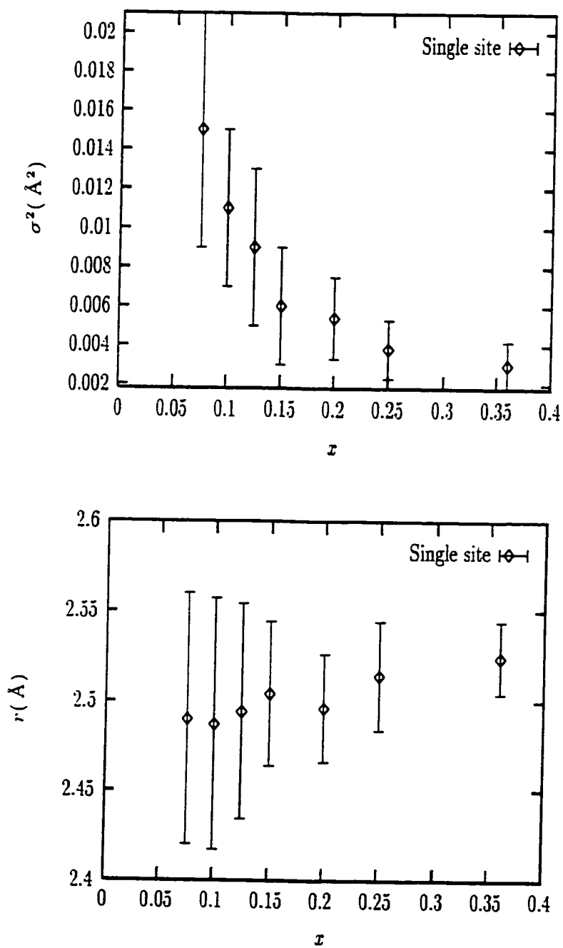
Figure 5.33: Fit results to the isolated O(2) apical signal with a single site model. The mean square-disorder (top) and the site distance (bottom) are shown as a function of Sr content.
