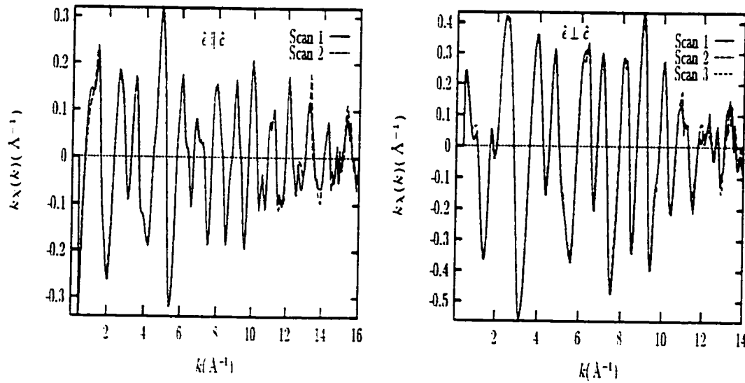
Figure 6.21: k\chi(k) reproducibility data for Cu K -edge, x = 0.125 in \text{La}_{2-x}\text{Ba}_x\text{CuO}_4 at T=10\text{K} . Left: \hat{c} -polarization; right: in-plane, \widehat{a\bar{a}} -polarization
