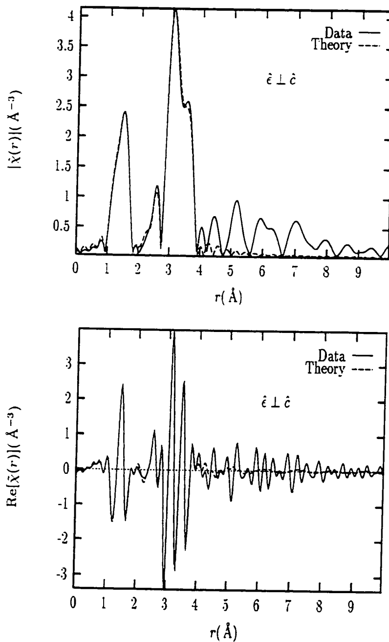
Figure 6.25: Fit results for the x = 0.15 sample at T = 10 K. The magnitude (top) and the real part (bottom) of the complex Fourier transform are shown for \hat{\epsilon} \perp \hat{c}
