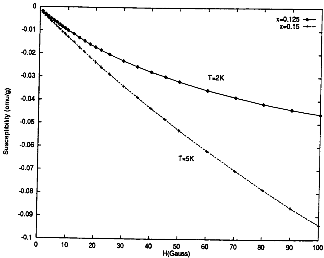
Figure 4.12: M/H curves on the \text{La}_{2-x}\text{Ba}_x\text{CuO}_4 system used to estimate the superconducting volume fraction of the samples.
