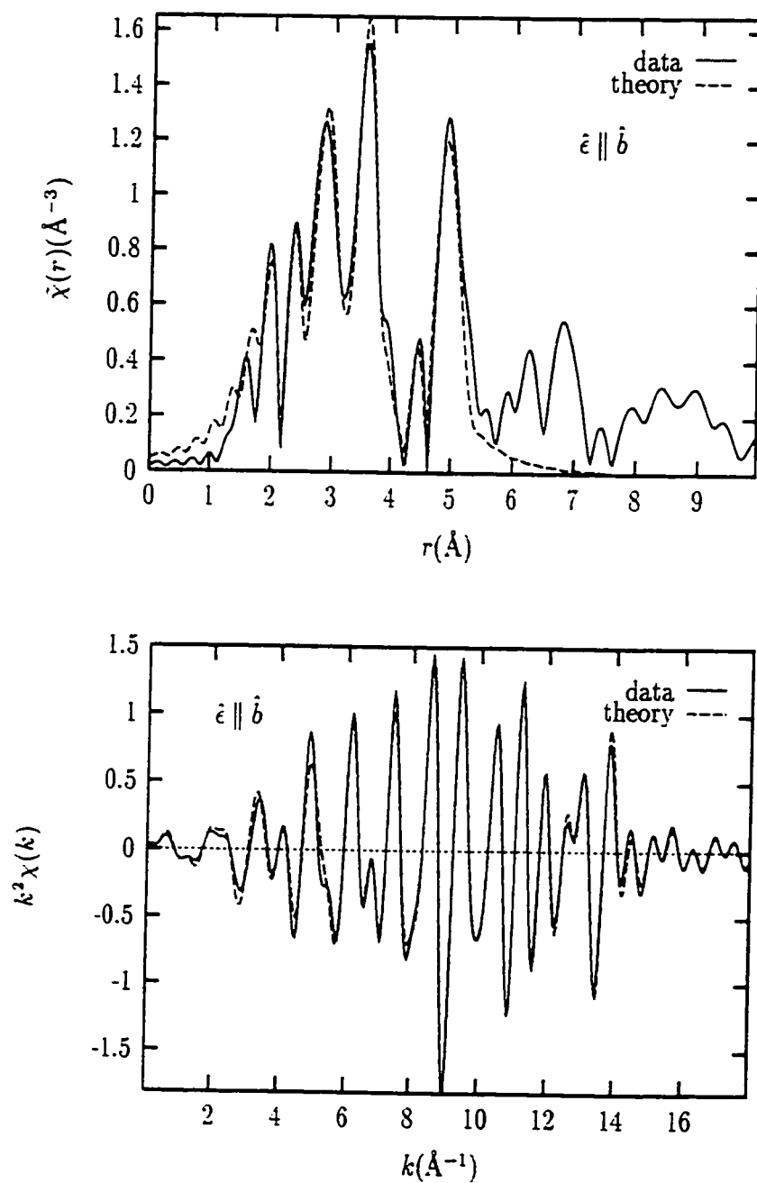
Figure 5.26: Sr K -edge fit results for x = 0.1 , \hat{\epsilon} \parallel \hat{b} at T=17\text{K} . Top: Magnitude of the complex Fourier transform; bottom: back Fourier transform of the fitted region of r -space.
