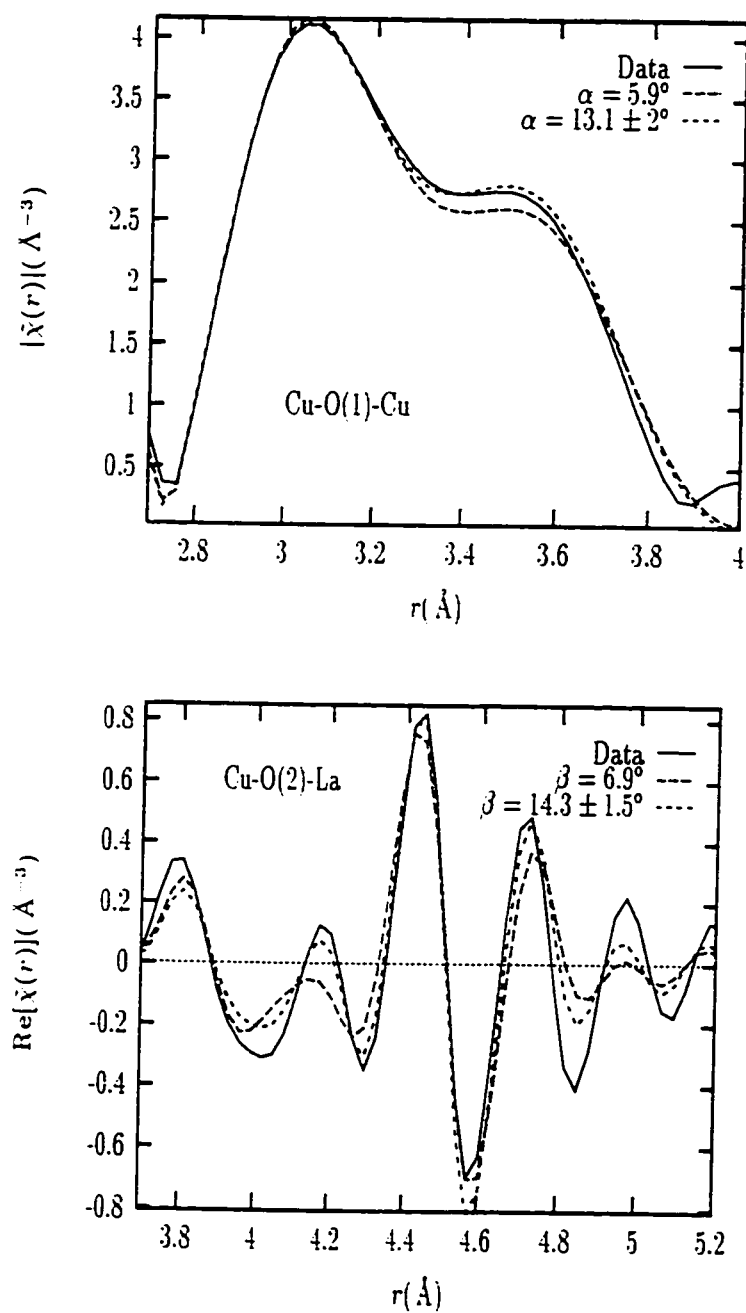
Figure 6.33: Comparison between the two models described in the text. Top: Cu-O(1)-Cu signal; bottom: Cu-O(2)-La signal. The region of r space fitted is emphasized. The improvement obtained by varying the buckling angle is readily seen. Fits here correspond to x = 0.125 at T=10\text{K} .
