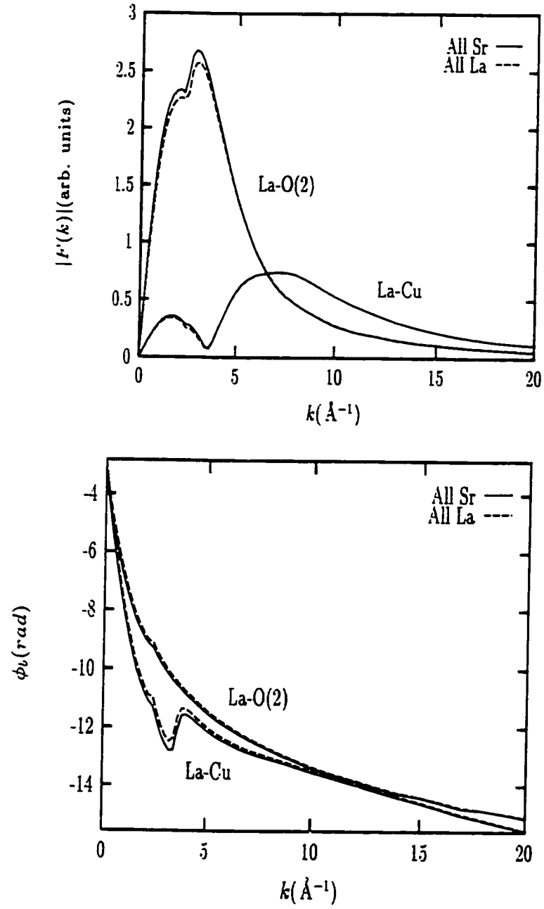
Figure 5.4: FEFF6 Backscattering amplitudes and phases for La-O(2) and La-Cu SS paths for all La atoms in the La/Sr sites vs. all Sr atoms (except of course the La central atom) in \text{La}_{2-x}\text{Sr}_x\text{CuO}_4 . Calculation corresponds to x = 0.075 and \hat{b} polarization.
