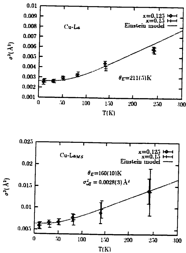
Figure 6.29: Fit results as obtained in the analysis of Cu K -edge polarized XAFS data for x = 0.125, 0.15 . From top to bottom: Cu-La, Cu-La MS XAFS Debye Waller factors. Fits of the disorder in bond length (using x = 0.125 data) to an Einstein model also shown. Einstein temperatures together with the additional static disorder \sigma_{\text{off}}^2 required (when shown) in fitting the data also shown. x = 0.15 results displaced by 2K for clarity.
