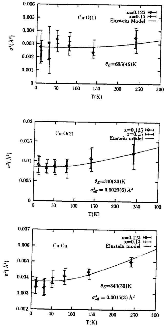
Figure 6.28: Fit results as obtained in the analysis of Cu K -edge polarized XAFS data for x = 0.125, 0.15 . From top to bottom: Cu-O(1), Cu-O(2), Cu-Cu XAFS Debye Waller factors. Fits of the disorder in bond length (using x = 0.125 data) to an Einstein model also shown. Einstein temperatures together with the additional static disorder \sigma_{\text{off}}^2 required (when shown) in fitting the data also shown. x = 0.15 results displaced by 2K for clarity.
