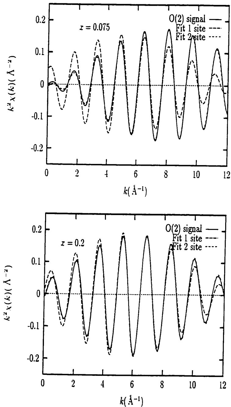
Figure 5.32: Fits to the isolated O(2) signal with single site and double site models. The improvement of the double site model decreases with x , in agreement with the changes in site occupancy shown in fig. 5.34
