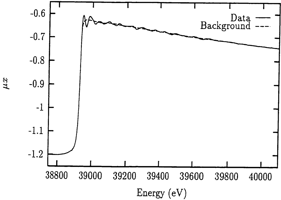
Figure 5.2: La K edge in \text{La}_{1.8}\text{Sr}_{0.2}\text{CuO}_4 at T=20\text{K} , \hat{b} -polarization
