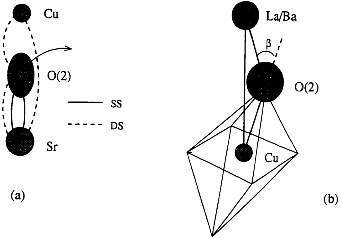
Figure 2.3: Two examples in which MS XAFS is exploited to solve structural issues. (a) Occupancy of highly disordered O(2) atom neighboring Sr, (b) Tilt angle of CuO 6 octahedra in La 2-x Ba x CuO 4 with x = 0.125 .
