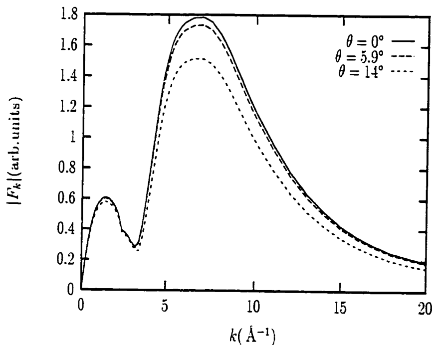
Figure A.9: F_k dependence on \theta for the Cu-O(1)-Cu DS path.
