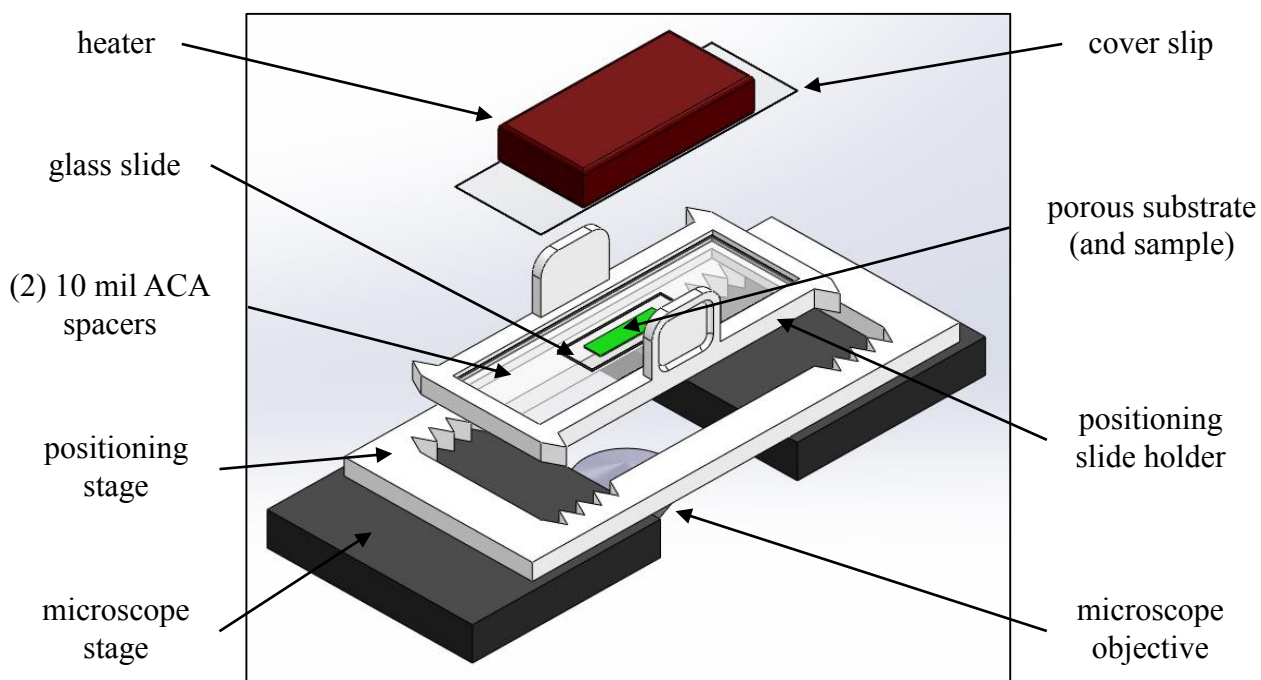
Figure 29. Experimental set-up for visualizing real-time amplification from dry reagents on the microscope.
