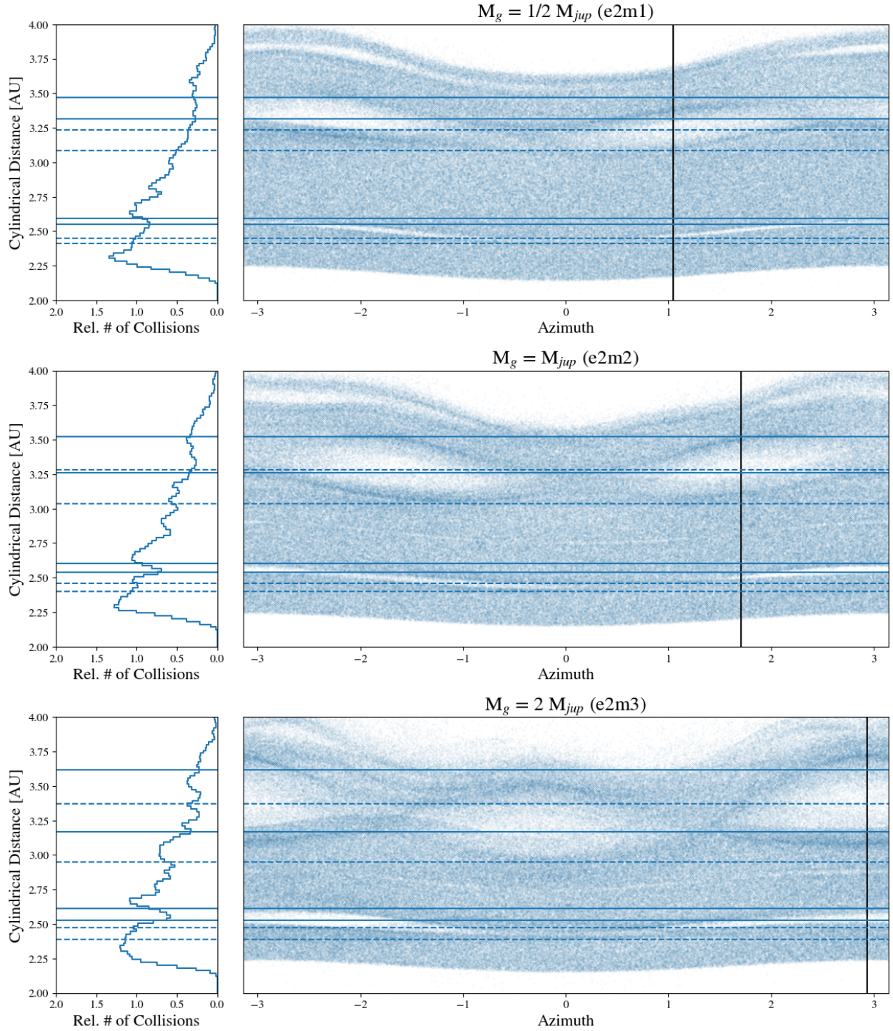
Figure 3.8: Similar to Figure 3.7, except the eccentricity of the planet is kept constant and the mass is varied. This has the effect of changing the width of the resonances, without altering the relative apo or peri distances of bodies near the edges. Except for the highest mass case, the apocenter and pericenter distances of the inner and outer edges of the 2:1 resonance are too close together to produce much of a dip or a bump feature.
