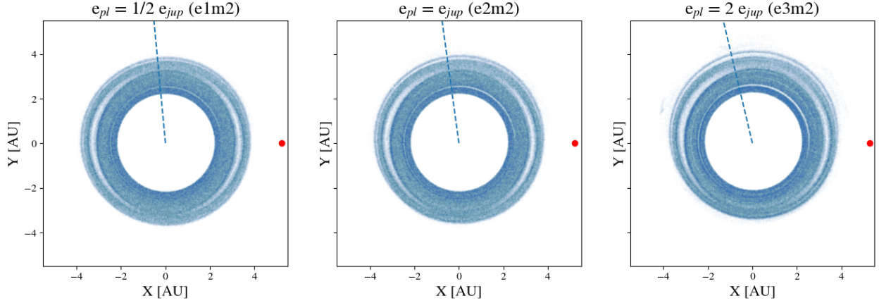
Figure 3.1: The positions of the remaining planetesimals at the end of the e1m2 (left), e2m2 (center) and e3m2 (right) simulations. The red dot indicates the position of the giant planet, and the dashed line points in the direction of the planet’s longitude of perihelion. Non-axisymmetric gaps are apparent near the locations of MMRs. At higher eccentricities, more resonances become visible. At the 2:1 MMR, gap features at \theta = 0 and \theta = \pi follow the giant planet in its orbit.
