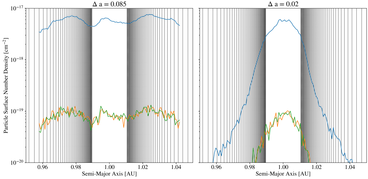
Figure 2.8: Number density profiles of the planetesimals at the end of the e_{hi} (left) and e_{narrow} simulations (right). The blue curves represent the number density of planetesimals less massive than the resonance heating mass ( 2 \times 10^{22} g) and the orange curves represent the number density of planetesimals above this mass. The green curves show the surface number density of planetesimals randomly drawn from the low mass bin, such that the total number of bodies matches that of the high mass bin. The vertical lines indicate the positions of first order mean motion resonances with an embryo at 1 AU.
