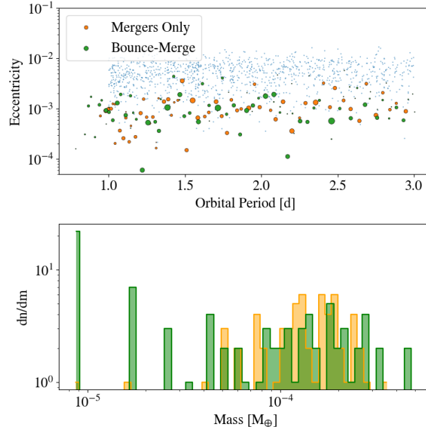
Figure 4.13: A comparison between the innermost region of the fdLo (orange) simulation, and a second version using a bounce-merge collision model (green). In the top panel, the period-eccentricity state of the particles is shown, with marker sizes indicating relative mass. The blue points represent the initial state of the simulations. The bottom panel compares the final differential mass distributions of the bodies.
