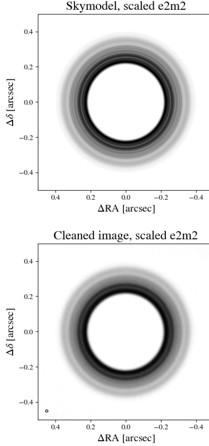
Figure 3.9: Simulated ALMA observations for the nominal (e2m2) case, operating under the assumption that the dust profile closely traces the planetesimal collision profile. Top: The sky model based on the radial collision distribution. The size of the disc has been scaled by a factor of 10 and placed at a distance of 100 pc. Bottom: The cleaned image using combined observations in configurations 8, 9, and 10. The circle in the bottom left indicates the simulated beam size. Gaps in the dust due to the 3:1 and 2:1 resonances are visible.
