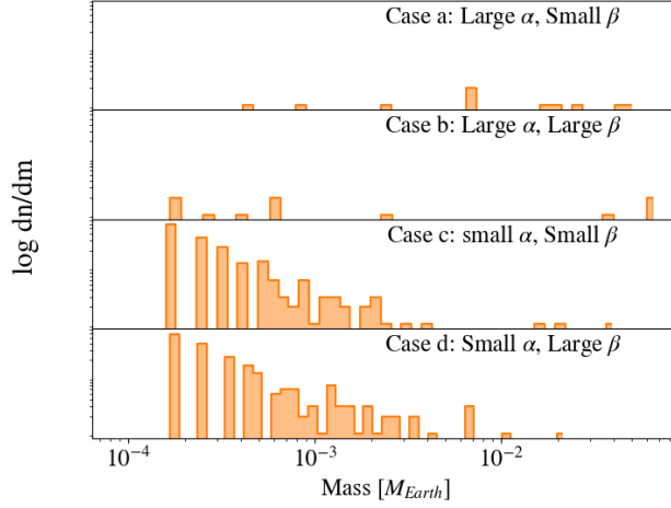
Figure 4.4: The final state of the mass distributions for the narrow annulus simulations described in section 4.4. For small \alpha , a few embryos form alongside a power law tail of planetesimals. For larger values of \alpha , the mass distribution stops being bimodal. As in the previous figure, the initial choice of \beta does not appear to have any meaningful impact on the end result.
