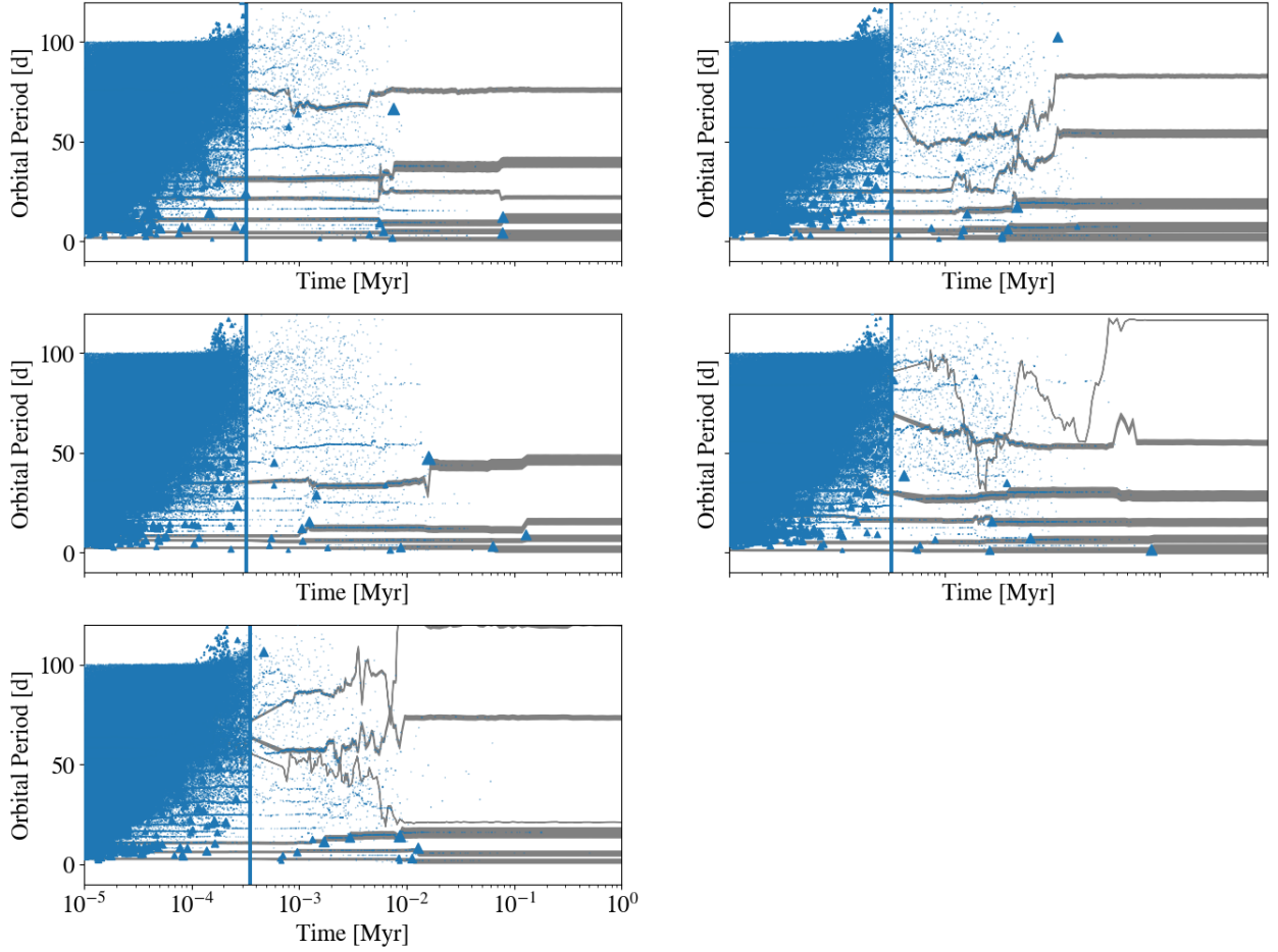
Figure 5.2: The evolution of the orbits of some of the last surviving bodies in the \delta = 1.5 simulations. Collisions are indicated with triangles, where the size denotes the relative mass of the body that was consumed in the merger. Gray curves indicate bodies which survived through the end of the simulation and the line width indicates their relative mass. The vertical blue line marks the time at which the CHANGA snapshots were passed to GENGA.
