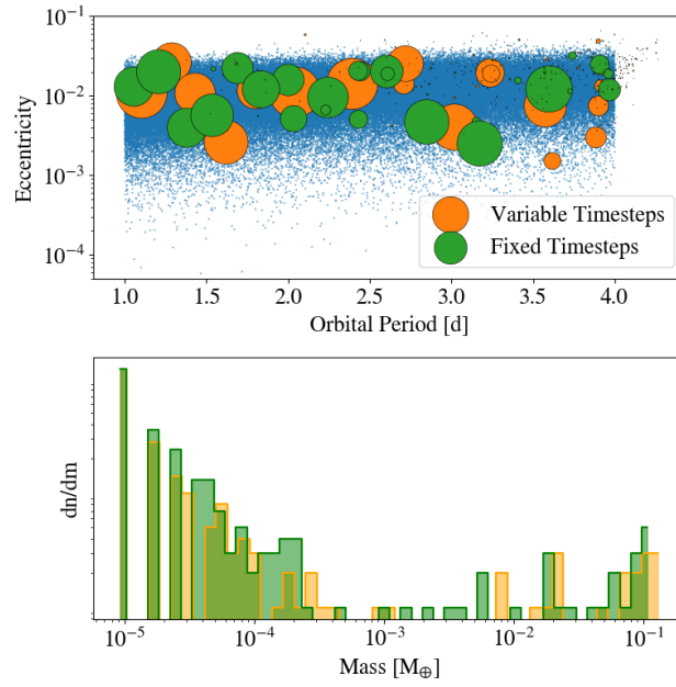
Figure 4.15: A comparison between the innermost region of the fdHi (orange) simulation, and a second version using a fixed timestep appropriate for the inner edge of the disk (green). In the top panel, the period-eccentricity state of the particles is shown, with marker sizes indicating relative mass. The blue points represent the initial state of the simulations. The bottom panel compares the final mass distributions of the bodies.
