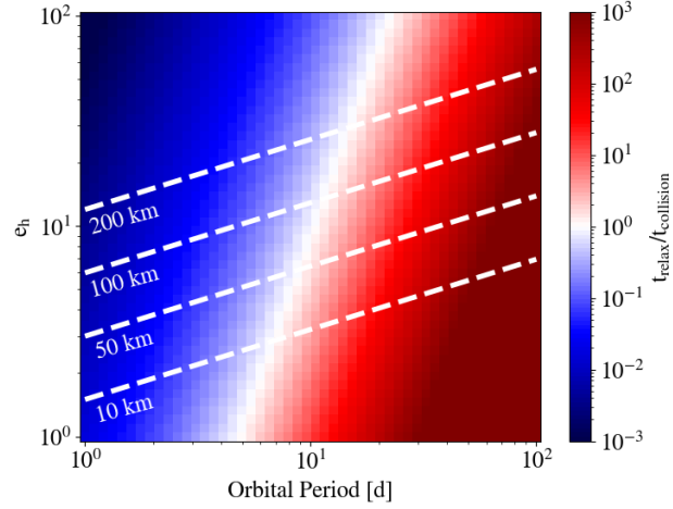
Figure 4.1: The ratio between the two-body relaxation and collision timescale for a population of equal-mass planetesimals with an internal density of 3 \text{ g cm}^{-3} . The dashed curves show the value of e_h for which the random velocity dispersion is equal to the escape velocity of the planetesimals for a range of sizes. Only in regions where t_{\text{relax}} \gg t_{\text{coll}} can the velocity distribution respond to changes in the mass of the bodies such that oligarchic growth can operate. This condition is no longer satisfied for a dynamically hot disk at sufficiently short orbital periods.
