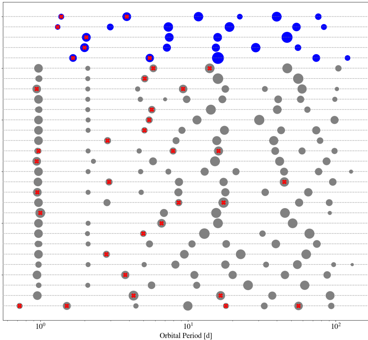
Figure 5.14: Final orbital architectures of planetary systems formed in the full (blue points) and isolation mass (gray points) simulations. Point sizes indicate relative masses. Bodies which underwent a collision where v_{coll}/v_{mut,esc} > 2 with a > 0.1 M_{\oplus} body are marked with a red X.
