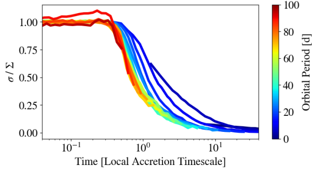
Figure 4.7: The time evolution of the planetesimal surface density (in units of the total solid surface density) in the fdHi simulation. Each curve represents a radial slice of the disk. The time is measured in units of the local accretion timescale at the center of each radial zone. The colors represent the orbital period at the center of each zone.
