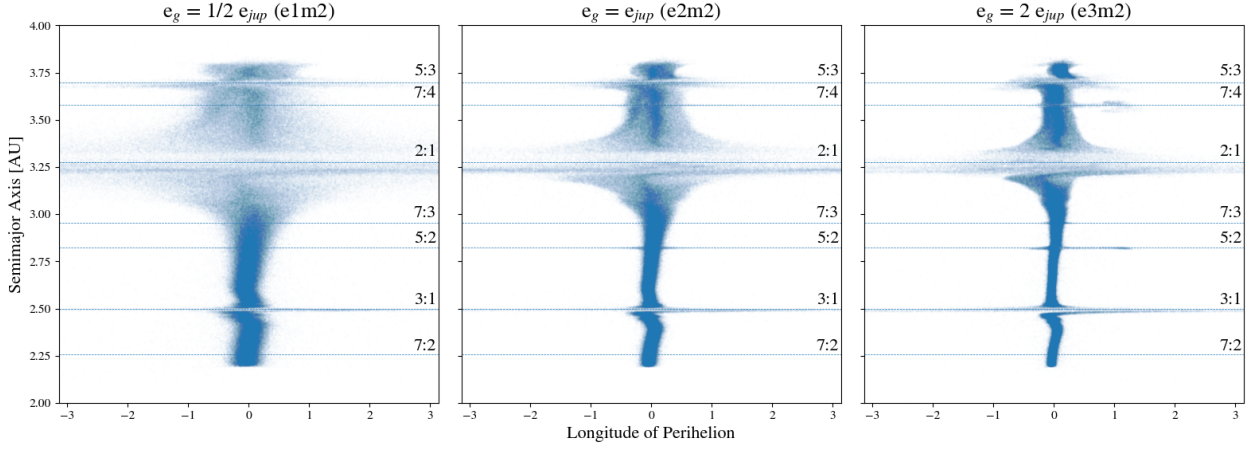
Figure 3.3: Shown here are the longitudes of pericenter and semimajor axes of the remaining planetesimals. The dashed lines again indicate the locations of prominent MMRs. Close to the resonances, the critical angle librates and drives fast precession of the longitudes of pericenter of the bodies. This overpowers the secular forcing by the planet and effectively randomizes the orientations of their orbits.
