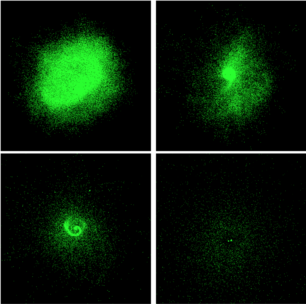
Figure 1.1: Simulation snapshots of a gravitationally bound pebble cloud formed via the streaming instability. Over the course of about 50 years (top left to bottom right), the clump collapses to form a binary planetesimal. (Adapted from figure 14 of [210])
