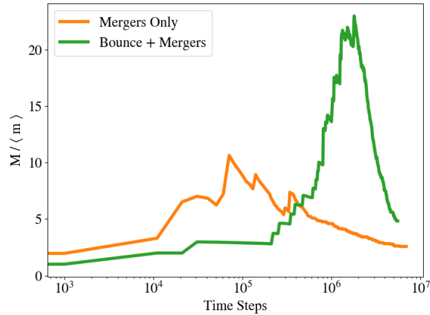
Figure 4.14: The evolution of the ratio between the maximum and mean mass of the simulations shown in figure 4.13. In both cases, the system first evolves through a phase of runaway growth, before the massive bodies consume the smaller bodies, driving down the mean mass. With the bounce-merge model, the mass ratio takes much longer to begin decreasing.
