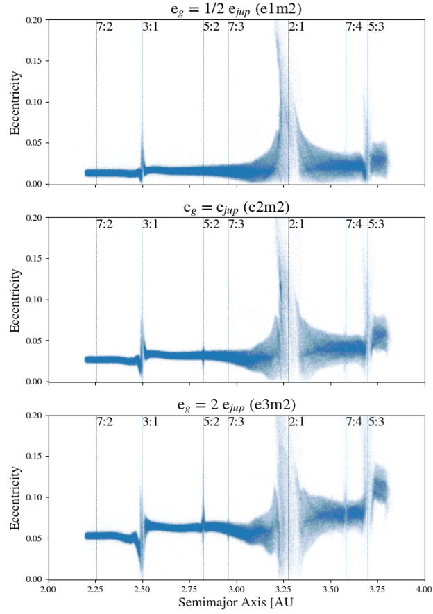
Figure 3.2: The semimajor axes and eccentricities of the remaining planetesimals are shown, with the locations of prominent resonances indicated by the vertical dashed lines. Libration of the critical angle drives large variations in eccentricity, which produce spikes in the a - e plane. Between the resonances, the nonzero eccentricity is due to secular forcing by the planet.
