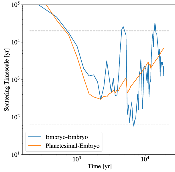
Figure 2.7: The mean scattering time-scale for embryo-embryo (blue curve) and planetesimal-embryo (orange curve) interactions over the course of the high resolution growth simulation. The dashed lines correspond to the simulation time-scale (upper) and longest relevant mean motion resonance time-scale (lower), which is set by the 65:64 resonance.
