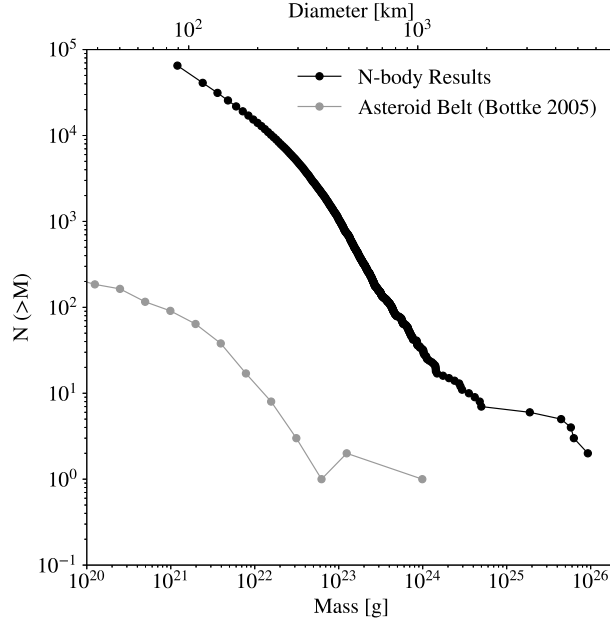
Figure 2.12: A comparison between the cumulative number of objects in our high resolution growth simulation (black curve) and the present day asteroid belt [33] (gray curve) as a function of size and mass.
