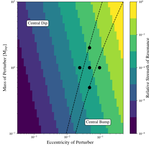
Figure 3.11: The presence of a dip or bump in the collision profile (and therefore the dust profile) near the 2:1 MMR can be used to constrain the mass and eccentricity of the perturbing planet. The color scale indicates the relative strength of the features, while the dashed lines indicate boundaries in parameter space where a dip or a bump will be produced at the resonance. Combinations of mass and eccentricity that fall between the dashed lines correspond to an inner apocenter and outer pericenter separation at the edges of the resonance that is smaller than the resonance width and therefore will not create any significant feature in the collision profile.
