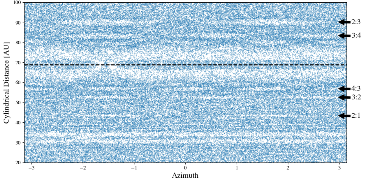
Figure 3.12: Positions of planetesimals at the end of the simulation presented in [30] in polar coordinates. The dashed line marks the location of a 50 M_{\oplus} planet embedded in the disc. First order MMRs with the planet are indicated with arrows. A second planet is also present at 32.3 au, although it is not massive enough to induce any significant structure in the disc near associated resonances.
