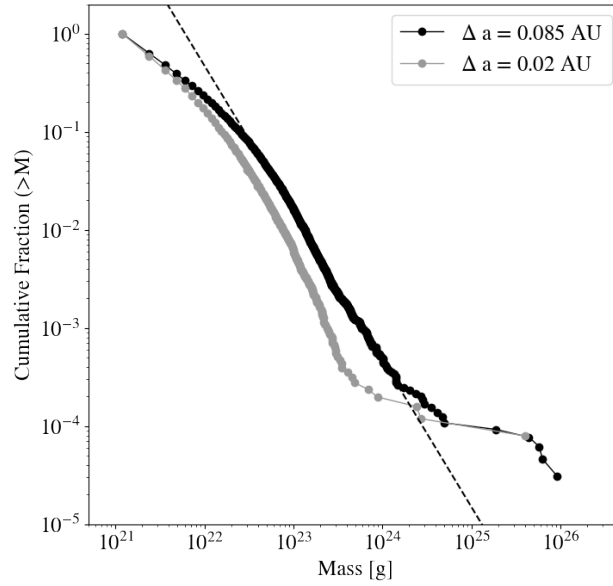
Figure 2.6: The cumulative fraction of bodies as a function of mass in the wide (solid dark curve) and narrow (gray curve) high resolution growth simulations. Decreasing the annulus width, which depopulates resonances, produces a less prominent 10^{22} g bump. The dashed black line shows the mass spectrum predicted by a runaway growth scenario using the coagulation equation [178, 262].
