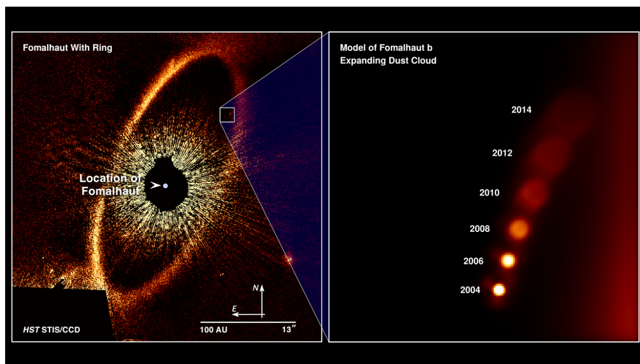
Figure 1.2: A composite of archival images from the Hubble Space Telescope showing dust in scattered light surrounding the Fomalhaut system. On the right, a closeup view of the model of the expanding dust cloud, produced by a planetesimal collision is shown expanding over the course of 10 years. Image credit: NASA/ESA
