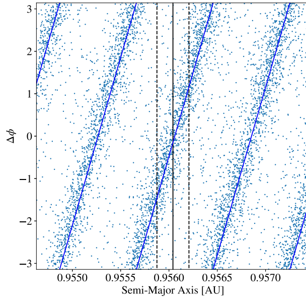
Figure 2.10: The change in the resonant argument for the oligarch and planetesimals near the 15:14 MMR over a 50 year time interval from the e_{hi} simulation. The solid vertical line designates the nominal resonance location and the dashed vertical lines indicate the minimum libration width. The diagonal blue lines represent the change in \phi due to the Keplerian shear of the disc, which is calculated analytically.
