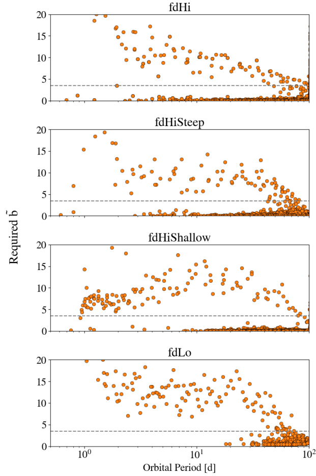
Figure 4.9: Feeding zone width (see equation 5.2) required to produce the final masses for the protoplanets from the simulations listed in table 4.1. For the fdHi, fdHiSteep and fdHiShallow simulations, we have included the results from five separate iterations of the simulations, each using a different random number seed. The horizontal dashed line indicates \tilde{b} = 2\sqrt{3} . Despite the vastly different initial solid surface density profiles, the feeding zone width reaches the circular orbit value around \sim 60 days in all cases.
