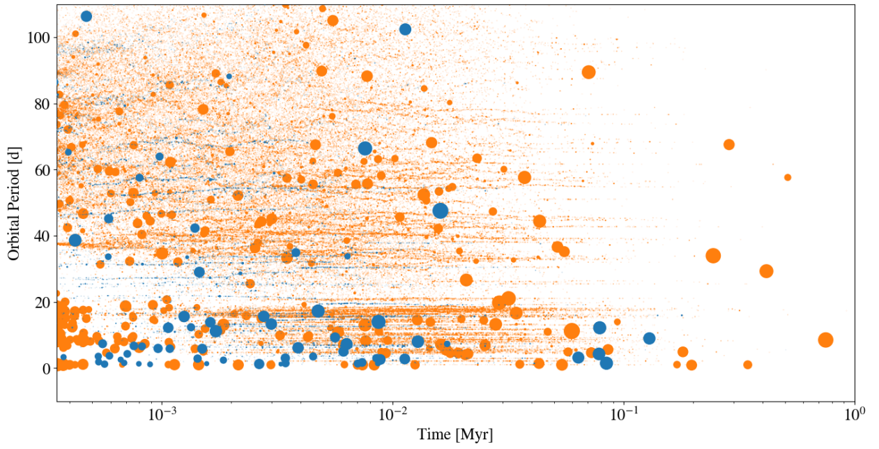
Figure 5.11: The combined timing and location of collisions from all versions of the full (blue) and synthetic (orange) simulations. Point sizes indicate the relative masses of bodies consumed in each merger. Collisions from the CHANGA phase of the full simulations are not shown.
