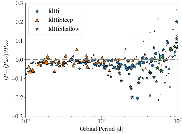
Figure 4.11: The relative separation between the final period of a body and the mean orbital periods of its accretion zone at the end of the fdHi, fdHiSteep and fdHiShallow simulations. The marker type and color denotes the simulation used, while the marker sizes indicate the relative masses of bodies. In each case, all five iterations of the simulations are plotted simultaneously.
