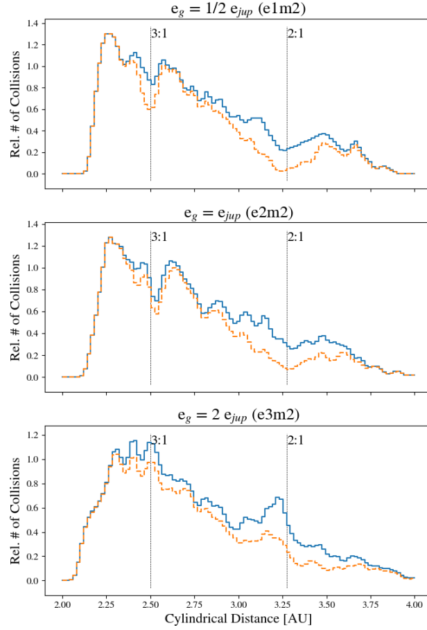
Figure 3.6: Here, collisions are instead ordered by cylindrical distance from the star. Features near the 3:1 and 2:1 MMRs are still present, but appear qualitatively different than in semimajor axis space. At low eccentricities, a dip appears around the center of the resonance. At the highest eccentricity, a bump is formed instead. The dashed lines shown the collision profile with collisions between bodies in resonance removed. The bump and dip features remain qualitatively the same, which suggests that they are produced by bodies outside of the libration width of the resonance.
