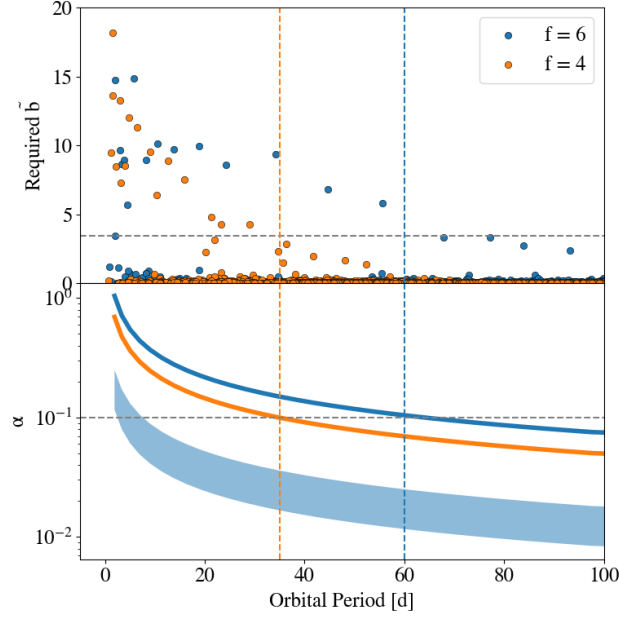
Figure 4.12: In the top panel, we show the required feeding zone sizes to produce the masses of the bodies seen at the end of the fdHi and fdHif4 simulations. The bottom panel shows the variation of \alpha with orbital period for the bodies used in each case (solid curves). The orbital period at which \alpha \simeq 0.1 matches well with the location at which \tilde{b} exceeds 2\sqrt{3} . This is highlighted by the vertical dashed lines. The shaded region in the bottom panel shows the values of \alpha for realistic-sized ( f = 1 ) planetesimals with bulk densities between 10 and 1 \text{ g cm}^{-3} .
