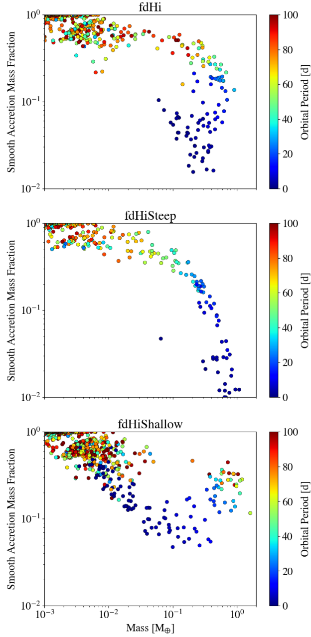
Figure 4.10: For all bodies with m > 100m_0 at the end of the high surface density simulations, the fraction of their total mass attained through mergers with initial mass planetesimals (smooth accretion) as a function of total mass. Colors indicate the orbital periods of the bodies in the final simulation snapshot. Bodies interior to \sim 20 to 30 days attain up to an order of magnitude less of their mass through minor merger events, while accretion of planetesimals plays a much more significant role at longer orbital periods.
