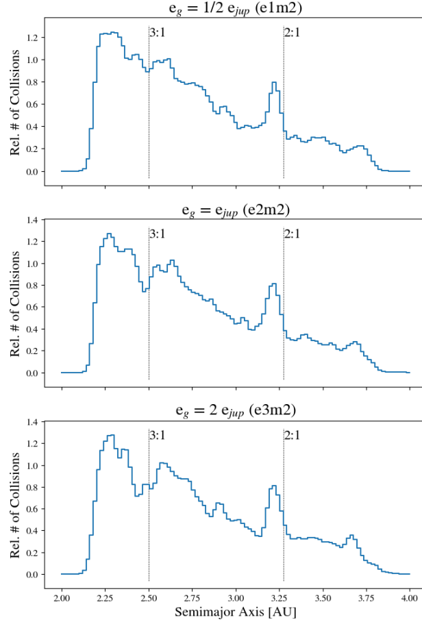
Figure 3.4: A PDF of the collision rate in each disc as a function of semimajor axis, generated using a KDE with a Gaussian kernel with a FWHM of 0.02 au. In semimajor axis space, prominent features appear near the 3:1 and 2:1 MMRs. Near the 3:1, the collision rate exhibits a local minimum, while an enhancement appears near the 2:1.
