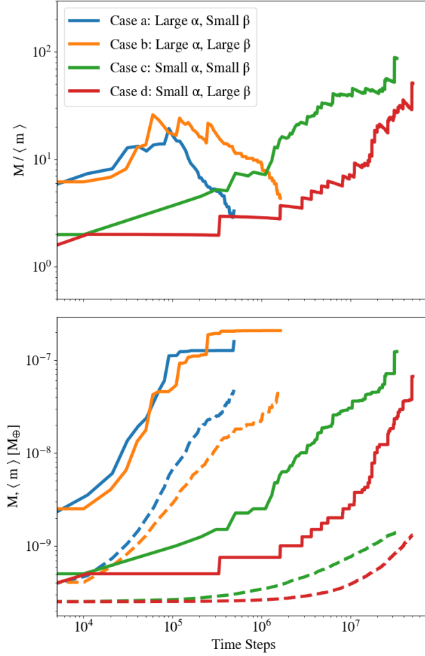
Figure 4.5: Top: The evolution of the ratio between the maximum and mean mass for the four simulations presented in section 4.4. The runaway growth phase can be identified by a positive trend in this ratio. For all values of \alpha , an increase in \beta has the effect of delaying runaway growth. Bottom: The evolution of the maximum (solid lines) and mean (dashed lines) shown individually.
