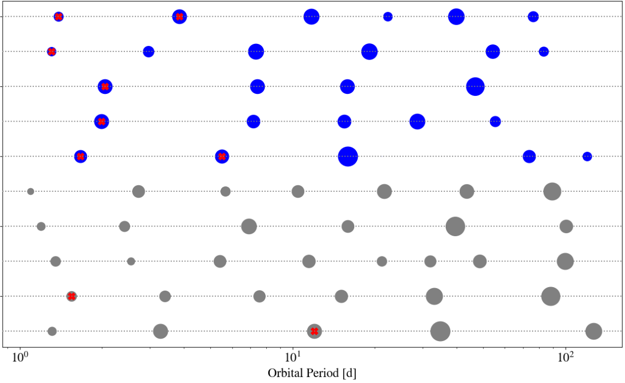
Figure 5.8: Final orbital architectures of planetary systems formed in the full (blue points) and isolation mass (gray points) simulations. Point sizes indicate relative masses. Bodies which underwent a collision where v_{coll}/v_{mut,esc} > 2 with a > 0.1 M_{\oplus} body are marked with a red X.
