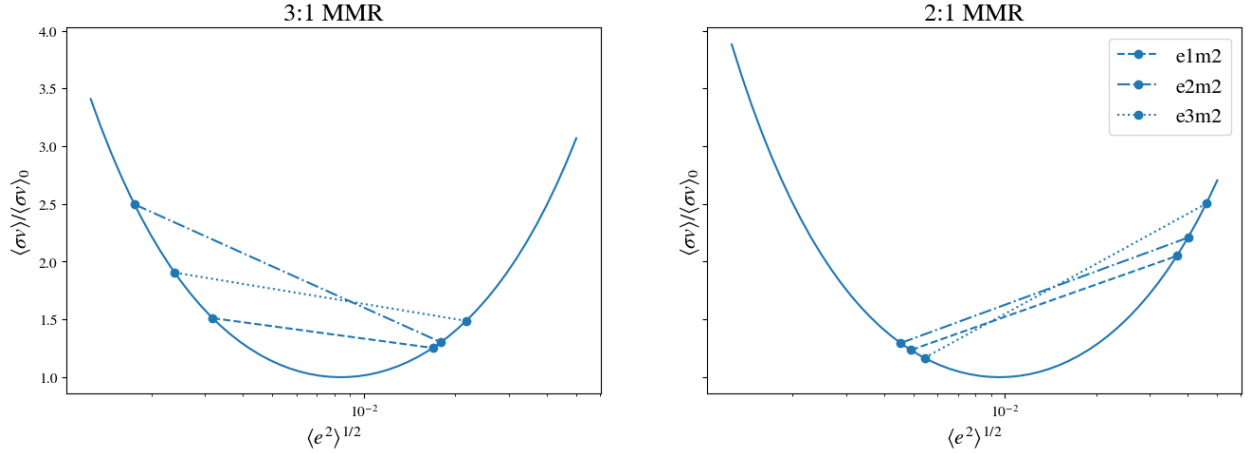
Figure 3.5: The collision rate (given by equation 3.6) of bodies in the vicinity of the 3:1 (left) and 2:1 (right) MMRs, relative to the minimum value, as a function of the local eccentricity dispersion. The pairs of points connected by lines show the values of the unperturbed (left-hand points in each subplot) and perturbed (right-hand points in each subplot) collision rates in the e1m2, e2m2 and e3m2 simulations. The unperturbed collision rate, along with the amount of dynamical heating that the planetesimal population experiences determines whether the MMR acts to suppress or enhance the collision rate
