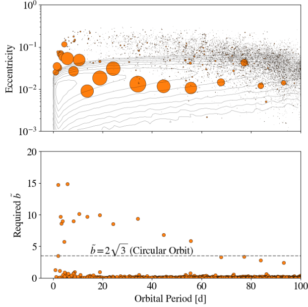
Figure 4.6: The final state of the fdHi simulation. In the top panel, the contours denote the initial period-eccentricity distribution of the planetesimals. Point sizes indicate the relative masses of bodies at the end of the simulation. In the bottom panel, we show the feeding zone width (see equation 5.2) required to produce the final masses of the bodies. The dashed line indicates the feeding zone size expected for bodies on circular orbits. For the shorter period bodies, the feeding zone size exceeds this expected value, which indicates that oligarchic growth is not operating here. This boundary occurs near roughly 60 d in orbital period.
