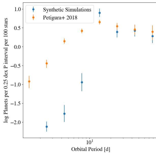
Figure 5.15: Occurrence rates of planets as a function of orbital period in 0.25 dex logarithmic bins. The de-biased occurrence rate measured from our synthetic simulations is shown in blue and the occurrence rate measured from planet candidates in the California Kepler Survey [222] is shown in orange.
