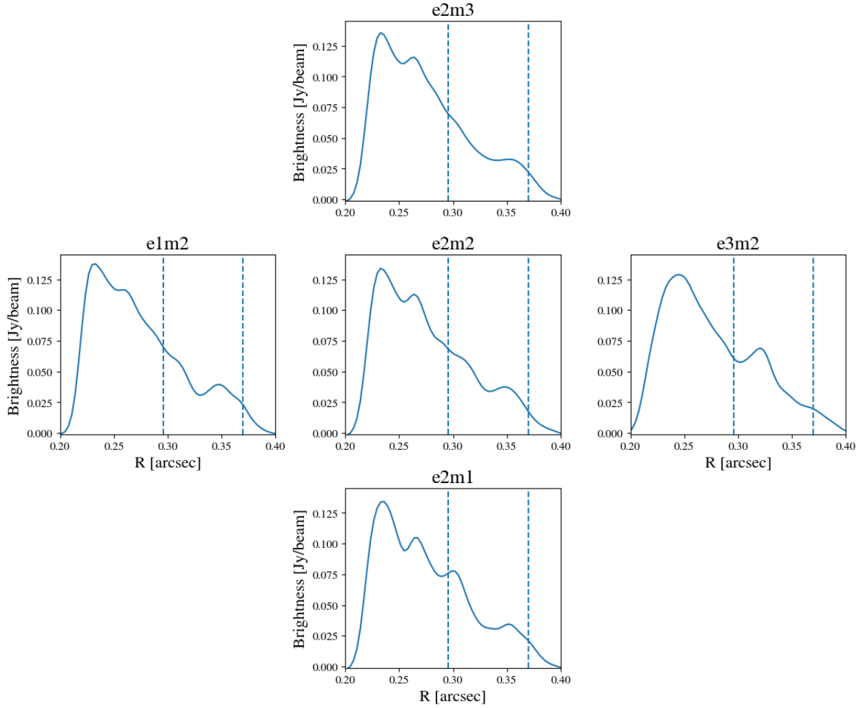
Figure 3.10: The azimuthally-averaged radial profile based on the simulated cleaned images from all five simulations. The eccentricity of the perturbing planet increases from left to right, while the mass of the planet increases from bottom to top. The vertical dashed lines indicate the locations of the 3:1 and 2:1 resonances. As in Figure 3.9, the size scale of the disc has been expanded by a factor of 10 and then placed at a distance of 100 pc.
