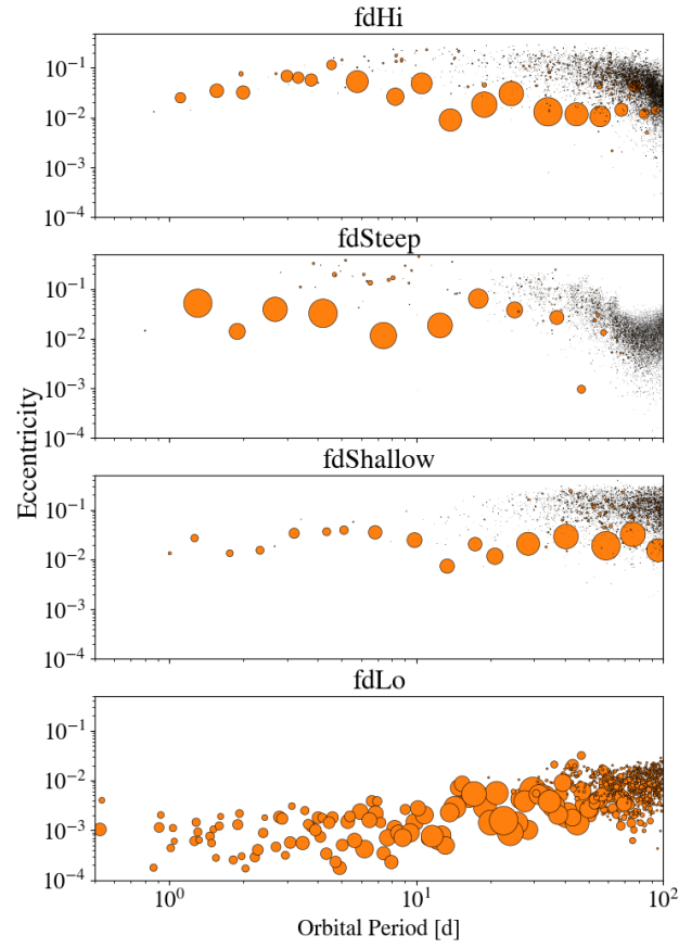
Figure 4.8: The final state of the full disk simulations listed in table 4.1. Point sizes indicate mass relative to the largest body in each simulation.
