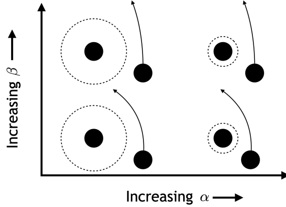
Figure 4.2: A diagram detailing how varying the values of \alpha and \beta affect the geometry of a two-body encounter. The solid circles represent the physical radius of a body and the dashed circles represent the Hill radius. As \alpha is increased, the Hill radius and the physical radius become comparable in size. As \beta is increased, the trajectory of a passing body for a fixed impact parameter is bent less and less.
