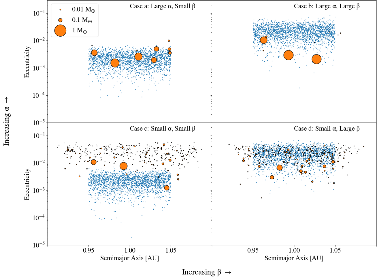
Figure 4.3: The initial (blue) and final (orange) states of the narrow annulus simulations described in section 4.4. Relative masses of the bodies are indicated by point size. In the case of large \alpha , almost no residual planetesimal population remains. Regardless of the initial choice of \beta , the protoplanets that form attain similar eccentricities.
