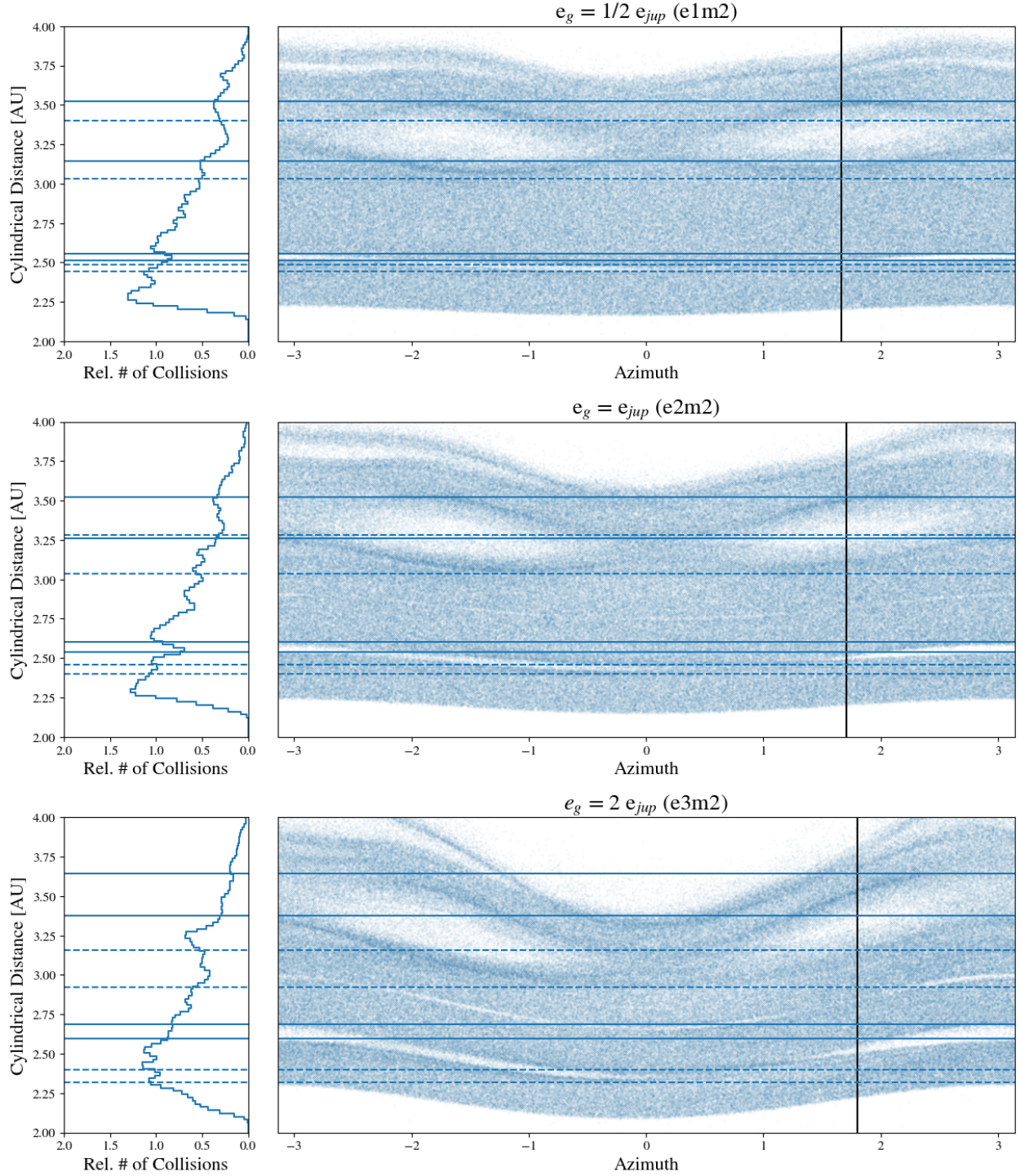
Figure 3.7: Collision profiles in Figure 3.6 are shown alongside the positions of the planetesimals, in polar coordinates. The dashed and solid lines show the pericenter and apocenter, respectively, of bodies at each edge of the 3:1 and 2:1 MMR. Here, the longitude of pericenter of the planet lies at \theta = 0 and the present position of the planet is indicated by the vertical line. For the 2:1 resonance, a bump, rather than a dip feature appears when the inner edge or the resonance's apocenter and outer edge's pericenter distance cross. The collision profile near the 3:1 resonance does not appear to follow this same qualitative behavior.
