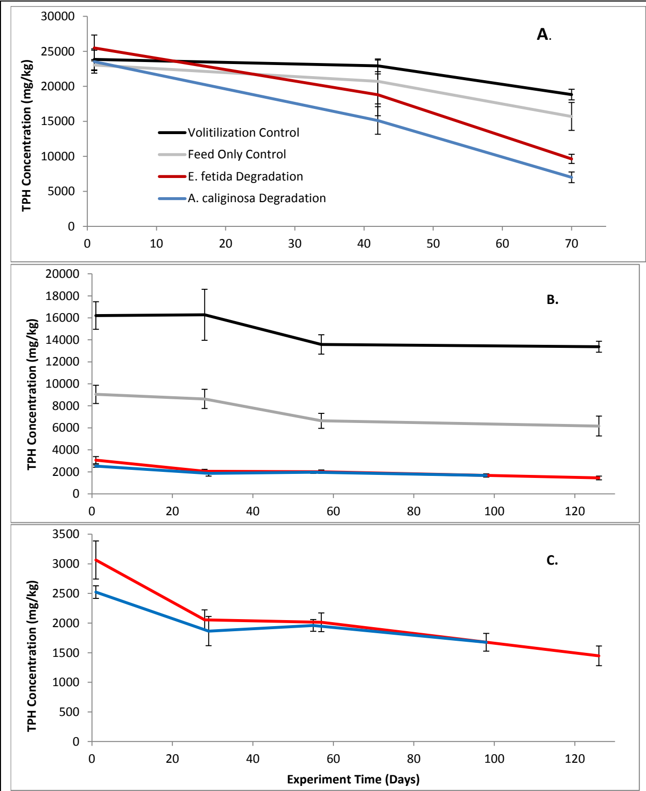
Figure 16: The influence of earthworms and feed on the native, contaminated soils. (A) Test 1a & 1b results: The initial TPH concentration was similar in all treatments (25,000 mg/kg) and concentrations of TPH were measured over time. (B) Test 2 results: The same treatments, with differing initial concentrations after the first experiment. (C) Detail of the Test 2 earthworm treatments. Concentrations of TPH were measured over time.
