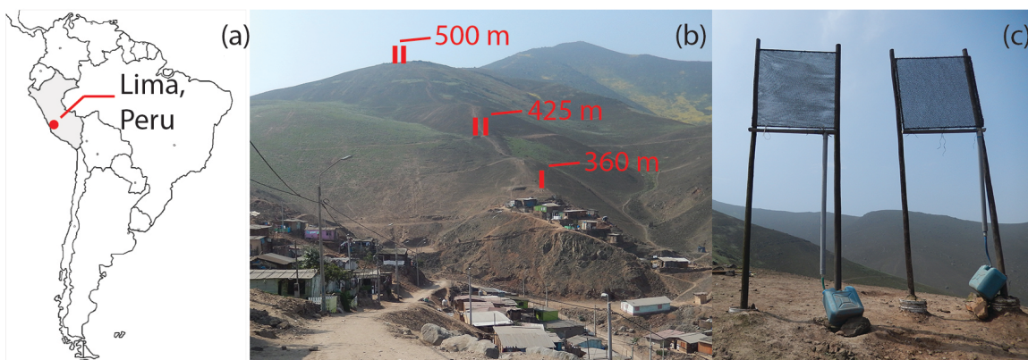
Fig. 2.3. Site Location. (a) Lima, Peru. (b) Nets are located above Eliseo Collazos, at 360 m, 425 m and 500 m. (c) Test SFC nets at the 425m site.
