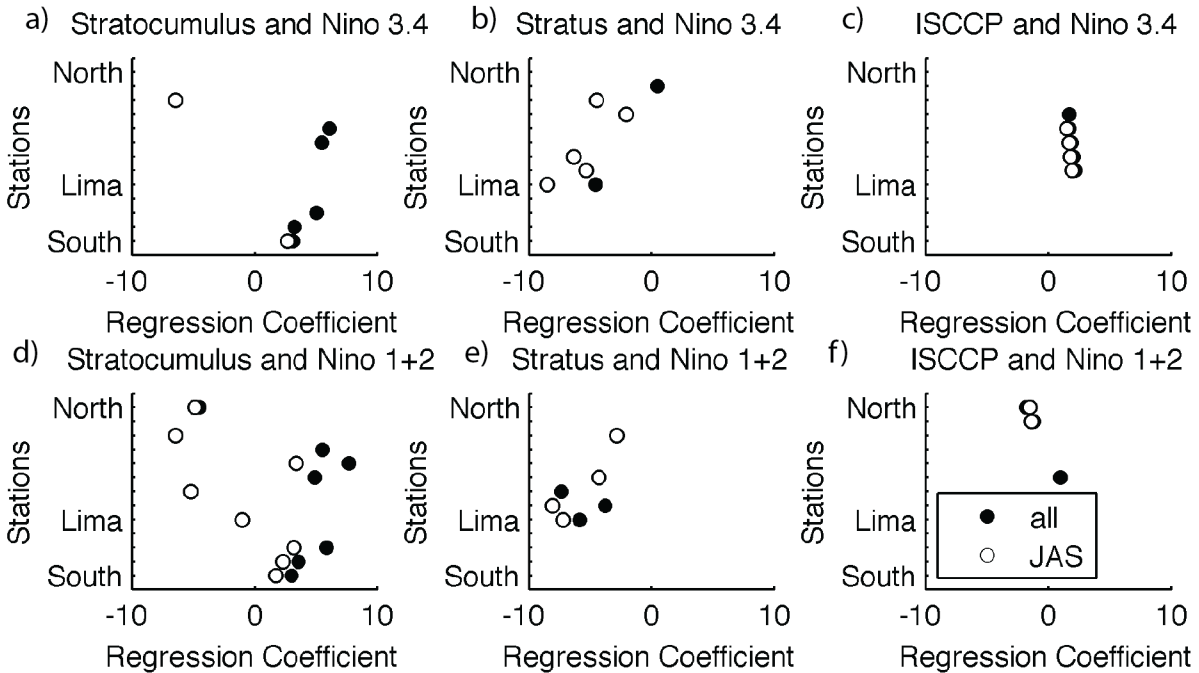
Figure 4.8. Regression coefficient ([% cloud cover ^{\circ}\text{C}^{-1} ]) for (a) stratocumulus cloud cover anomalies and Niño 3.4 anomalies, (b) stratus cloud cover anomalies and Niño 3.4 anomalies, (c) ISCCP cloud fraction anomalies and Niño 3.4 anomalies, (d) stratocumulus cloud cover anomalies and Niño 1+2 anomalies, (e) stratus cloud cover anomalies and Niño 1+2 anomalies, and (f) ISCCP cloud fraction anomalies and Niño 1+2 anomalies. Shown are regression coefficients from significant ( p < 0.05 ) correlations for all months, and JAS. Stations are shown from north to south. Correlation values are found in Appendix A [Figure A1].
