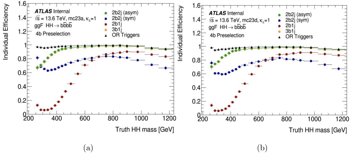
Figure 9.1: Individual trigger efficiencies for non-resonant HH \rightarrow b\bar{b}b\bar{b} production in the (a) mc23a and (b) mc23d simulated samples, shown after applying a 4b preselection. The preselection requires four jets with p_T > 25 GeV, |\eta_{\text{jet}}| < 2.5 , and GN2 b -tagging at the 77% working point [158].
