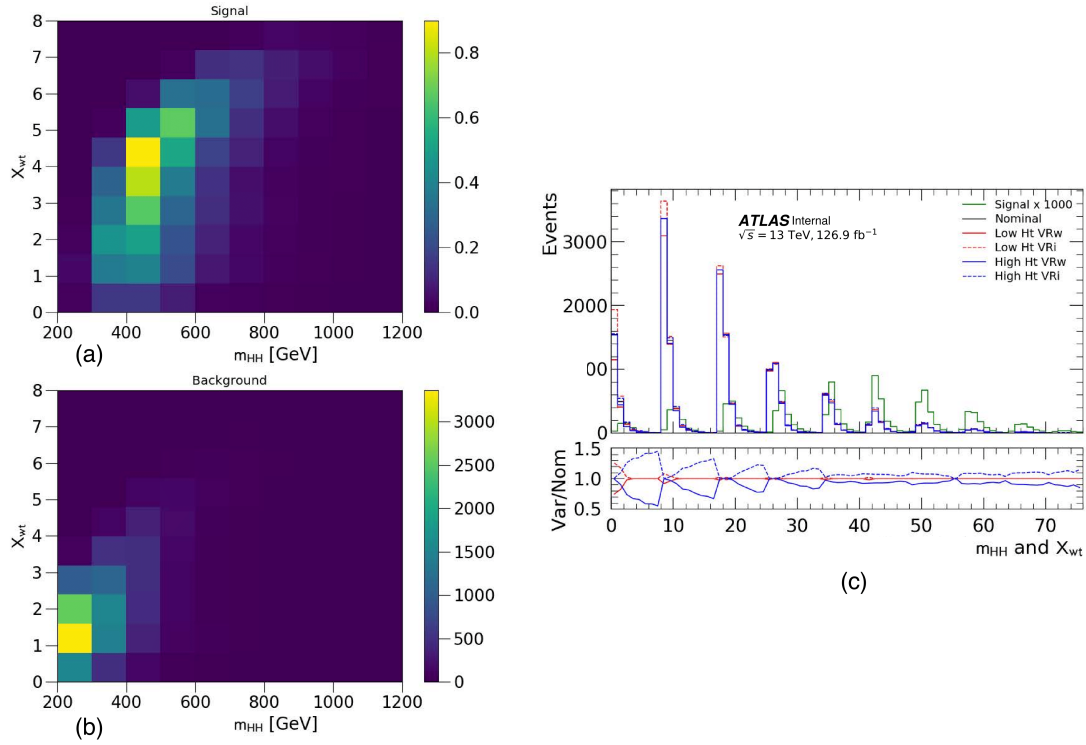
Figure 8.7: The m_{HH} vs X_{Wt} distributions for (a) signal and (b) average estimated background in the SR illustrating the correlations between m_{HH} and X_{Wt} . The transformation into a 1D histogram for fitting purposes (c), shown for these distributions, where the 2D histogram is "rolled out" starting from the bottom-left hand corner to the top-right corner.
