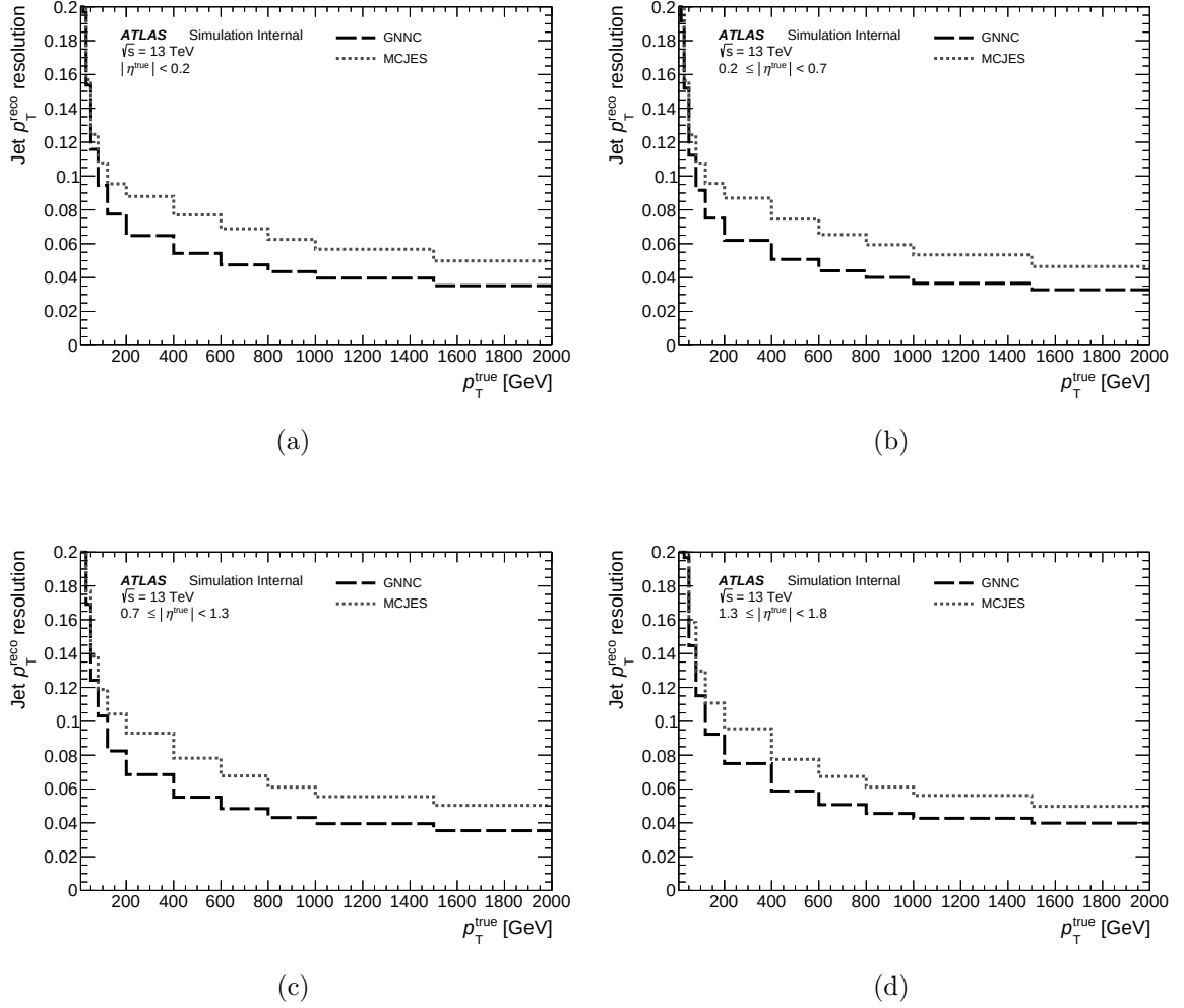
Figure 4.9: The jet p_T resolution for AF3 small- R UFO jets with the application of the global neural network calibration (GNNC) after the previous MC-JES calibration for the Pythia dijets in MC20 as shown for the \eta ranges of 0.0-0.2 in 4.9a, 0.2-0.7 in 4.9b, 0.7-1.3 in 4.9c, and 1.3-1.8 in 4.9d. All areas of the phase space see great improvement in p_T response and resolution.
