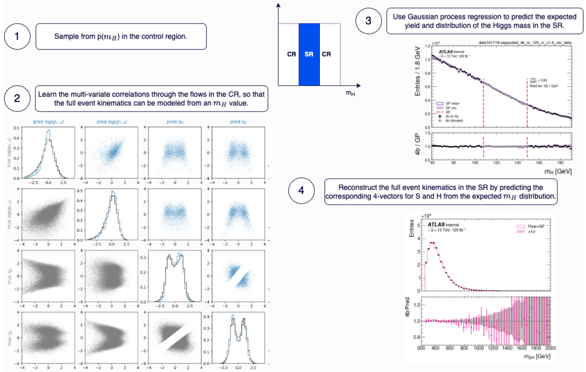
Figure 6.7: A general illustration of the data-driven background estimation method employed in the X \rightarrow SH \rightarrow b\bar{b}b\bar{b} analysis. Further technical details of the method and the results will follow in the subsequent chapters.
