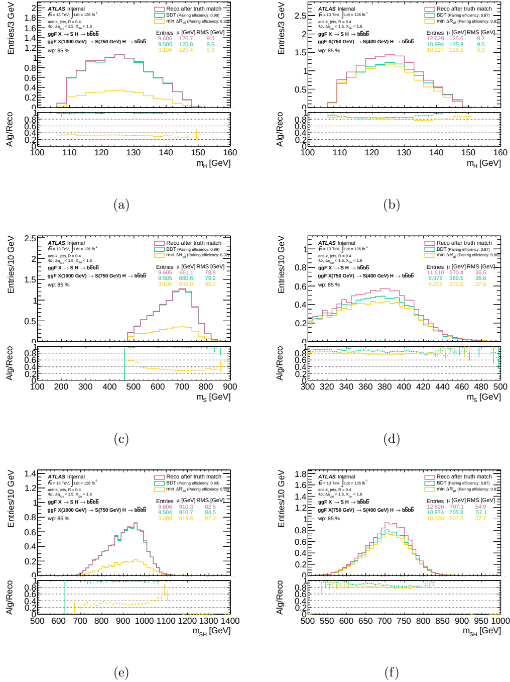
Figure 2.3: Reconstructed mass distributions for H ((a), (b)), S ((c), (d)), and X ((e), (f)) for a compressed signal ( m_X = 1000 GeV, m_S = 750 GeV; left column) and a non-compressed signal ( m_X = 750 GeV, m_S = 400 GeV; right column). Results are shown for BDT pairing (green), min \Delta R pairing (yellow), and truth-matching (pink). See SH4b Internal Note [145].
