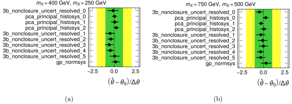
Figure 7.30: The major background systematic nuisance parameter pulls for (a) (m_X, m_S) = (400 \text{ GeV}, 250 \text{ GeV}) and (b) (m_X, m_S) = (750 \text{ GeV}, 500 \text{ GeV}) . These systematics nuisance parameters include the dominant shape systematics, the 3b non-closure uncertainty, and the normalization uncertainty from the GP regression.
