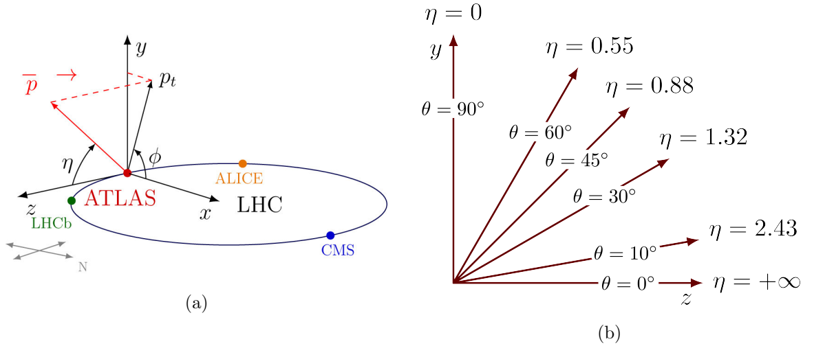
Figure 3.5: The typical coordinate system used in analyzing collisions at the LHC in 3.5a based on the four-vector of (p_T, \eta, \phi, m) . The pseudorapidity, \eta , is related to the polar angle in 3.5b.
