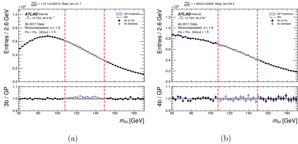
Figure 7.26: GP fits to the m_H distribution in the blinded pseudo-signal region for: (a) 3b , |\Delta\eta_{SH}| < 1.5 and (b) 4b , |\Delta\eta_{SH}| > 1.5 events, both in the non-compressed region ( m_H < m_S ) for 2017 data. Non-closure observed in the 3b region is used to define the associated systematic uncertainty.
