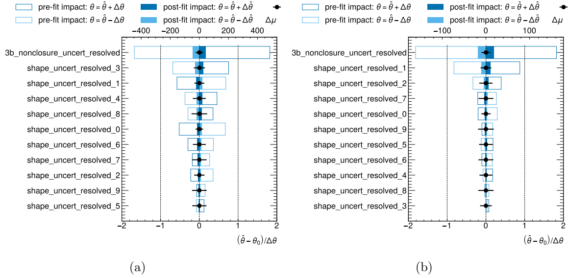
Figure 7.31: The dominant pulls and impacts of the background systematic uncertainties, including the nominal shape systematic uncertainties with the 3b non-closure uncertainties, ranked by magnitude of post-fit impact and shown for (a) (m_X, m_S) = (400 \text{ GeV}, 250 \text{ GeV}) and (b) (m_X, m_S) = (750 \text{ GeV}, 500 \text{ GeV}) . See the SH4b Internal Note [145].
