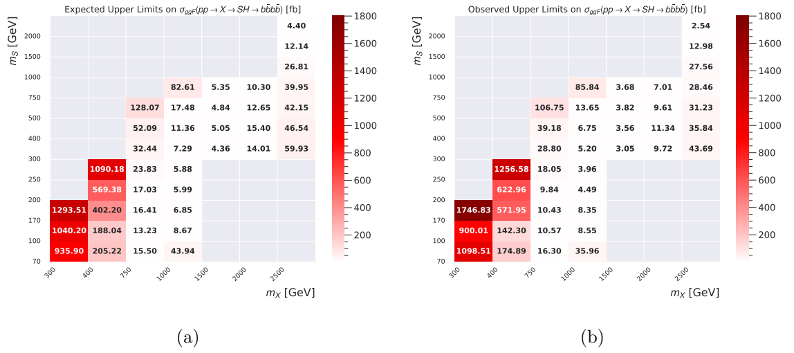
Figure 7.32: Expected (a) and observed (b) 95% CL upper limits on the cross section times the branching ratio for X \rightarrow SH \rightarrow b\bar{b}b\bar{b} for the resolved signal mass pairs including all background systematic uncertainties.
