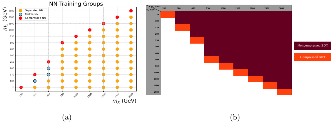
Figure 7.6: Assignment of signal mass points to the training groups of the NN (a) and the BDT (b). The compressed group consists of signal points where the mass difference between X and S + H is small, resulting in S and H being produced nearly at rest. The non-compressed group in the BDT and the separated group in the NN contain signal points where both scalars are significantly boosted. The NN includes an additional group, referred to as the middle group, representing mass points whose kinematics are intermediate between the compressed and separated groups.
