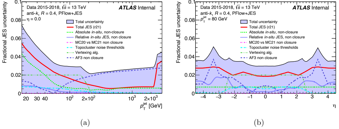
Figure 4.12: AF3 JES non-closure uncertainties for PFlow jets in the central region ( 0.0 < |\eta| < 0.2 ). (a) JES uncertainties dominate for high- p_T jets above 200 GeV. (b) For jets with 80 < p_T < 100 GeV, the uncertainties are particularly large in the forward region, highlighting AF3’s degraded performance near subdetector boundaries, as discussed in Section 4.2.
