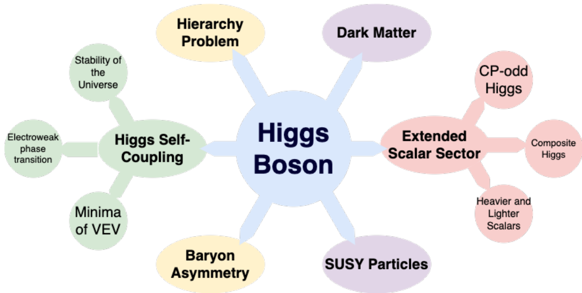
Figure 10.1: The central role of the Higgs boson in modern particle physics. The Higgs field not only gives mass to elementary particles via electroweak symmetry breaking but also connects to a broad array of theoretical and experimental frontiers, including Higgs self-coupling, dark matter, baryon asymmetry, supersymmetric particles, the stability of the vacuum, composite Higgs models, and extensions to the scalar sector. Each branch highlights a key area where the Higgs boson could provide insight into physics beyond the Standard Model.
