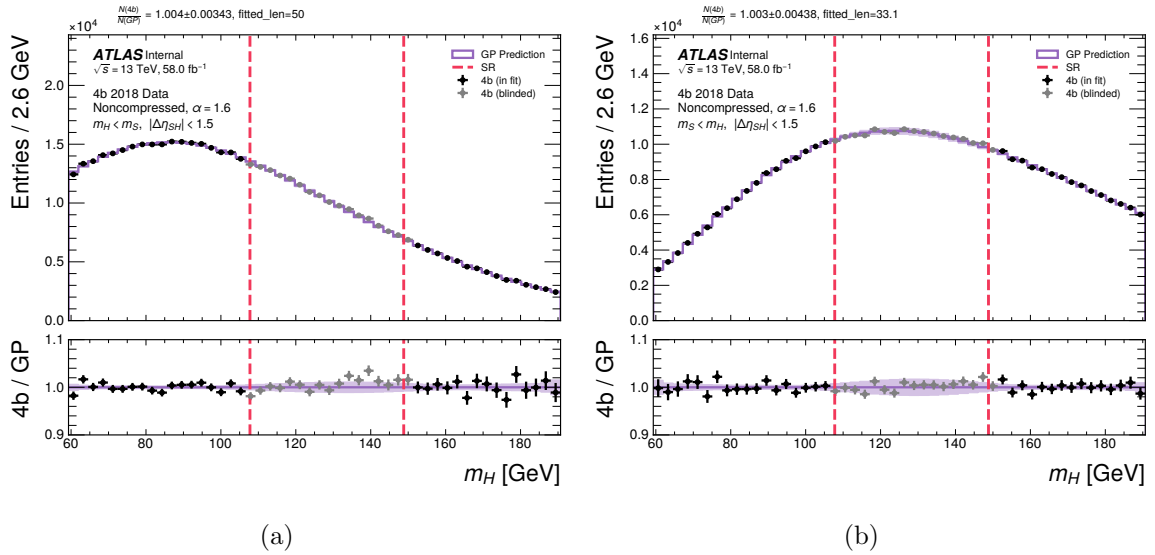
Figure 7.20: Gaussian process regression for the Higgs candidate mass ( m_H ) distribution in the (a) non-compressed minH and (b) non-compressed minS selection for the nominal 4b data in 2018. Points show data in the CR and SR, while the shaded band show the GP prediction and its uncertainty.
