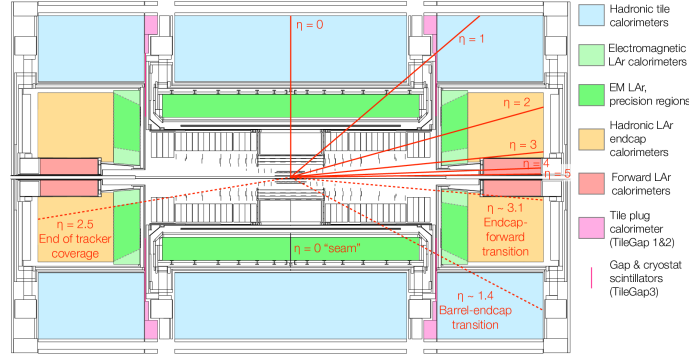
Figure 4.5: A two-dimensional slice of the ATLAS detector showing the calorimeter geometries at specific pseudorapidities along the beam axis. The poor modeling of jet \eta in AF3 tends to occur near the calorimeter boundaries [84].
