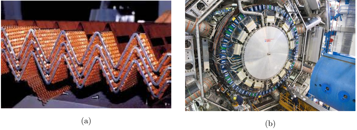
Figure 3.8: Illustrations of the two main calorimeter systems in the ATLAS detector. (a) View of the accordion-shaped structure of alternating absorber and readout layers of the Electromagnetic Calorimeter. (b) View of the Tile Hadronic Calorimeter, which consists of alternating layers of steel and plastic scintillator tiles. This system is optimized for measuring the energy of hadrons and forms the largest and most massive component of the calorimeter system.
