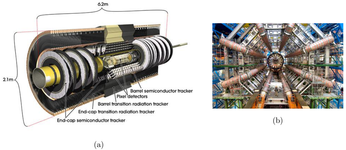
Figure 3.7: Overview of ATLAS tracking and magnet systems. (a) The Inner Detector (ID), composed of the Pixel Detector, Semiconductor Tracker (SCT), and Transition Radiation Tracker (TRT), provides high-precision tracking of charged particles. (b) The eight superconducting coils of the Barrel Toroid magnet, part of the ATLAS toroidal system, generate a magnetic field used primarily to bend muon trajectories in the outer detector region. Together with the Central Solenoid, these systems are essential for tracking and identifying particles across a wide momentum range.
