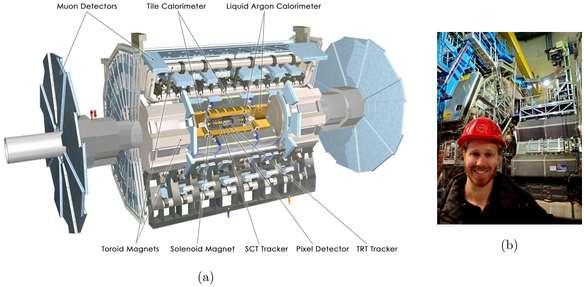
Figure 3.6: A layout of the ATLAS subdetector systems in 3.6a with two people shown left for size. In 3.6b is myself standing in front of the ATLAS Detector during one of the winter shutdowns when cavern visits are allowed.
