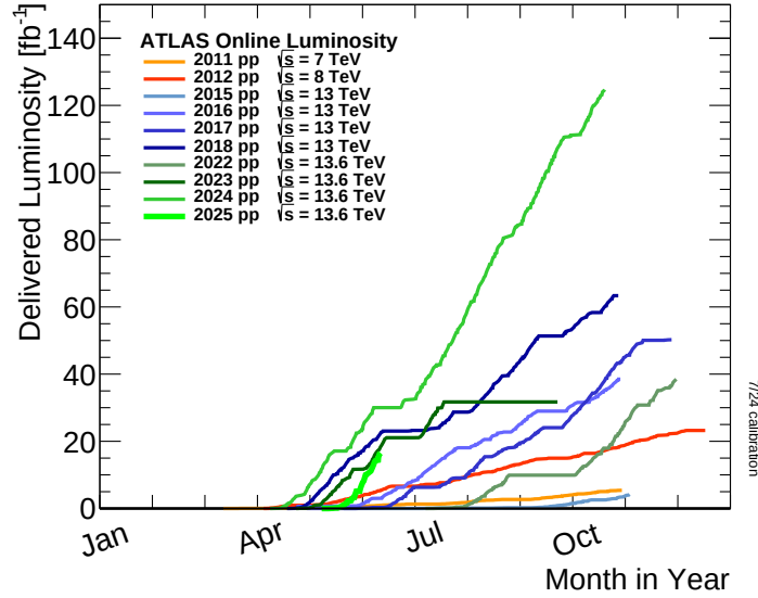
Figure 3.4: Cumulative luminosity versus day delivered to ATLAS during stable beams and for high energy pp collisions for each data-taking year. Note that data-taking for 2025 is ongoing [51].
