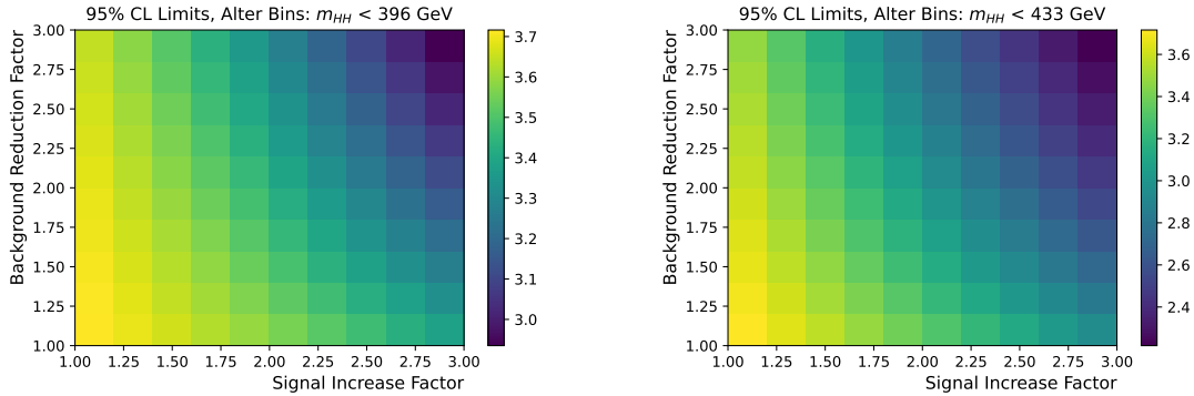
Figure 1.5: Stat-only 95% CL limits when both increasing the signal and reducing the background by factors between 1 and 3 for low-mass events, with boundaries at (a) m_{HH} < 396 GeV and (b) m_{HH} < 433 GeV.
