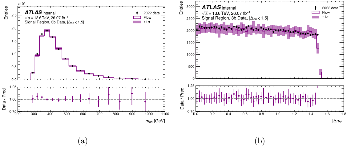
Figure 9.11: The distribution of the data and the background prediction for (a) m_{HH} and (b) |\Delta\eta_{HH}| for the 3b validation region with |\Delta\eta_{HH}| < 1.5 in 2022 in the SR. The modeling is generally well within the uncertainty of the standard deviation of the 25 predictions outside of the kinematic boundary.
