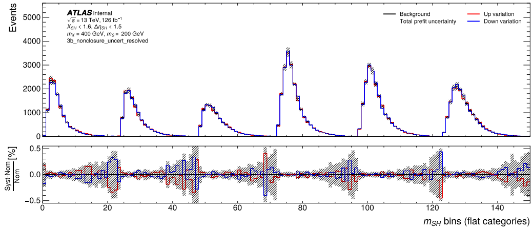
Figure 7.24: The 3b non-closure uncertainty as a function of m_{SH} , derived for the non-compressed BDT pairing when m_X = 400 GeV, m_S = 200 GeV. The up and down variations from the non-closure is shown in red and blue respectively. See the SH4b Internal Note [145].
