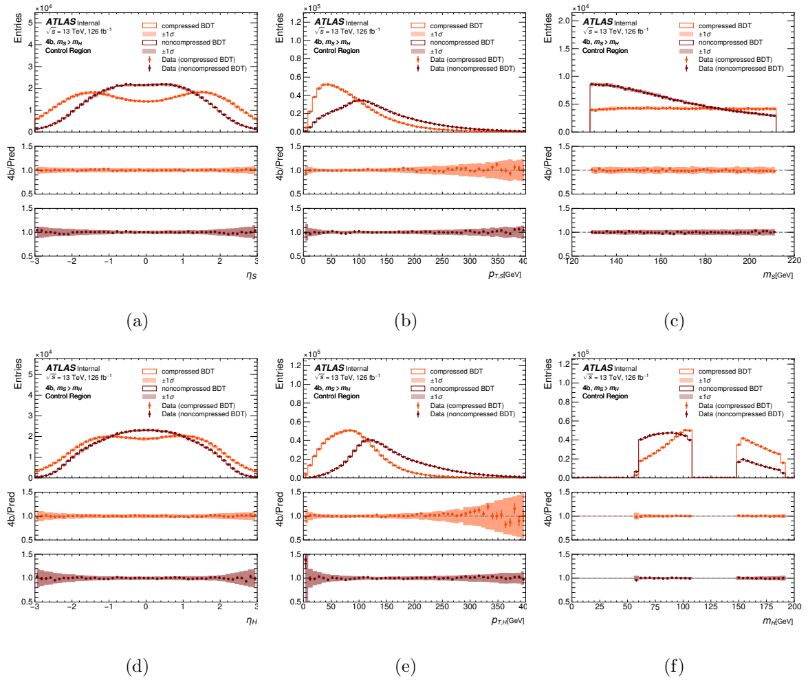
Figure 7.18: Distributions of kinematic variables of the S and Higgs candidate bosons for the predictions from the normalizing flows in the Control Region for the compressed and non-compressed BDT pairings when m_S > m_H .
