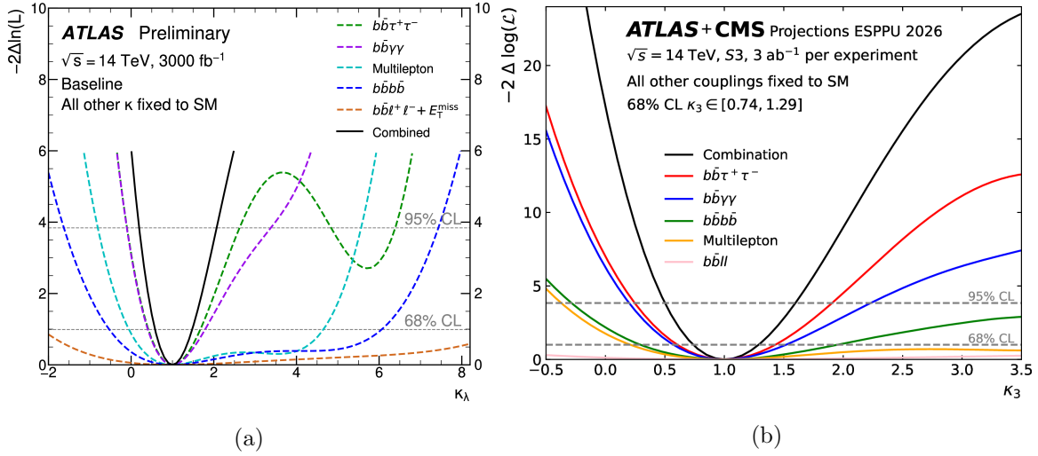
Figure 10.2: Expected values of the negative log-likelihood ratio as a function of \kappa_\lambda for an integrated luminosity of 3000 fb -1 at \sqrt{s} = 14 TeV for the ATLAS (ATLAS+CMS) combination of different channels and their statistical combination in the baseline scenario in Figure 10.2a (10.2b) [160, 161].
