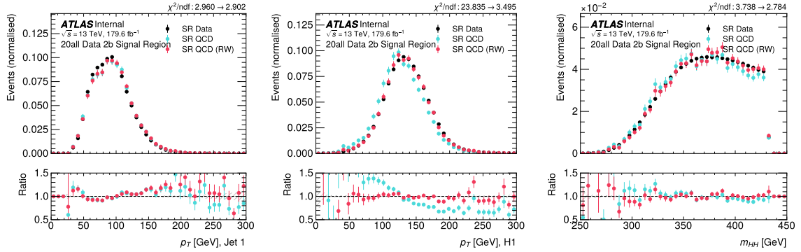
Figure 1.6: Distributions of (a) the p_T of the leading Higgs candidate jet 1, (b) the p_T of the leading Higgs candidate, and (c) m_{HH} for low-mass 2b events from simulated multi-jet QCD, after NN reweighting to match Run 2 and partial Run 3 data in the SR. Good closure is observed across the kinematic phase space.
