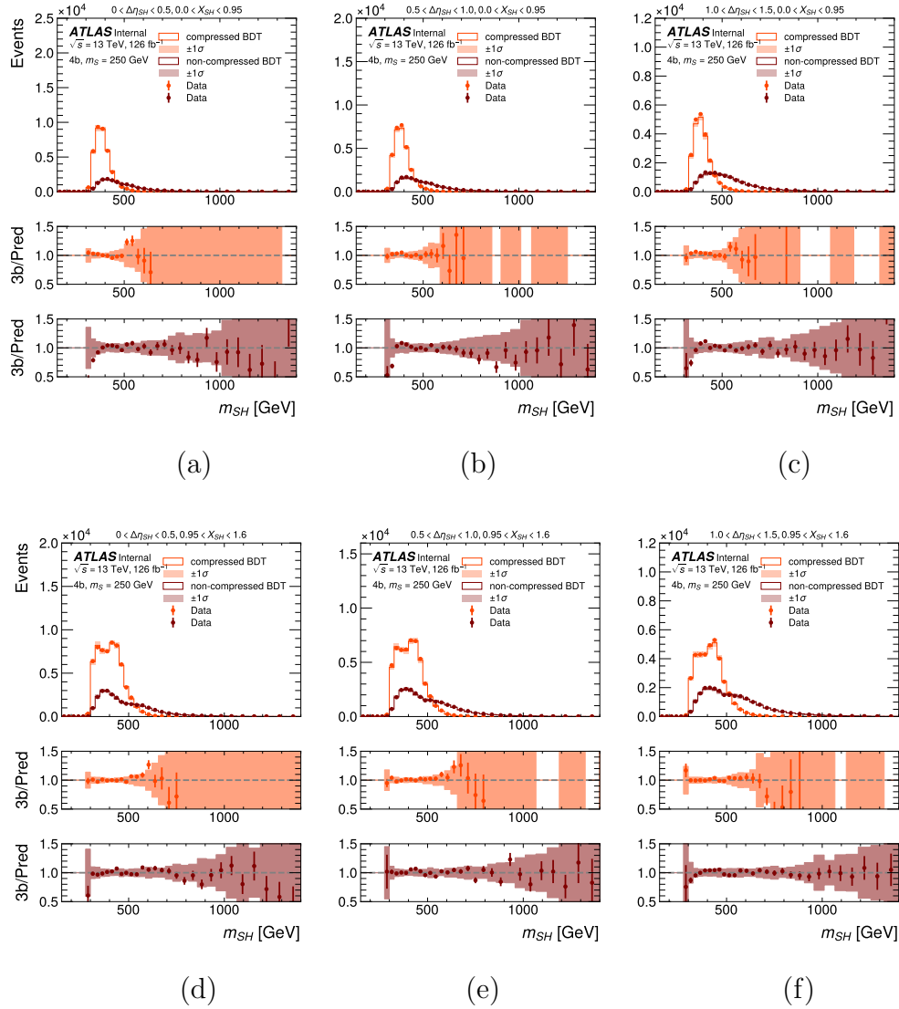
Figure 7.29: The categorized m_{SH} distribution in the unblinded 4b signal region for m_S = 250 GeV. The six subplots correspond to: (a) Category 0: 0.0 < |\Delta\eta_{SH}| < 0.5 , 0.0 < X_{SH} < 0.95 , (b) Category 1: 0.5 < |\Delta\eta_{SH}| < 1.0 , 0.0 < X_{SH} < 0.95 , (c) Category 2: 1.0 < |\Delta\eta_{SH}| < 1.5 , 0.0 < X_{SH} < 0.95 , (d) Category 3: 0.0 < |\Delta\eta_{SH}| < 0.5 , 0.95 < X_{SH} < 1.6 , (e) Category 4: 0.5 < |\Delta\eta_{SH}| < 1.0 , 0.95 < X_{SH} < 1.6 , and (f) Category 5: 1.0 < |\Delta\eta_{SH}| < 1.5 , 0.95 < X_{SH} < 1.6 .
