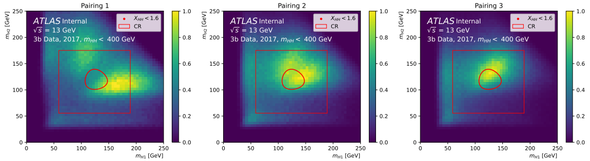
Figure 1.3: Distributions of 3b events with m_{HH} < 400 GeV from 2017 data in the m_{H1} - m_{H2} plane for each of the three possible jet pairings. With jets ordered by decreasing p_T and indices [1,2,3,4] : pairing 1 is [(1,2), (3,4)] , pairing 2 is [(1,3), (2,4)] , and pairing 3 is [(1,4), (2,3)] .
