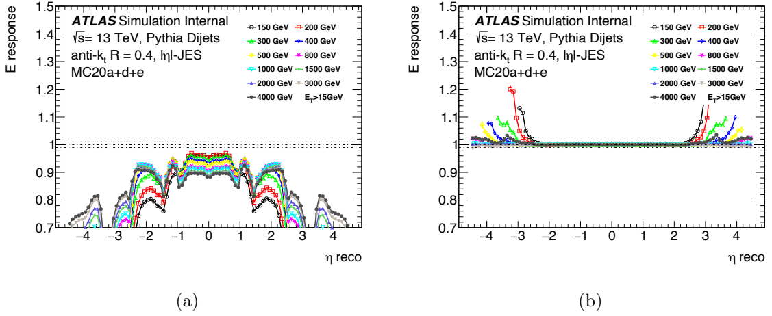
Figure 4.8: Jet energy response before and after applying the absolute JES calibration for small- R UFO jets in AF3 simulation. (a) Mean jet energy response, defined as E_{\text{reco}}/E_{\text{truth}} , as a function of jet energy and |\eta| prior to calibration, showing significant deviations from unity across the detector. (b) Response after applying the JES correction function C(E_{\text{reco}}) obtained from numerical inversion and polynomial fitting. Closure is achieved in the central region ( |\eta| < 2.5 ), indicating that the calibrated jet energies now accurately match the corresponding truth-level energies.
