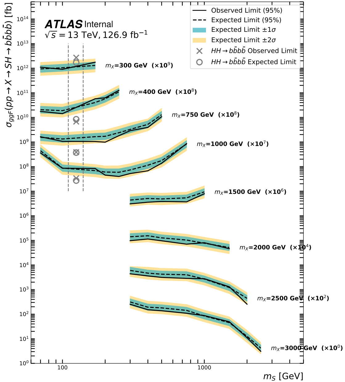
Figure 3.2: Observed (solid black line) and expected (dashed black line) 95% CL upper limits on the cross section times the branching ratio. For each unique m_X value, a scaling factor is applied to the limits so that all mass pairs can be visualized together. The inner green (outer yellow) bands represent the 1\sigma and 2\sigma uncertainties, respectively. The observed and expected limits on the cross section times the branching ratio for the resonant HH \rightarrow b\bar{b}b\bar{b} results are depicted (approximately) in gray.
