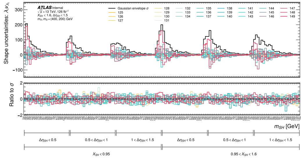
Figure 7.23: Leading principal component variations in the m_{SH} distribution from the deep ensemble for the non-compressed region ( m_X = 400 GeV, m_S = 200 GeV). The shaded envelope indicates the standard deviation across the 25 ensemble predictions in each bin. See the SH4b Internal Note [145].
