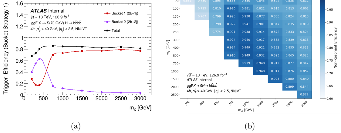
Figure 7.4: (a) Total trigger efficiency of Bucket Strategy 1 as a function of m_X for m_S = 70 GeV, showing the contribution from each individual bucket. Bucket 1 provides higher efficiency at large m_X values, while Bucket 2 is more efficient at lower m_X values. (b) Total efficiency of Bucket Strategy 1 for all signal mass pairs considered up to m_X = 3000 GeV. See the SH4b Internal Note [145].
