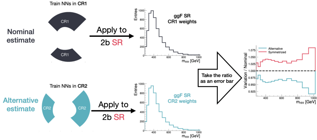
Figure 8.2: Illustration of the background shape systematic derivation. The top row shows the nominal estimate from CR1, while the bottom row shows the alternative estimate from CR2. The right plot displays the symmetrized shape variation (pink histogram), used to define the “CR12 shape systematic”. Variations are defined per |\Delta\eta_{HH}| and X_{HH} category as appropriate. Figure from [155].
