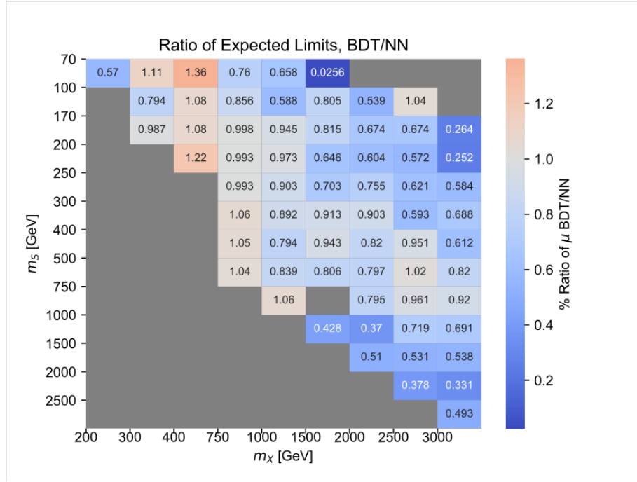
Figure 7.9: Ratio of statistical-only 95% confidence level upper limits for X \rightarrow SH \rightarrow b\bar{b}b\bar{b} between the NN and BDT pairing methods, evaluated using resolved signal samples. The NN pairing shows slightly better sensitivity for some low-mass points, while the BDT provides a substantial improvement at higher masses.
