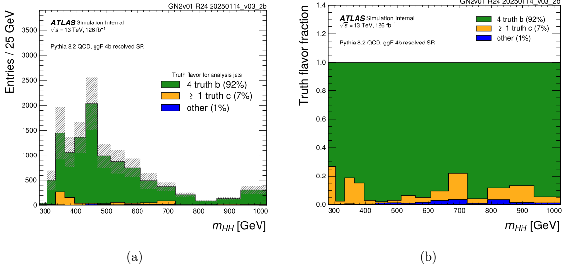
Figure 6.5: (a) Flavor composition of the QCD background in the 4b signal region of the HH \rightarrow b\bar{b}b\bar{b} analysis. (b) Bin-by-bin normalized version of (a), showing the fractional contribution of different jet flavors.
