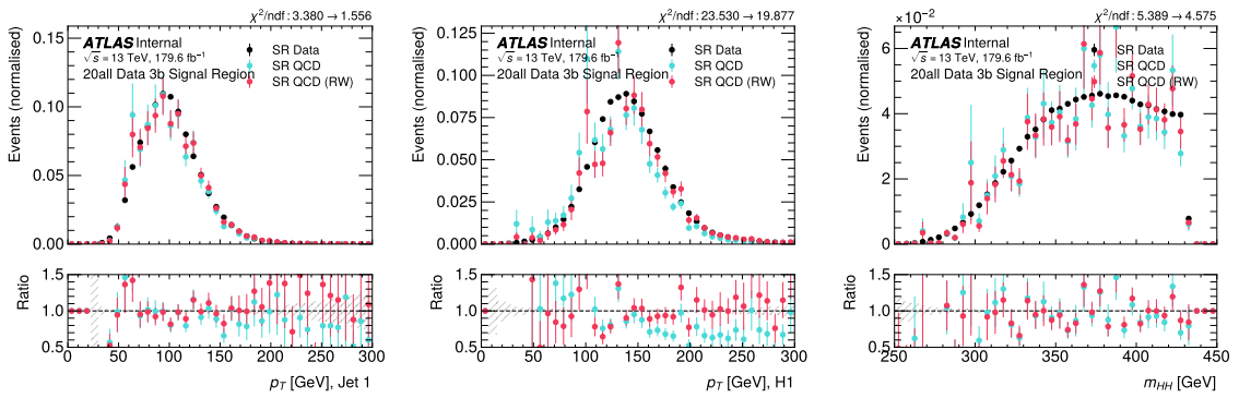
Figure 1.7: Distributions of (a) the p_T of the leading Higgs candidate jet 1, (b) the p_T of the leading Higgs candidate, and (c) m_{HH} for low-mass 3b events from simulated multi-jet QCD, after NN reweighting to match Run 2 and partial Run 3 data in the SR. While closure improves, significant modeling challenges remain.
