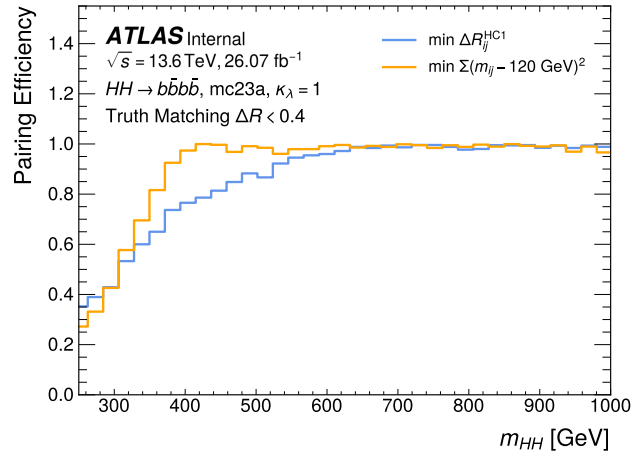
Figure 9.2: Pairing efficiency as a function of the reconstructed m_{HH} for the min \Delta R and min \chi^2 = \sum(m_{jj} - m_X)^2 pairing algorithms. The min \Delta R pairing method, which is the nominal pairing method, is poor at low masses, but very accurate for m_{HH} > 500 GeV.
