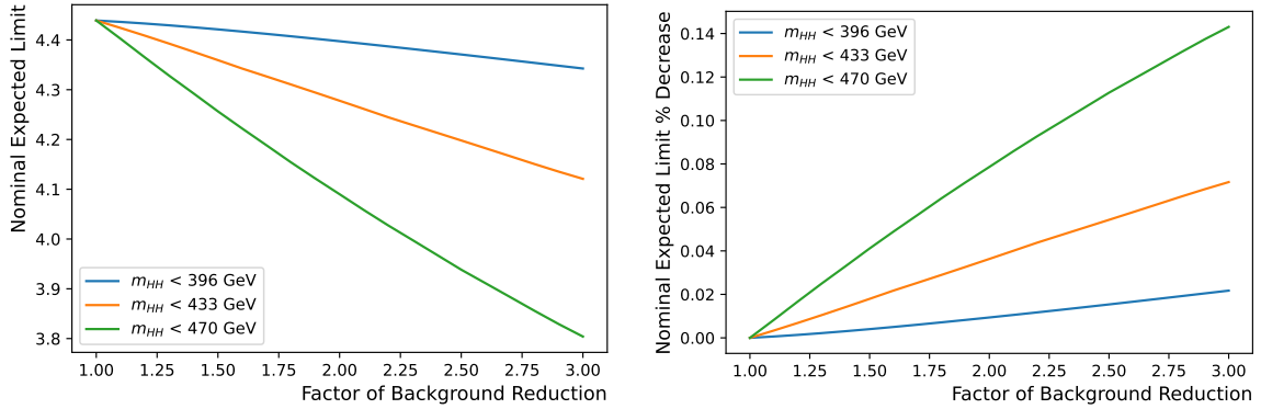
Figure 1.4: (a) Stat-only 95% CL limits and (b) their percentage improvement when reducing the low-mass background by a factor of up to three, for several boundaries of m_{HH} .
