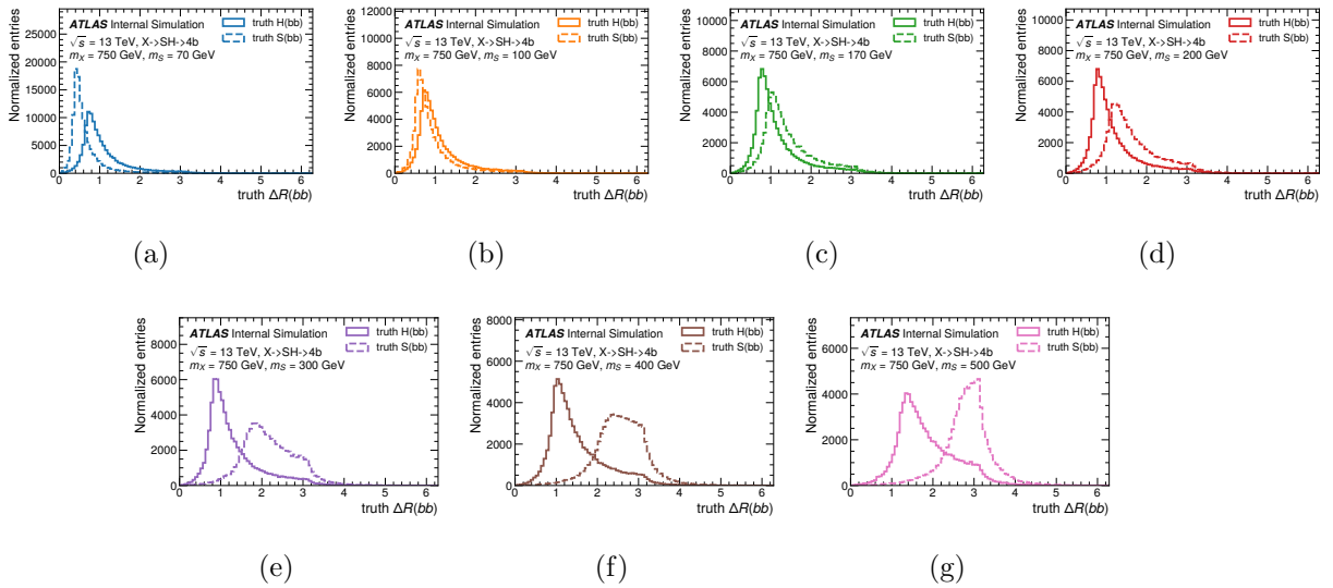
Figure 7.10: Distribution of \Delta R between the two b -quarks from the decays of the scalar S (dashed) and the SM Higgs boson (solid) for signal samples with m_X = 750 GeV and m_S as indicated in each panel. See the SH4b Internal Note [145].
