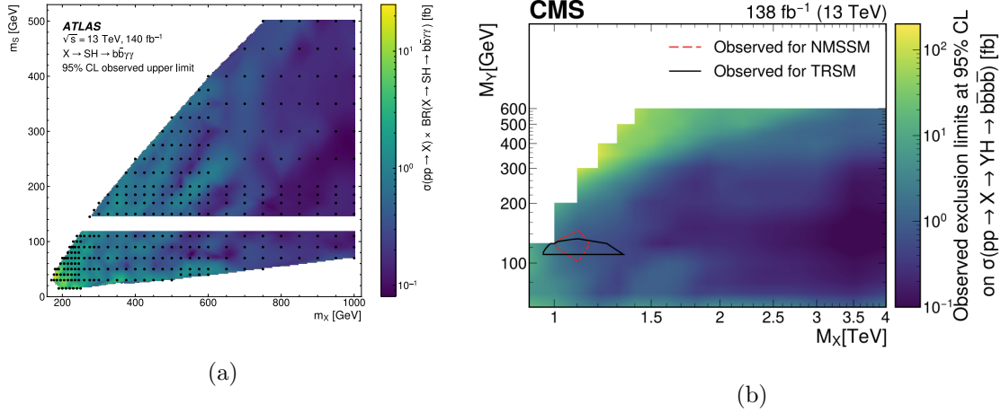
Figure 5.9: (a) Observed 95% CL upper limits on the signal cross section times branching fraction for the X \rightarrow SH \rightarrow b\bar{b}\gamma\gamma signal in the ATLAS Run 2 analysis, in the (m_X, m_S) plane with the points show where the limits were evaluated [132]. (b) Observed 95% CL upper limits on the signal cross section times branching fraction for the boosted X \rightarrow YH \rightarrow b\bar{b}b\bar{b} signal in the CMS Run 2 analysis, in the (m_X, m_S) plane with the boundaries of the excluded regions of the NMSSM and TRSM included [133].
