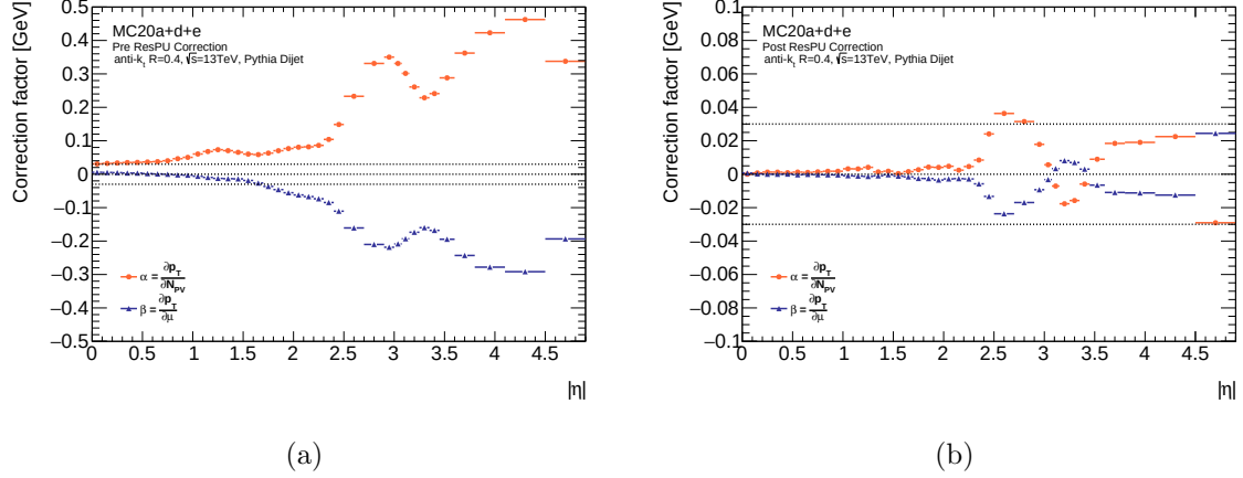
Figure 4.7: Residual pile-up correction factors for AF3-simulated jets as a function of |\eta| using Pythia dijet samples from the MC20 campaign. (a) Correction factors \alpha and \beta obtained from the first iteration, before applying any residual pile-up correction. (b) Correction factors recalculated after the initial correction is applied. Values below 0.03 across all |\eta| regions indicate that pile-up effects have been effectively mitigated.
