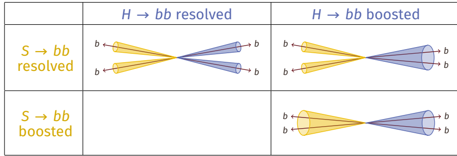
Figure 6.3: Illustration of possible topological configurations for the b\bar{b}b\bar{b} final state in the SH \rightarrow 4b analysis. In the resolved topology, all four b -quarks hadronize into separate, individually reconstructed small- R jets. In the intermediate topology, one b\bar{b} pair is sufficiently boosted that both quarks are reconstructed within a single large- R jet. In the boosted topology, both b\bar{b} pairs are sufficiently boosted that they are reconstructed within two separate large- R jets.
