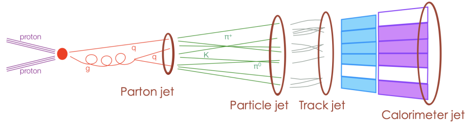
Figure 4.1: The different stages of jet development going from the pp collision to the produced partons to stable particle jets to track jets and then the final calorimeter jets. Figure taken from [73].
