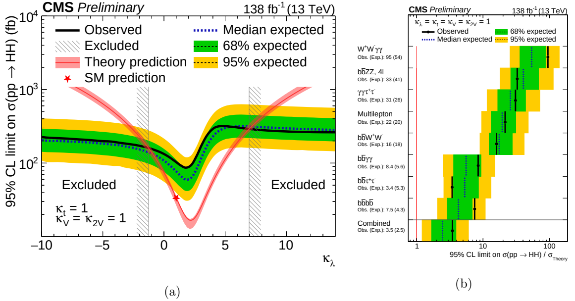
Figure 5.7: (a) The 95% CL upper limits on the inclusive HH cross section as a function of \kappa_\lambda when all other couplings are set to values predicted by the SM. The inner (green) band and the outer (yellow) band indicate the 68% and 95% CL intervals [129].
