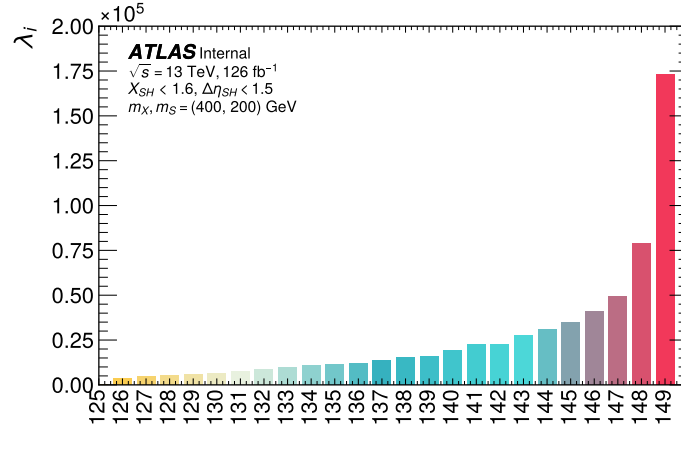
Figure 7.22: Eigenvalues from the principal component analysis of the ensemble background prediction for the non-compressed signal region ( m_X = 400 \text{ GeV} , m_S = 200 \text{ GeV} , 2016–2018 data). The largest eigenvalues correspond to the retained shape systematics. See the SH4b Internal Note [145] .
