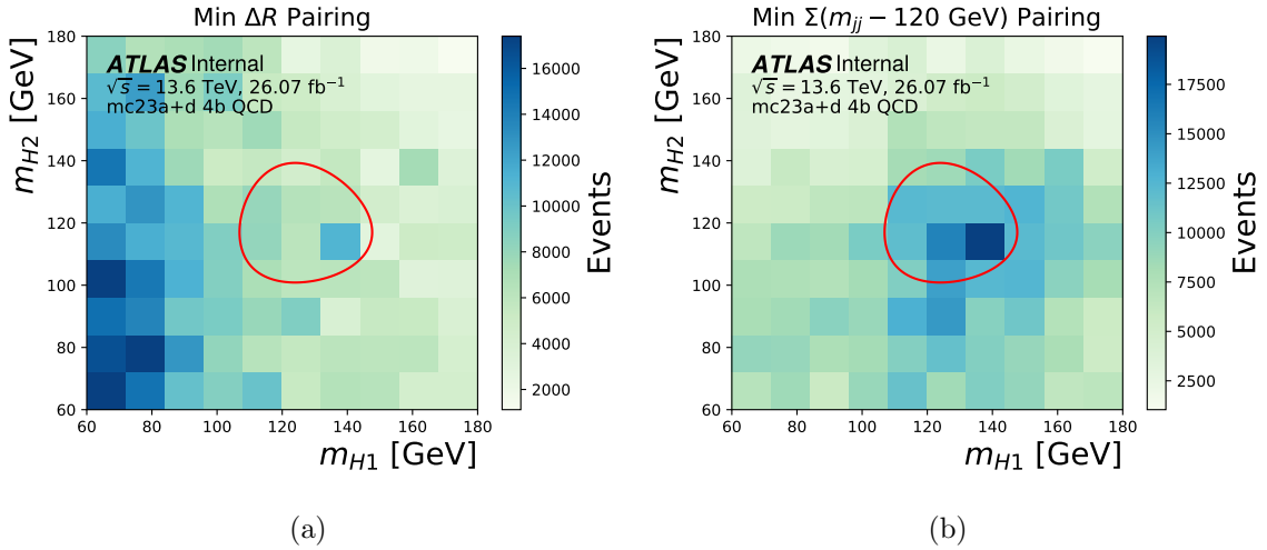
Figure 9.3: Distributions of simulated 4b QCD events for mc23a+d in the m_{H1} - m_{H2} mass plane for the (a) min \Delta R pairing and the (b) mass-based pairing. The min \Delta R approach leads to much less background in the signal region (red contour).
