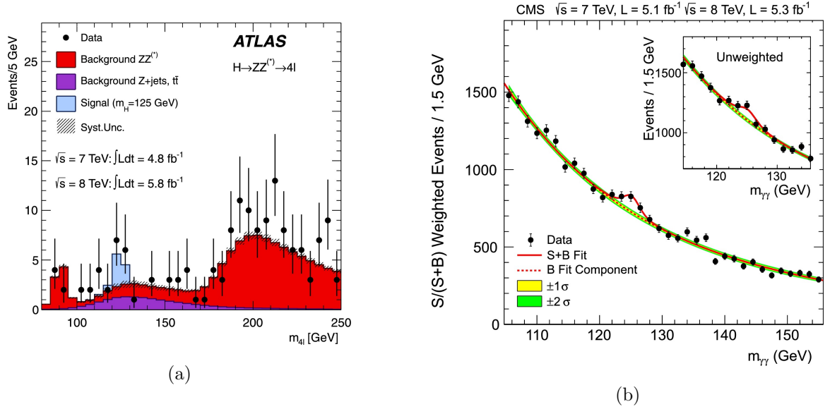
Figure 2.2: Distributions used in the Higgs boson discovery: (a) the four-lepton invariant mass m_{4\ell} from the ATLAS analysis of H \rightarrow ZZ^* \rightarrow 4\ell , showing data compared to the background expectation and the signal prediction for a 125 GeV Higgs, combining \sqrt{s} = 7 TeV and 8 TeV data; (b) the diphoton invariant mass distribution from the CMS analysis of H \rightarrow \gamma\gamma , with events weighted by S/(S+B) to enhance signal sensitivity [40, 41].
