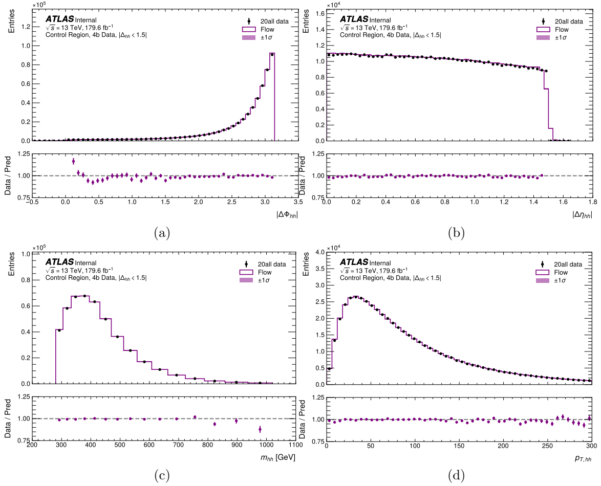
Figure 9.7: Distributions of 4b data and normalizing flow predictions for all data-taking years (2016–2018, 2022–2023) in the control region: (a) |\Delta\phi_{HH}| , (b) |\Delta\eta_{HH}| , (c) m_{HH} , and (d) p_{T,HH} . There is overall great closure between data and prediction outside of the boundary of the |\Delta\eta_{HH}| cut.
