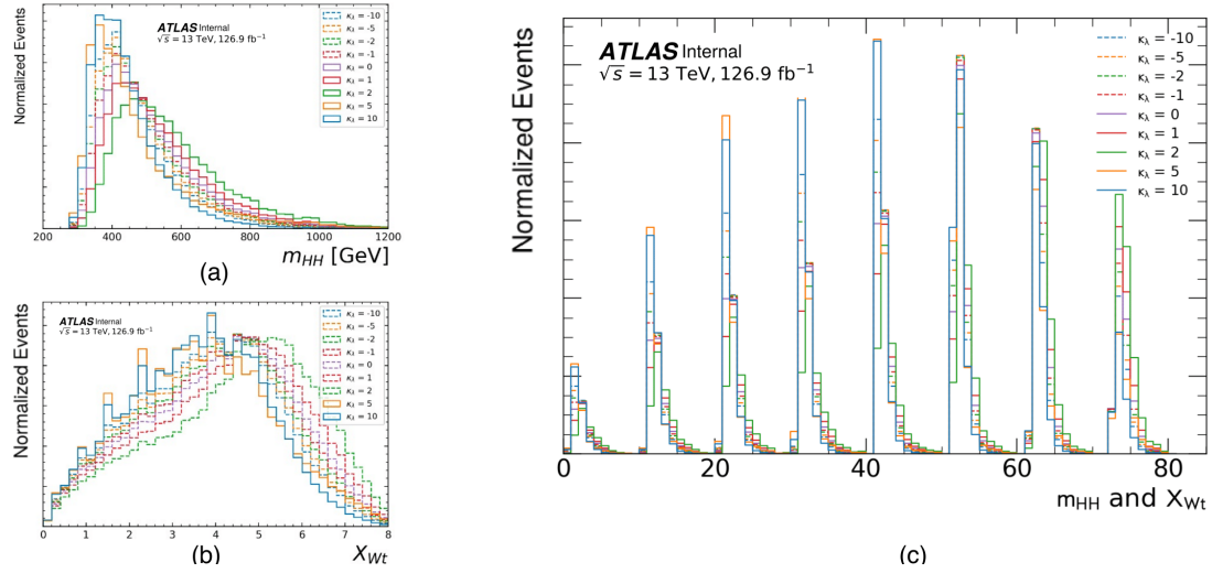
Figure 8.8: Normalized distributions of (a) m_{HH} and (b) X_{Wt} for several representative \kappa_\lambda values, and their transformation into a (c) 2D discriminant employed in the statistical fit. The use of a 2D discriminant consistently improves the statistical-only 95% CL limits on \kappa_\lambda . The effect of varying \kappa_\lambda on the distribution shapes is clearly observed.
