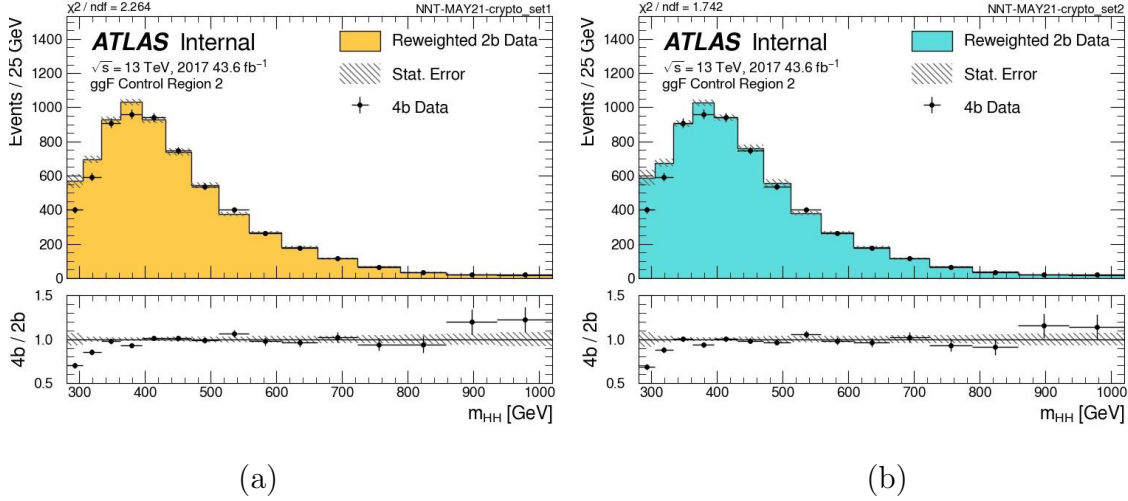
Figure 8.4: Distributions of the reweighted 2b events and 4b data for m_{HH} in Control Region 2 for 2017 data, shown for configurations 1 (with Poisson sampling) and 2 (without Poisson sampling). No significant difference is observed in the average prediction of the resulting distributions.
