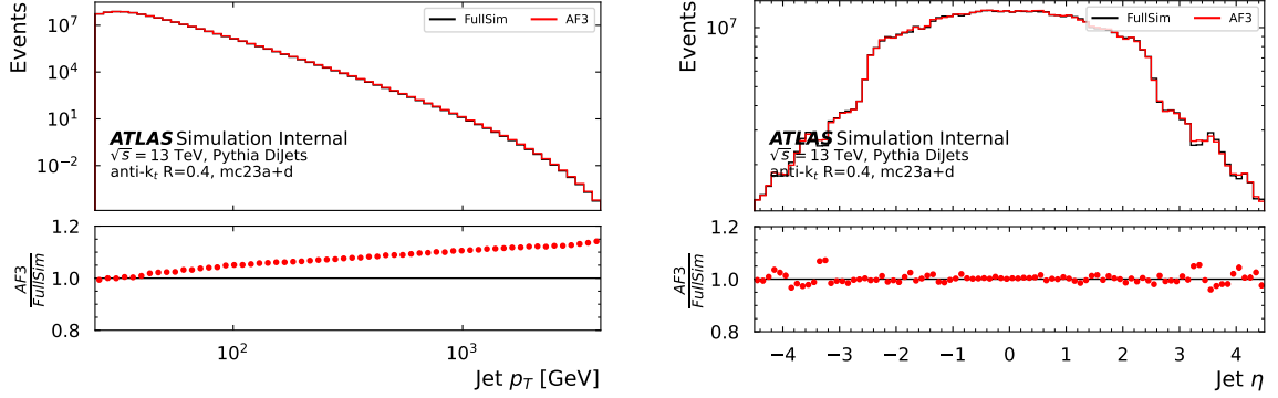
(a) Reconstructed jet p_T distribution.
