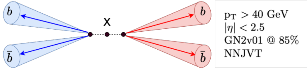
Figure 7.5: Schematic representation of the event selection criteria in the resolved channel of the SH4b analysis. Events are required to contain at least four small- R ( R = 0.4 ) jets satisfying the specified kinematic and tagging requirements.
