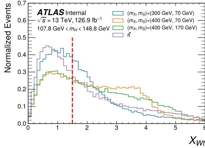
Figure 7.12: The distribution of the top veto discriminant, X_{Wt} with signal samples of (m_X \text{ GeV}, m_S \text{ GeV}) : (300,70), (400,70), (400,170) and the simulated t\bar{t} . Requiring that X_{Wt} > 1.5 as an additional kinematic cut would result in a significant loss in signal events for these samples despite the background reduction.
