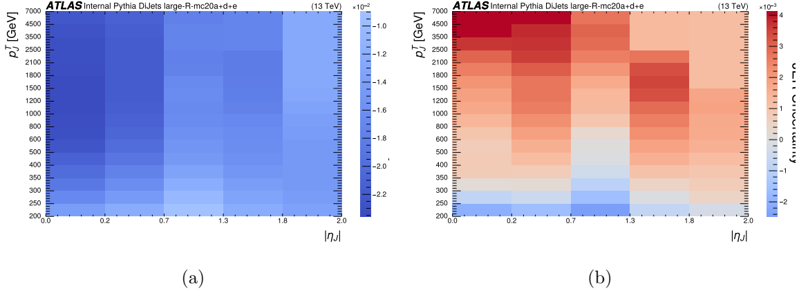
Figure 4.11: Jet energy uncertainties as a function of jet \eta and p_T , derived by comparing FullSim and AF3 Pythia DiJet samples for large- R PFlow jets in the mc20 campaign. (a) Jet Energy Scale (JES) uncertainty, calculated according to Equation 4.2, indicates a general overestimation of the response in AF3 relative to FullSim. (b) Jet Energy Resolution (JER) uncertainty, defined in Equation 4.4, tends to increase with higher p_T at fixed \eta . Irregular features at high p_T and in forward regions are attributed to limited MC statistics.
