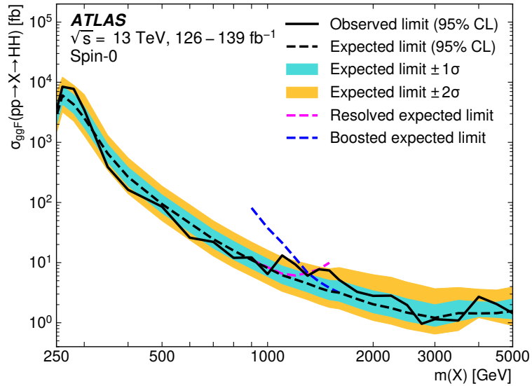
Figure 3.1: Expected (dashed black lines) and observed (solid black lines) 95% CL upper limits on the cross section times the branching ratio of resonant HH production in the spin-0 model. The inner green (outer yellow) bands represent the 1\sigma and 2\sigma uncertainties. Expected limits using each of the resolved and boosted channels individually (dashed colored lines) are shown [105].
