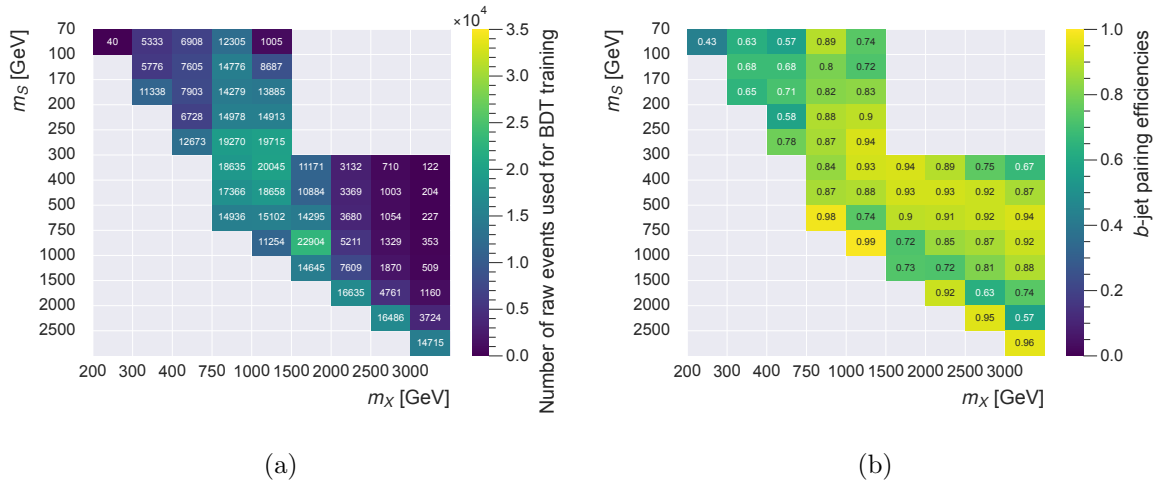
Figure 2.2: (a) Number of simulated events passing selection in the training dataset. (b) BDT pairing efficiencies for different signal mass points, defined as the weighted fraction of selected events with the correct pairing identified. See SH4b Internal Note [145].
