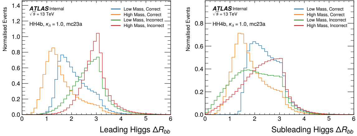
Figure 1.1: Truth distribution of the angular distance between the b -quarks for the (a) leading and (b) subleading Higgs bosons in the mc23a signal, showing both correct and incorrect pairings for low-mass ( m_{HH} < 450 GeV) and high-mass ( m_{HH} > 450 GeV) events.
