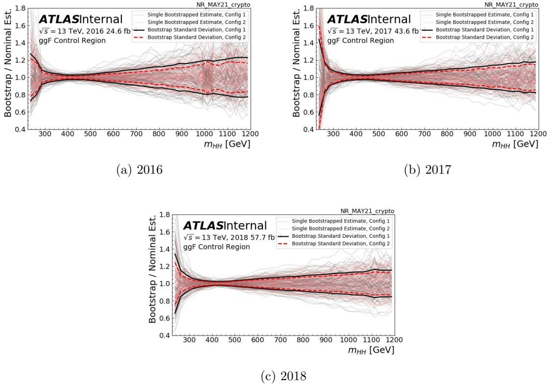
Figure 8.5: The bootstrap band procedure, shown as a ratio to the nominal (average) estimate in the CR1. Each lightly colored line is from the m_{HH} prediction for a single bootstrap training while the darker line shows the standard deviation of histograms for its corresponding dataset. All three years are included separately for ggF from configurations 1 (black) and 2 (red).
