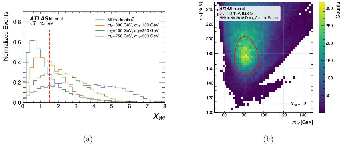
Figure 6.6: (a) Distribution of the top veto discriminant X_{Wt} for simulated t\bar{t} background and X \rightarrow SH \rightarrow b\bar{b}b\bar{b} signal hypotheses, showing reduced separation when m_S is near the top quark or W boson mass. (b) Reconstructed W boson and top quark candidate masses in the non-resonant HH \rightarrow b\bar{b}b\bar{b} Control Region (2018 data), using the jet combination with minimum X_{Wt} (see Eq. 6.1). The ellipse marks the region excluded by the X_{Wt} cut.
