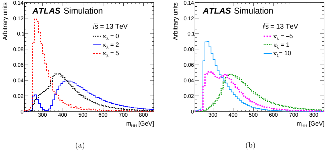
Figure 5.3: The destructive interference between the triangle and box diagrams of the ggF Higgs boson pair production showing how the distribution for m_{HH} , the invariant mass of the di-Higgs system, changes depending on the Higgs self-coupling value. The green line in 5.3b where \kappa_\lambda = 1 indicates the distribution for the Standard Model prediction [103].
