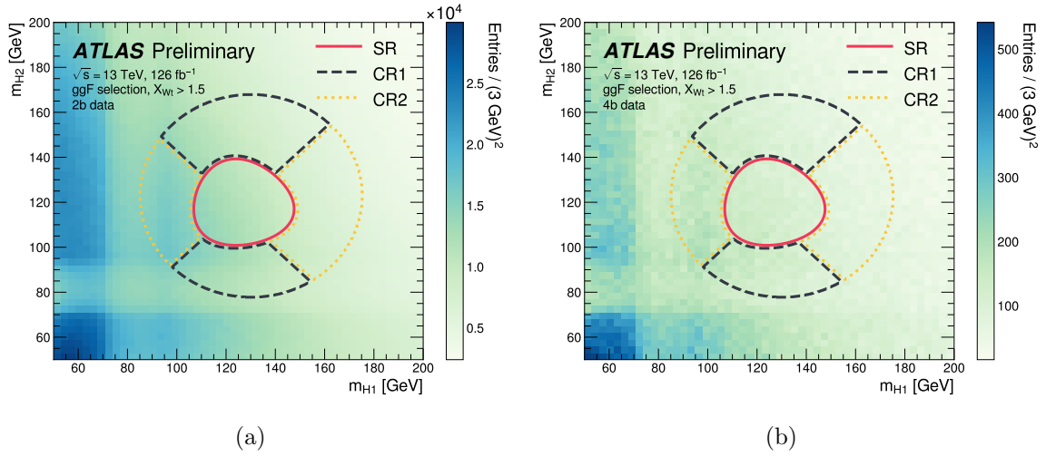
Figure 8.1: The (m_{H1}, m_{H2}) mass planes for (a) 2b and (b) 4b events from 2016-2018 data, showing the SR (red oval) and CR (surrounding bands). The full ggF selection is applied including a kinematic cut for X_{Wt} > 1.5 which greatly reduces the t\bar{t} background.
