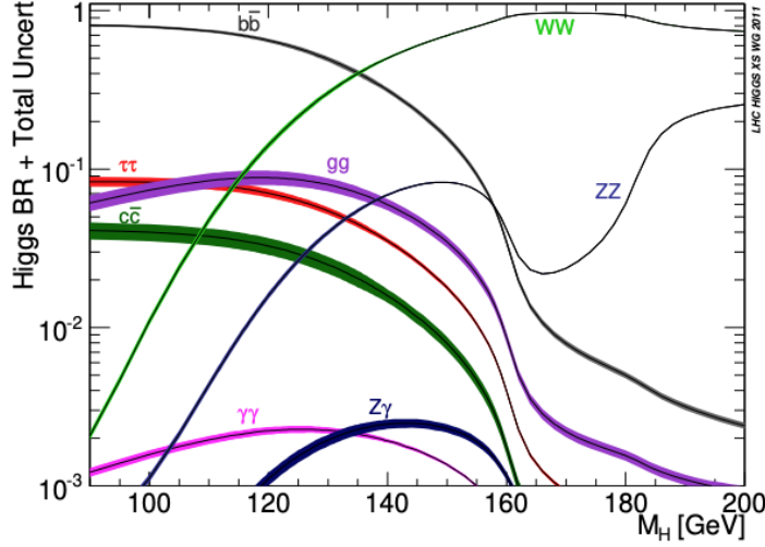
Figure 2.3: SM Higgs branching ratios and their uncertainties for possible Higgs boson masses in the range from 90 - 200 GeV [42].
