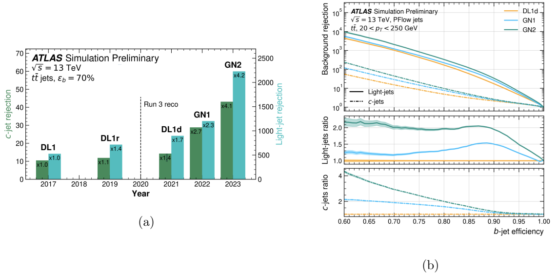
Figure 6.2: The c-jet and light-jet rejections of the different ATLAS flavor tagging algorithms over time in the t\bar{t} MC simulation in Figure 6.2a provided at the 70% efficiency b -tagging working point where the improvement is normalized to the DL1 tagger. The background rejection is also plotted against b -jet efficiency for the same samples in Figure 6.2b where the ratio for the different taggers is taken according to the DL1d tagger [141].
