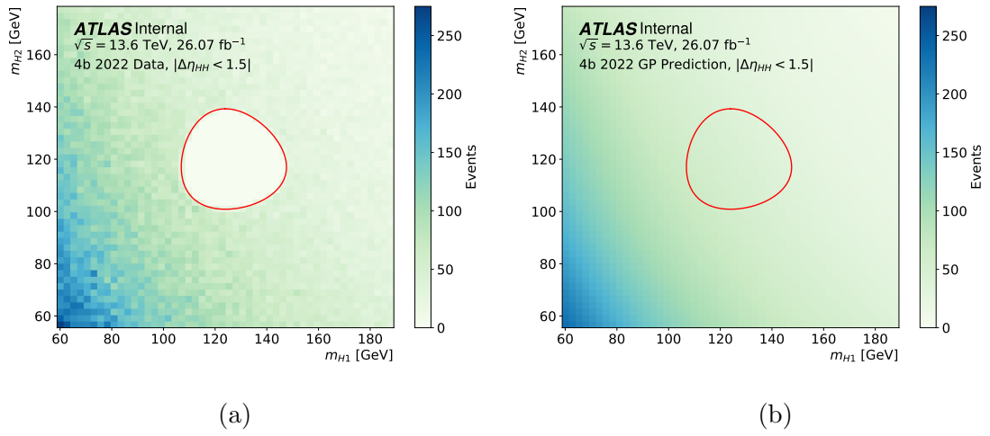
Figure 9.8: The distribution of the (a) data and the (b) average GP prediction over the (m_{H1}, m_{H2}) mass plane for the 4b data in 2022 for events where |\Delta\eta_{HH}| < 1.5 . The 4b data is blinded in the SR (red) of (a).
