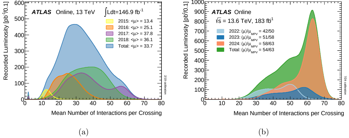
Figure 4.2: The average number of interactions per bunch crossing, \langle\mu\rangle , illustrating the pile-up density profiles for the data-taking years of Run 2 (4.2a) and Run 3 (4.2b) [50, 51].
