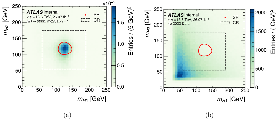
Figure 9.4: The (m_{H1}, m_{H2}) mass planes for (a) simulated SM signal (mc23a) and (b) blinded 4b data from 2022, showing the signal region (red ellipse) and control region (dashed black box) defined for the analysis. Higgs candidate masses are reconstructed using the min \Delta R pairing.
