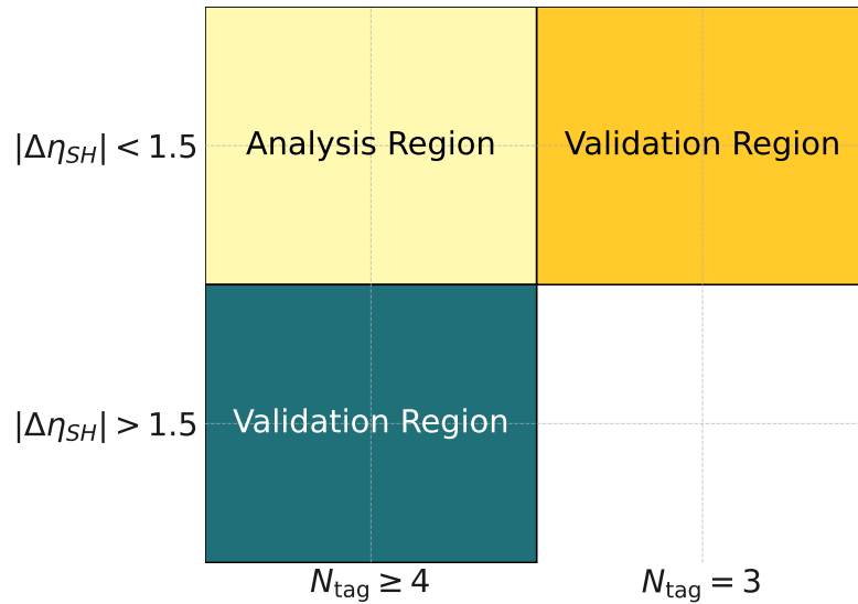
Figure 7.25: Definition of the validation regions used to test the data-driven background estimate. These regions are obtained by inverting kinematic cuts or altering the b -tag multiplicity from the nominal selection.
