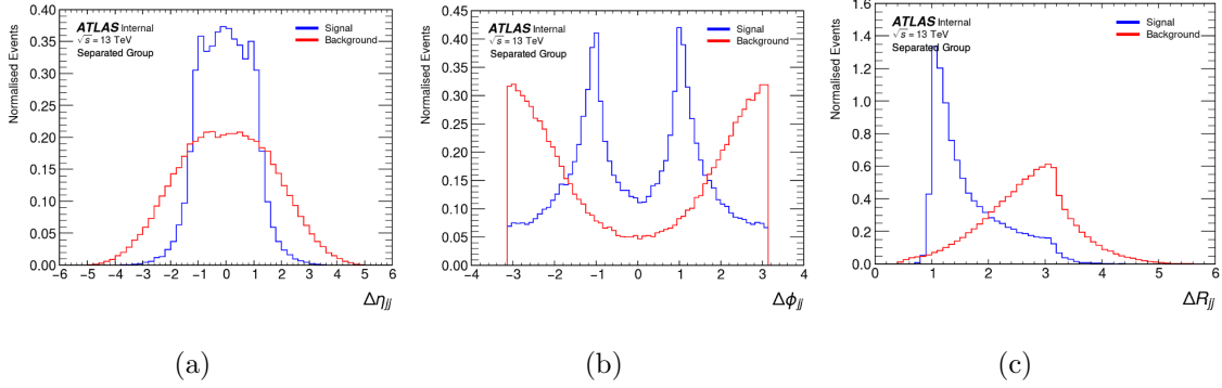
Figure 7.7: Distributions of key NN training inputs for the separated group: (a) \Delta\eta_{jj} , (b) \Delta\phi_{jj} , and (c) \Delta R_{jj} , for S and H candidates. The signal corresponds to correctly paired jets, while the background consists of incorrect pairings. The histograms are normalized to account for the fact that there are twice as many incorrect pairings as correct pairings per event.
