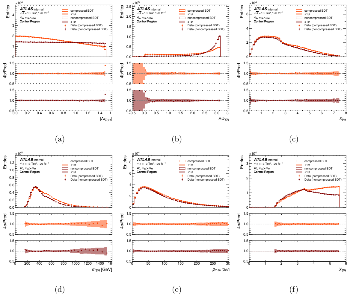
Figure 7.19: Distributions of kinematic variables of the SH candidates and event level variables X_{SH} and X_{Wt} for the predictions from the normalizing flows in the Control Region for the compressed and non-compressed BDT pairings when m_S > m_H .
