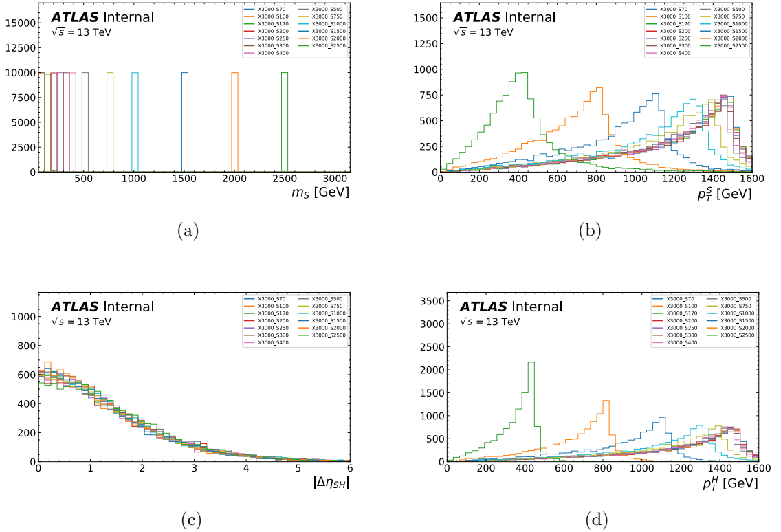
Figure 7.2: Truth-level distributions from the signal MC validation: (a) mass and (b) transverse momentum of the scalar boson S in addition to (c) |\Delta\eta_{SH}| and (d) the transverse momentum of the Higgs boson for all signal mass pairs at m_X = 3 TeV. These checks were used to verify correct event generation and kinematic coverage for the X \rightarrow SH \rightarrow bbbb analysis.
