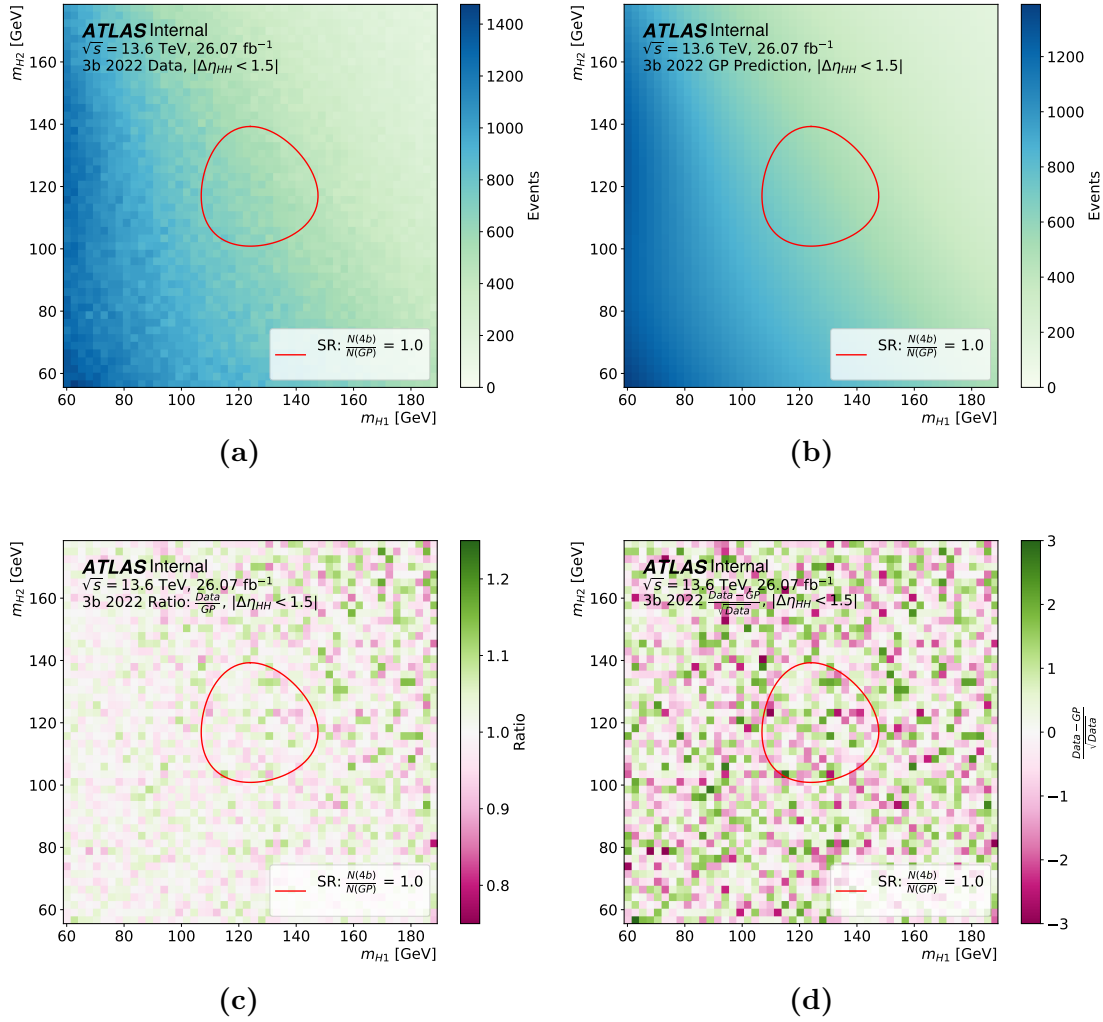
Figure 9.10: Binned distributions in the (m_{H1}, m_{H2}) mass plane for the 3b validation region with |\Delta\eta_{HH}| < 1.5 in 2022: (a) observed data, (b) GP-based background prediction, (c) ratio of data to prediction, and (d) the difference between data and prediction normalized to the statistical uncertainty in the data. The agreement between data and prediction is excellent across the phase space. The signal region ( X_{HH} < 1.6 ) is indicated by the red contour.
