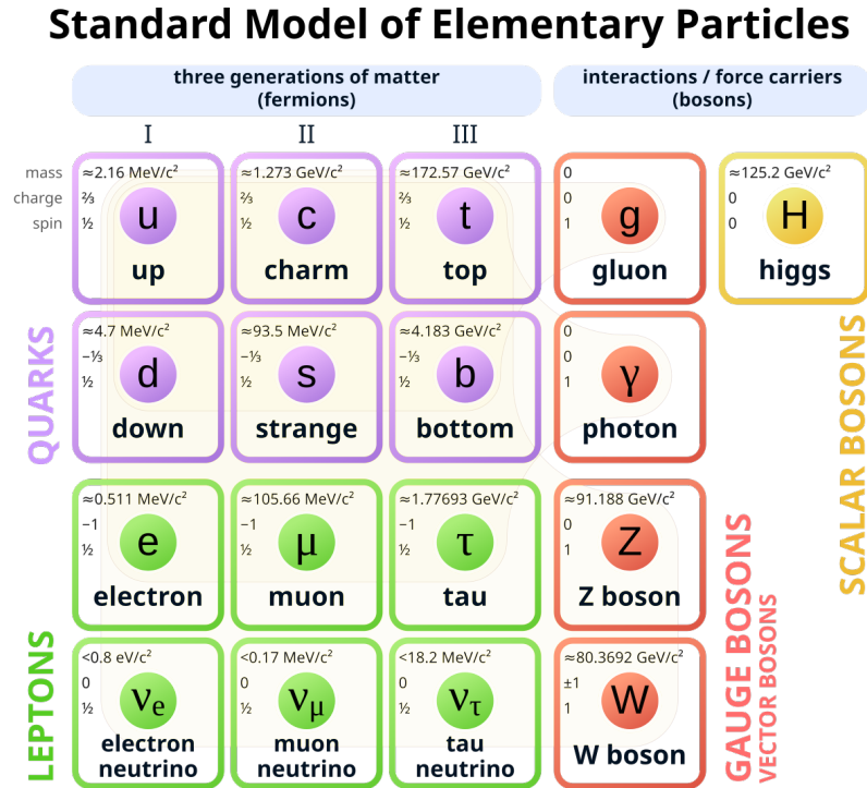
Figure 2.1: The fundamental particles of the Standard Model illustrating the different classifications and generations of matter and the force carriers that mediate their interactions [15].
