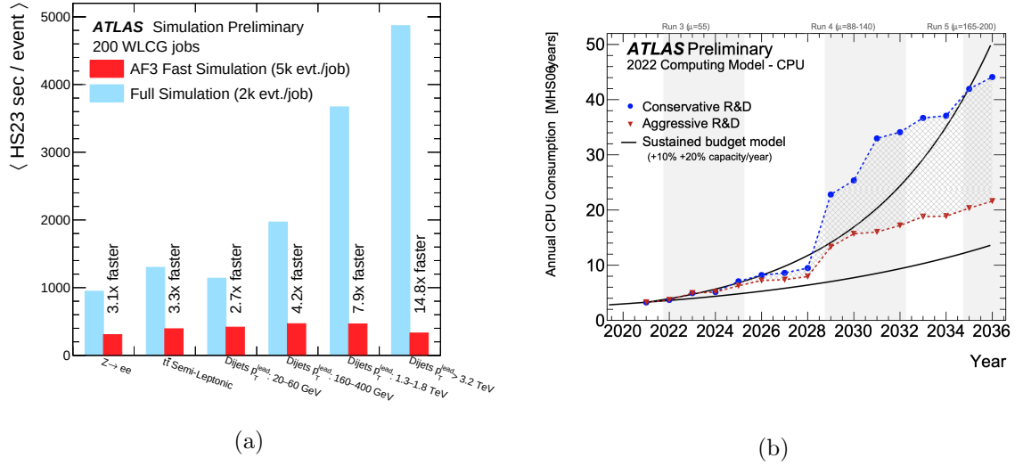
Figure 4.3: The mean CPU time per event simulated in Fast Simulation (AF3) and Full Simulation measured in standardized HS23 seconds for six different physics processes in 4.3a. Figure 4.3b show projected CPU consumption for the ATLAS experiment from 2020 to 2036 varies based on R&D investment [90, 91].
