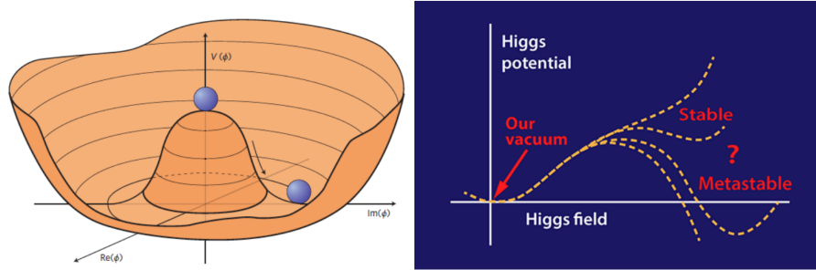
Figure 5.1: The Higgs potential, featured on the left, for \mu^2 < 0 . Choosing any of the points at the bottom of the potential spontaneously breaks the rotational U(1) symmetry. Quantum corrections, featured on the right, can change the shape of the Higgs potential indicating whether the universe is stable or metastable. Here, the minimum of our vacuum is taken at |\phi| = \frac{v}{\sqrt{2}} . [98]
