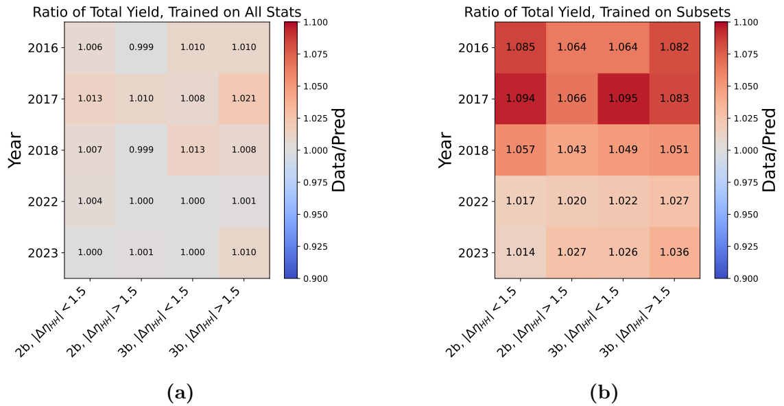
Figure 9.12: Ratio of the total data yield to the predicted background yield in the signal region for each 2b and 3b validation region, shown separately for all data-taking years. Panel (a) shows the result when the normalizing flows and Gaussian processes are trained on the full statistics, while panel (b) presents the average ratio from models trained on 10 downsampled subsets (each averaged over 25 seeds). The comparison illustrates the degree of non-closure in each region, with a pronounced under-prediction of the total yield for Run 2 years, reaching up to 10% in the most extreme case, while the agreement is notably improved for the Run 3 years though still not perfect.
