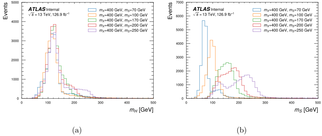
Figure 7.8: Reconstructed mass distributions using the NN pairing for m_X = 400 GeV: (a) m_H and (b) m_S . Clear mass peaks are observed, with a small excess near 125 GeV in (b) due to events where jets are correctly paired but S and H assignments are swapped.
