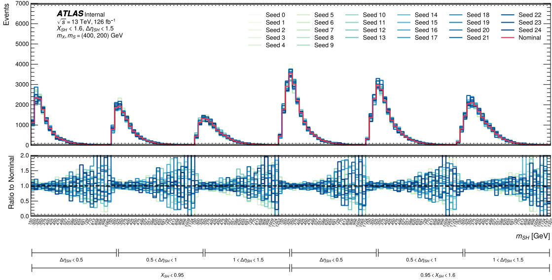
Figure 7.21: Twenty five predictions of the categorized m_{SH} distributions from the normalizing flows, each conditioned on a different GP sample for the non-compressed signal region ( m_X = 400 GeV, m_S = 200 GeV). The average prediction is shown in red. See the SH4b Internal Note [145].
