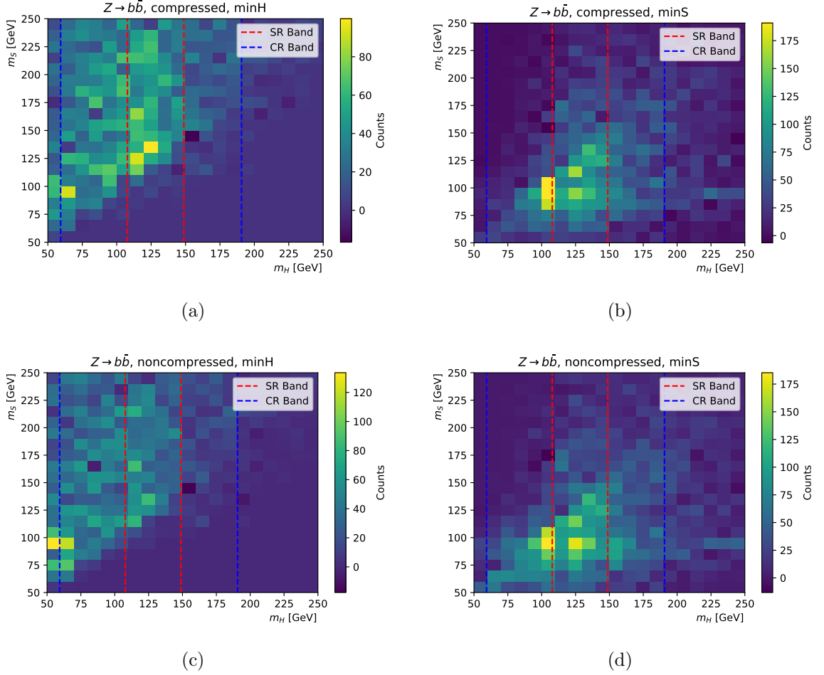
Figure 7.17: Distributions of m_H versus m_S for Z \rightarrow b\bar{b} production, shown in the four BDT pairing configurations: (a) compressed/minH, (b) compressed/minS, (c) non-compressed/minH, and (d) non-compressed/minS. The signal band (encompassing all sub-signal regions) and control region are indicated. These distributions demonstrate that the Z \rightarrow b\bar{b} background is smoothly distributed across the mass plane and does not introduce any problematic resonance within the signal region.
