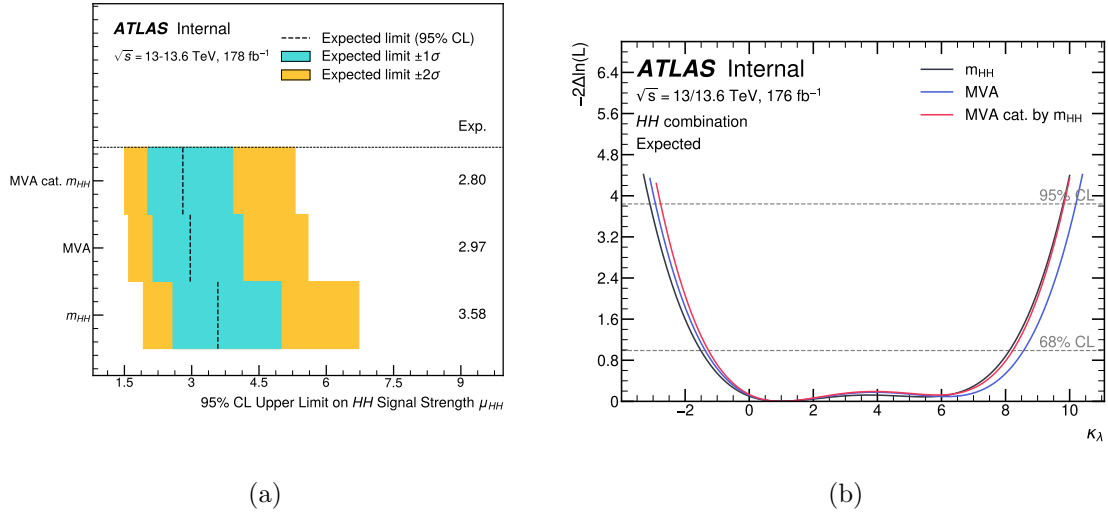
Figure 9.13: (a) Expected 95% CL upper limits on the signal strength for non-resonant HH \rightarrow b\bar{b}b\bar{b} production via ggF in the resolved channel, shown for three discriminants: categorized m_{HH} , MVA, and MVA categorized in m_{HH} . The median expected limit is presented along with the \pm 1\sigma and \pm 2\sigma uncertainty bands, assuming no signal contribution. (b) Expected 68% and 95% confidence level upper limits on non-resonant HH \rightarrow b\bar{b}b\bar{b} production as a function of \kappa_\lambda , for each discriminant strategy with all other couplings fixed to their Standard Model values.
