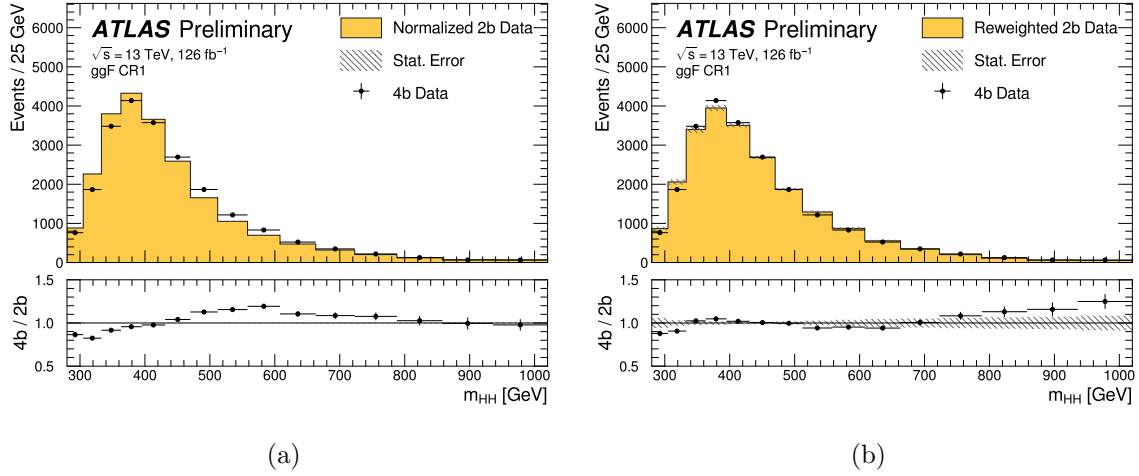
Figure 8.3: Distributions of m_{HH} in 4b data (black points) within Control Region 1 (CR1) of the ggF selection. (a) The yellow histogram shows the 2b CR1 m_{HH} distribution normalized to the 4b yield; (b) the yellow histogram shows the 2b CR1 after NN reweighting. Hatched bands indicate the statistical uncertainty on the 2b sample: Poisson only in (a), and including the bootstrap uncertainty in (b).
