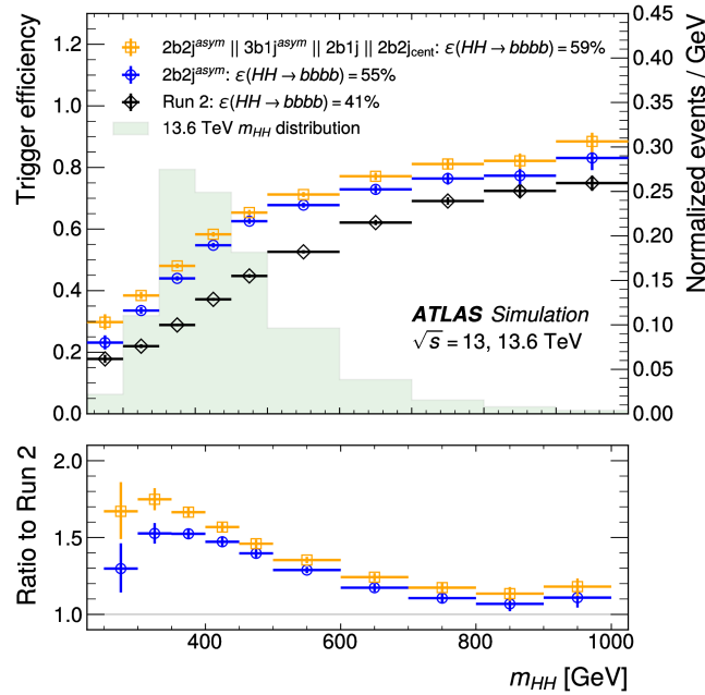
Figure 8.10: Performance of the b -jet trigger HLT selections in simulated HH \rightarrow b\bar{b}b\bar{b} events. The trigger efficiency, evaluated relative to all inclusive HH \rightarrow b\bar{b}b\bar{b} events, is shown as a function of the true di-Higgs boson invariant mass, m_{HH} . The efficiency is presented for the 2b2j^{asym} selection and for the logical OR of the 2b2j^{asym} , 3b1j^{asym} , 2b1j , and 2b2j^{cent} triggers and is compared with the trigger strategy employed in Run 2 [156].
