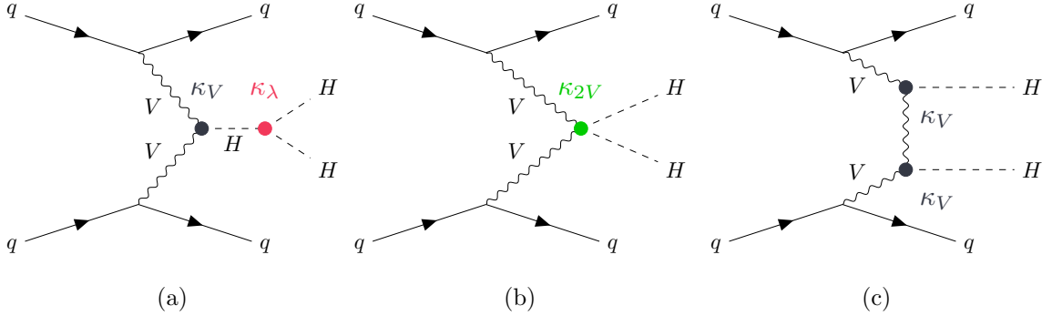
Figure 5.4: Feynman diagrams illustrating the three main contributions to non-resonant Higgs pair production via vector boson fusion (VBF). The process proceeds through: 5.4a a diagram involving the Higgs self-coupling, proportional to \kappa_\lambda ; 5.4b a diagram featuring a direct coupling of two Higgs bosons to vector bosons, governed by \kappa_{2V} ; 5.4c a diagram with a single-Higgs coupling to vector bosons, proportional to \kappa_V [102].
