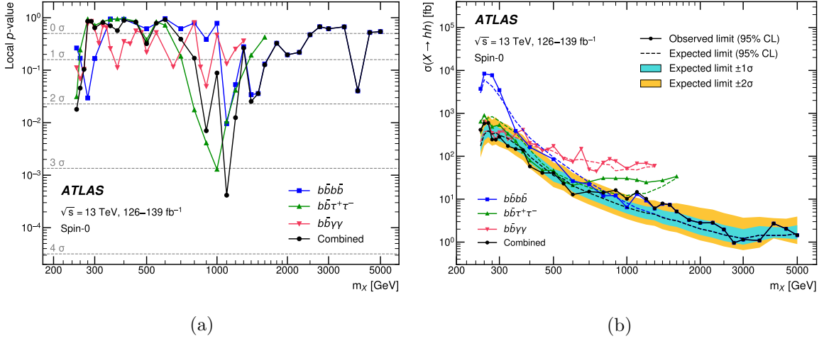
Figure 5.8: (a) Local p -value and (b) observed and expected upper limits at the 95% CL on the resonant Higgs boson pair production cross section as a function of the resonance mass m_X [109].
