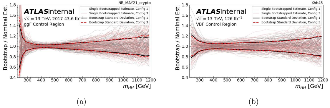
Figure 8.6: The bootstrap band procedure, shown as a ratio to the nominal (average) estimate in the CR1. Each lightly colored line is from the m_{HH} prediction for a single bootstrap training while the darker line shows the standard deviation of histograms for its corresponding dataset. Data for 2017 for the ggF analysis (a) and for all three years from the VBF analysis (b) are included for configurations 1 (black) and 3 (red).
