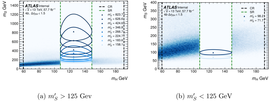
Figure 7.15: Mass plane and kinematic regions for 2018 data, using the BDT pairing in the non-compressed region for a selected number of m'_S mass points considered in the resolved analysis. a shows the m_H - m_S mass plane and kinematic regions for m'_S > 125 GeV and b shows this for m'_S < 125 GeV
