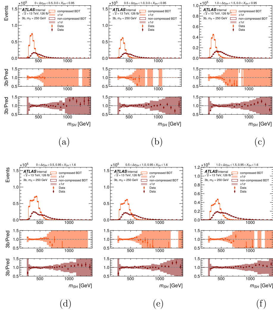
Figure 7.27: The categorized m_{SH} distribution in the 3b signal region for m_S = 250 GeV. The six subplots correspond to: (a) Category 0: 0.0 < |\Delta\eta_{SH}| < 0.5 , 0.0 < X_{SH} < 0.95 , (b) Category 1: 0.5 < |\Delta\eta_{SH}| < 1.0 , 0.0 < X_{SH} < 0.95 , (c) Category 2: 1.0 < |\Delta\eta_{SH}| < 1.5 , 0.0 < X_{SH} < 0.95 , (d) Category 3: 0.0 < |\Delta\eta_{SH}| < 0.5 , 0.95 < X_{SH} < 1.6 , (e) Category 4: 0.5 < |\Delta\eta_{SH}| < 1.0 , 0.95 < X_{SH} < 1.6 , and (f) Category 5: 1.0 < |\Delta\eta_{SH}| < 1.5 , 0.95 < X_{SH} < 1.6 .
