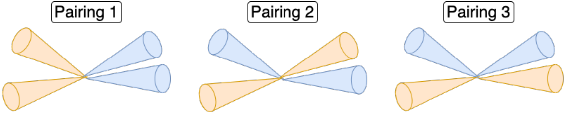
Figure 6.4: There are six possible ways to reconstruct four small- R jets into two unique scalars and three possible ways to reconstruct them into two identical scalars.
