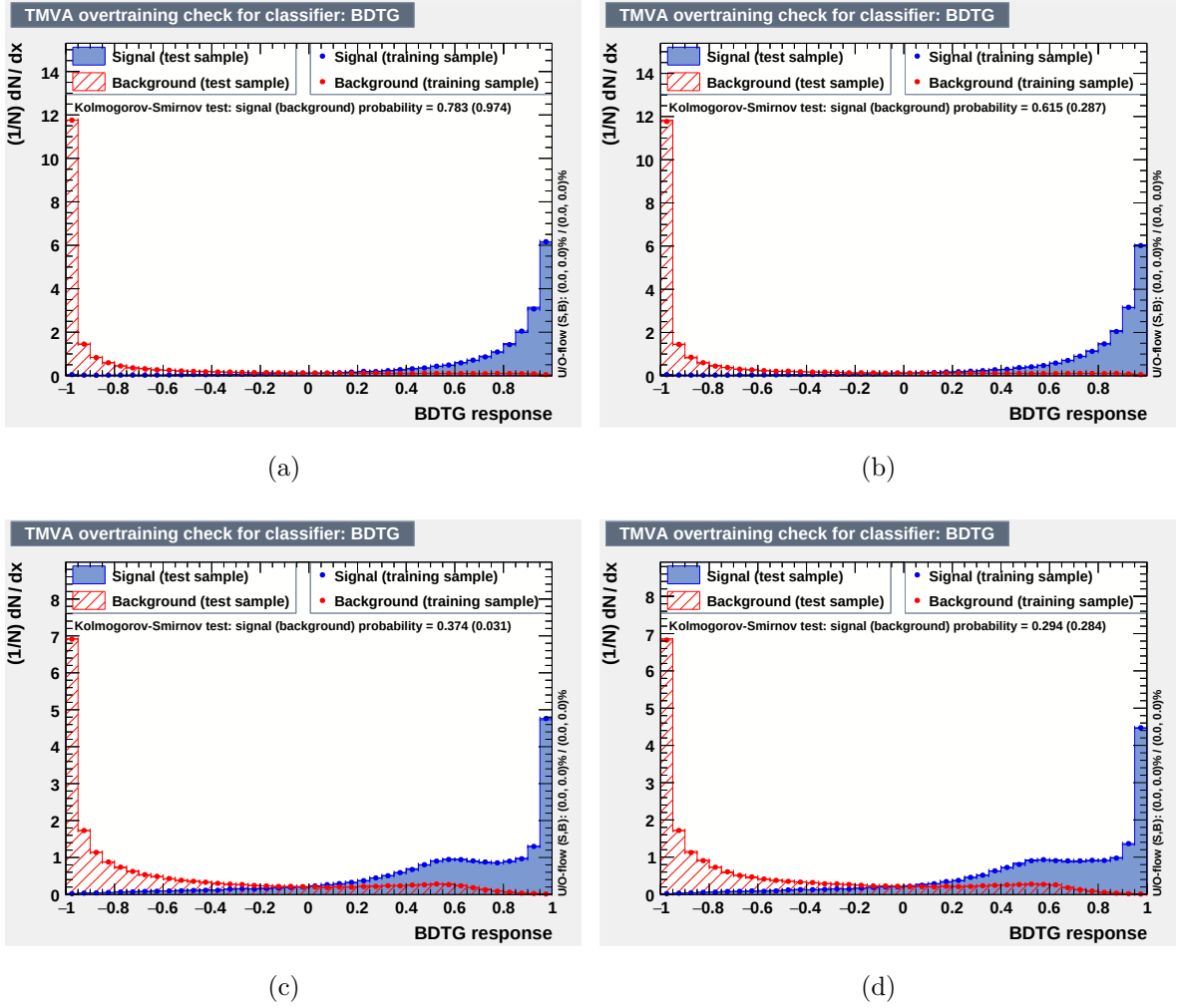
Figure 2.1: Distributions of the BDT output for signal (correct pairing, score near 1) and background (incorrect pairing, score near -1) for (a) odd and (b) even events in the compressed region, and (c) odd and (d) even events in the non-compressed region. The agreement between training and test samples indicates no overtraining. See SH4b Internal Note [145].
