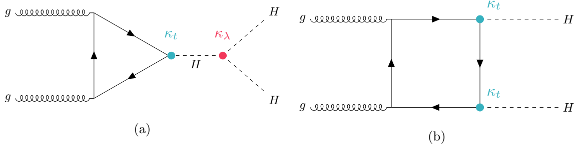
Figure 5.2: The Feynman diagrams for the non-resonant Higgs boson pair production through gluon-gluon fusion (ggF) where the triangle diagram in 5.2a works through a top loop process including the Higgs self-coupling while the box diagram in 5.2b does not include the self-coupling. These diagrams destructively interfere [101, 102].
