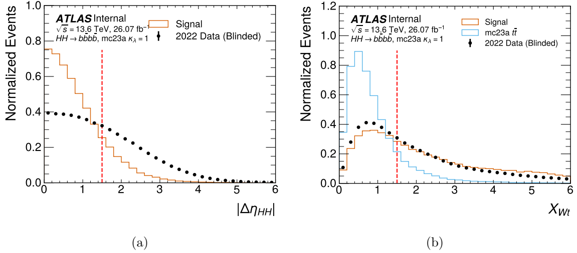
Figure 9.5: Distributions of the simulated SM mc23a signal and blinded four- b data from 2022, where events in the signal region (SR) are masked, for (a) |\Delta\eta_{HH}| and (b) X_{Wt} . The red vertical lines indicate the kinematic selection cuts: |\Delta\eta_{HH}| < 1.5 and X_{Wt} < 1.5 . The X_{Wt} distribution also shows the simulated t\bar{t} background, demonstrating the effectiveness of the veto in suppressing this background while preserving signal events.
