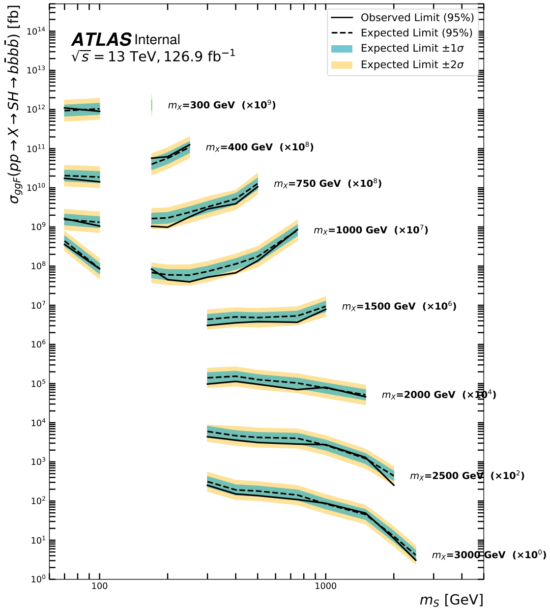
Figure 7.33: Observed (solid black line) and expected (dashed black line) 95% CL upper limits on the cross section times the branching ratio. For each unique m_X value, where a scaling factor is applied to the limits so that all mass pairs can be visualized together. The inner green (outer yellow) bands represent the 1\sigma and 2\sigma uncertainties, respectively. The mass grid used in this analysis allows for interpolation across m_S , except in regions between m_S = 100 \text{ GeV} and m_S = 170 \text{ GeV} .
