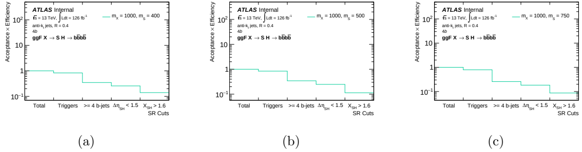
Figure 7.13: Acceptance \times efficiency plots obtained for the trigger, 4b selections, QCD background rejection ( \Delta\eta_{SH} ) selections in SRs defined by X_{SH} < 1.6 , when using the BDT-paired jets for m_X = 1000 GeV and (a) m_S = 400 GeV, (b) m_S = 500 GeV, (c) m_S = 750 GeV. See the SH4b Internal Note [145].
