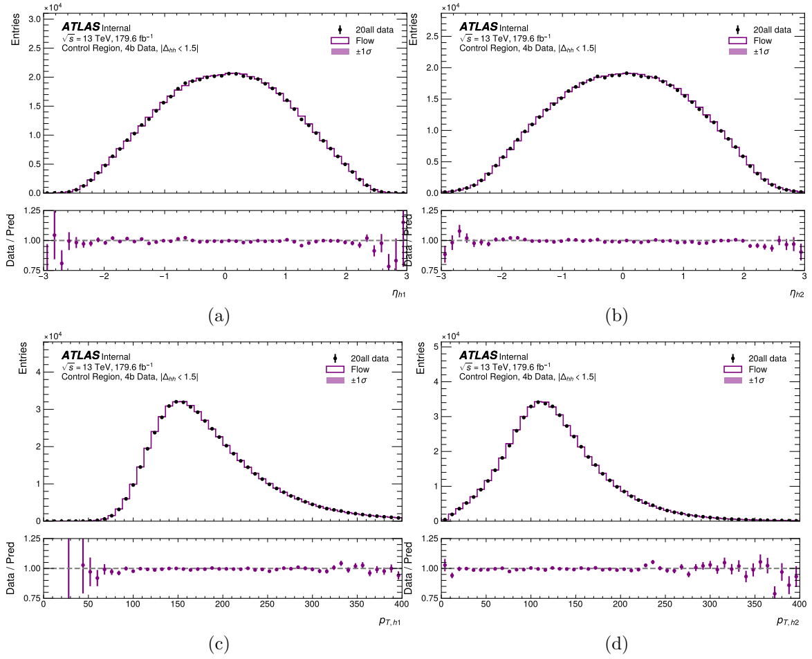
Figure 9.6: Distributions of 4b data and normalizing flow predictions for all data-taking years (2016–2018, 2022–2023) in the control region: (a) \eta_{H1} , (b) \eta_{H2} , (c) p_{T,H1} , and (d) p_{T,H2} . There is overall great closure between data and prediction.
