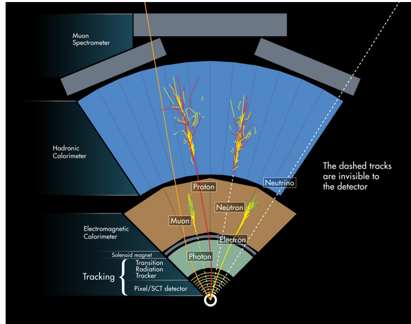
Figure 3.10: A 2D slice of the ATLAS Detector showing the different subdetector systems and how they function for object reconstruction in the events. The dashed lines indicate the neutrinos that pass through undetected.
