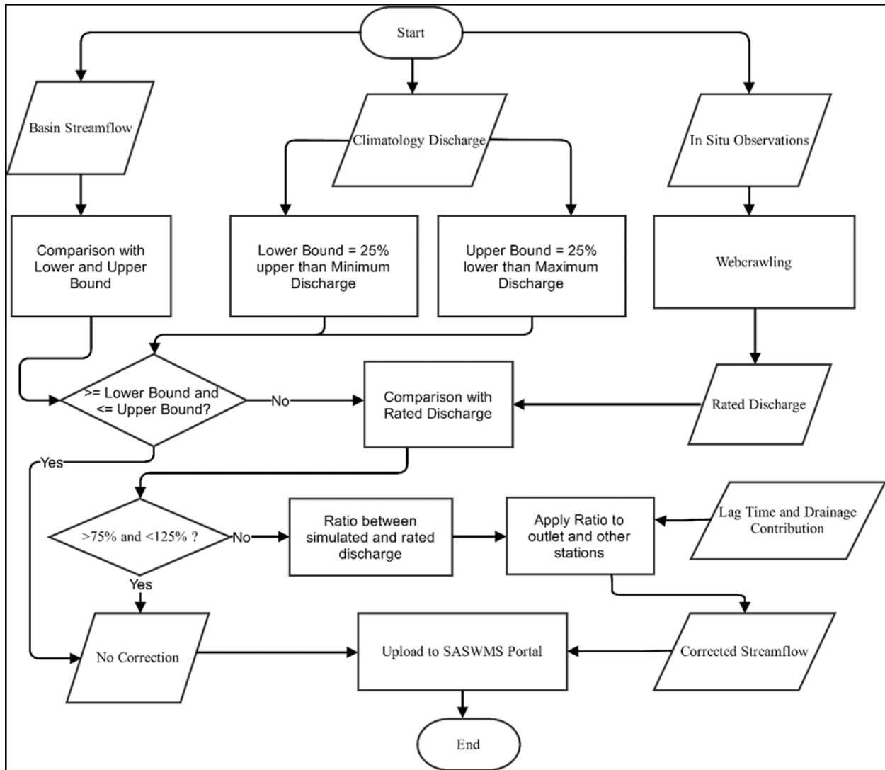
Figure 2.12. Streamflow correction Methodology
