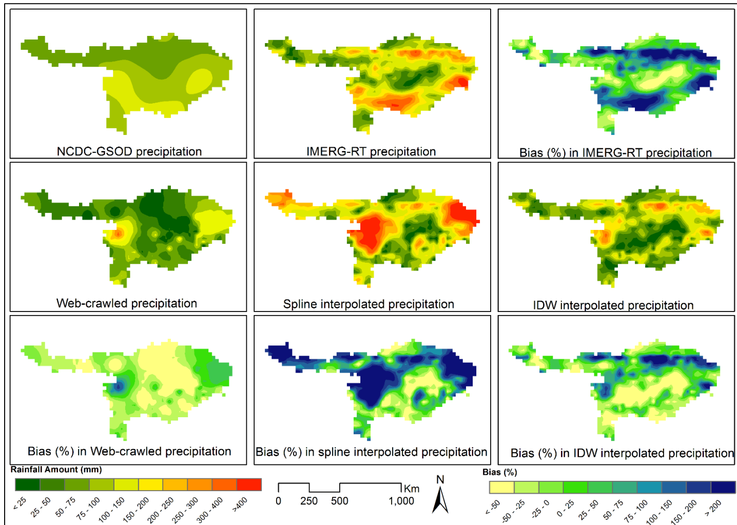
Figure A.19. Comparison of precipitation from IMERG, Web crawled, IDW bias interpolated and spline bias interpolated precipitation along with bias amount (in percentage with respect to NCDG-GSOD precipitation) in every product over Brahmaputra Basin for dry (January-March) season.
