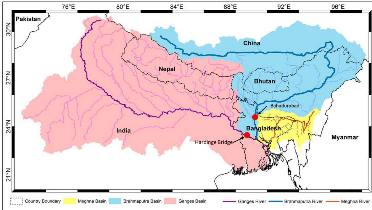
Figure 1.3. Ganges-Brahmaputra-Meghna Basin
