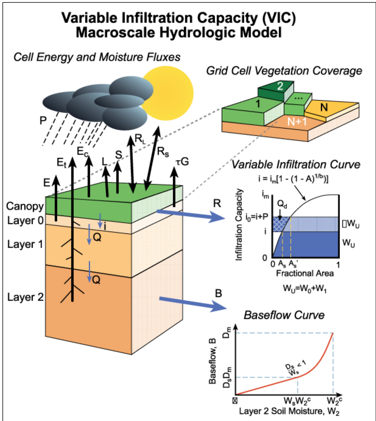
Figure 2.1. Schematic diagram of Variable Infiltration Capacity (VIC) Hydrological Model. (Image Source: Figure 1 of http://vic.readthedocs.io/en/master/Overview/ModelOverview/ )
