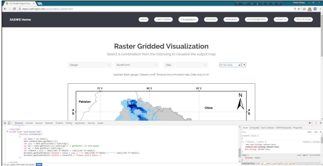
Figure A.11. Date Time Initialization using JavaScript
