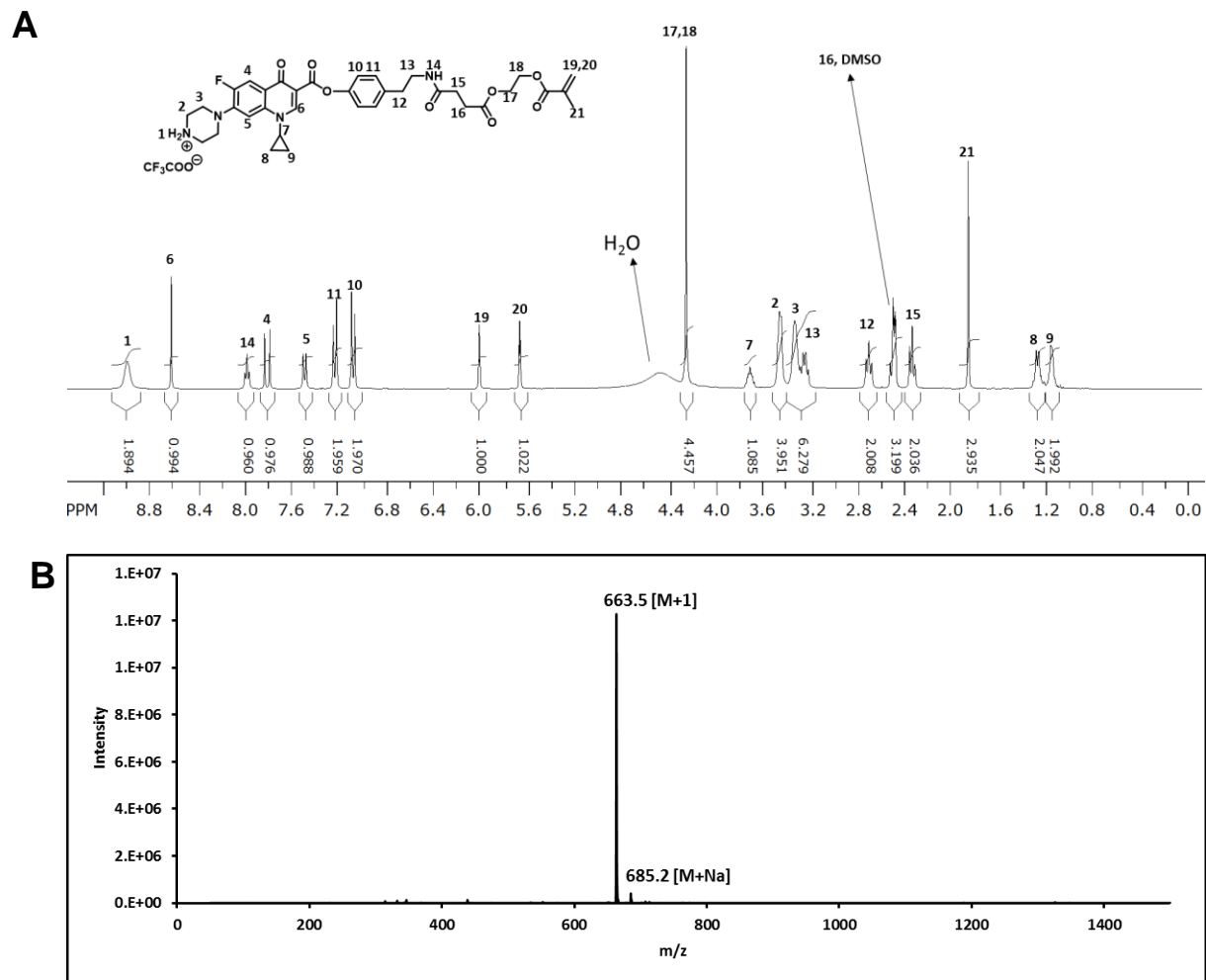
Figure 3.7. (A) 1 H-NMR spectrum of CTM and (B) ESI-Mass spectrum of CTM.
