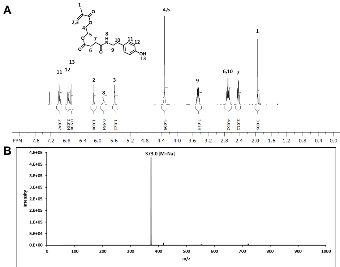
Figure 3.4. (A) ^1\text{H-NMR} spectrum of butanoic acid, 4-[(4-hydroxyphenyl)ethylamino]-4-oxo, 1-(2-methacryloyloxy)ethyl ester (1) and (B) ESI-Mass spectrum of butanoic acid, 4-[(4-hydroxyphenyl)ethylamino]-4-oxo, 1-(2-methacryloyloxy)ethyl ester (1).
