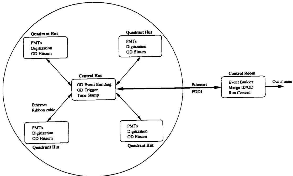
Figure 6.1: Overview of outer detector DAQ electronics
