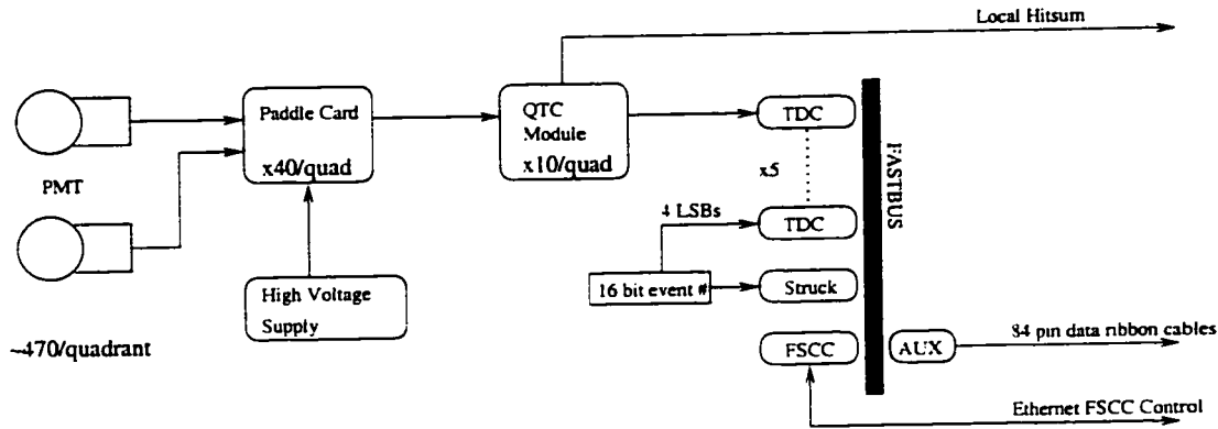
Figure 6.2: OD DAQ quadrant electronics
