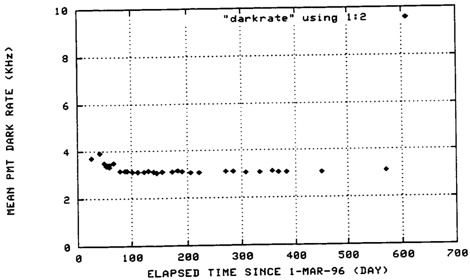
Figure 9.4: Dark rate for inner detector photo-multiplier tubes
