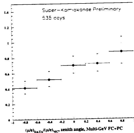
Figure 13.30: R versus zenith angle, multi-GeV (FC+PC)
