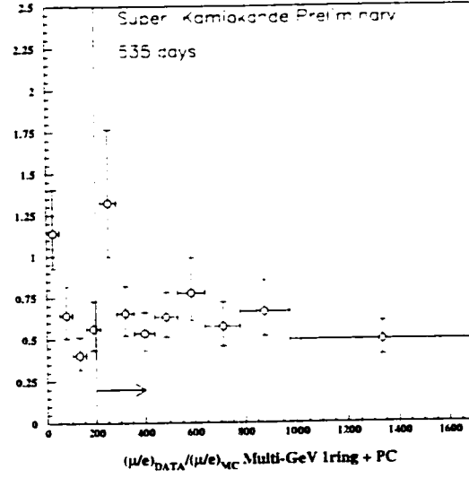
Figure 13.32: R versus wall distance, multi-GeV (FC+PC)
