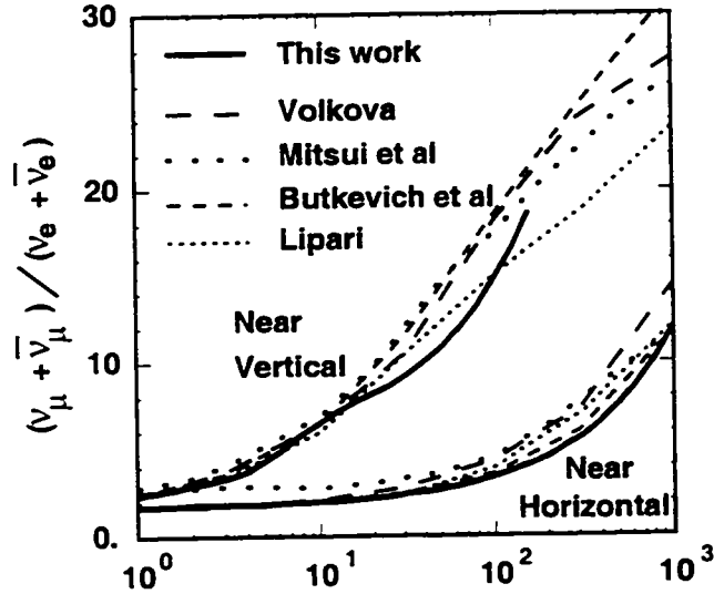
Figure 11.1: Neutrino flux ratio versus E_\nu (GeV), from [2].
