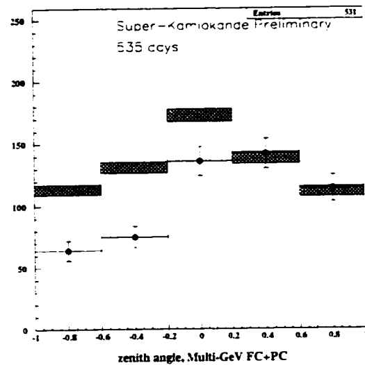
Figure 13.26: Zenith angle distribution, \mu -like, multi-GeV (FC+PC)
