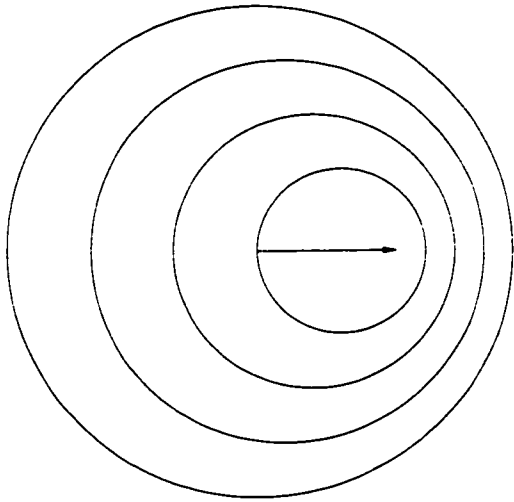
Figure 4.2: Particle with v < c/n
