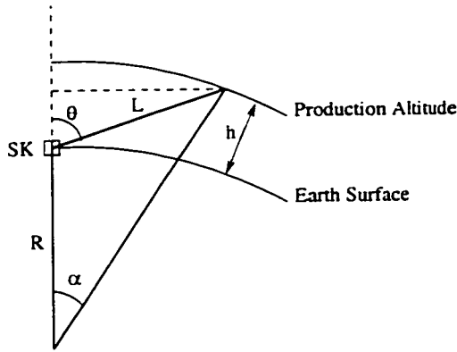
Figure 14.1: Neutrino Path Length Calculation
