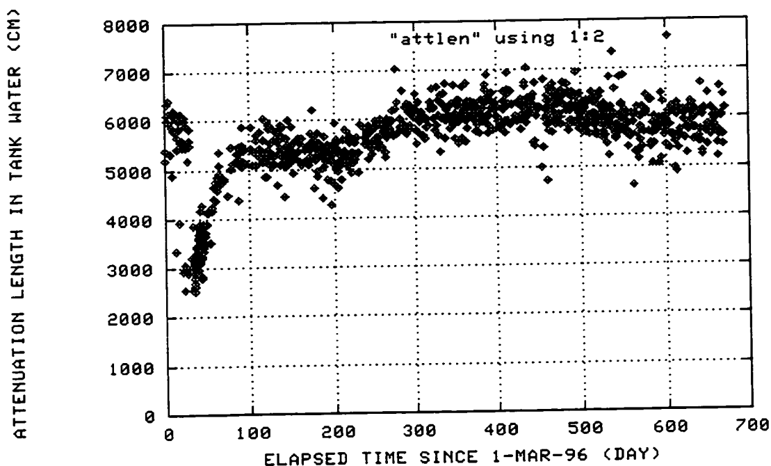
Figure 9.1: Attenuation length over time
