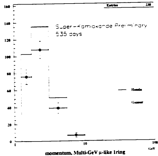
Figure 13.22: Muon-like momentum, 1-ring, multi-GeV (FC)
