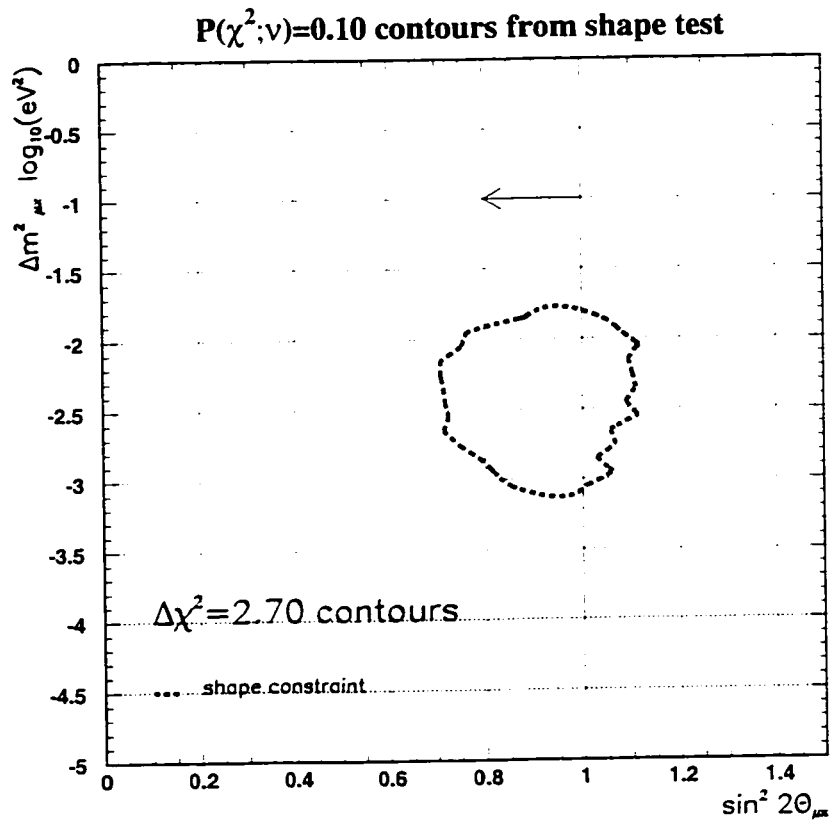
Figure 14.8: \Delta\chi^2 = 2.7 contours
