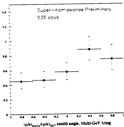
Figure 13.29: R versus zenith angle, multi-GeV (FC)
