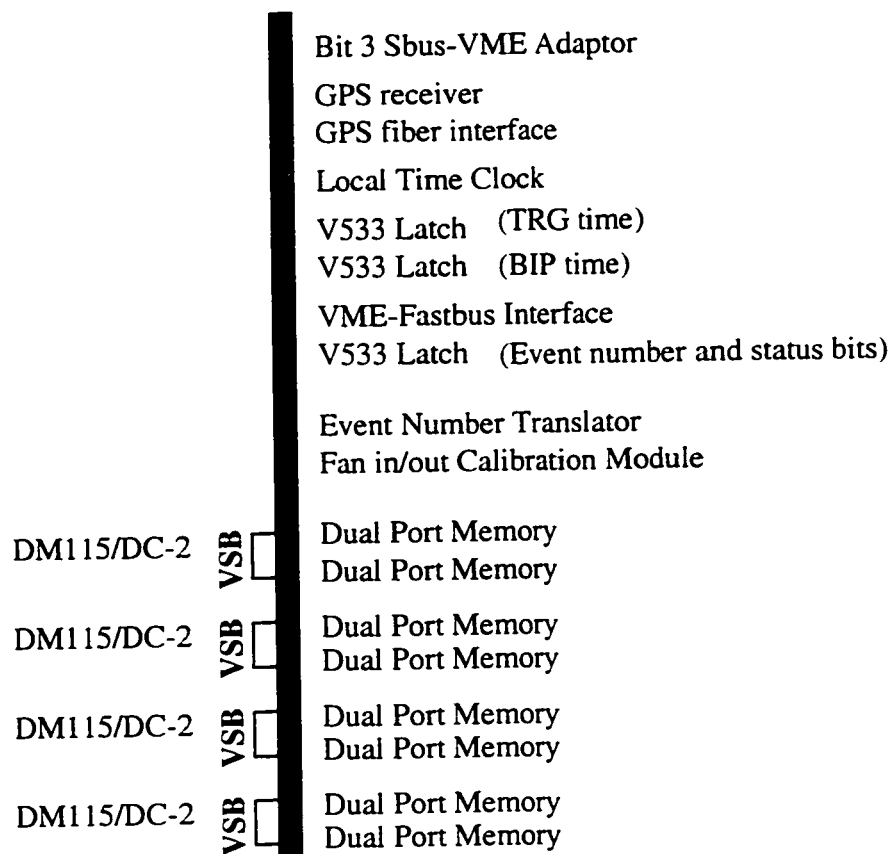
Figure 6.3: OD DAQ central hut VME crate modules
