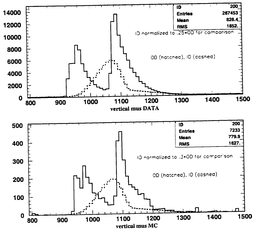
Figure 11.4: Time distributions
