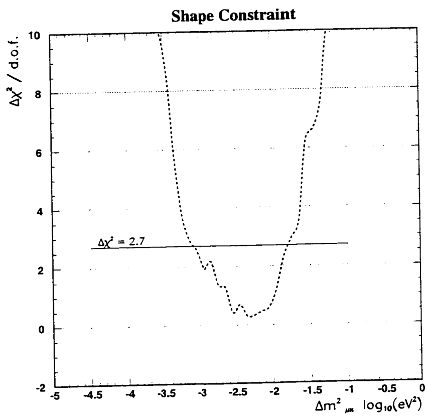
Figure 14.9: \Delta\chi^2/\text{d.o.f}
