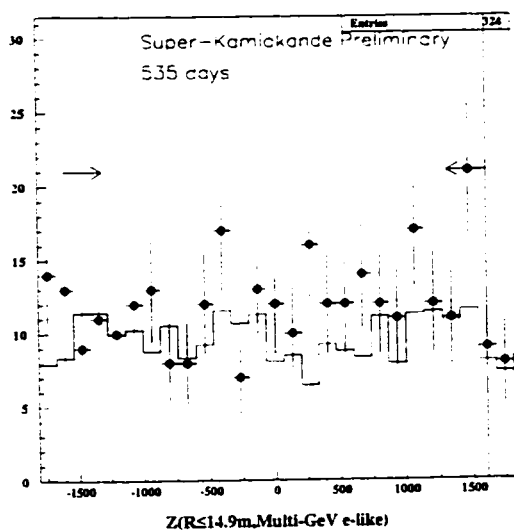
Figure 13.5: Z Distribution (FC e-like)
