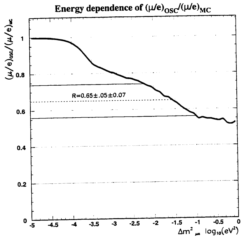
Figure 14.7: R vs \Delta m^2
