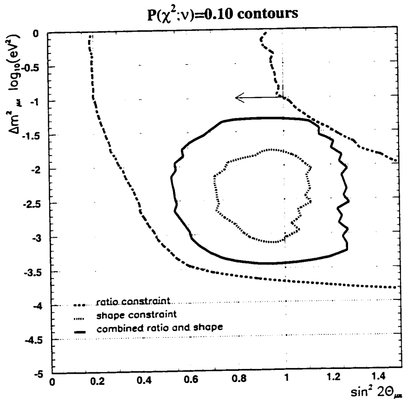
Figure 14.10: \Delta\chi^2 = 7.78 contours
