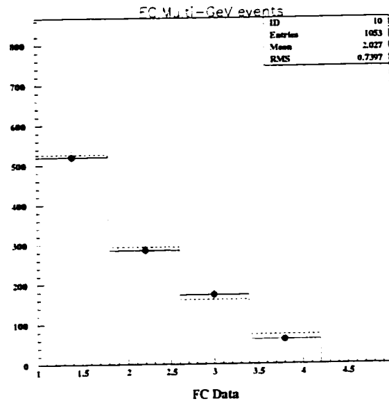
Figure 13.15: Number of rings (FC)
