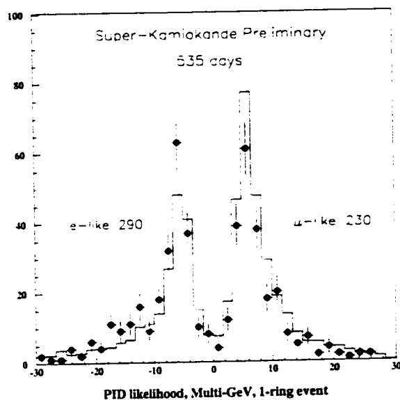
Figure 13.20: PID Likelihood for Multi-GeV 1-ring events (FC)
