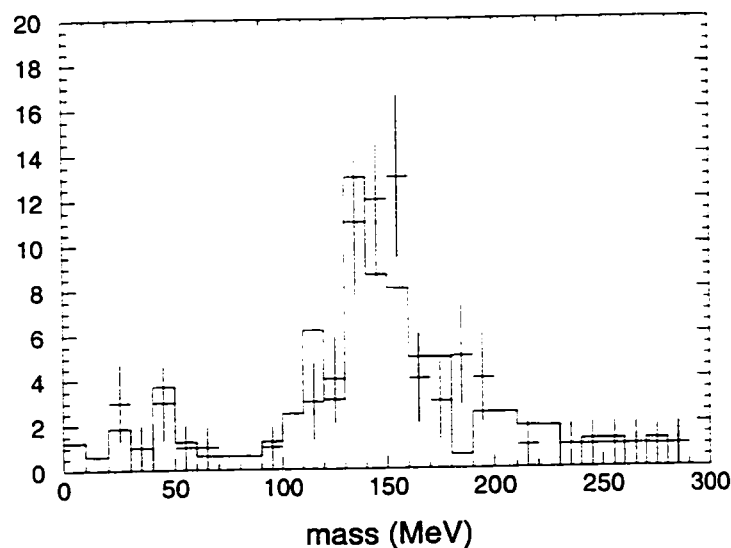
Figure 10.1: Reconstructed \pi^0 Mass
