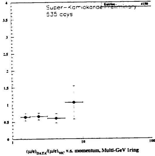
Figure 13.31: R versus momentum, multi-GeV (FC+PC)
