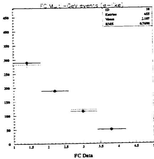
Figure 13.16: Number of rings (FC e-like)
