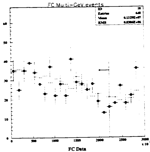
Figure 13.7: R^2 Distribution (FC)
