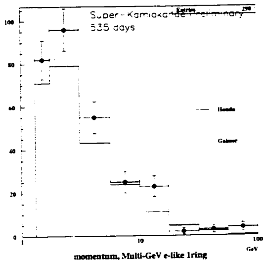
Figure 13.21: Electron-like momentum, 1-ring, multi-GeV (FC)
