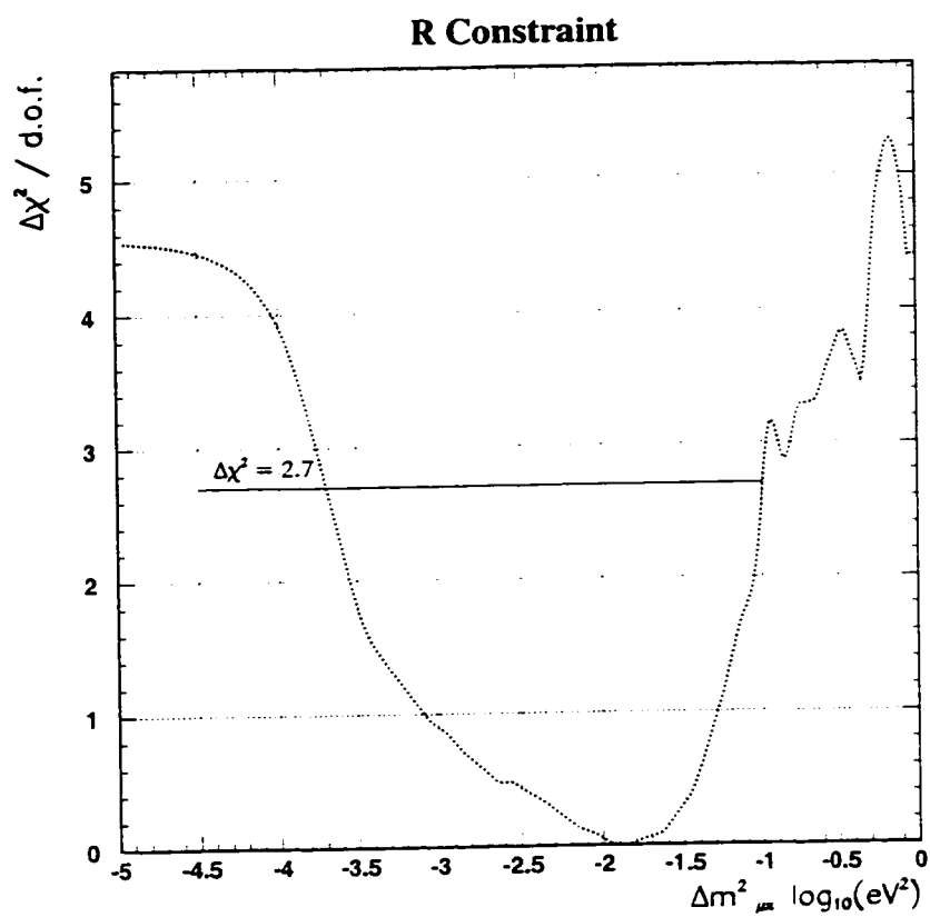
Figure 14.6: \Delta\chi^2/\text{d.o.f} for \sin^2(2\theta)=1
