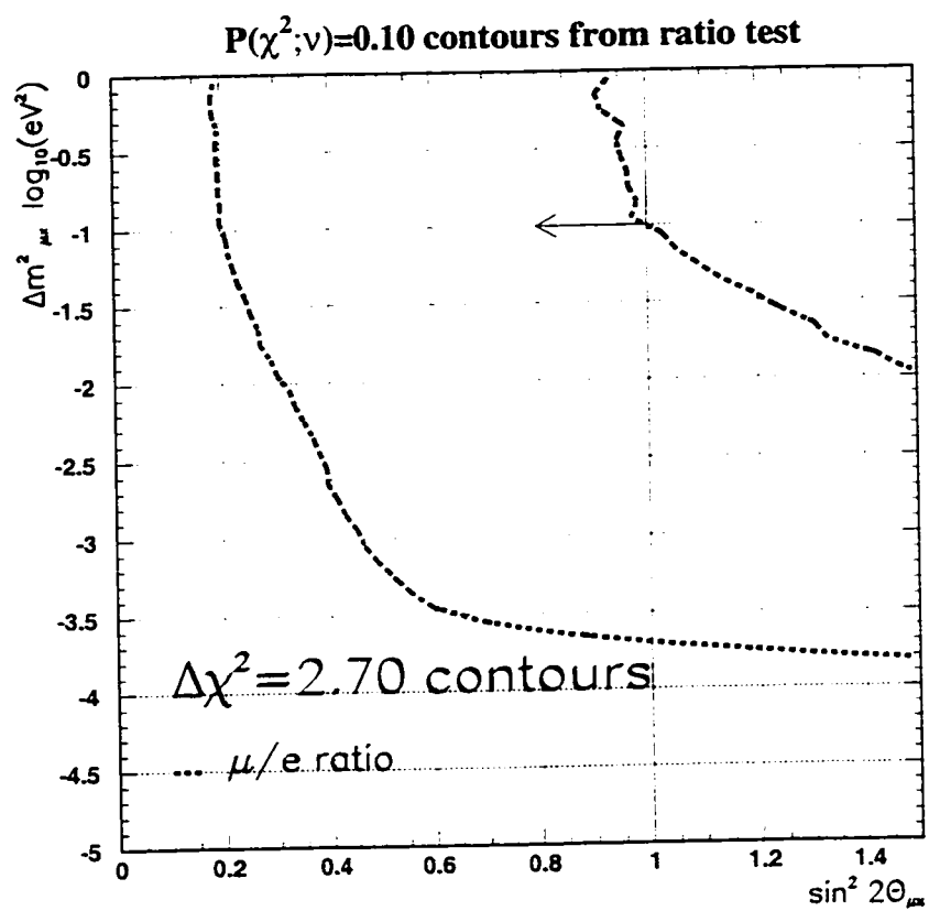
Figure 14.5: \Delta\chi^2 = 2.7 contours
