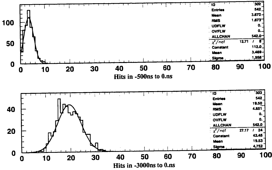
Figure 11.5: Good hit distributions for data
