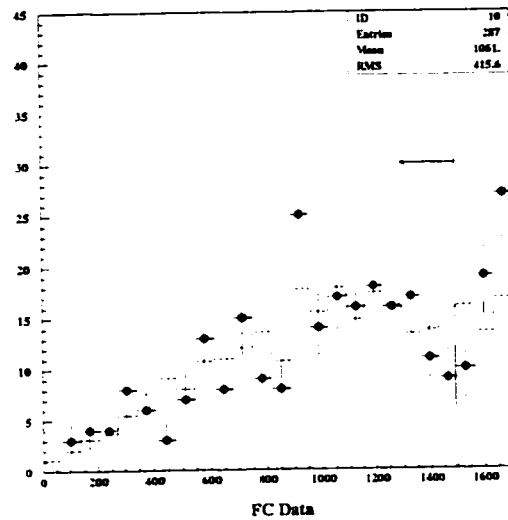
Figure 13.12: Radial Distribution (FC mu-like)
