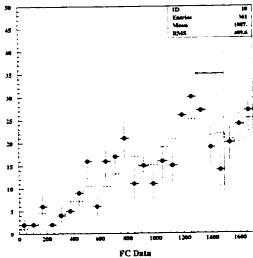
Figure 13.11: Radial Distribution (FC e-like)
