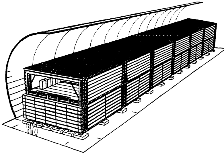
Figure 3.2: MACRO detector
