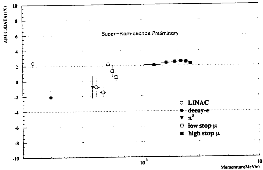
Figure 13.33: Comparison of calibration sources with Monte Carlo.
