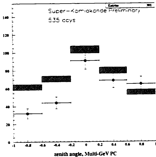
Figure 13.25: Zenith angle distribution, (PC)
