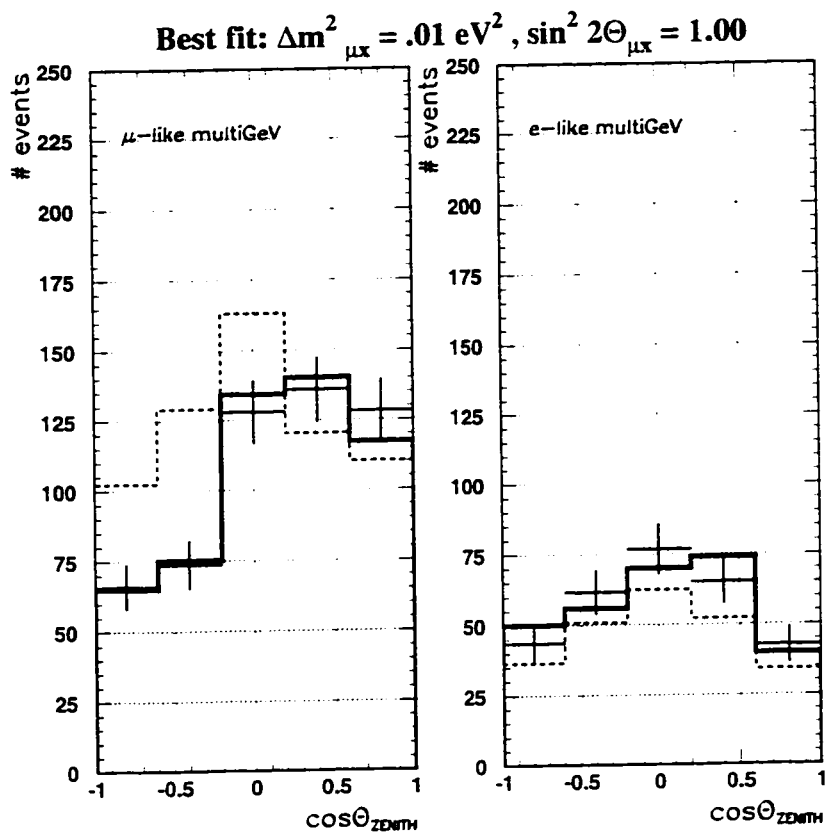
Figure 14.12: Comparison of data and Monte Carlo at best fit parameters
