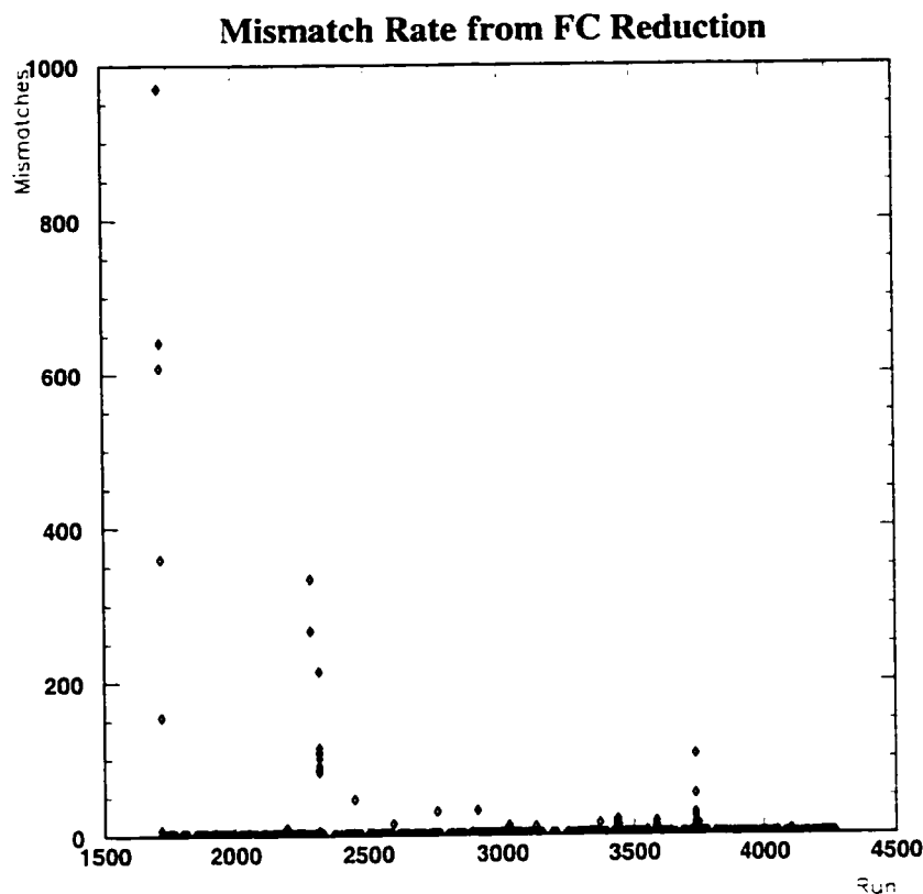
Figure A.2: Mismatched events vs. run
