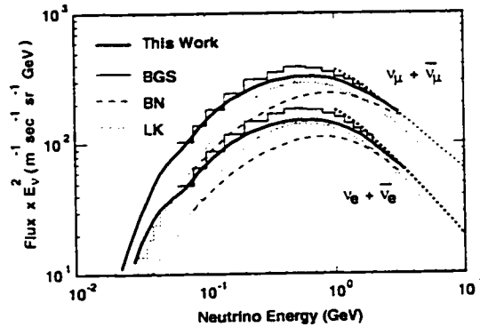
Figure 11.3: Atmospheric \nu fluxes multiplied by E_\nu^2 for the Kamioka site at solar mid from [2]. The dotted line is a high energy calculation without the rigidity cutoff.
