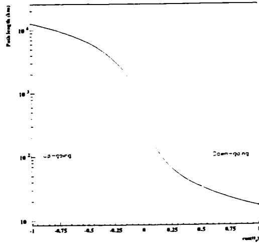
Figure 14.2: Neutrino flight path length vs. \cos(\theta_z)
