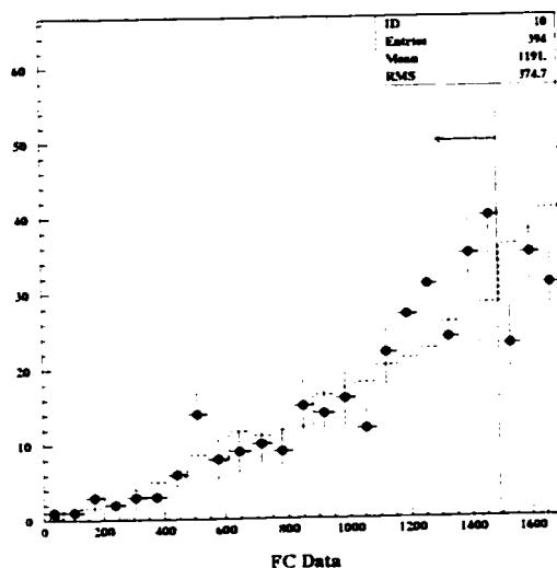
Figure 13.10: Radial Distribution (PC)
