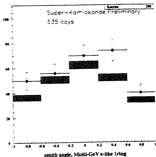
Figure 13.23: Zenith angle distribution, 1-ring e-like, multi-GeV (FC)
