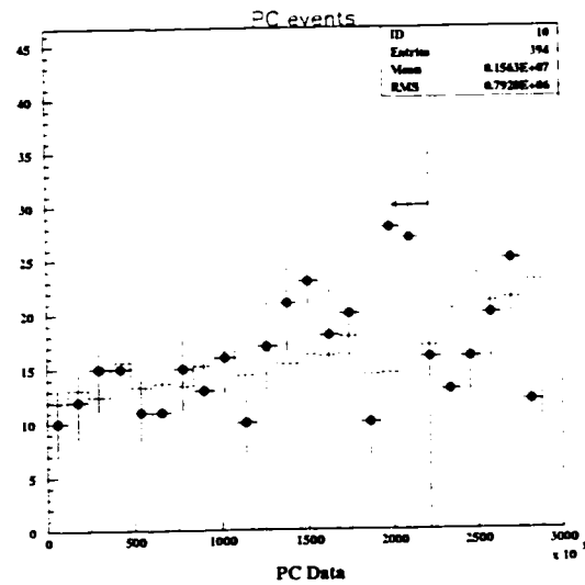
Figure 13.8: R^2 Distribution (PC)
