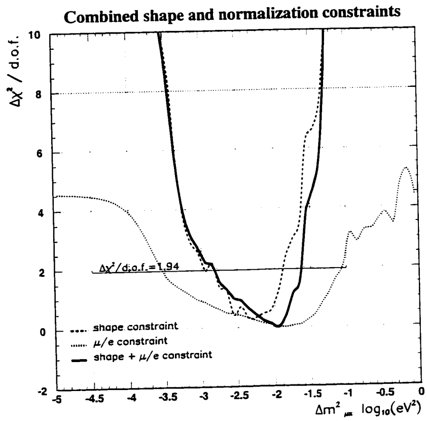
Figure 14.11: \Delta\chi^2/\text{d.o.f.}
