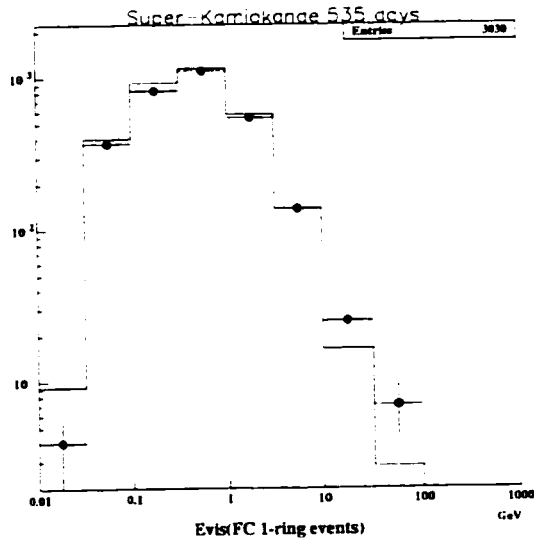
Figure 13.18: Visible energy (FC)
