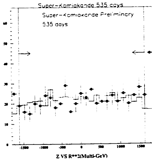
Figure 13.3: Z Distribution (FC)
