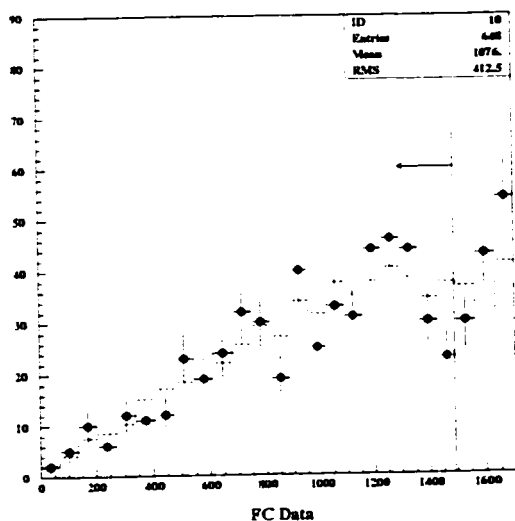
Figure 13.9: Radial Distribution (FC)
