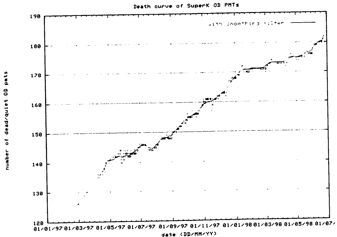
Figure 9.3: Outer detector tube death
