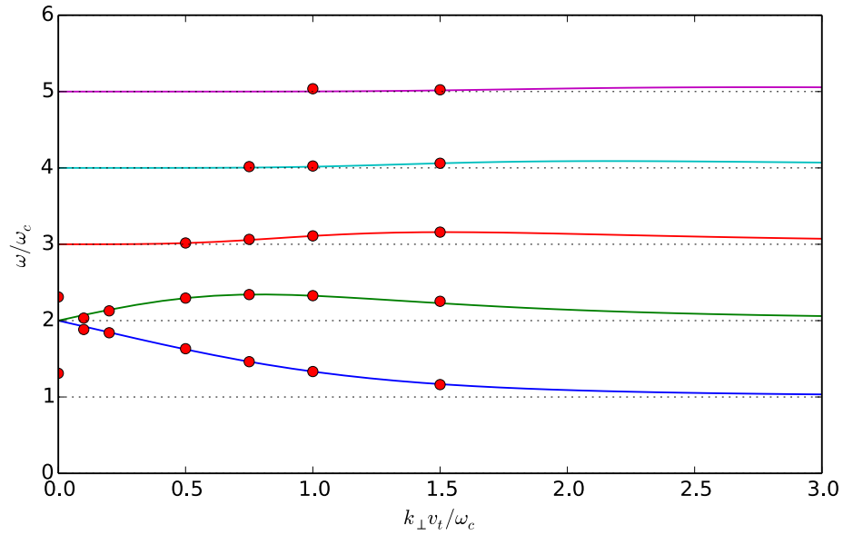
Figure 6.9: \omega_p^2 / \omega_c^2 = 3
