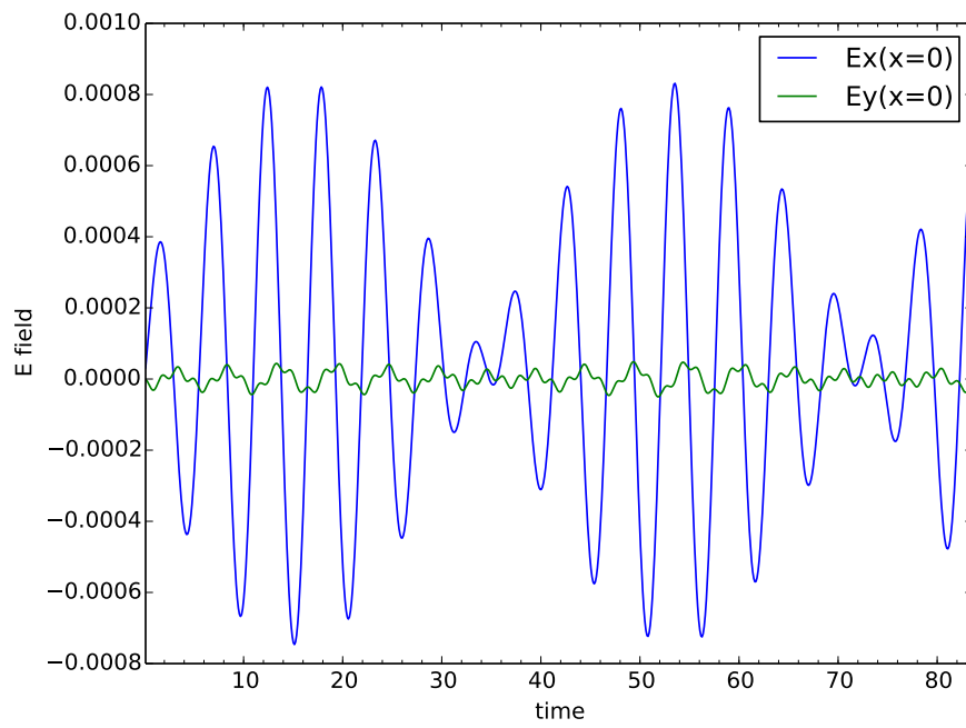
Figure 6.10: \omega_p^2/\omega_c^2 = 3
