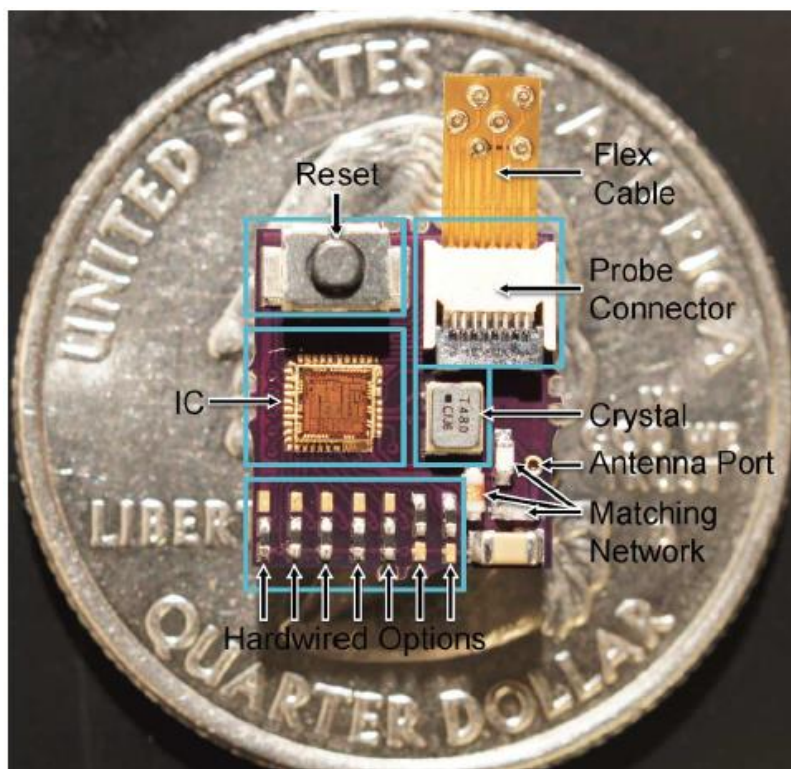
Figure 2.1 Deployable bio-signal system [11]
