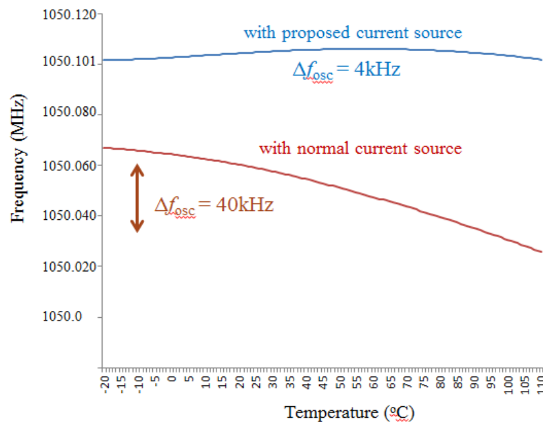
Figure 4.1 simulation result for resonance frequency drift with/without temperature compensated current source technique
