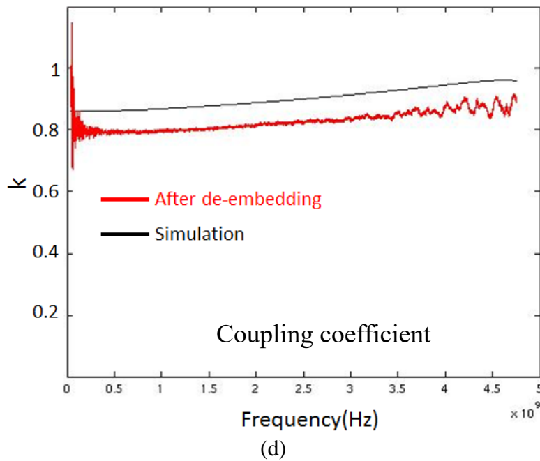
Figure 3.21 Test result with/without de-embedding process for (a) real and (b) imaginary part of Z_{11} , (c) inductance and (d) coupling coefficient for transformer with simulation result of electrical model
