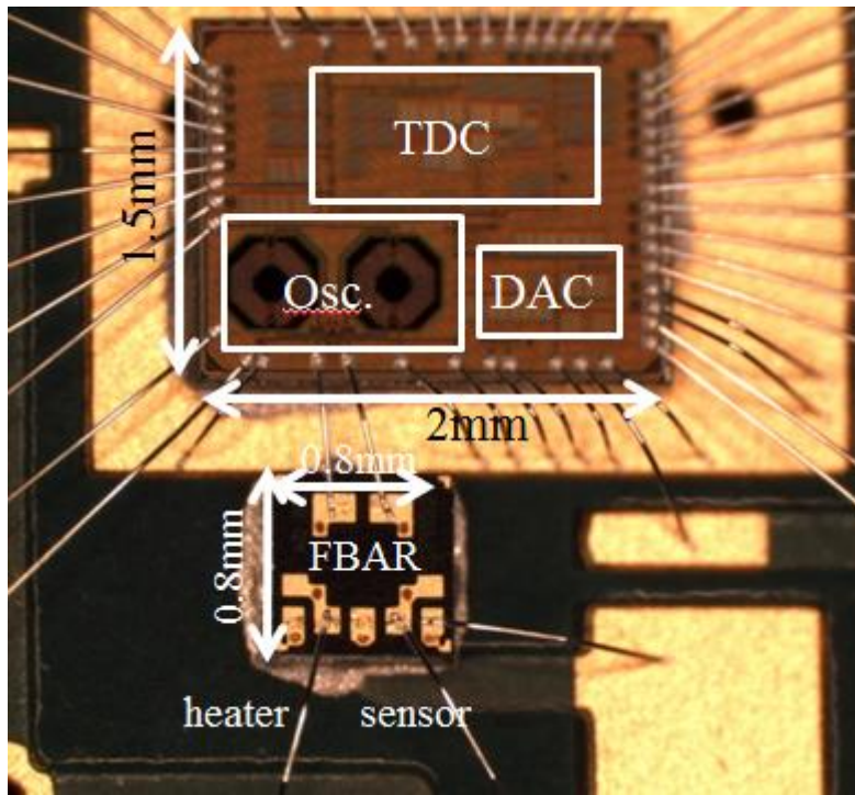
Figure 4.34 Die photo of the oven controlled temperature compensation system with FBAR.
