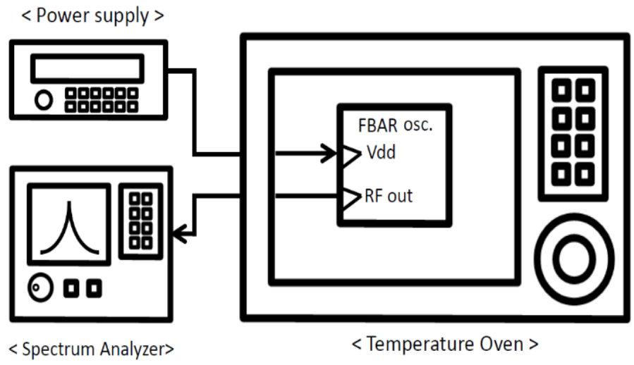
Figure 4.4 Block diagram for test bench
