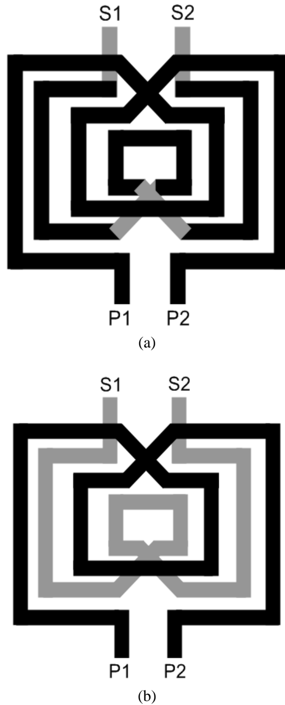
Figure 3.16 (a) Planar and (b) stacked transformer structure
