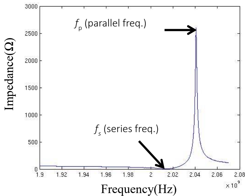
Figure 2.4 Impedance characteristic of FBAR over frequency
