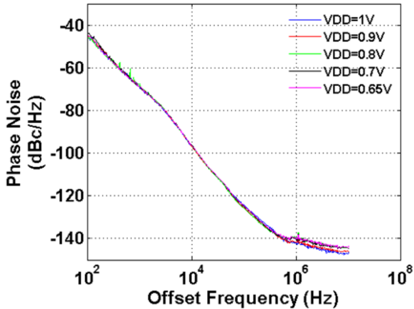
Figure 3.26 Phase noise plot with V_{DD} change
