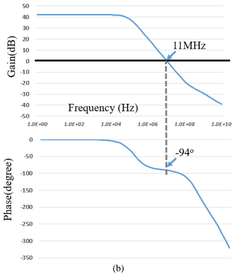
Figure 4.29 (a) Block diagram of opamp (OP1) used at DAC and (b) its gain with phase margin
