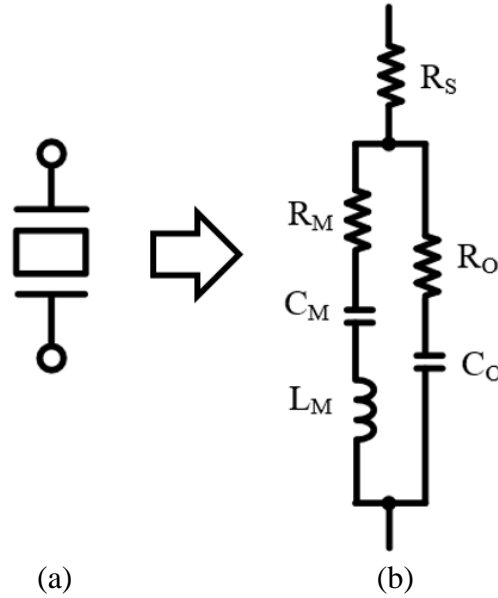
Figure 2.6 (a) Circuit symbol and (b) MBVD equivalent circuit of AlN CMR
