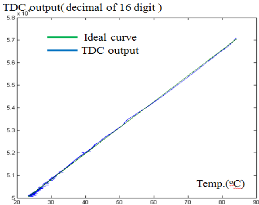
Figure 4.17 Best TDC linearity with 980mV V_{DD} .
