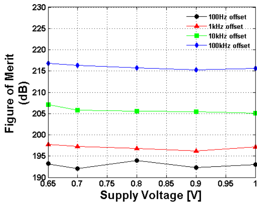
Figure 3.28 Figure of merit plot according to V_{DD} change
