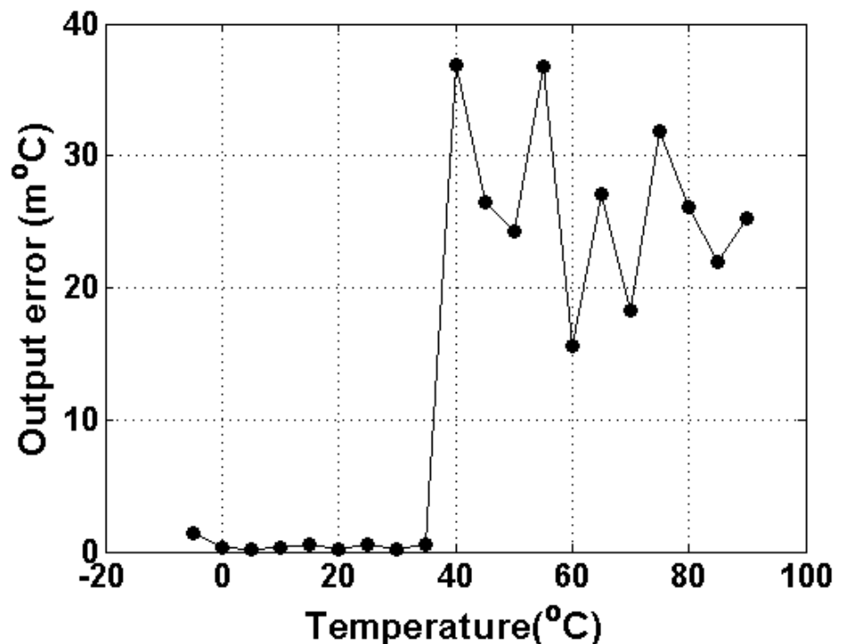
Figure 4.24 TDC output error
