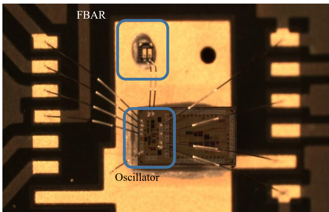
Figure 3.7 Die photo of Zigbee receiver with FBAR
