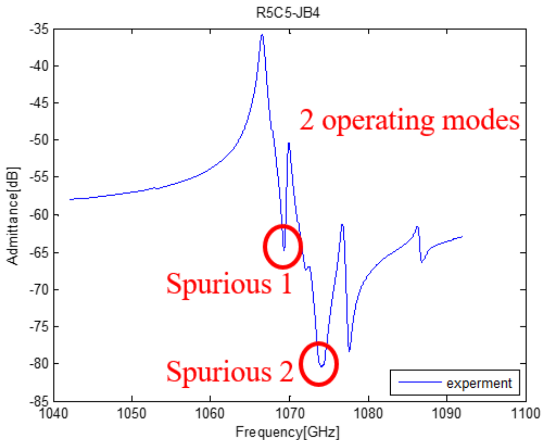
Figure 3.11 Admittance of AIN CMR according to frequency change.
