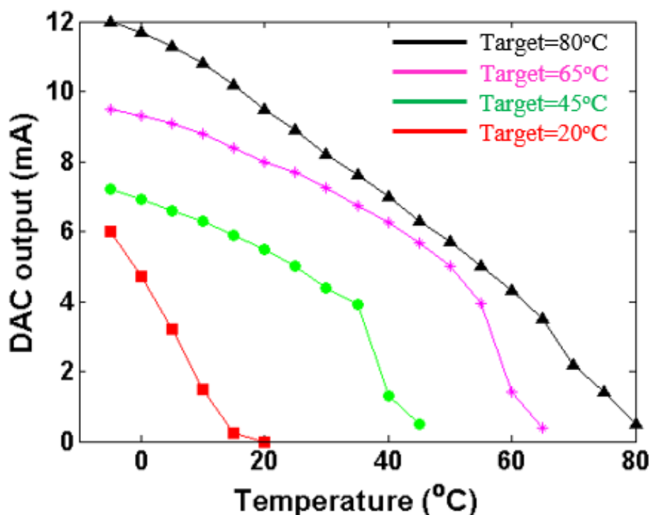
Figure 4.37 Output current variation of the DAC over temperature change with various target setting.
