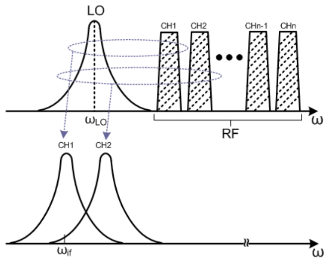
b) Down converted channel with noisy LO
