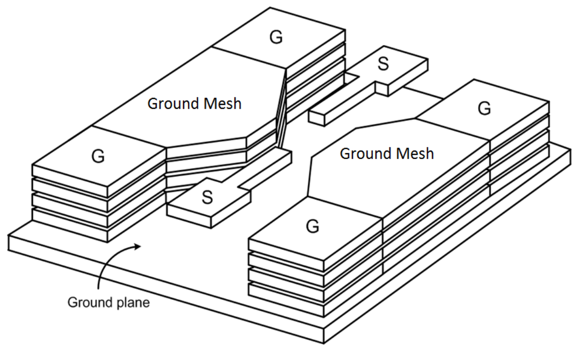
Figure 3.19 Test structure for extracting parasitic components from ground plane and test Pads.
