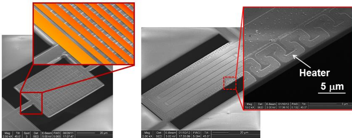
Figure 4.7 SEM photo for sensor and heater for AlN CMR
