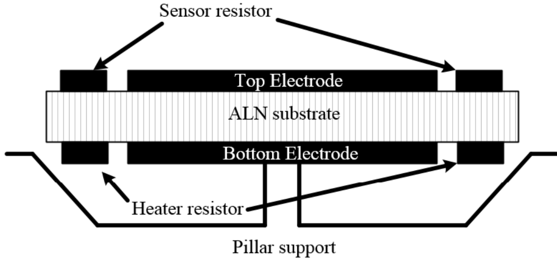
Figure 4.6 Block diagram of the FBAR with sensor and heater
