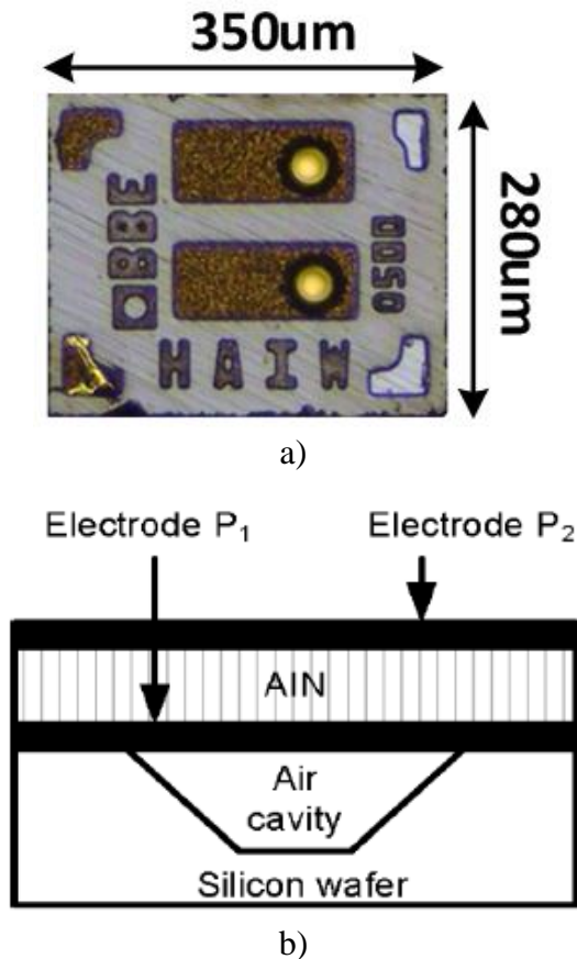
Figure 2.3 (a) Die photo of FBAR and (b) cross section view
