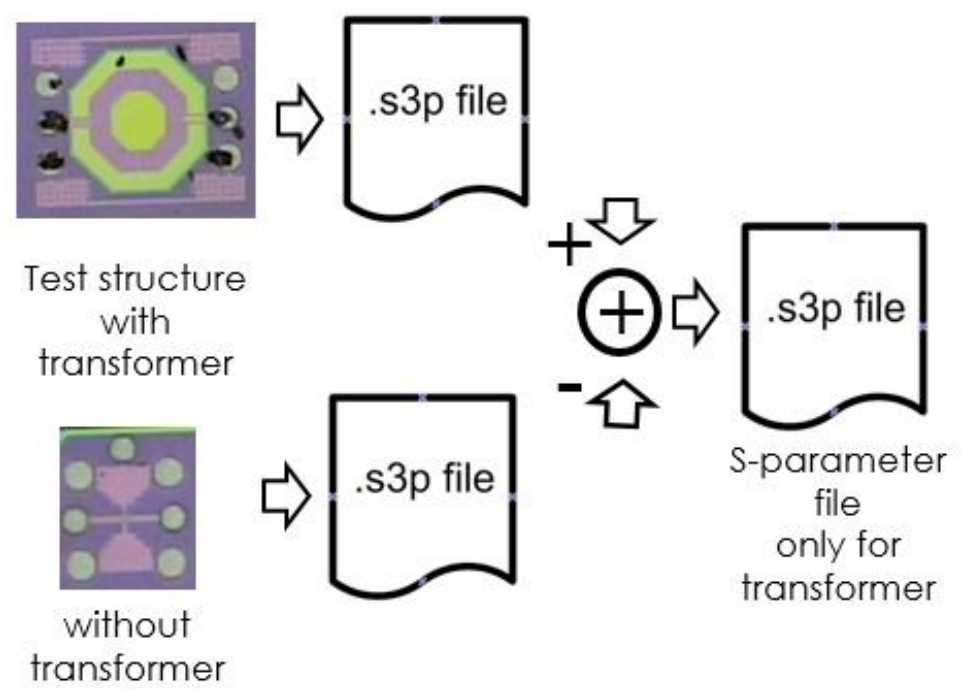
Figure 3.20 De-embedding process to extract transformer characteristic
