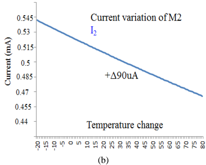
Figure 4.3 the current variation of (a) M1 and (b) M2 under the temperature change.
