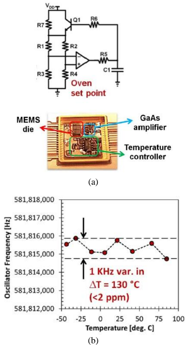
Figure 4.11 (a) Wheat stone bridge based temperature compensation system and (b) test result
