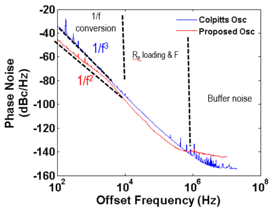
Figure 3.25 Measured phase noise performance with Colpitts oscillator
