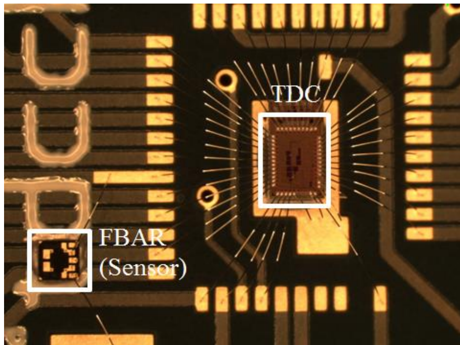
Figure 4.14 Die photo showing connection between FBAR sensor and TDC chip
