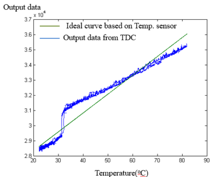
Figure 4.16 TDC output according to temperature with RTD
