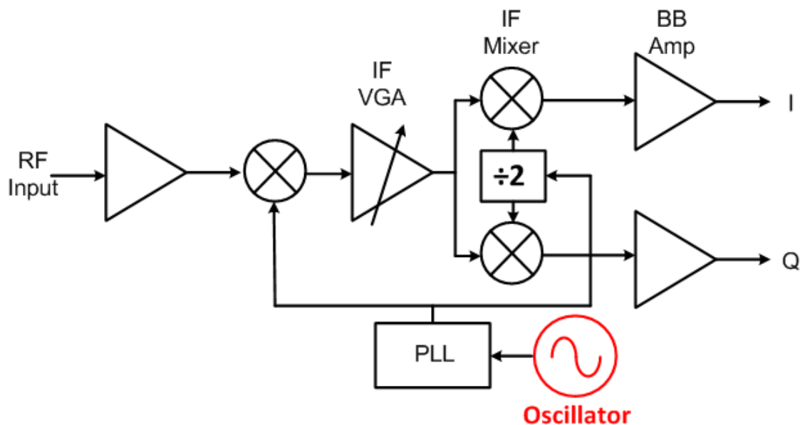
Figure 1.3 Block diagram of the 60GHz receiver with Frac-N PLL
