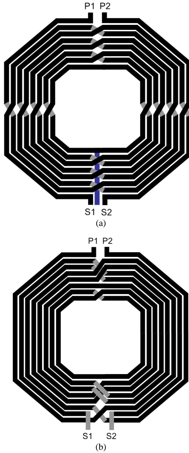
Figure 3.17 Transformer layout for (a) 2GHz BLE application and (b) 1GHz AlN CMR device
