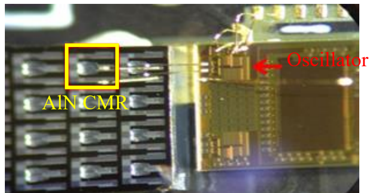
Figure 3.8 Die photo of Colpitts oscillator using AlN CMR
