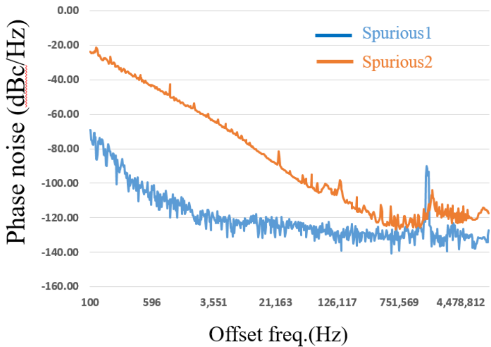
Figure 3.12 Two phase noise performances at different modes
