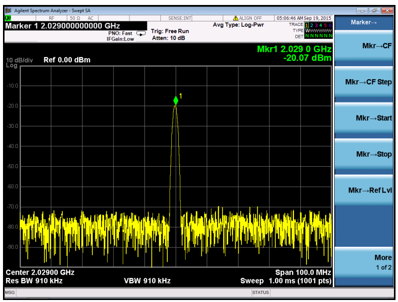
Figure 3.24 Test result from frequency spectrum analyzer
