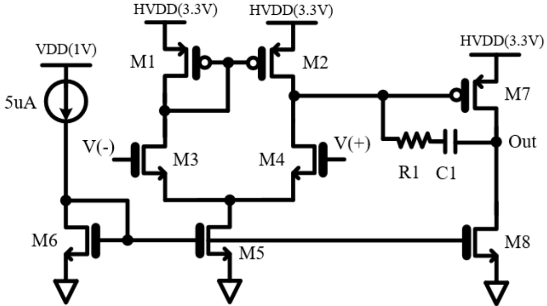
Block diagram of OP2
