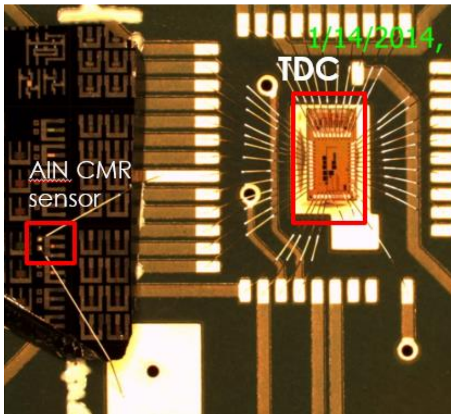
Figure 4.19 Die photo of TDC connected to AIN CMR sensor
