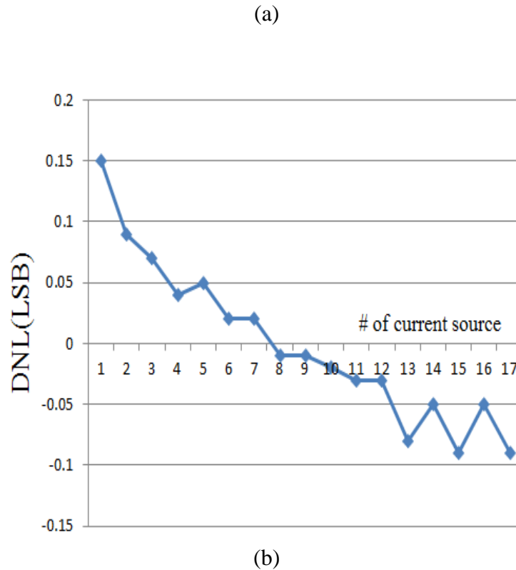
Figure 4.27 (a) INL and (b) DNL error of 1 st prototype current steering DAC
