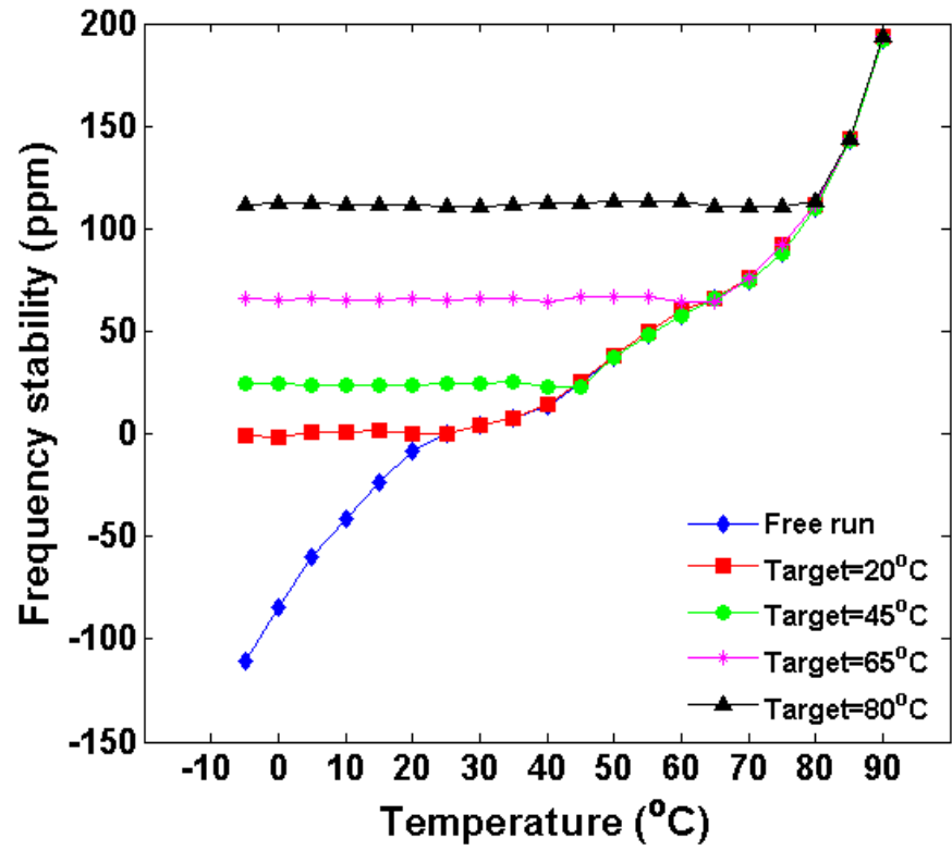
Figure 4.35 Frequency drift of the oscillator over the temperature change with system on and off
