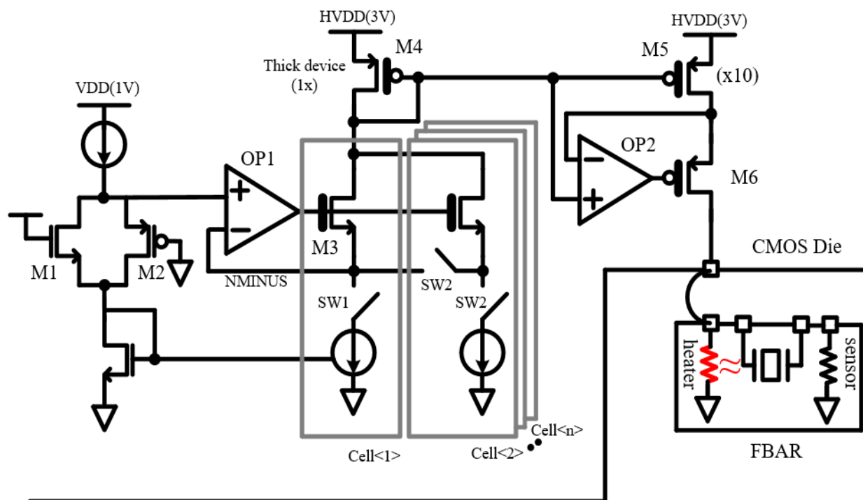
Figure 4.28 2 nd prototype for current steering DAC
