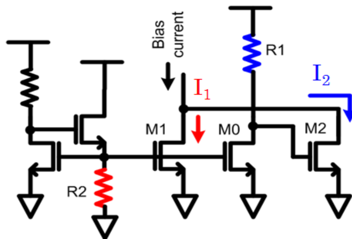
Figure 4.2 Temperature compensated current source
