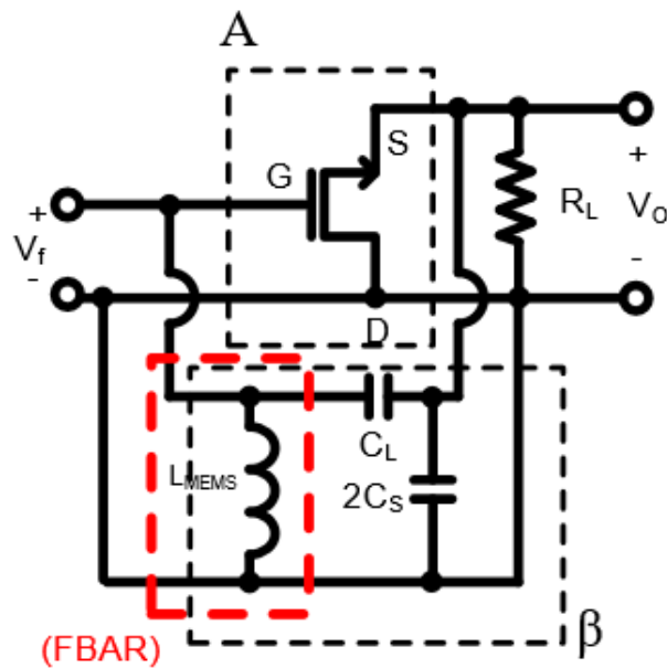
Figure 3.3 AC equivalent block diagram of the single-ended colpitts oscillator
