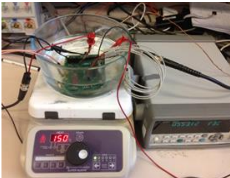
Figure 4.15 Test set up for TDC with oil tank and heat plate
