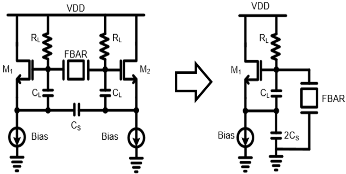
Figure 3.2. Block diagram of the differential colpitts oscillator and its equivalent single-ended structure
