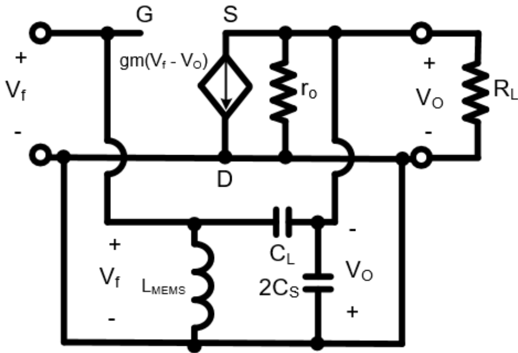
Figure 3.4 Small-signal model of the single-ended Colpitts oscillator
