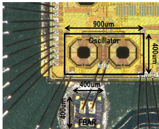
Figure 3.23 Die photo of the transformer coupled Colpitts oscillator with 2GHz FBAR
