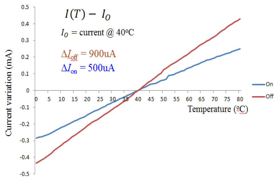
Figure 4.5 Test result with temperature compensated bias circuit.
