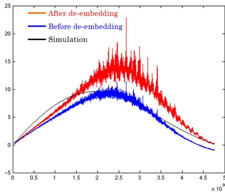
Figure 3.22 Quality factor (Q) of primary inductor
