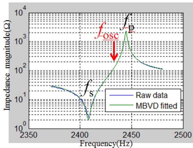
Figure 4.8 Impedance plot of a FBAR according to frequency
