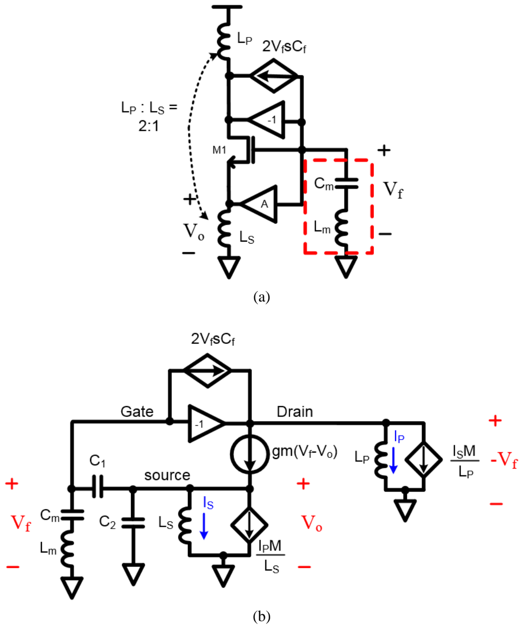
Figure 3.15 (a) Single-ended block diagram of transformer coupled oscillator and (b) its small signal model
