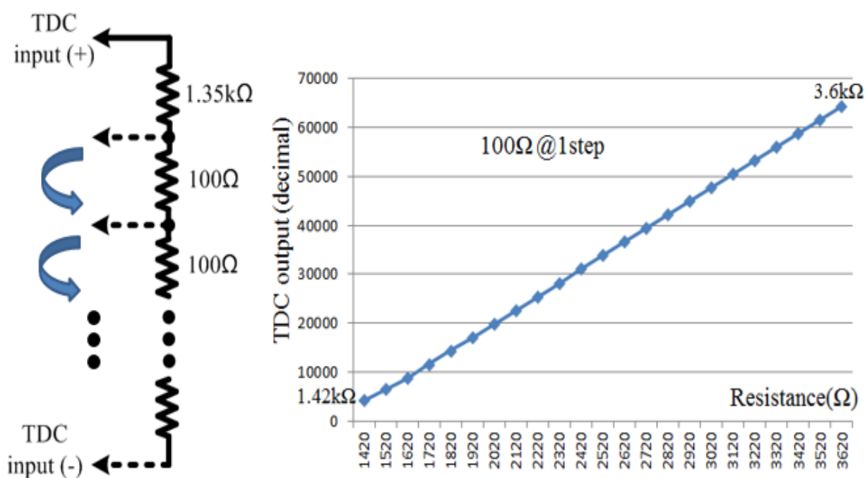
Figure 4.23 Test result for detection range of TDC
