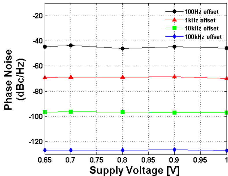
Figure 3.27 Phase noise at close-in offset frequency with variable V_{DD}
