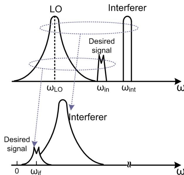
Figure 1.1. Signal down conversion with a noisy LO
