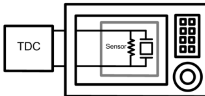
Figure 4.21 Test set up with sensor inside chamber
