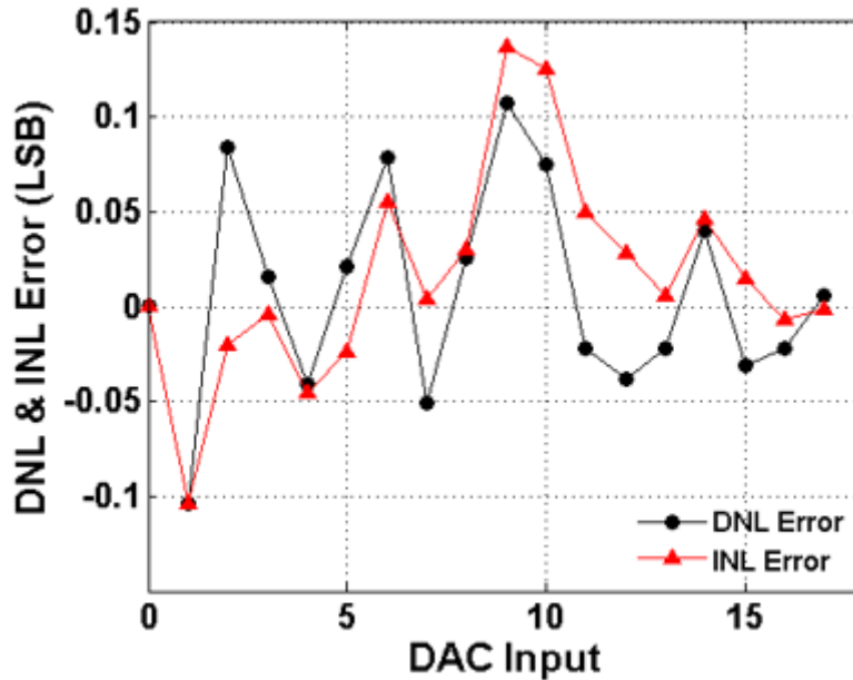
Figure 4.32 INL and DNL of the current steering DAC
