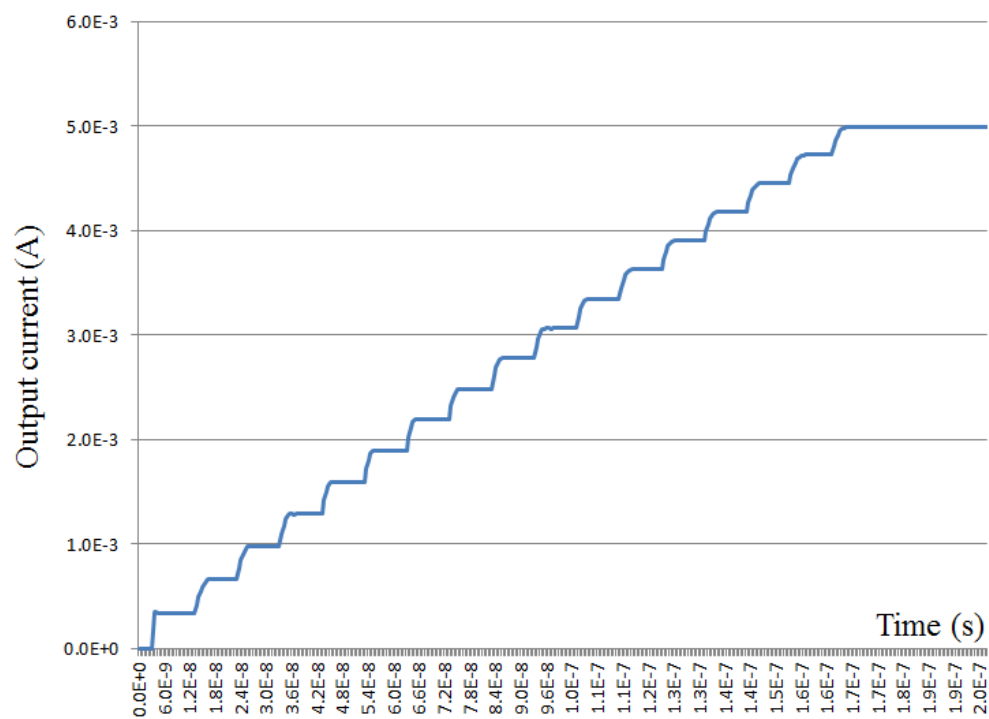
Figure 4.26 Simulation result with 20Mbps input data rate
