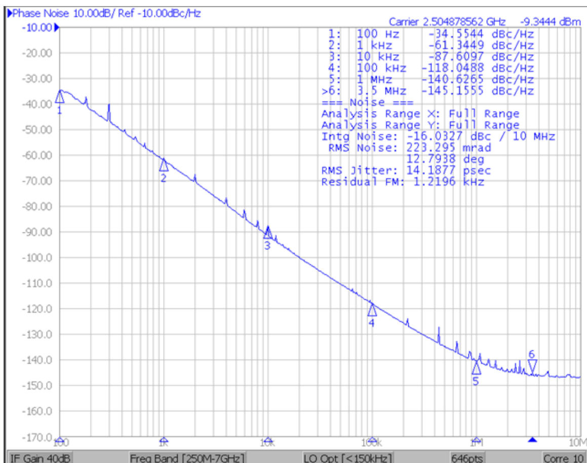
Figure 3.6 Measured phase noise of the Colpitts oscillator using FBAR
