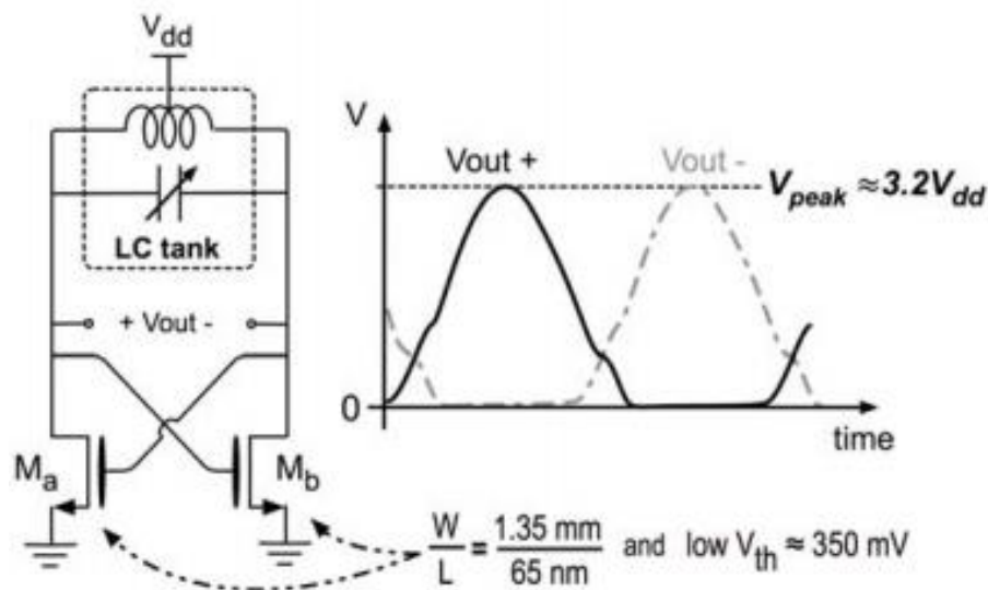
Figure 3.1 CMOS Class-D VCO
