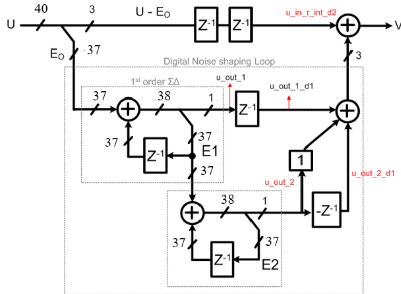
Figure 4.33 Block diagram of the 2 nd order MASH type sigma delta modulator
