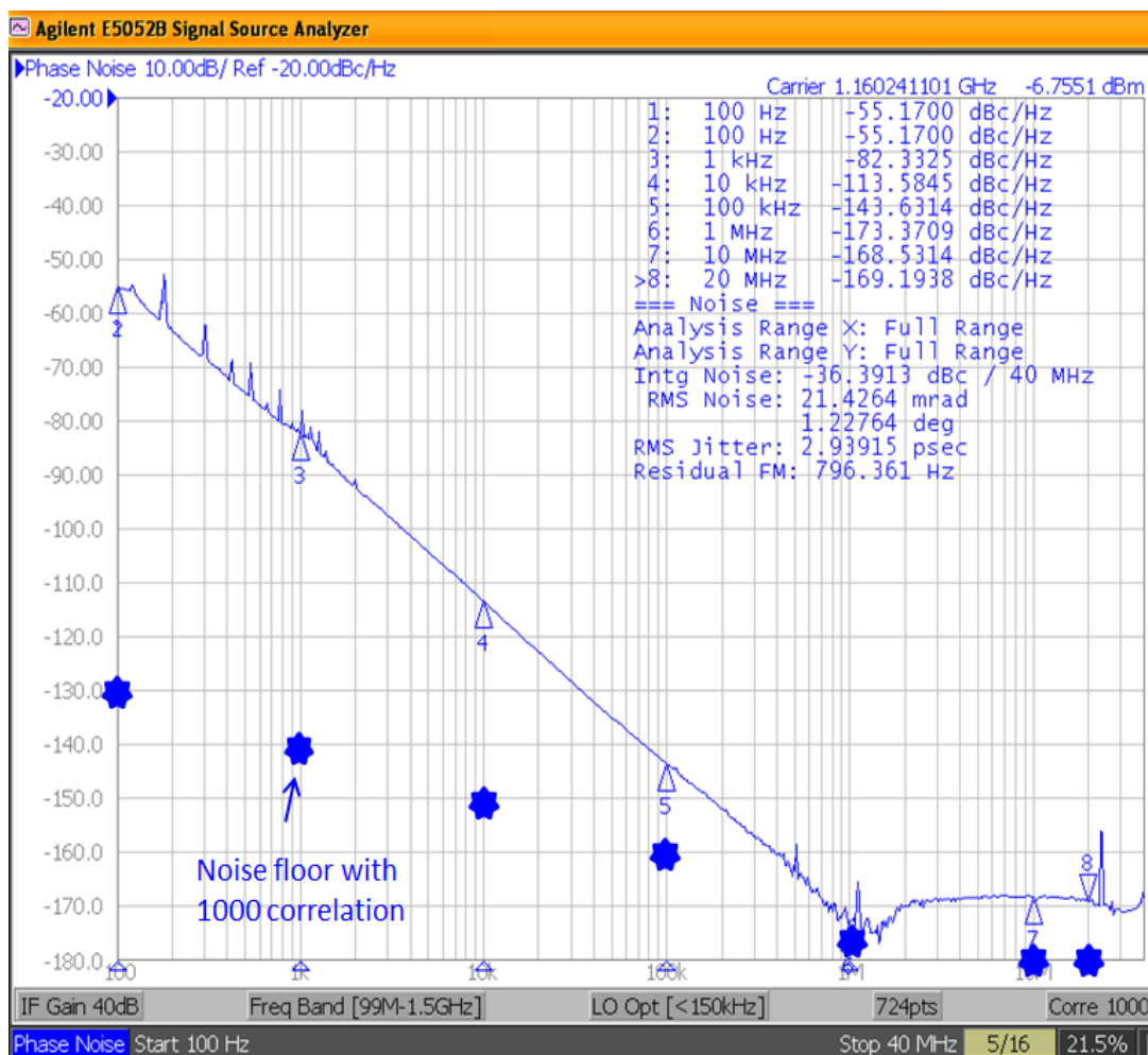
Figure 3.9 Measured Phase noise of AIN CMR with noise floor of test equipment
