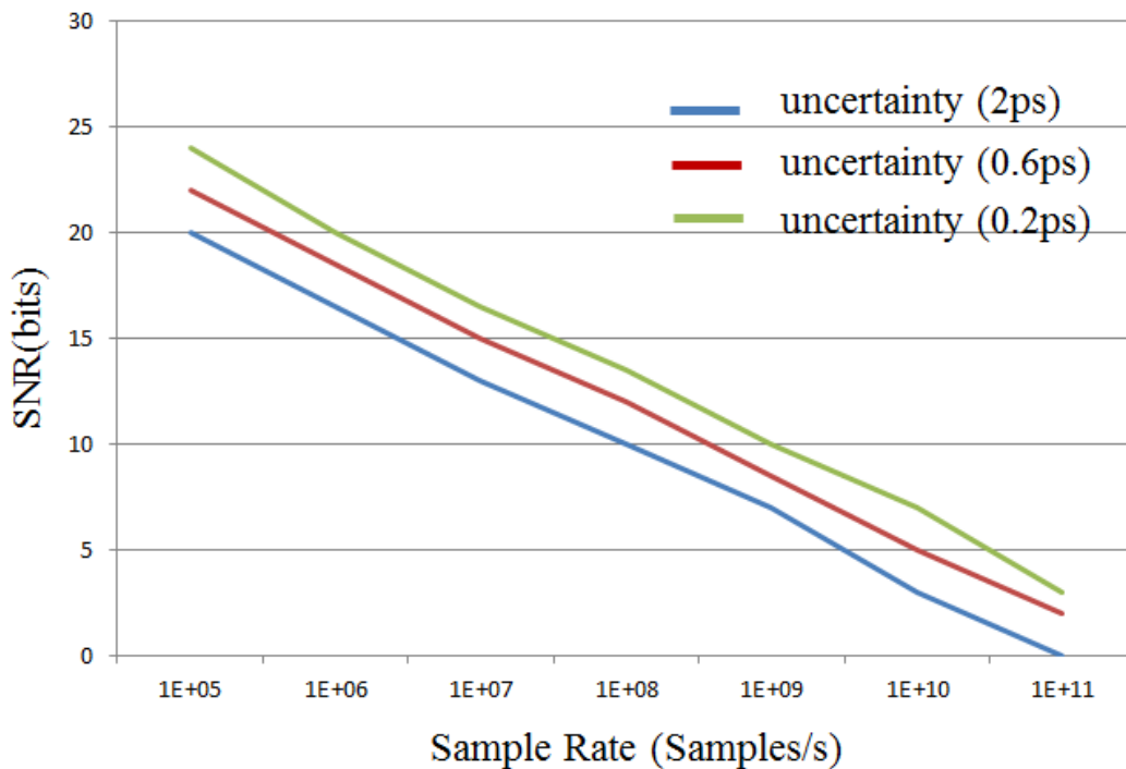
Figure 1.4 Signal-to-Noise ratio performance limitation due to aperture uncertainty
