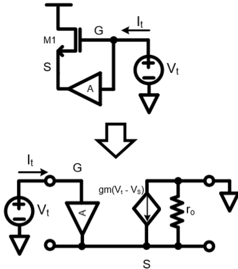
Figure 3.5 Small signal model with test voltage.
