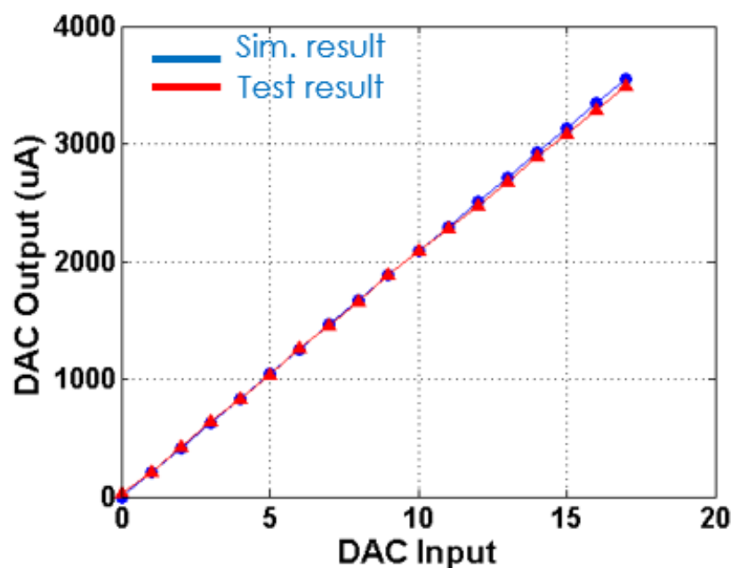
Figure 4.31 Test result of the current steering DAC
