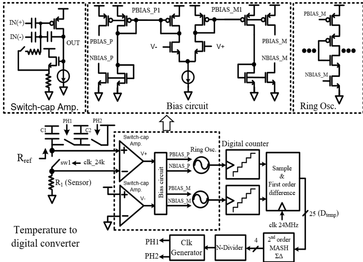
Figure 4.13 Block diagram of temperature to digital converter
