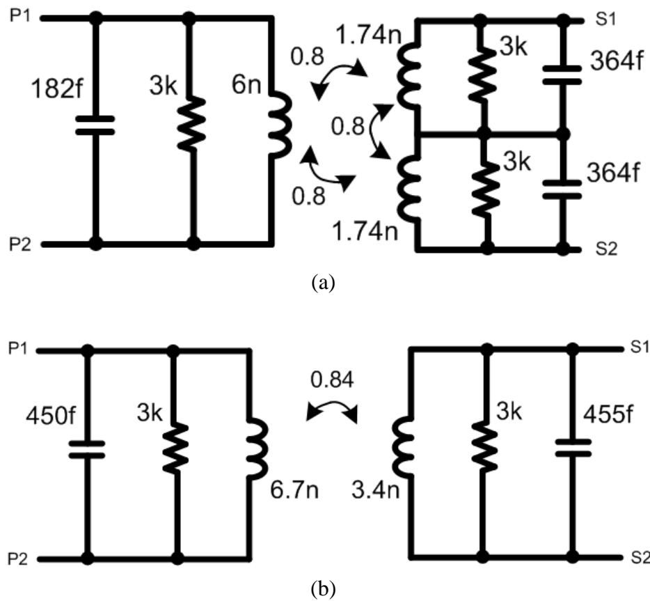
Figure 3.18 Electrical model of the transformer for (a) BLE application and (b) AIN CMR
