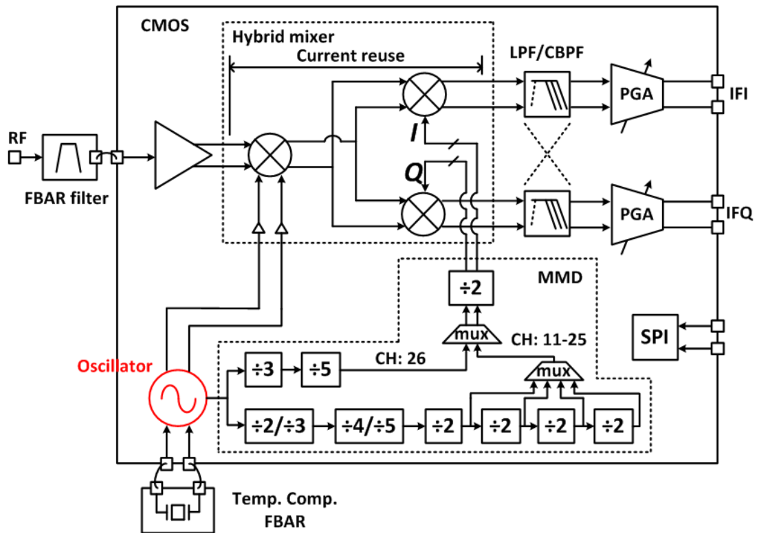
a) Receiver for Zigbee application
