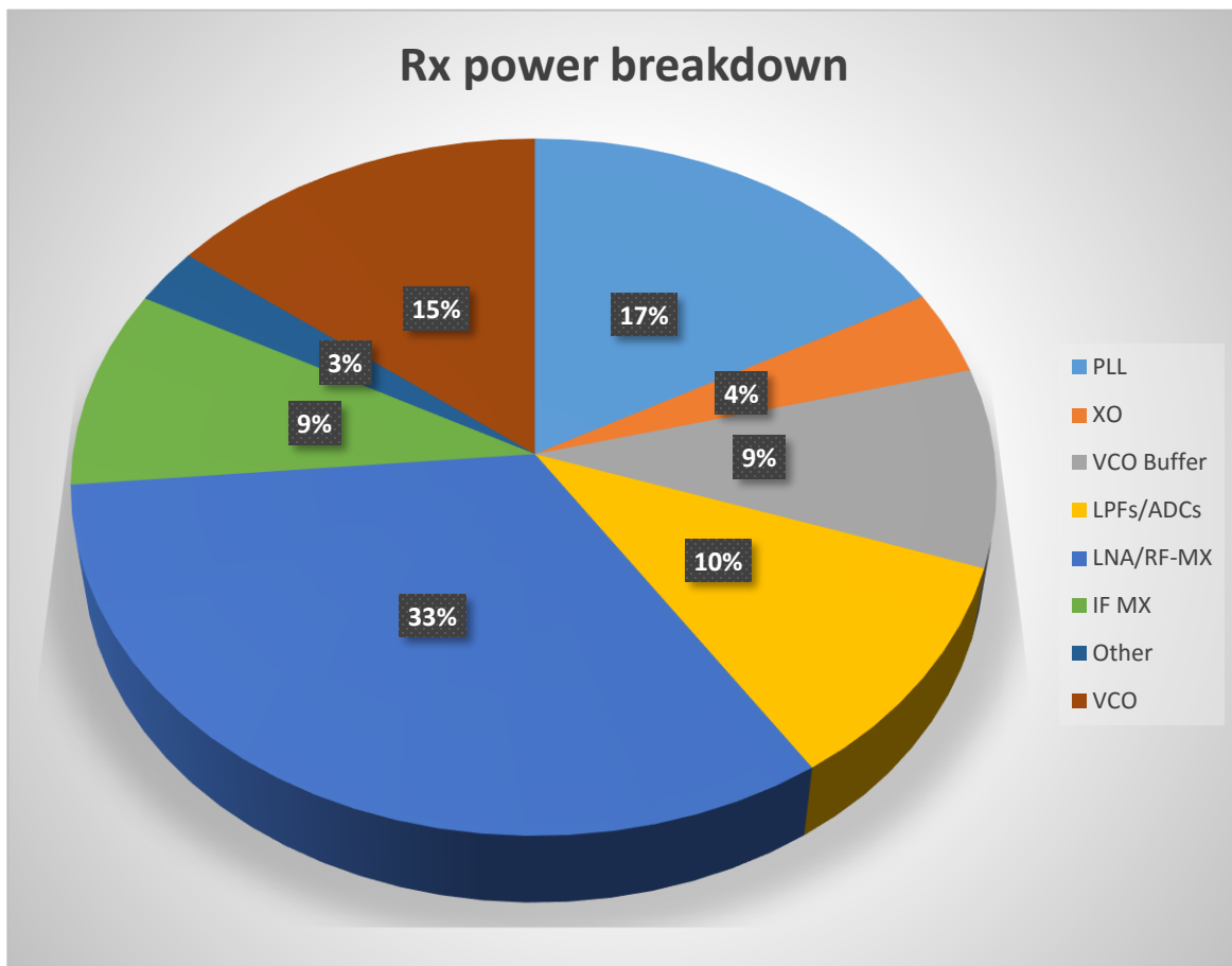
Figure 2.2 The measured Bluetooth low energy receiver power breakdown [13]
