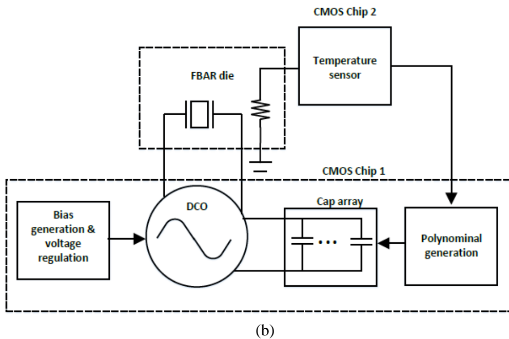
Figure 4.9 (a) frequency variation of the FBAR based oscillator without temperature compensation and (b) block diagram of the temperature compensation system
