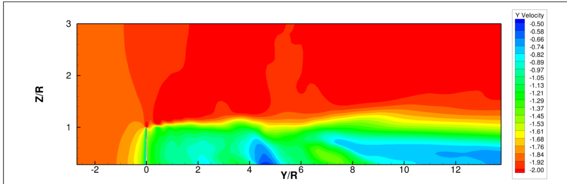
Figure 2.21: Streamwise velocity contours, not fully converged, in the turbulent wake simulated in NNMREC.
