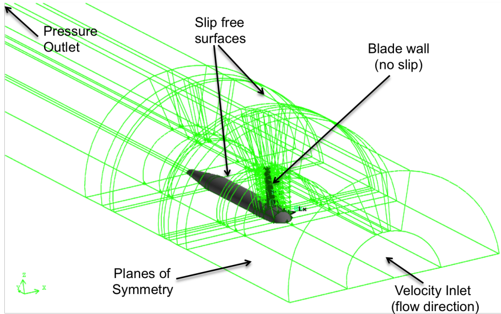
Figure 2.3: Computational domain and boundary conditions used with the SRF model. The actual geometry of the scaled HAHT blade (gray region) is included in this computational domain.
