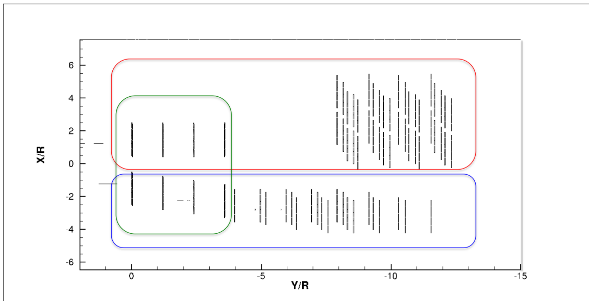
Figure 3.14: Top view of the computational domain for investigating the effect of the dominant spacing variables in different turbine array configurations.
