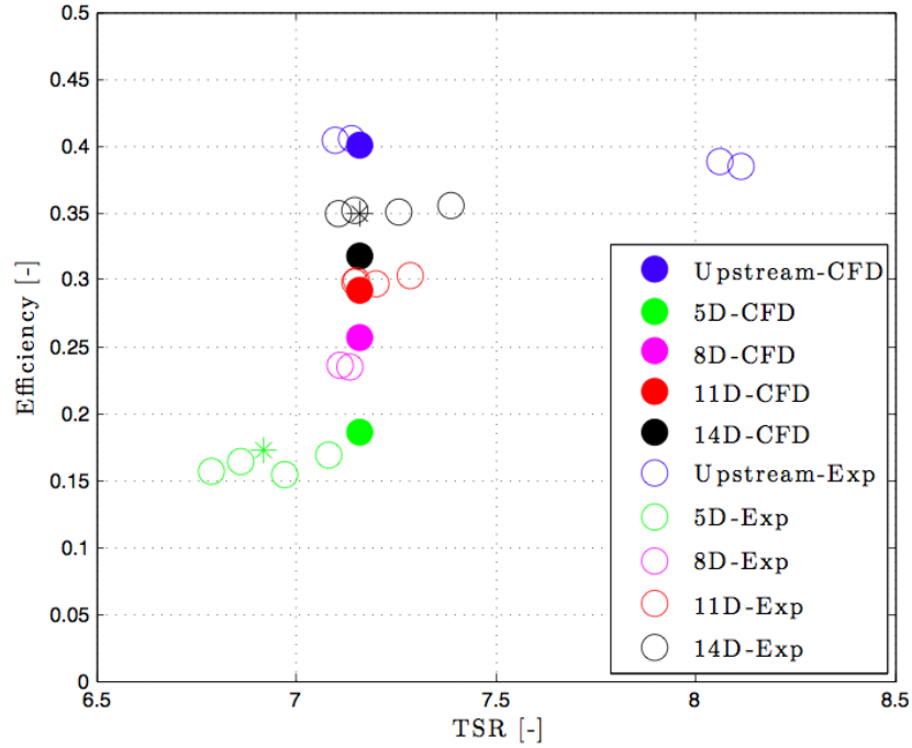
Figure 3.7: CFD versus experimental results for arrays of two coaxial turbines with correction for 5D and 14D turbines.
