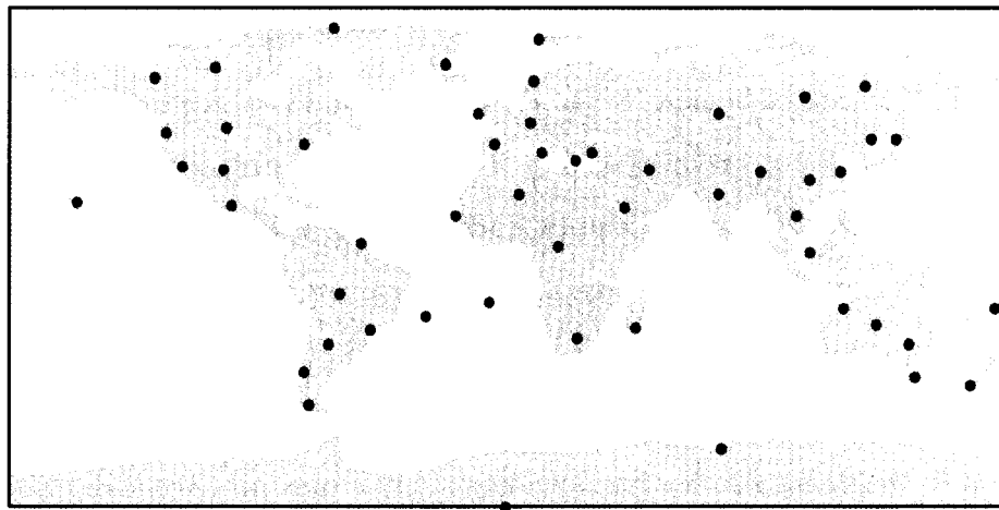
Figure 1.1: Locations of 53 weather balloon release sites used in the present analysis. Sites were chosen for their broad spatial distribution and based on availability of data. Map courtesy of L. M. McCoy.
