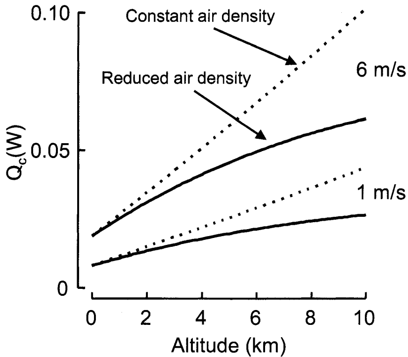
Figure 1.3: Instantaneous convective heat loss across altitude for an idealized insect (approximated by a cylinder) at two wind speeds assuming an initial body temperature of 40°C, a sea level air temperature of 25°C and a 6°C/km decrease in air temperature with altitude. See text for equations and details. Solid lines represent the estimate of true convective heat loss taking into account the empirical decrease in air density with altitude; dotted lines indicate convective heat loss predicted for a constant-density atmosphere.
