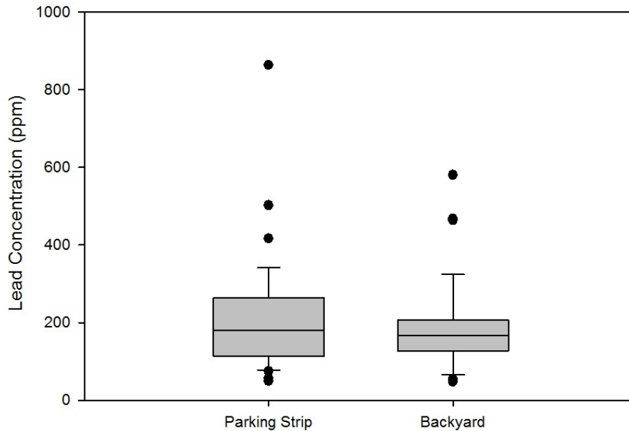
Figure 14: Comparison of parking strip soil to backyard soil for lead concentrations.
