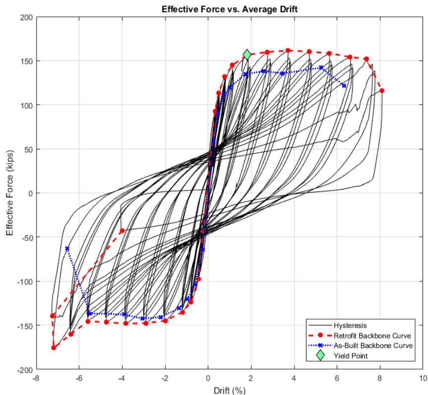
Figure 7-28. Effective force vs. average drift
