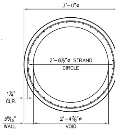
TYPICAL SECTION
