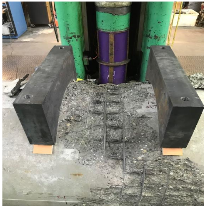
Figure 4-2. Concrete crushing and buckled strands
