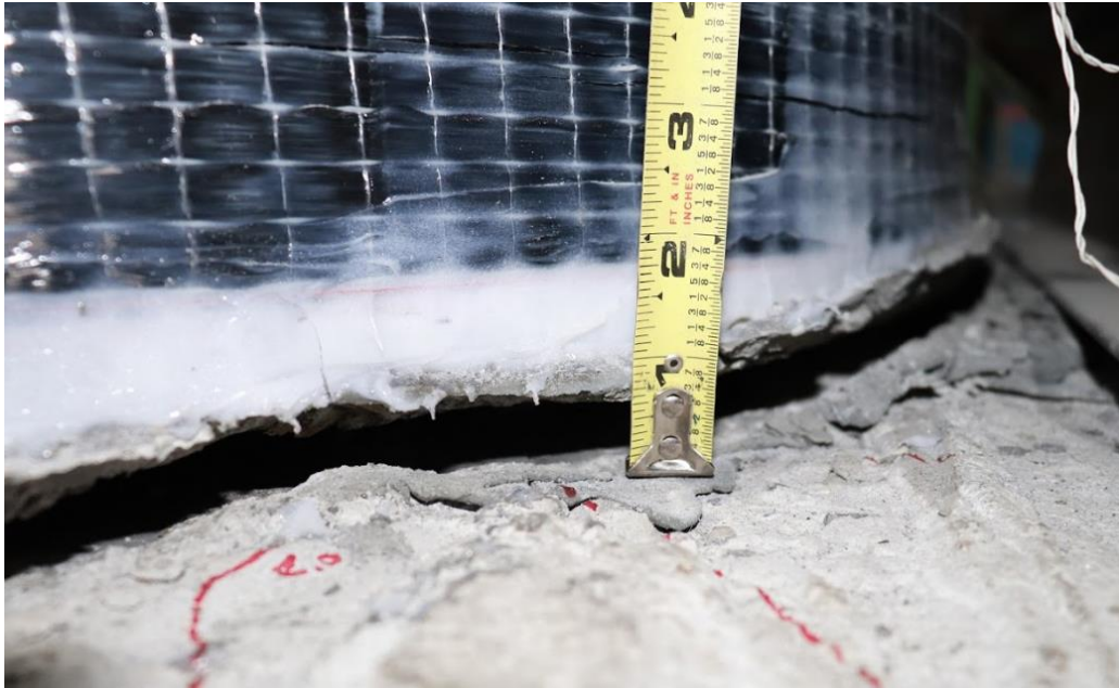
Figure 7-7. Uplift on Cycle 3 of Series 7 (+3.71%, -4.54% drift)
