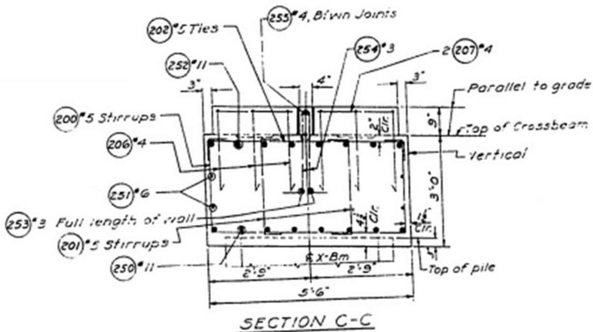
Figure A-12. Cap beam cross-section for typical bent (Slide)
