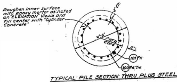
Figure A-10. Details of inner plug reinforcement (Slide)
