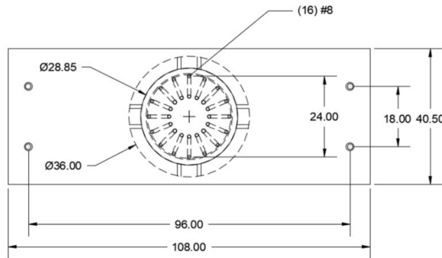
Figure 6-4. Plug dimensions and reinforcement
