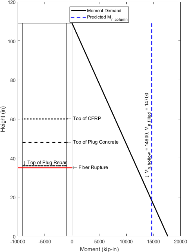
Figure 8-8. Conditions at maximum moment
