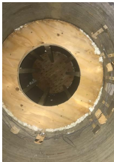
Figure 3-14. Solid disc connected to two plywood rings by 2x4 studs inside Four-point bending specimen
