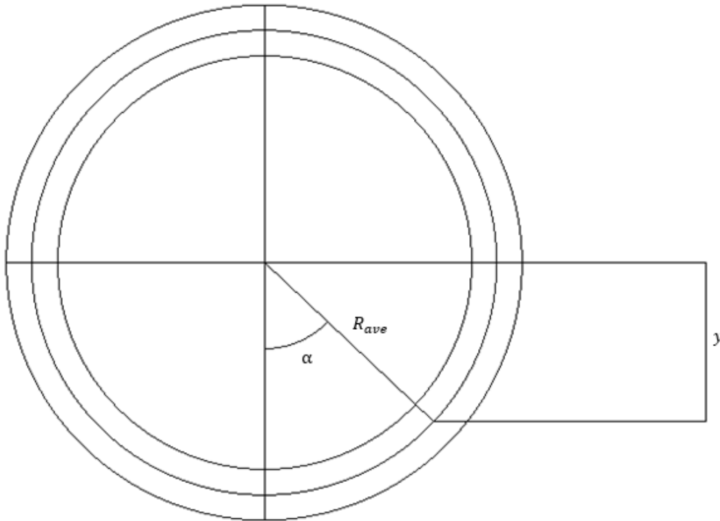
Figure 5-7. Cross-section of test specimen used for transverse load capacity calculations
