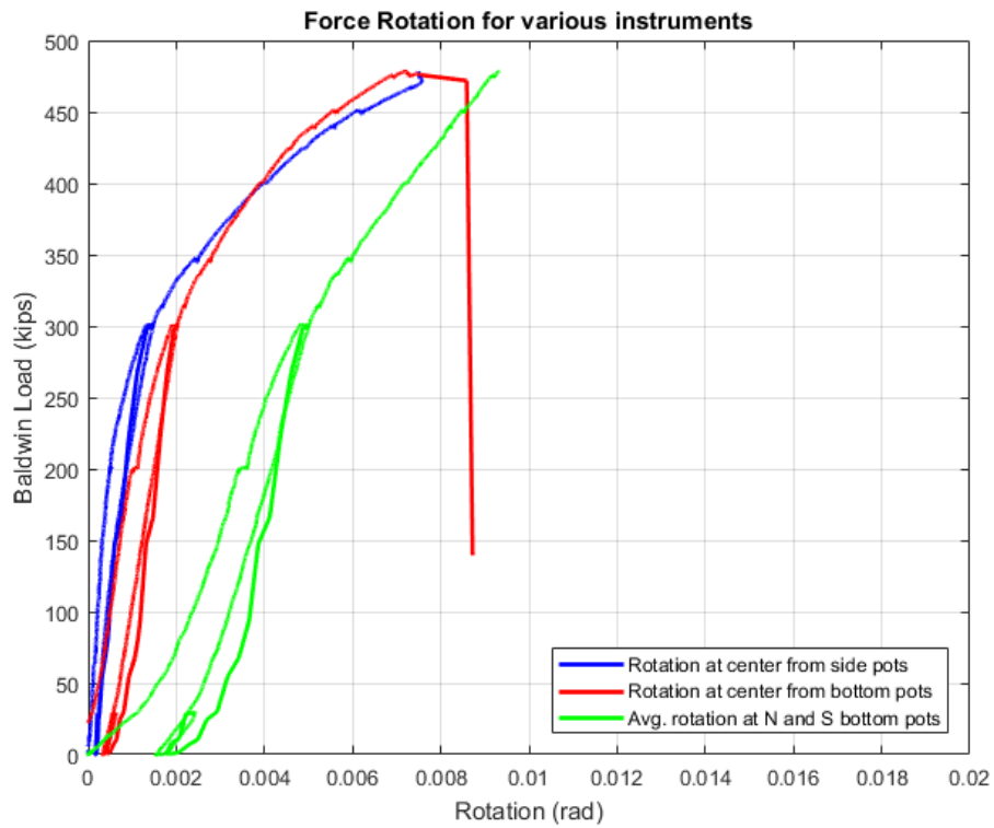
Figure 5-5. Force-rotation curves for all potentiometers
