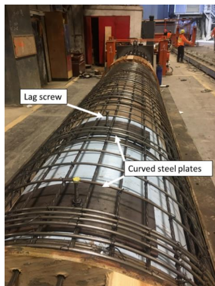
Figure 3-11. Hold-down plates used for sonotube during casting
