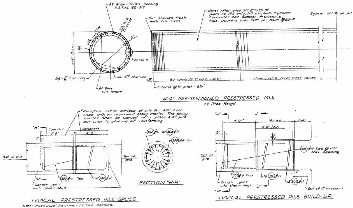
Figure 1-4. Typical details for pretensioned pile-column
