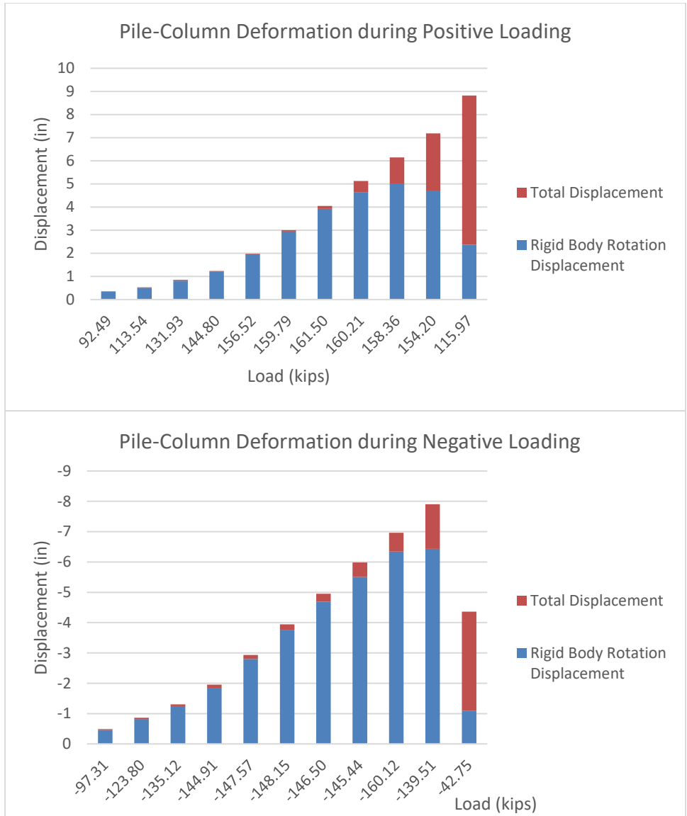
Figure 7-29. Difference between total displacement and rigid body displacement
