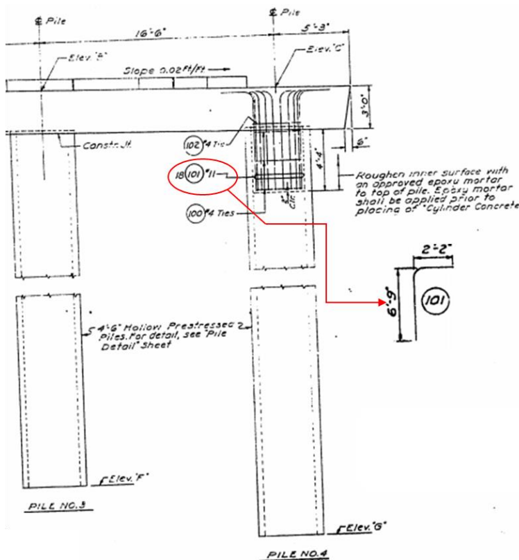
Figure 6-5. Plug reinforcement details for Le Line Slide Bridge
