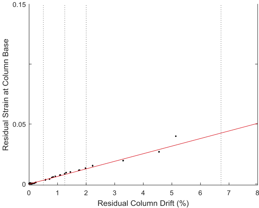
Figure 4.11 Residual strain vs. residual drift for Bridge 11Ar with ground motion in the transverse direction
