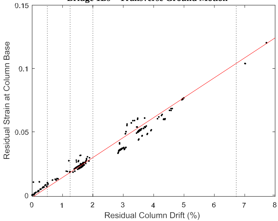
Bridge 1Bs – Transverse Ground Motion
