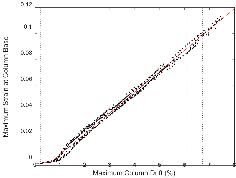
Bridge 1Br – Longitudinal Ground Motion
