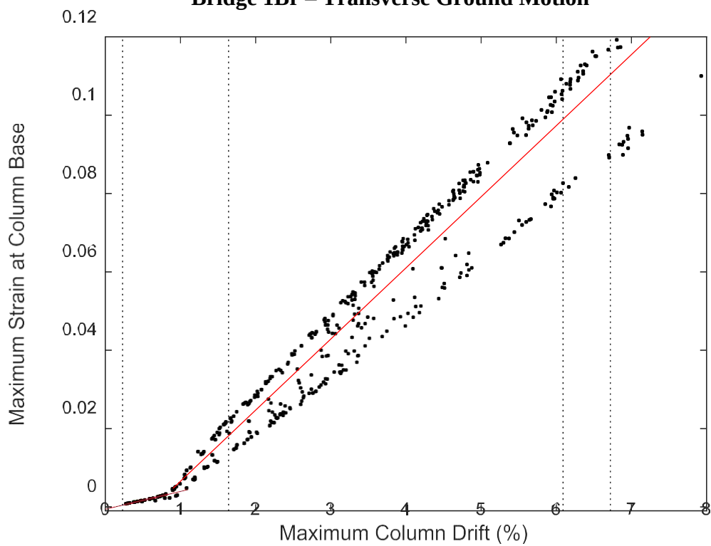
Bridge 1Br – Transverse Ground Motion
