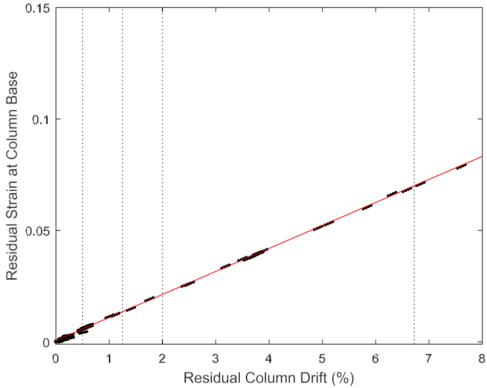
Bridge 11Bs – Transverse Ground Motion
