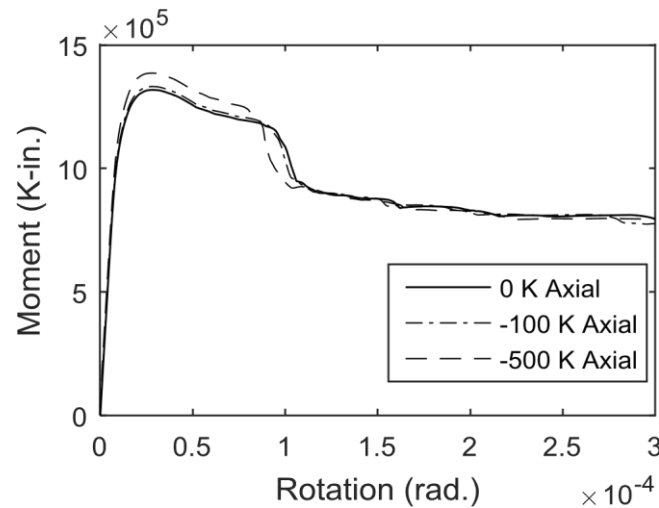
Figure 3.6 Moment-rotation behavior of the deck section
