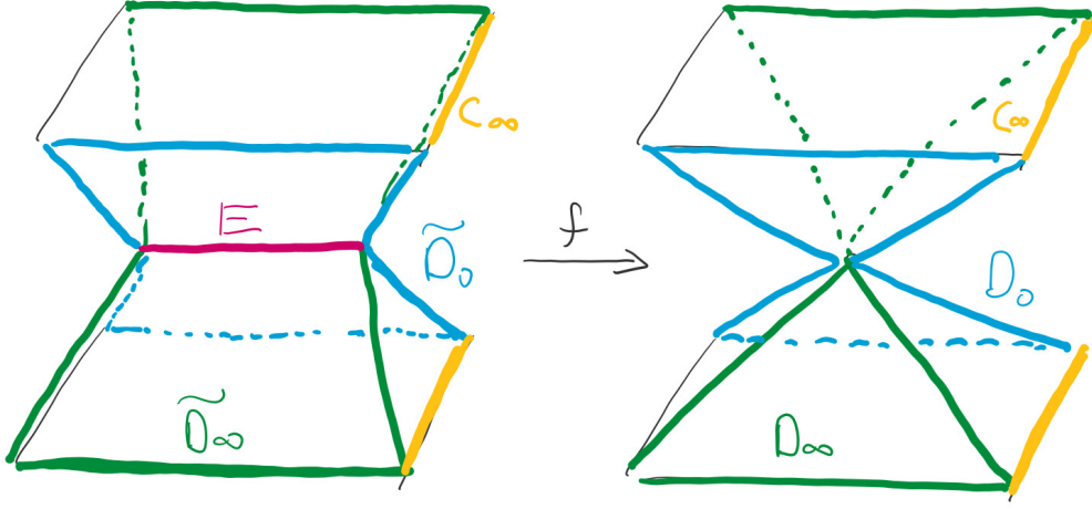
Figure 1.2: The small resolution of Example 1.4.2
