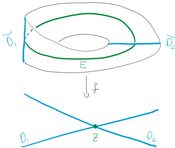
Figure 1.1: The blowup appearing in Example 1.4.1
