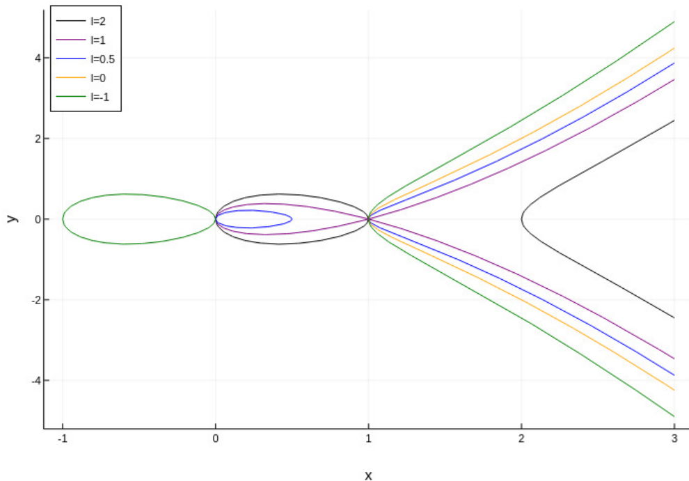
Figure 3.2: The “ \lambda -family” of Example 3.3.26
