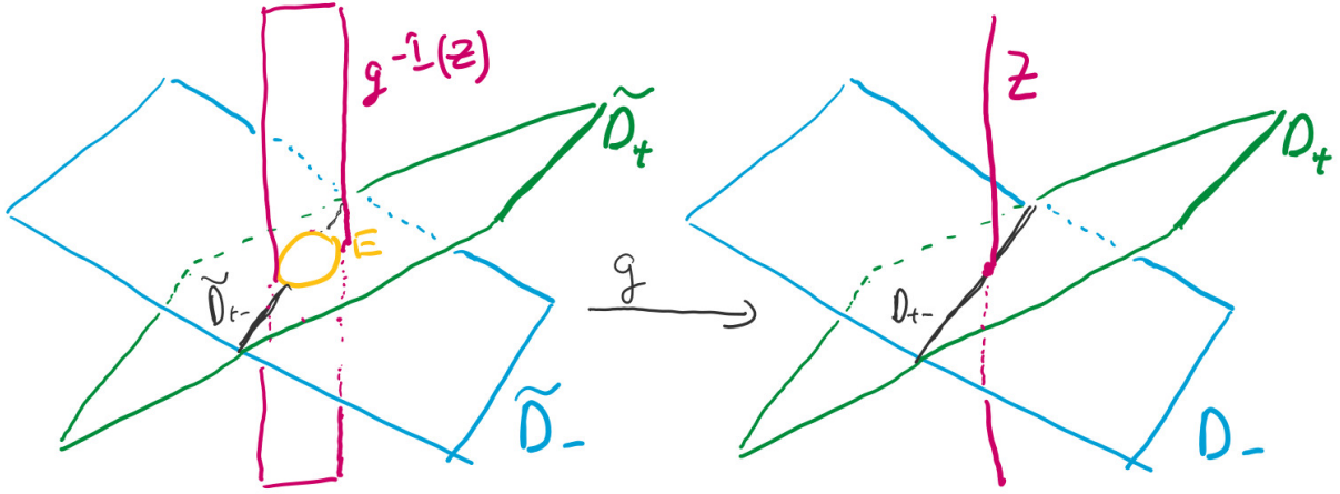
Figure 1.3: The blowup of Example 1.4.12
