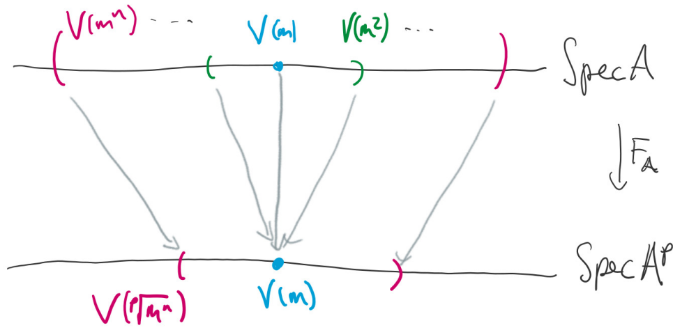
Figure 3.1: Abstract illustration of Lemma 3.3.13 — Frobenius shrinks thickenings
