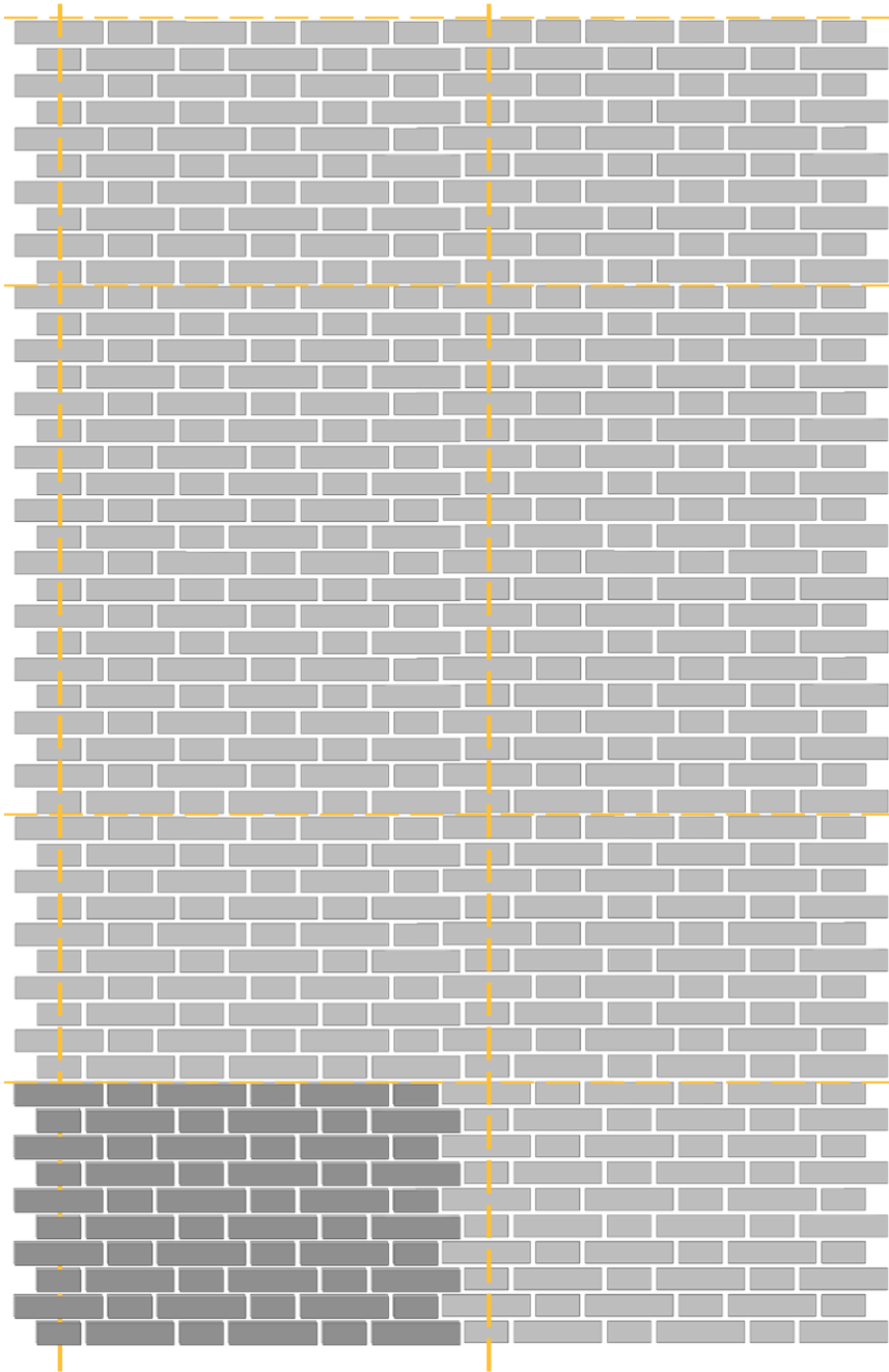
Figure 61: Brick switch pattern
