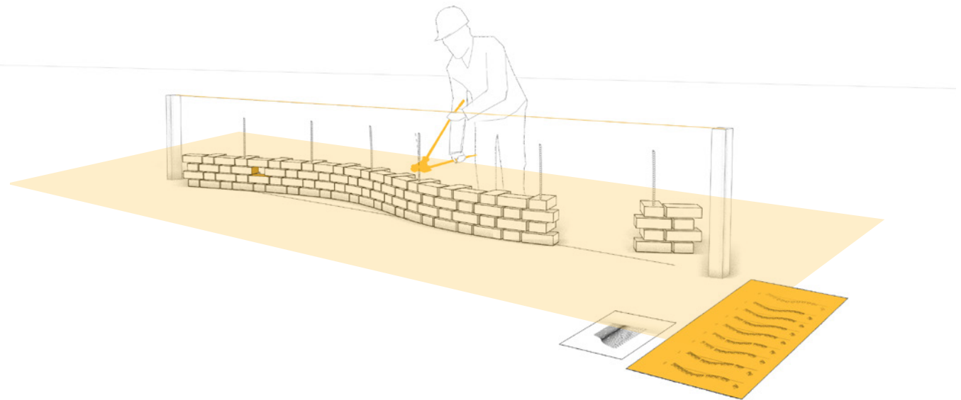
Figure 85: Construction sketch 6: bend the r-bars to match the curvature
