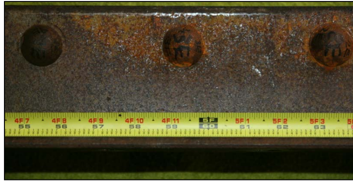
(a) East Angle Prior to Testing
