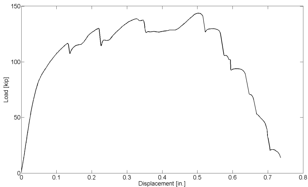
Figure 4.13 Load vs. Overall Displacement - Specimen 4R
