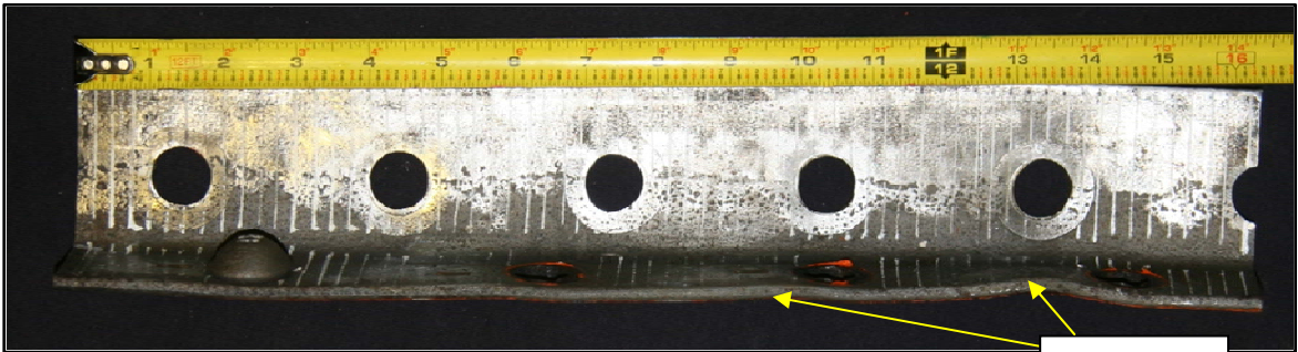
(b) After Testing
