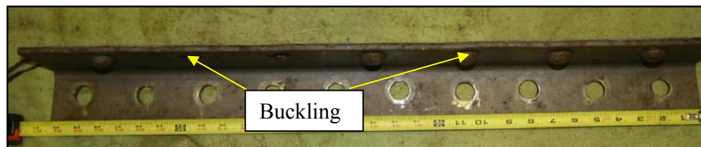
(b) After Testing
