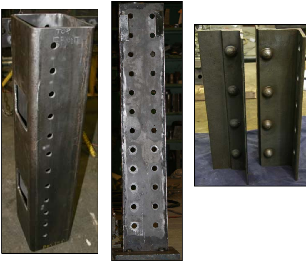
Figure 3.33 Test parts prior to assembly (a) Part 1 - HSS Tube (b) Part 3 - Middle Plate (c) Parts 4 & 5 - Guard Rail
