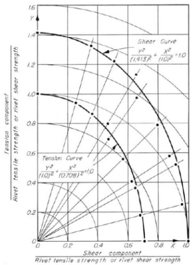
Figure 2.15 Interaction Curve for Shear-Tension Ratios Preliminary Tests (Munse & Cox, 1956)
