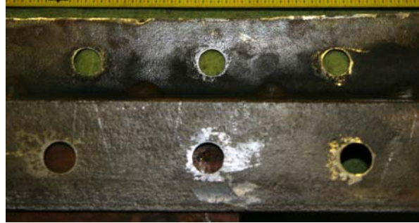
(a) West Channel Before Testing
