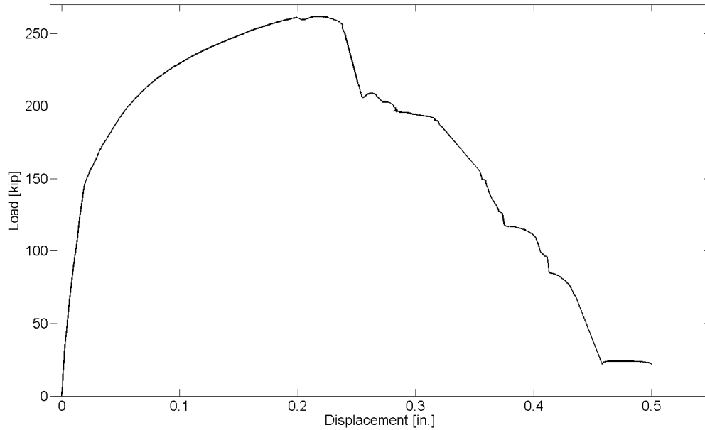
Figure 4.43 Load vs. Overall Displacement - Specimen 7R
