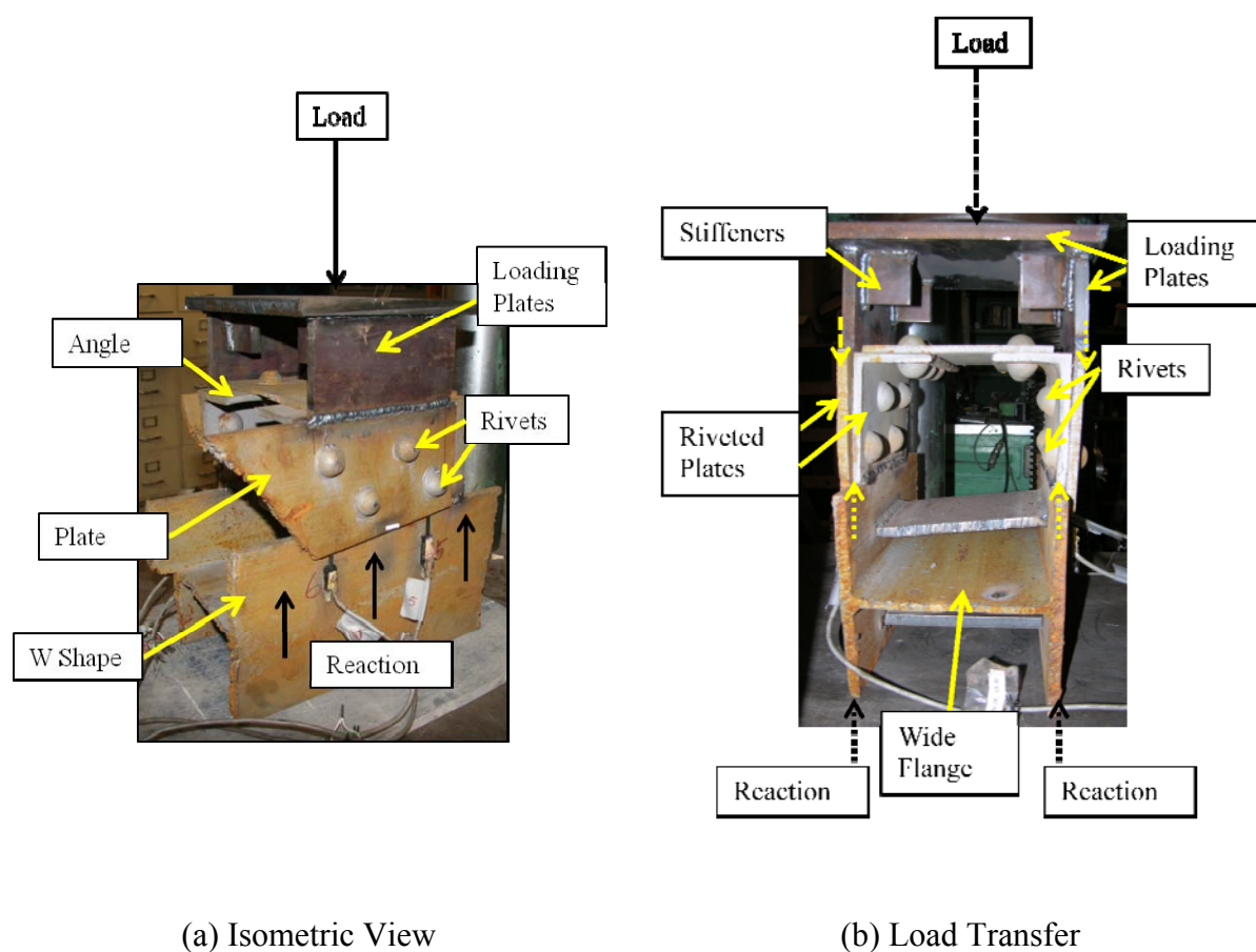
Figure 4.9 Box Test to Measure Rivet Shear Strength
