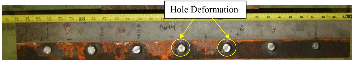
(b) East Angle After Testing
