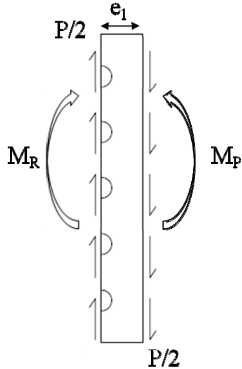
Figure 3.29 Free Body Diagram of Channel
