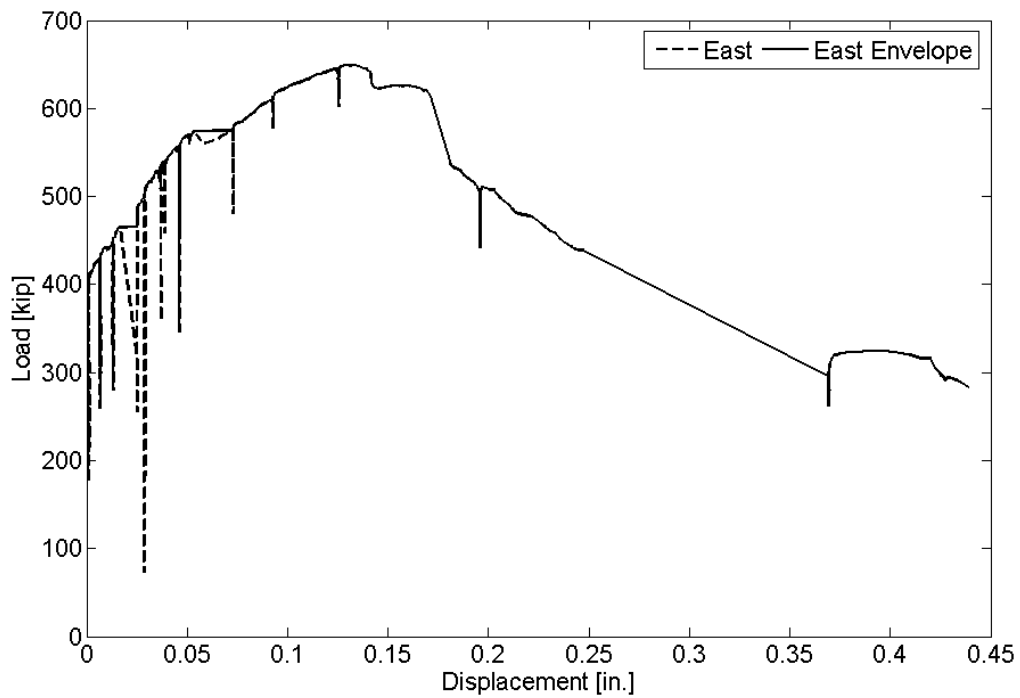
Figure E.6 Load vs. Rivet Deformation - Test 17R
