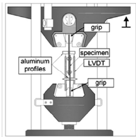
Figure 2.28 Test Setup (D'Aniello, Portioli, & Landolfo, 2011)
