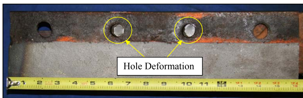
(b) Angle After Testing
