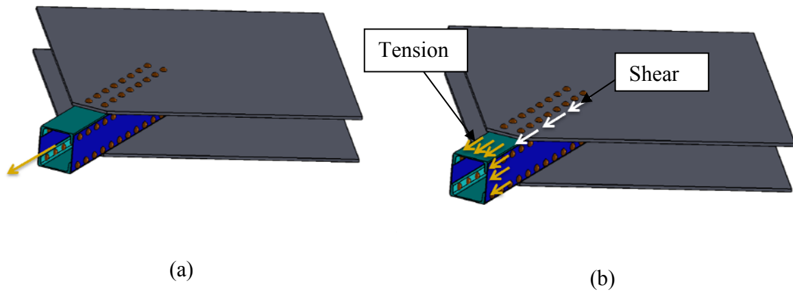
Figure 3.17 Gusset Plate Loading via Tension and Shear
