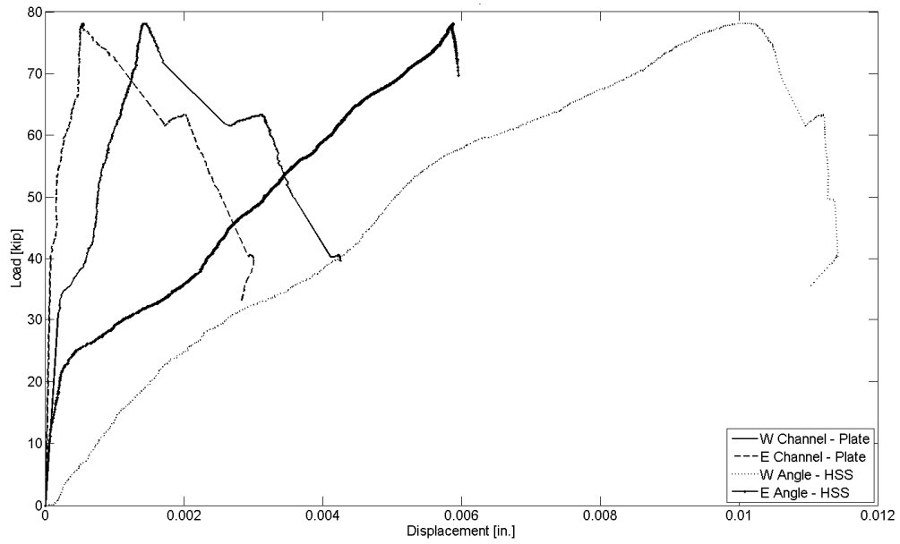
Figure E.10 Load vs. Bolt Slip – Test 2R (4L)
