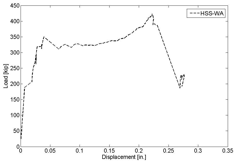
Figure E.12 Load vs. Angle Bolt Slip - Test 11R
