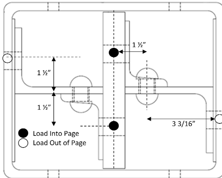
Figure 3.15 Cross Section With Load Transfer
