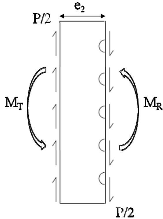
Figure 3.28 Free Body Diagram of Angle
