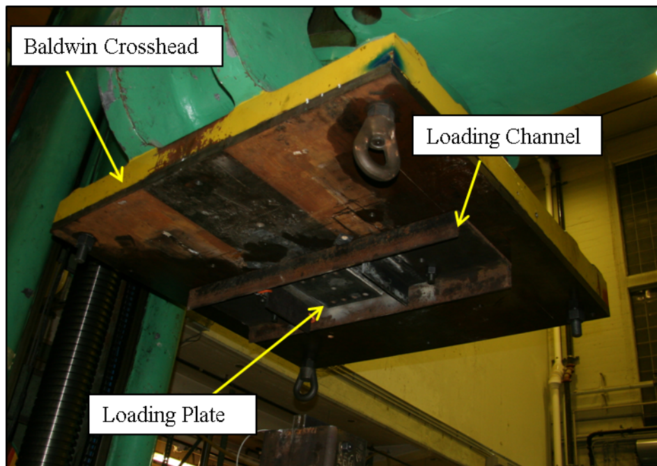
Figure 4.50 Loading Channel for Baldwin Tests
