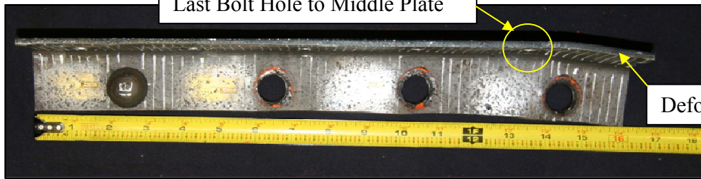
(b) East Channel Flange Rivet Surface
