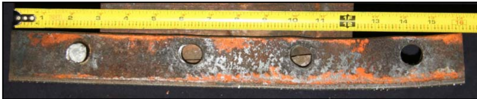
(a) East Channel Flange Faying Surface
