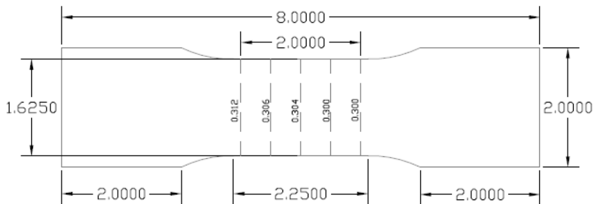
Figure 4.6 Tension Coupon A2 (all dimensions in inches)
