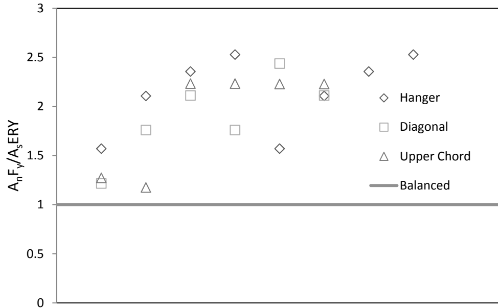
Figure 3.21 Cle Elum River A_n F_y / A_s E R Y Ratio - Nominal Values
