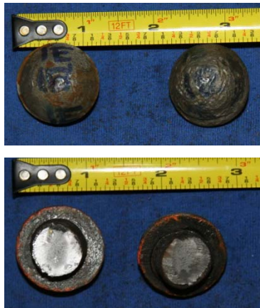
Figure 4.32 Test 2R Fractured Rivets
