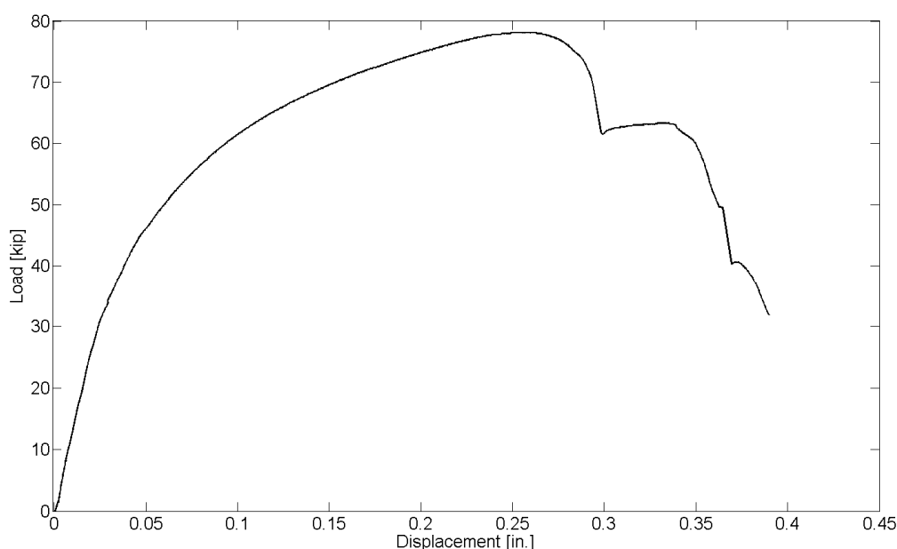
Figure 4.35 Load vs. Overall Displacement - Test 2R (4L)
