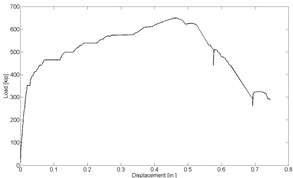
Figure 4.62 Load vs. Overall Displacement - Test 17R
