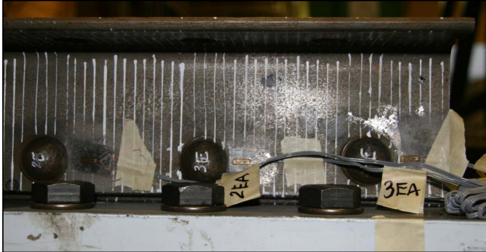
Figure 3.40 Strain Gauge Placement on East Angle
