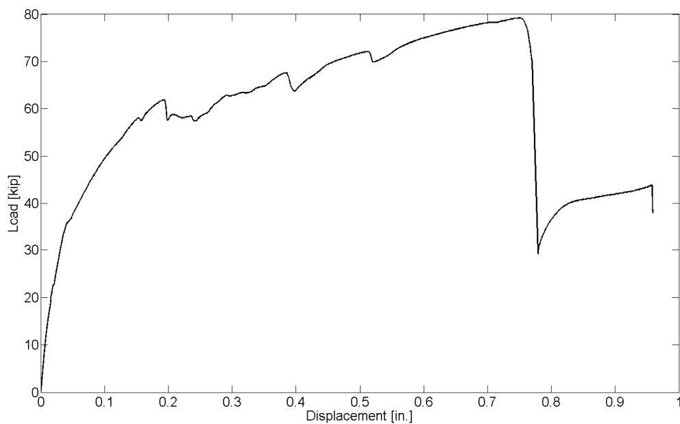
Figure 4.25 Load vs. Overall Displacement – Test 2R
