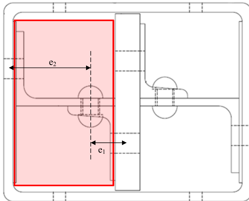
Figure 3.26 Free Body Diagram of Guardrail Configuration
