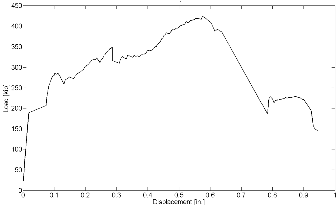
Figure 4.52 Load vs. Overall Displacement – Specimen 11R
