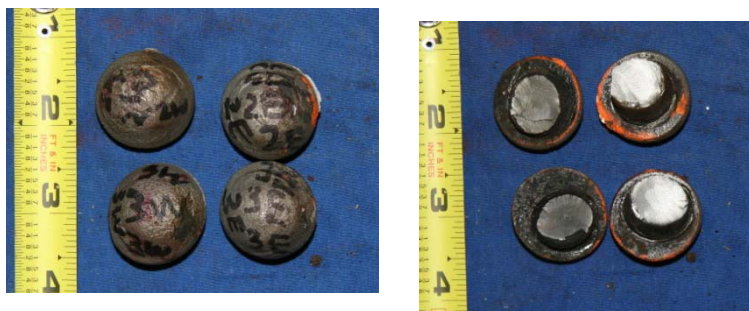
Figure 4.40 Fractured Rivets – Specimen 2R (4L)
