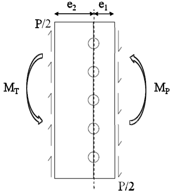
Figure 3.27 Guardrail Section Free Body Diagram
