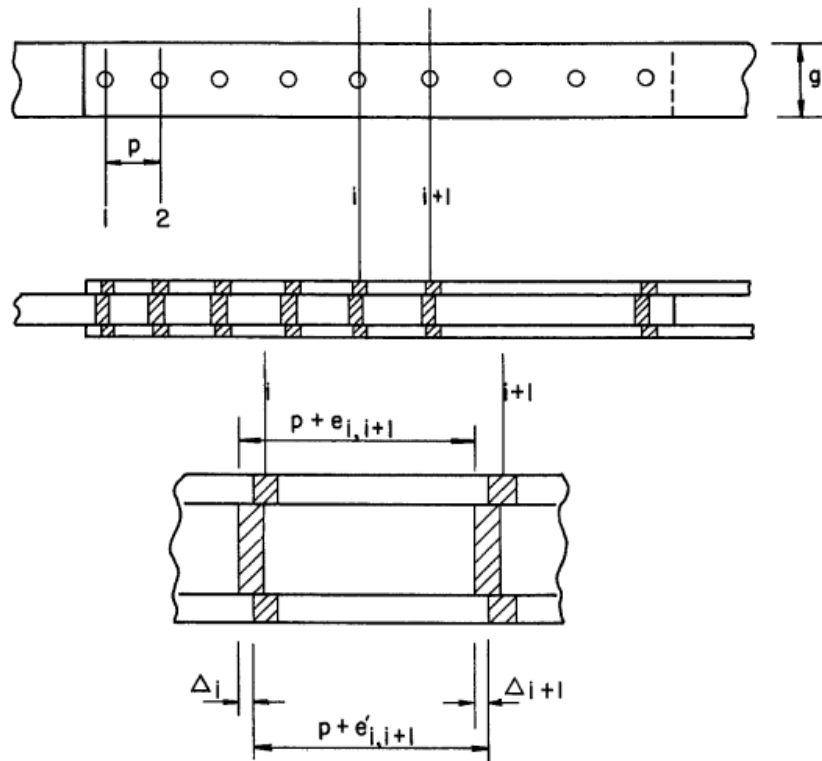
Figure 2.19 Joint Deformation in Plates and Bolts (Fisher & Rumpf, 1967)
