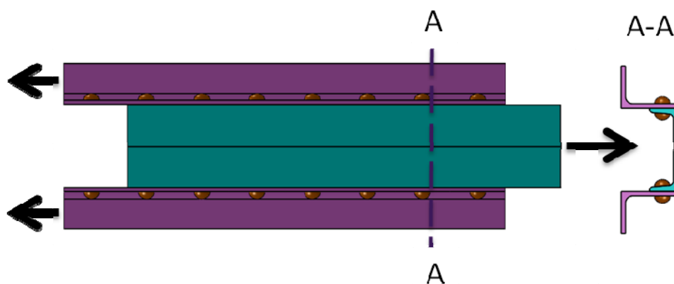
Figure 3.9 Testing Guardrail in Tension "Lap-Splice"
