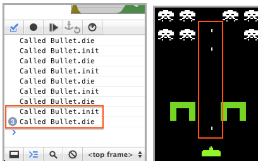
Figure 5.4: Screenshots of the logging output window and the defect’s manifestation in the game. Steph added logging statements to the die and init methods. At left, the logging output shows the order of method entries, with the blue circle summarizing 3 identical logging outputs. According to the last 4 logging statements (outlined in red), calls to die and init are unbalanced. At right, three in-flight bullets correspond to the three calls to Bullet.init .
