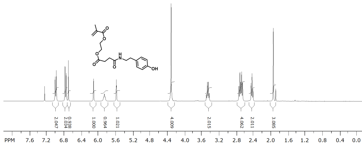
Figure S5. 1 H-NMR spectrum of butanoic acid, 4-[(4-hydroxyphenyl)ethylamino]-4-oxo, 1-(2-methacryloyloxy)ethyl ester ( 12 )
