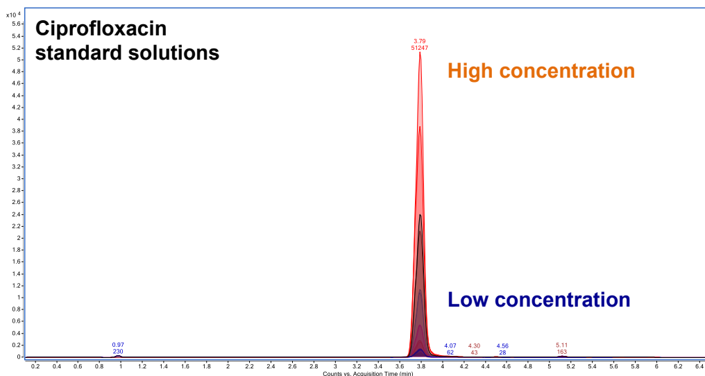
Fig. 3 Representative overlay LC chromatogram of ciprofloxacin standard solutions.
