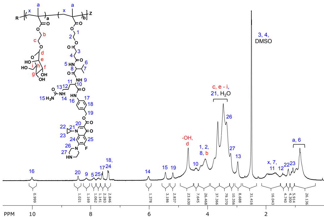
Figure S11. Representative ^1\text{H-NMR} (300 MHz, \text{DMSO-d}_6 ) of synthesized polymeric ciprofloxacin prodrug with Val-Cit dipeptide linker, poly(Man-co-VC).
