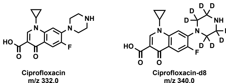
Fig. 1 Chemical structures of ciprofloxacin and ciprofloxacin-d8 internal standard.
