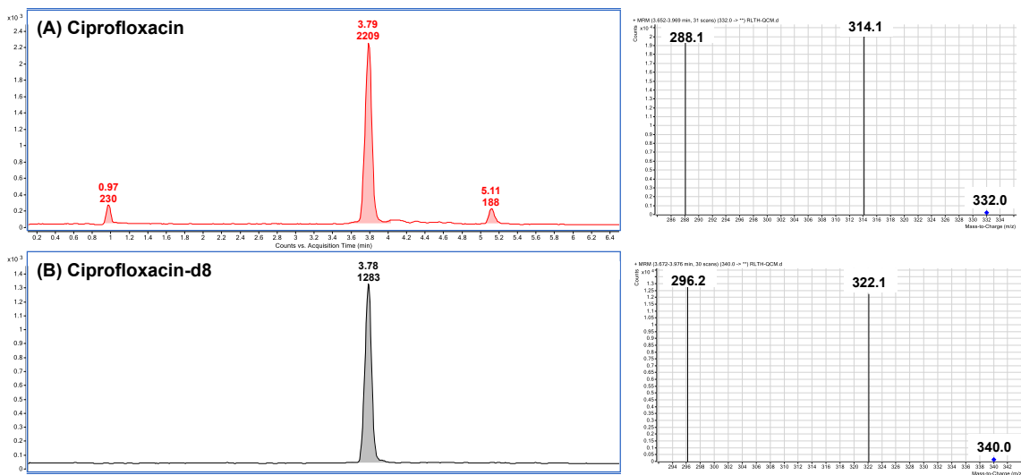
Fig. 2 Chromatograms and mass spectra for (A) ciprofloxacin ( 5 \text{ ng mL}^{-1} standard) and (B) ciprofloxacin-d8 internal standard ( 5 \text{ ng mL}^{-1} ) in lung tissue matrix.
