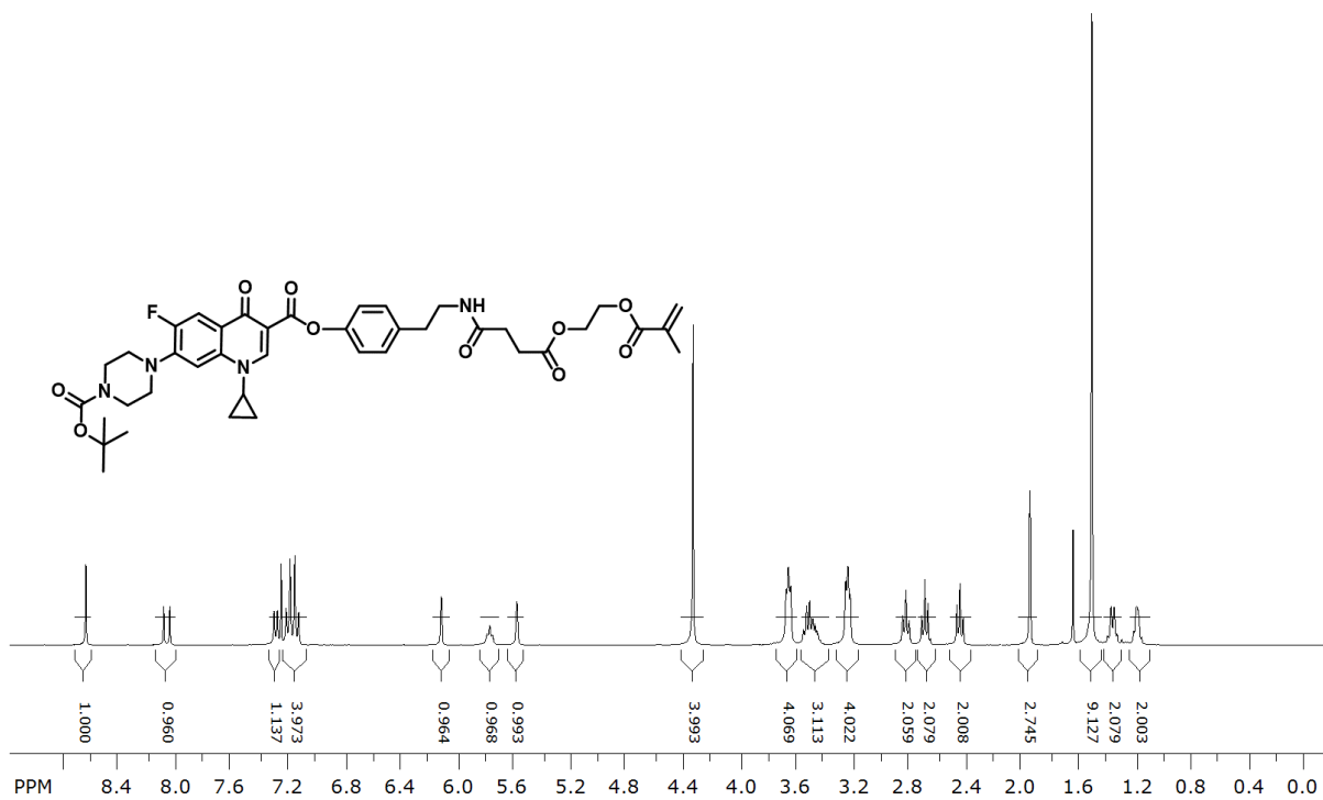
Figure S6. 1 H-NMR spectrum of BocCTM ( 13 )
