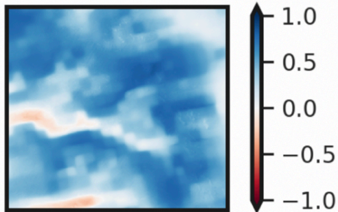
Figure 4: Spatial comparison of the mean dot-products between wind vectors of different wind fields for WY2017. Wind field vectors are normalized before the dot-product is taken so that only the modeled wind directions are compared. Regions of value 1 indicate agreement between the wind fields on the wind direction, whereas regions of value -1 indicate disagreement.
