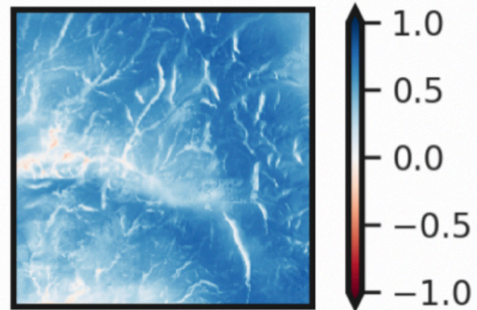
HRRR+MM · HRRR+WN
