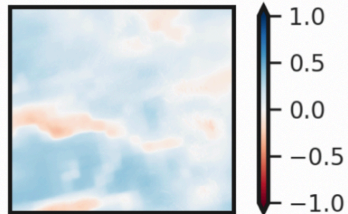
Figure 4: Spatial comparison of the mean dot-products between wind vectors of different wind fields for WY2017. Wind field vectors are normalized before the dot-product is taken so that only the modeled wind directions are compared. Regions of value 1 indicate agreement between the wind fields on the wind direction, whereas regions of value -1 indicate disagreement.
