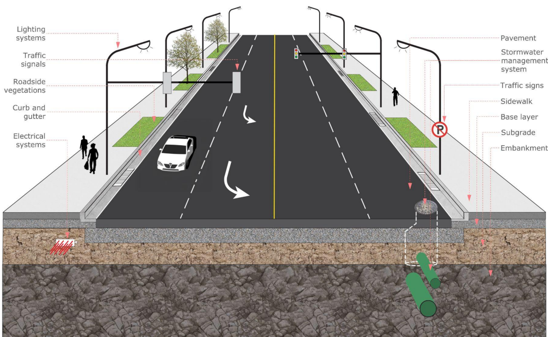
Figure 1. Roadway infrastructure components include not just pavement, but also sidewalks, traffic signals, lighting systems, stormwater management systems, curbs and gutters, sanitary water conveying systems, embankments, among others. Graphic Credit: Sindhu Raju. © Carbon Leadership Forum
