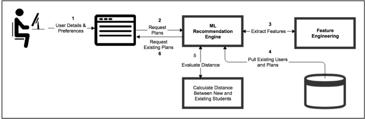
Figure 3.11: Data flow description of Recommendation System
