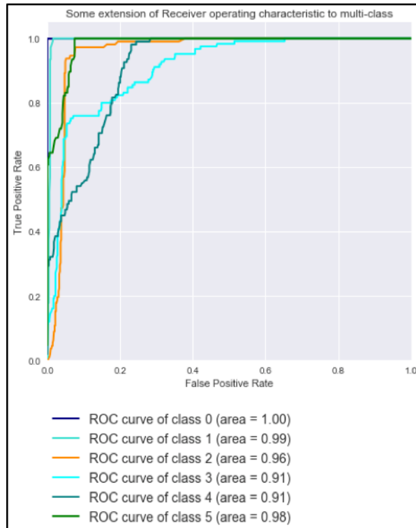
Figure 4.5: ROC curve for ANN
