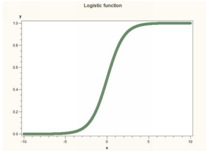
Figure 2.3: Representation of Sigmoid function to predict probability[28]
