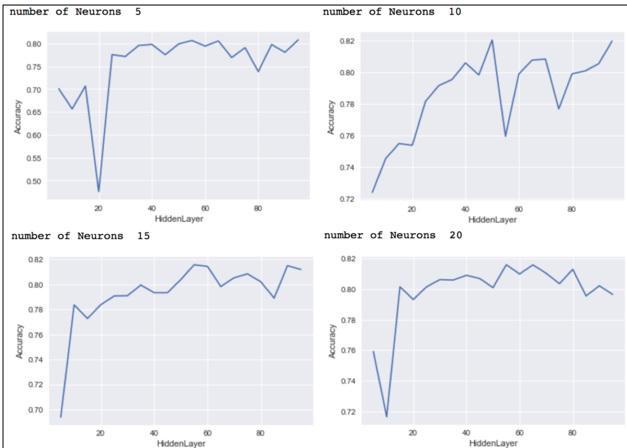
Figure 4.3: Accuracy of our ANN after min-max scaling, varying number of neurons and increasing number of hidden layers.
