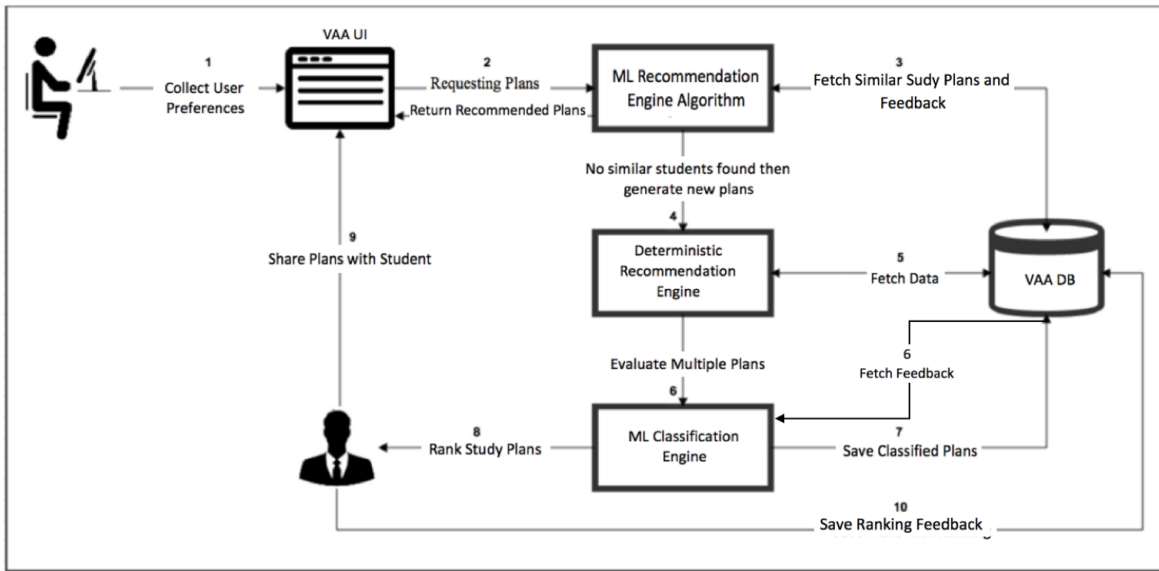
Figure 3.2: Overview of VAA Workflow
