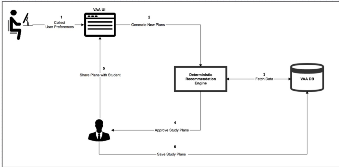
Figure 1.3: Original System Architecture Overview: user preferences are collected through the UI and are used by a deterministic recommendation algorithm to generate study plans.
