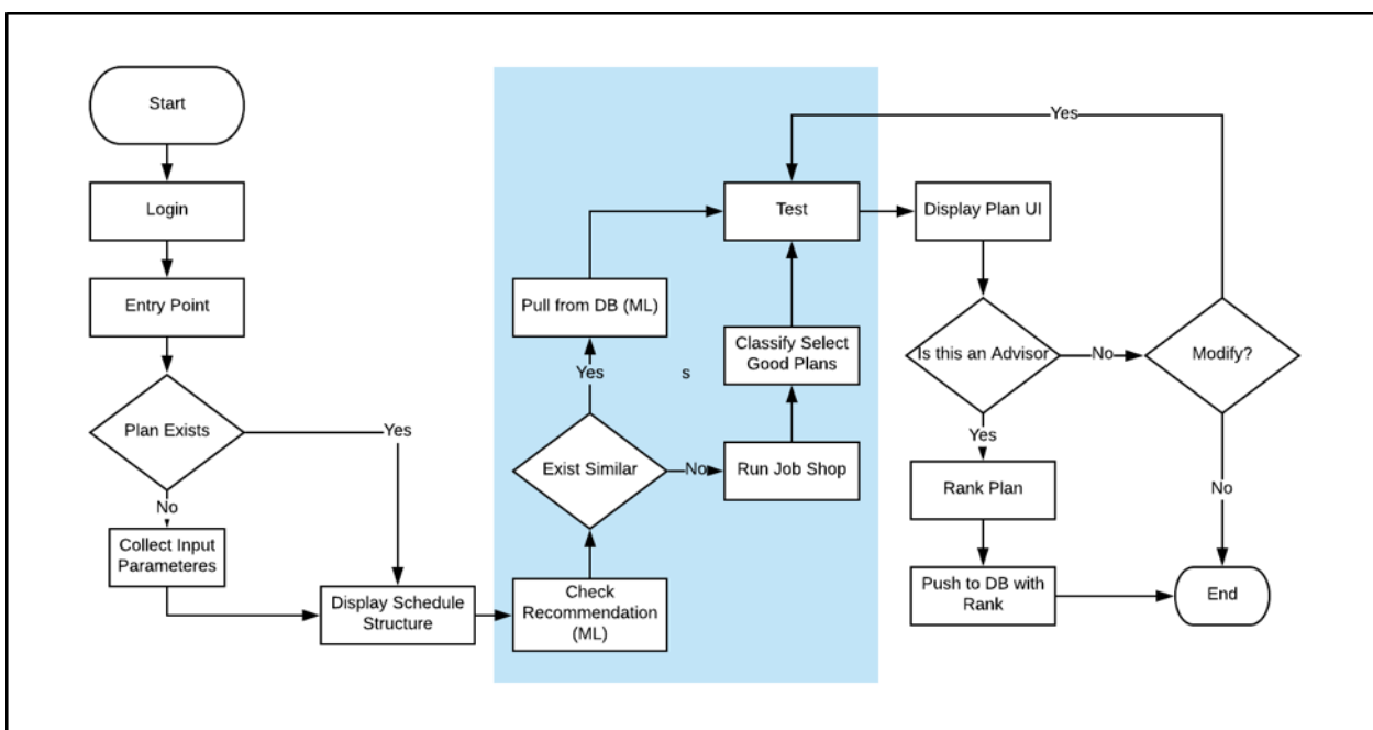
Figure 1.4: Data Flow of the proposed solution
