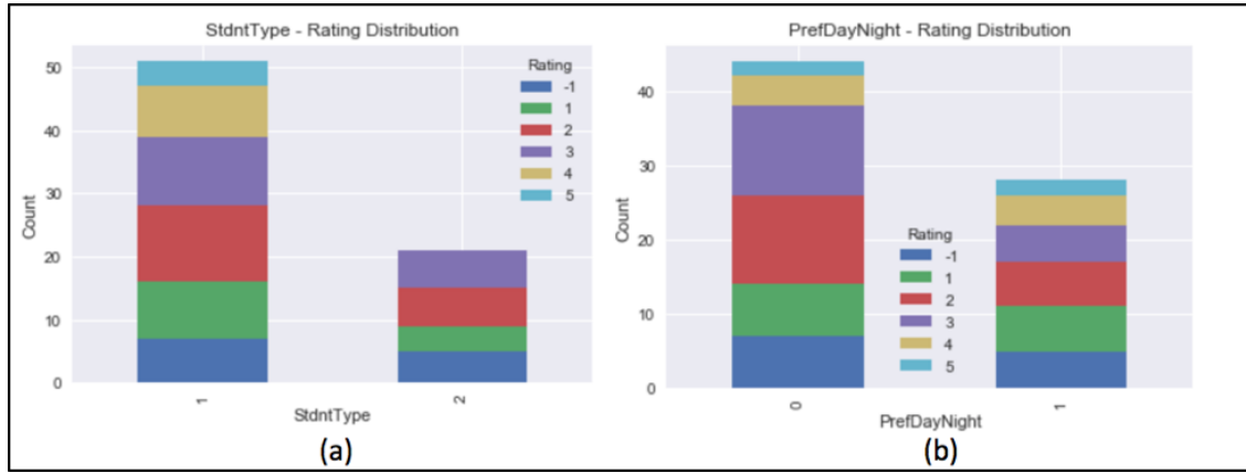
Figure 3.3: Univariate Analysis
