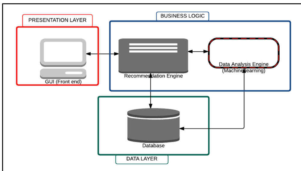
Figure 3.1: High-level architecture
