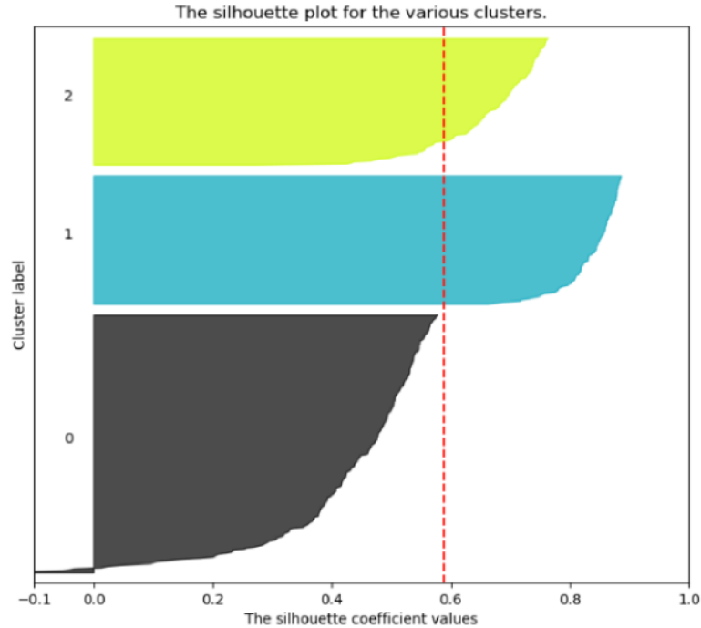
Figure 3.19: Example of Silhouette analysis for depicting appropriate number of K [48]
