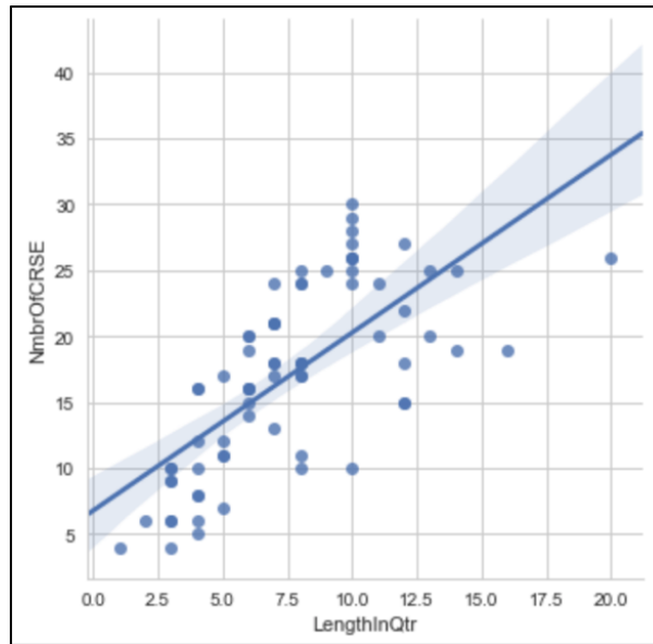
Figure 3.6: Scatter Plot where x-axis represents “Length of a study plan in Quarters” and y-axis represents “Total number of core courses”
