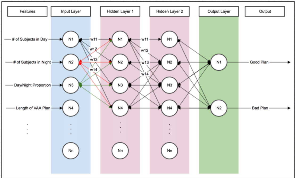
Figure 3.10: Neural Network implementation overview
