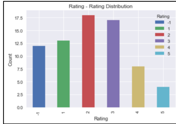
Figure 3.4: Rating Distribution
