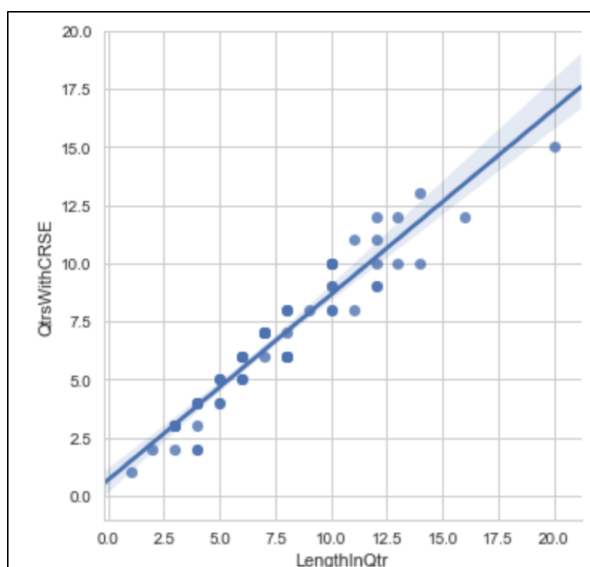
Figure 3.5: Scatter Plot to explain correlation between LengthInQtr and QtrsWithCRSE
