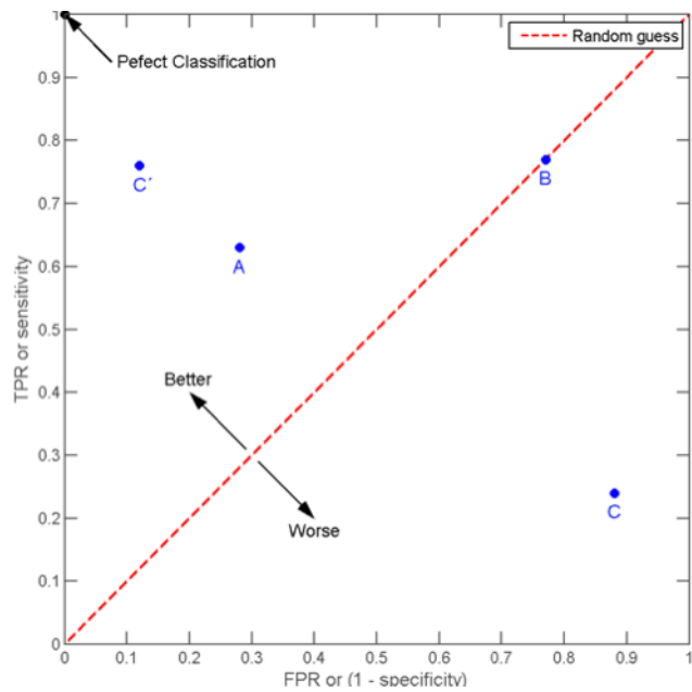
Figure 3.21: Example of area under ROC curve [53]: The red line represents the ROC for a random classifier, i.e., 50% chance of classifying correctly. When the line curves following the (Better) arrow, the AUC increases, indicating better classifier performance.
