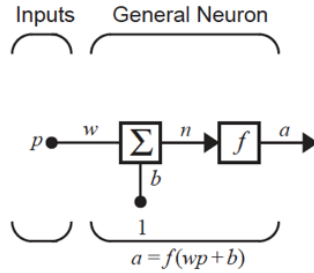
Figure 2.1: Illustration of a single neuron [22]
