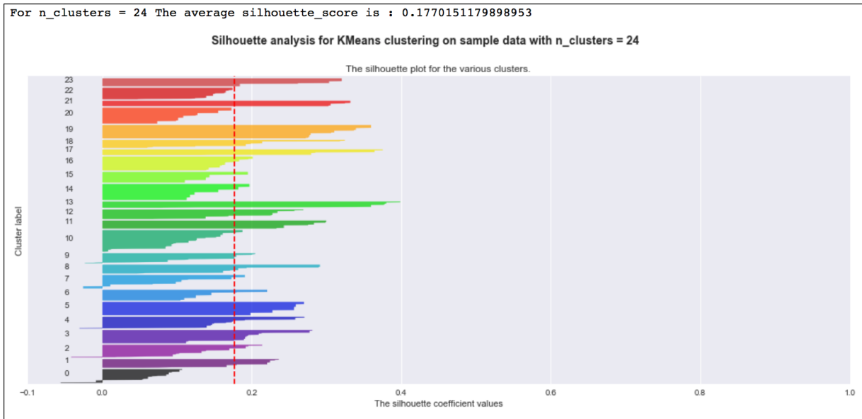
Figure 4.11: Silhouette Analysis for clusters K = 20 and K = 24 . The x -axis represents silhouette coefficient value between -1 to 1 and y -axis represents labels for clusters.
