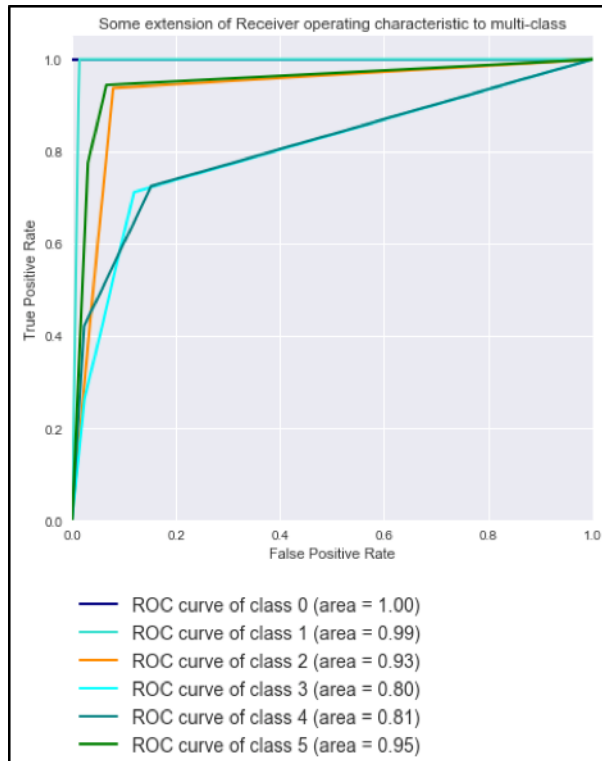
Figure 4.9: ROC curve for kNN
