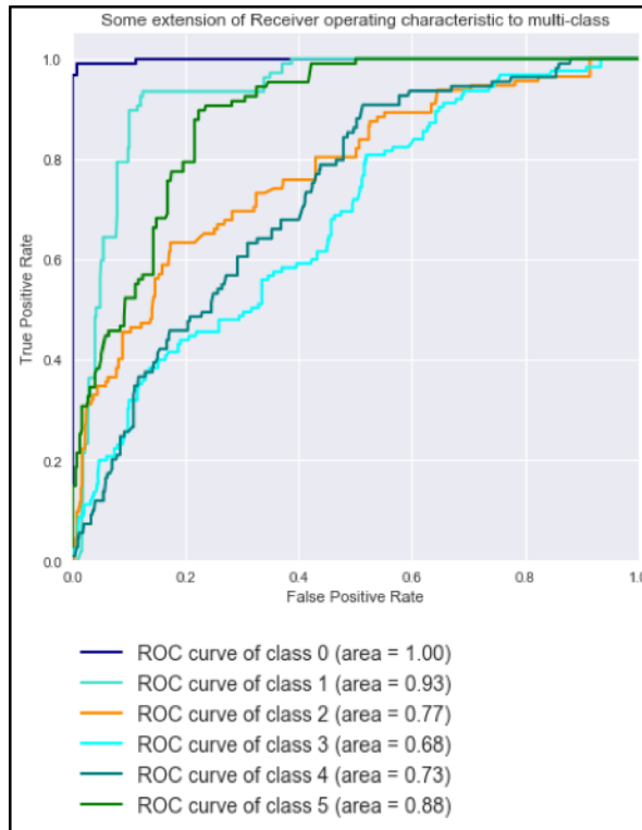
Figure 4.7: ROC curve for Logistic Regression
