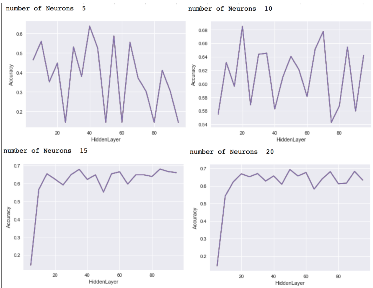
Figure 4.2: Accuracy of our ANN before min-max scaling, varying the number of neurons and increasing the number of hidden layers.
