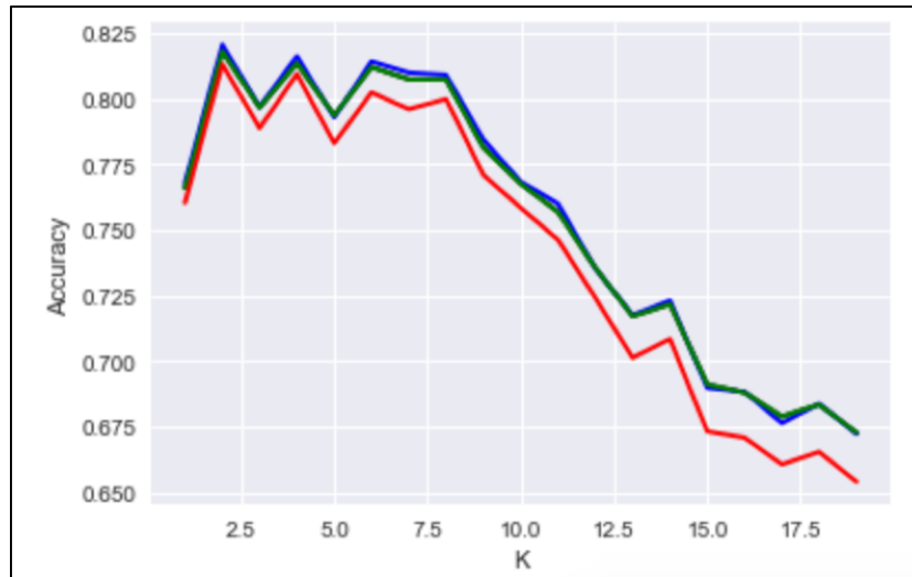
Figure 4.1: Representation of classification metrics for kNN
