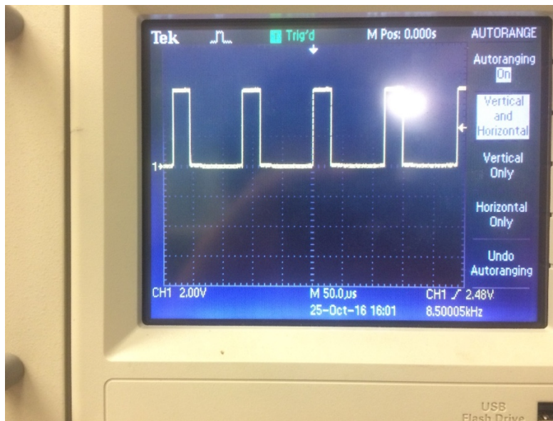
Figure C8: Output voltage of the system in a form of pulse waves, as a response to the light source provided from the LED.
