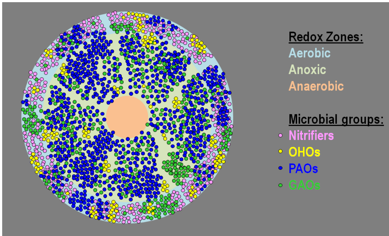
Figure 4-3. Schematic representation of microbial spatial distribution in aerobic granules with anaerobic feeding and aeration period for simultaneous nitrification-denitrification and EBPR.
