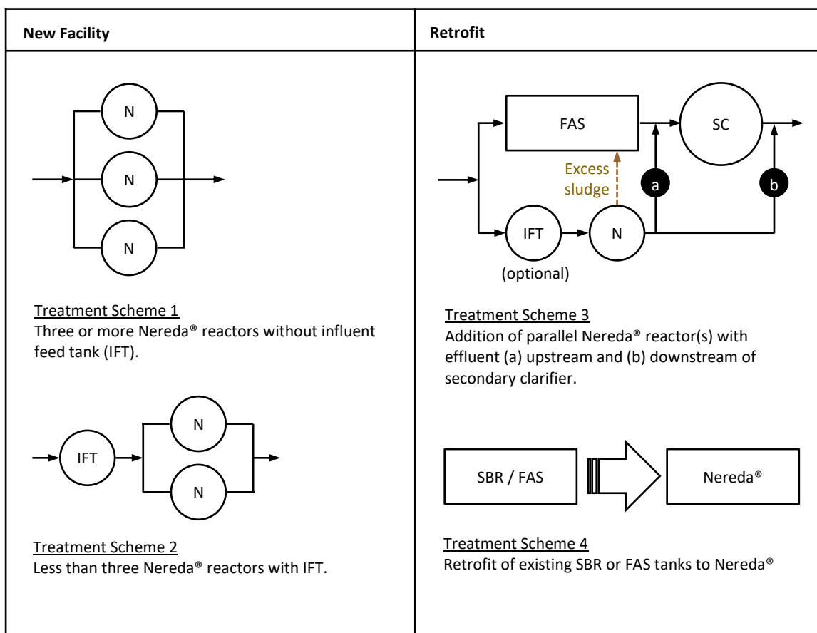
Figure 7-4. Nereda® process application configuration options.
