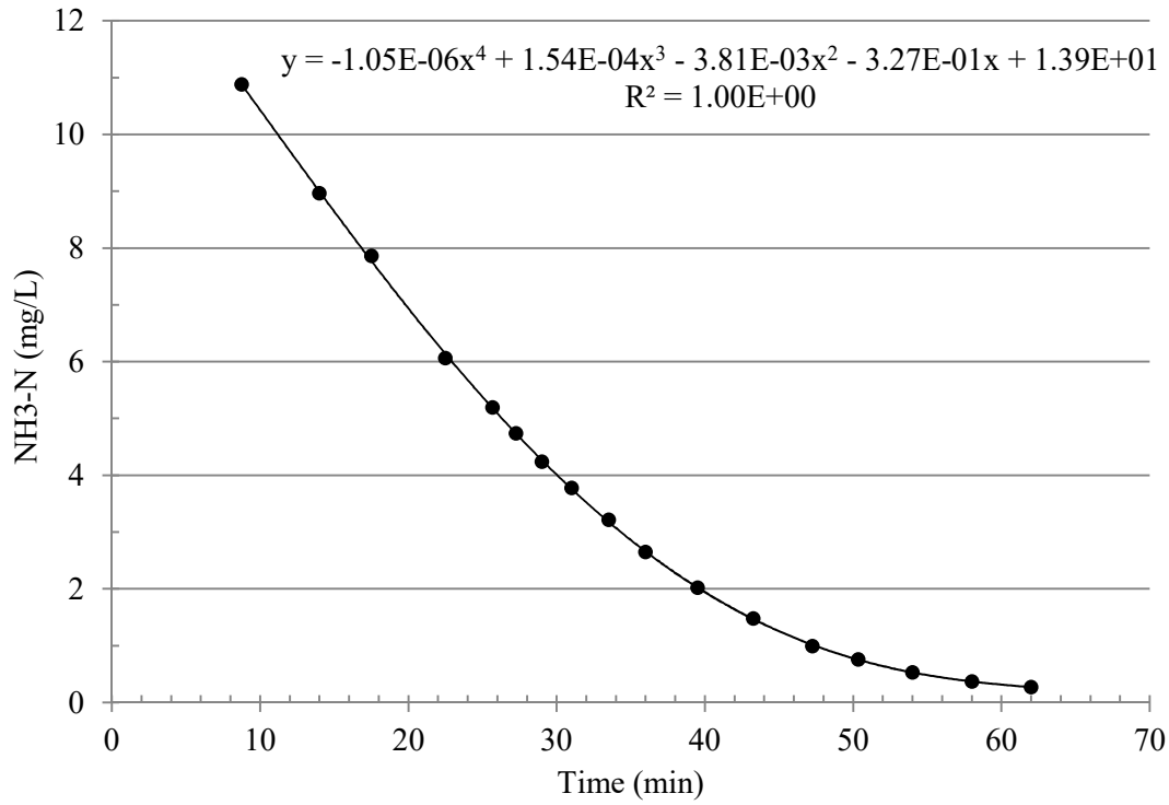
Figure C4. Experimental data for determination of apparent \text{NH}_3\text{-N} half-saturation coefficient for sidestream nitrifying-denitrifying granules. Error bars for triplicate measurements are shown but hidden by markers for average values. The value for the derivative of the regression equation at minute 38 is half that at minute 10 and corresponds to an \text{NH}_3\text{-N} concentration of 2.3 mg/L.
