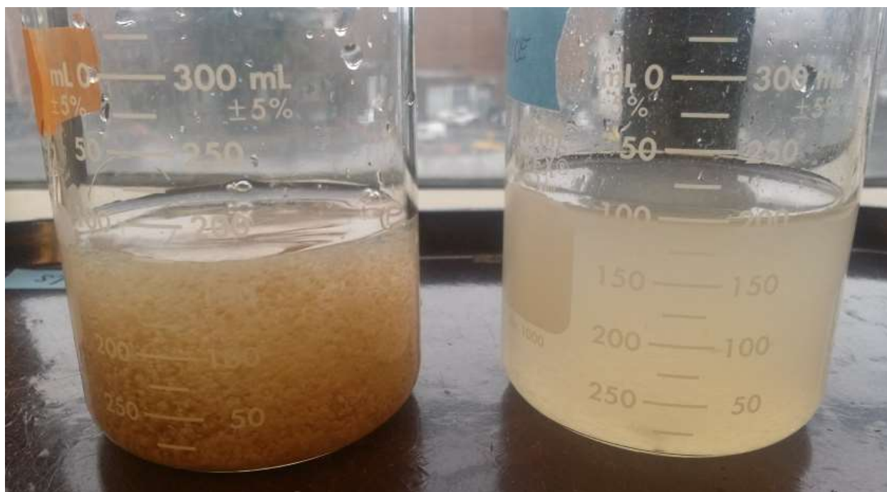
Figure C8. Mainstream reactor mixed granular (left) and flocculent (right) solids fractions after sieving protocol.
