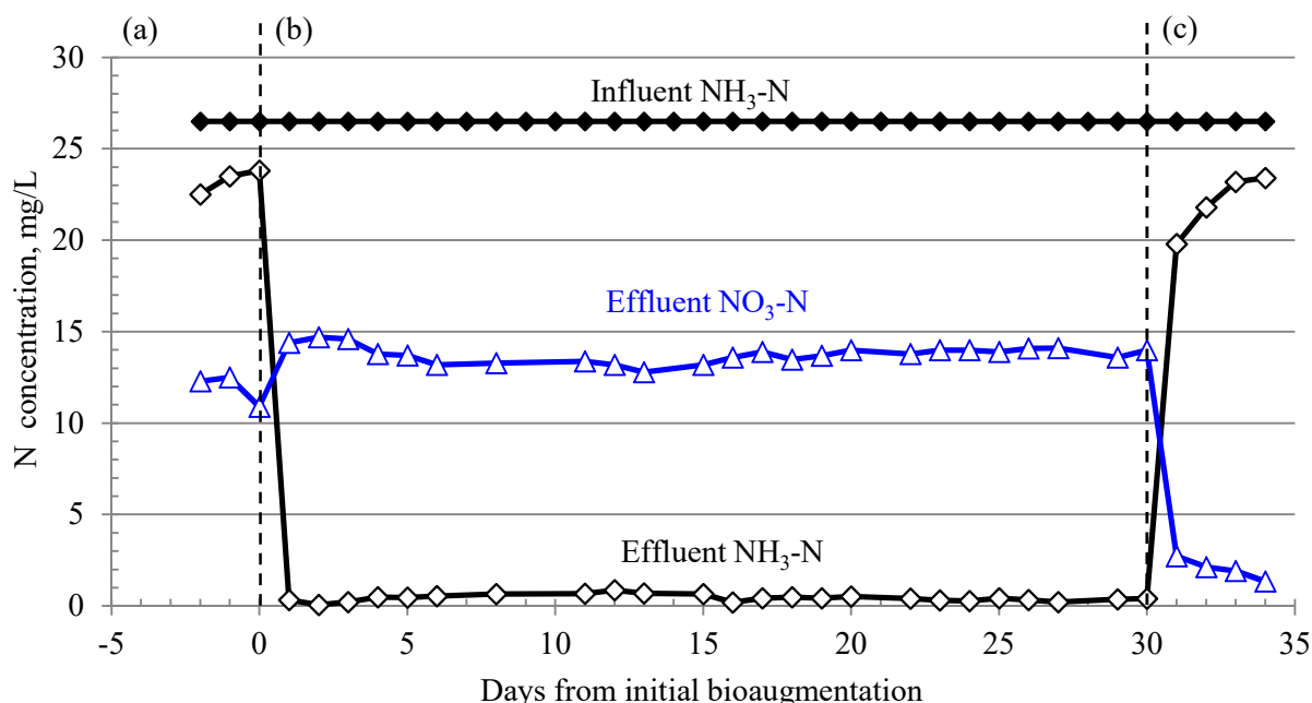
Figure 5.2. Mainstream reactor influent NH 3 -N and effluent NH 3 -N and NO 3 -N concentrations during pre-bioaugmentation (a), bioaugmentation with granule addition (b), and post-bioaugmentation after granule removal (c). Influent included 5.5 mg/L of organic nitrogen. Effluent NO 2 -N concentration averaged 0.2 mg/L with a maximum of 0.4 mg/L over all periods.
