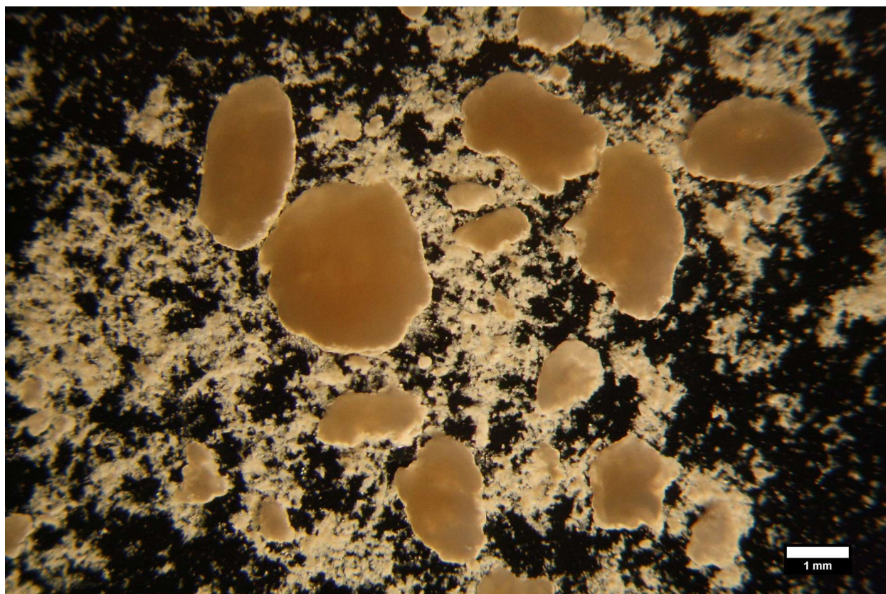
Figure C7. Mainstream reactor mixed liquor suspended solids on the third day of the bioaugmentation period (6x magnification and 1mm scale bar).
