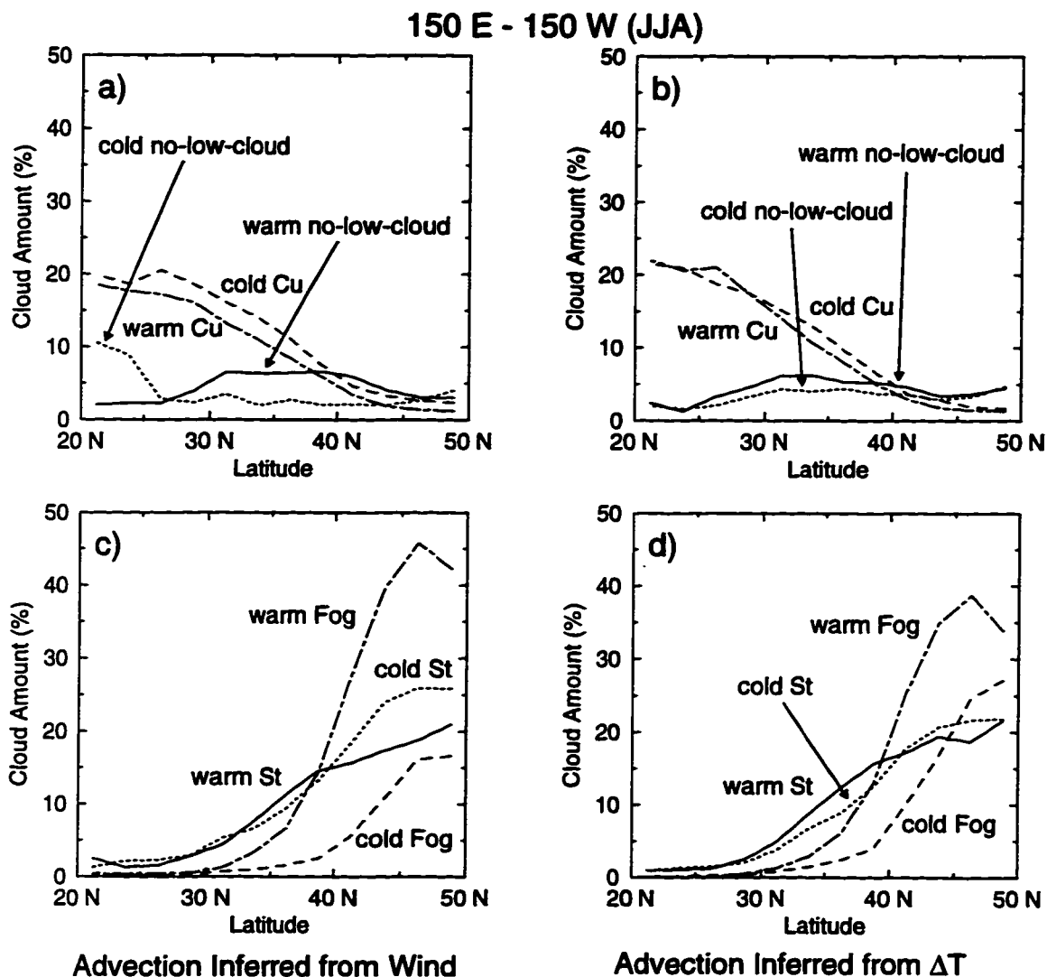
Figure 4.17: (a) As in Fig. 4.15a, except for no-low-cloud ( C_L 0 ) FQ (in same units as cloud amount) associated with warm (solid) and cold (dotted) advection and cumulus ( C_L 1+2 ) cloud amount associated with warm (dot-dash) and cold (dashed) advection. (b) As in (a), except for advection inferred from \Delta T . (c) As in (a), except for fair-weather stratus ( C_L 6 ) cloud amount associated with warm (solid) and cold (dotted) advection and amount of sky-obscuring fog associated with warm (dot-dash) and cold (dashed) advection. (d) As in (c) except for advection inferred from \Delta T . Cloud values for advection inferred from \Delta T are for nighttime good illumination conditions only; otherwise daytime only.
