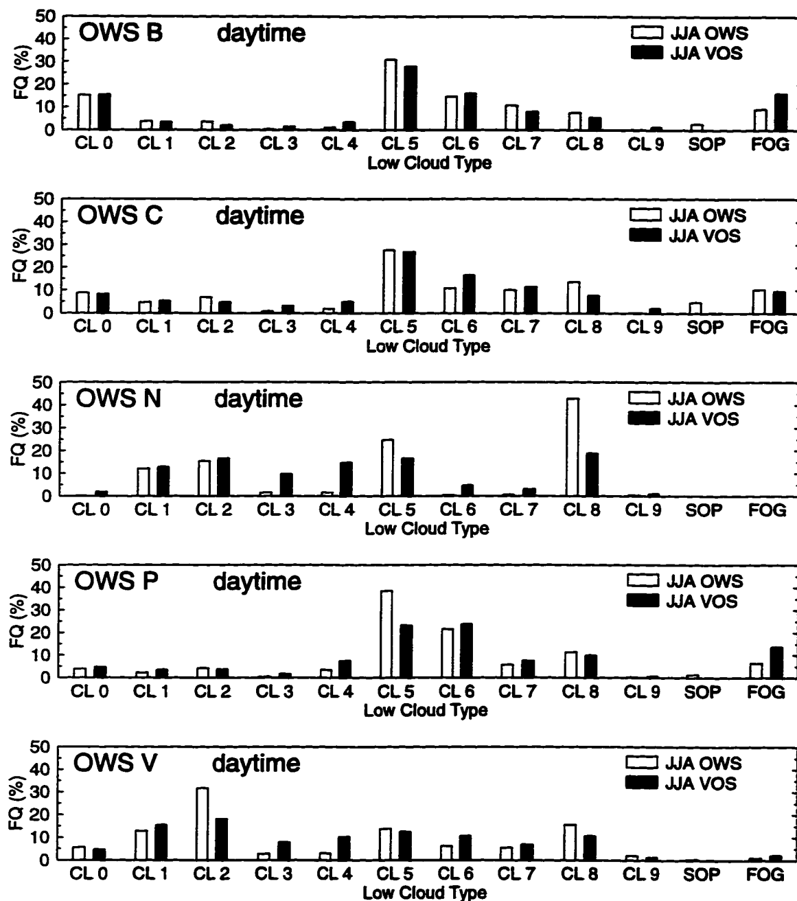
Figure 4.1: Daytime FQ of the low cloud types described in Table 3.2 along with sky-obscuring precipitation (SOP) and sky-obscuring fog (FOG) for OWS B, C, N, P, and V and nearby VOS during JJA. VOS observations are from a 2^\circ \times 2^\circ box centered on the OWS. Both OWS and VOS data are from the time period 1954–1972. Color coding of bars: white - OWS; black - VOS.
