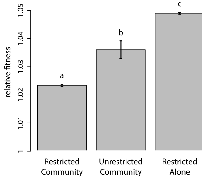
SI Figure 4: The average fitness of resistant cells relative to their ancestor after 36 cycles of simulated evolution in a 12×16 lattice. Simulation runs in the Unrestricted Community treatment in which the three strains did not coexist were excluded. Mean relative fitness of each treatment is shown and bars give the standard error of the mean. Letters distinguish treatments significantly different using post hoc comparisons (single factor ANOVA; F_{2,2208}=1427.5 , p<0.001 , multiple comparisons by Tukey's HSD).
