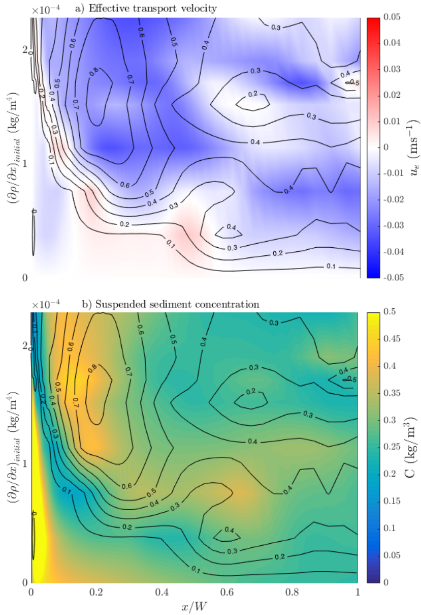
Figure 4.9: (a) Effective transport velocity. Contour lines represent top-bottom ellipticity difference, \Delta\varepsilon . (b) Vertically averaged suspended sediment concentrations over the bottom 1 m. Contour lines represent top-bottom ellipticity difference, \Delta\varepsilon .
