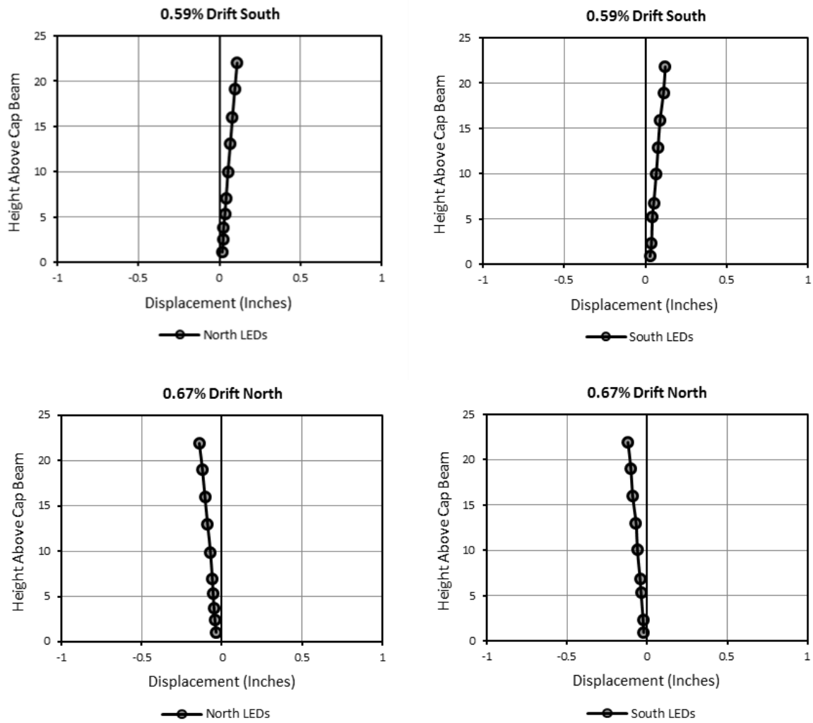
Figure 6.39: EMB80 Buckled Profile – Drift Set 5
