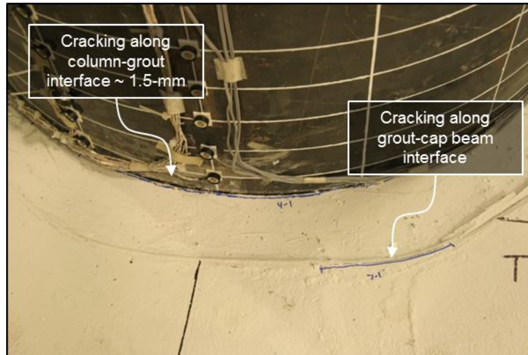
Figure 5.65: EMB96 South grout pad cracking at 1.02% drift North
