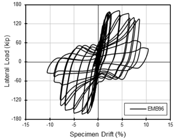
Figure 6.2: EMB96 Force-Drift Response
