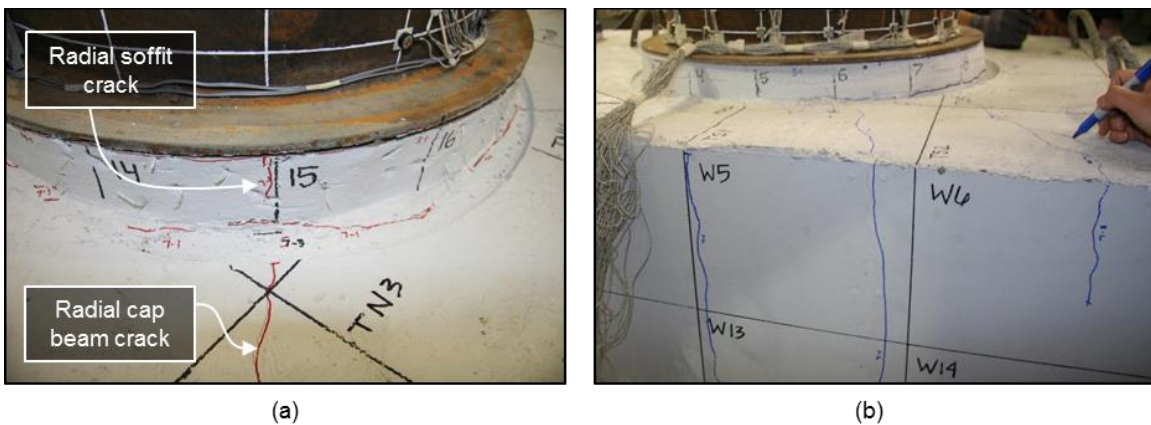
Figure 5.18: WRC radial cracking on (a) North side of column at 1.48% drift, and (b) south side of column at 1.62% drift
