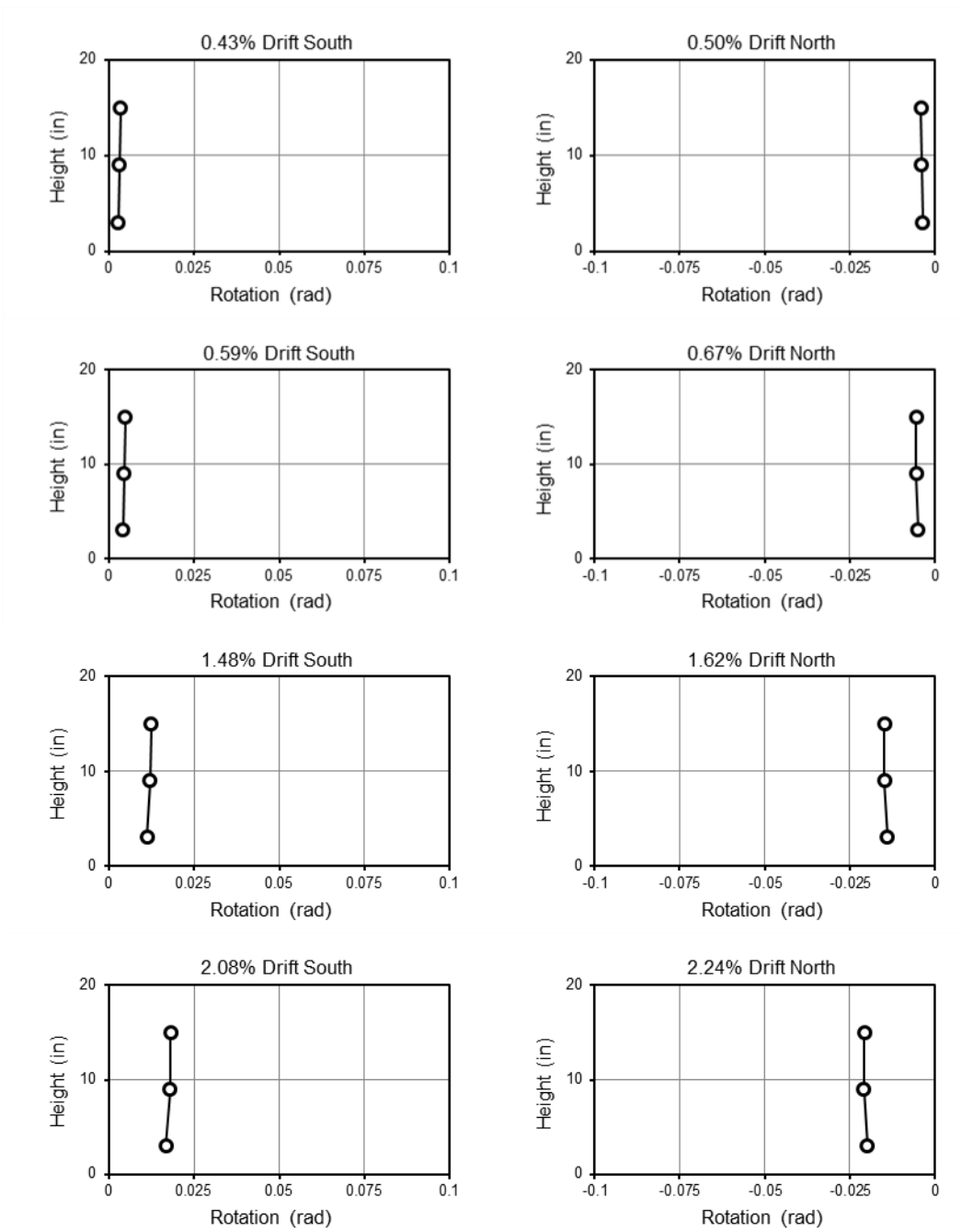
Figure 6.25: WRC Rotation profiles
