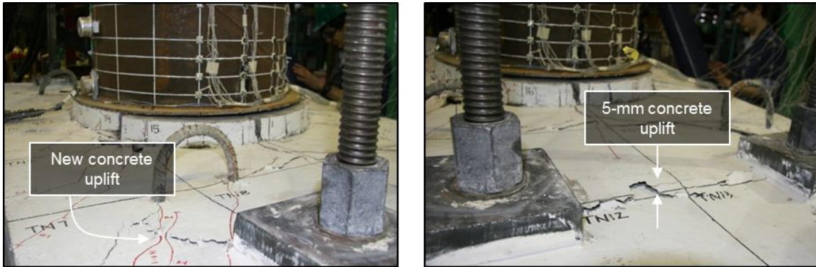
Figure 5.32: WRC North cap beam uplift at 9.71% drift South (Cycle 2)
