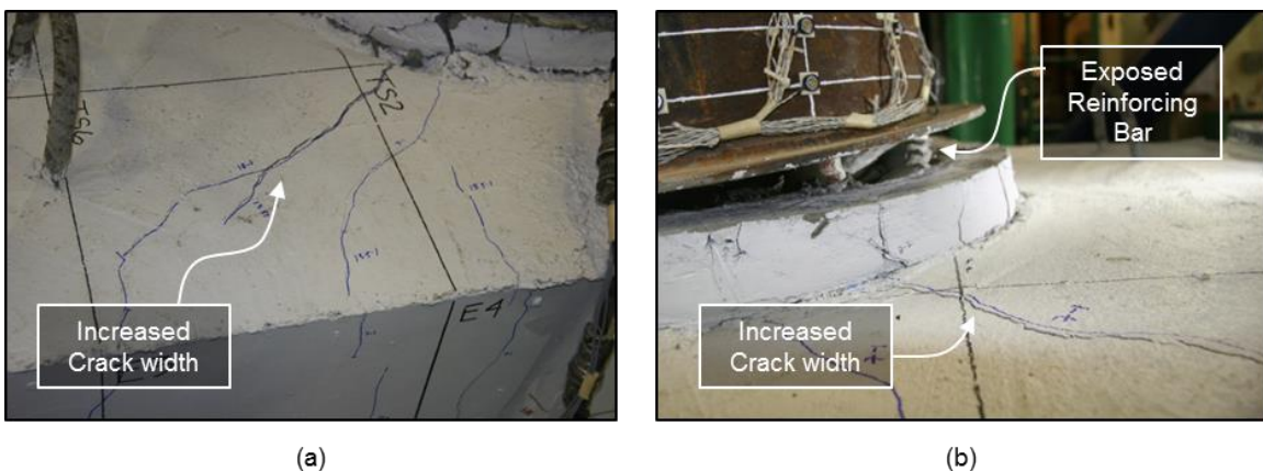
Figure 5.45: WRCUB South (a) cap beam cracking, and (b) exposed reinforcing bar at 8.19% drift North
