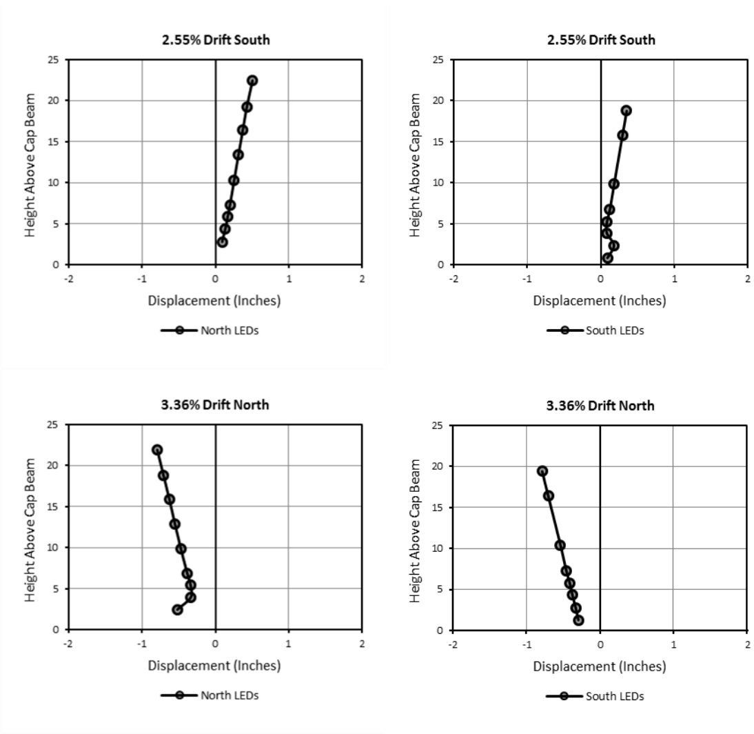
Figure 6.42: EMB96 Buckled Profile – Drift Set 11
