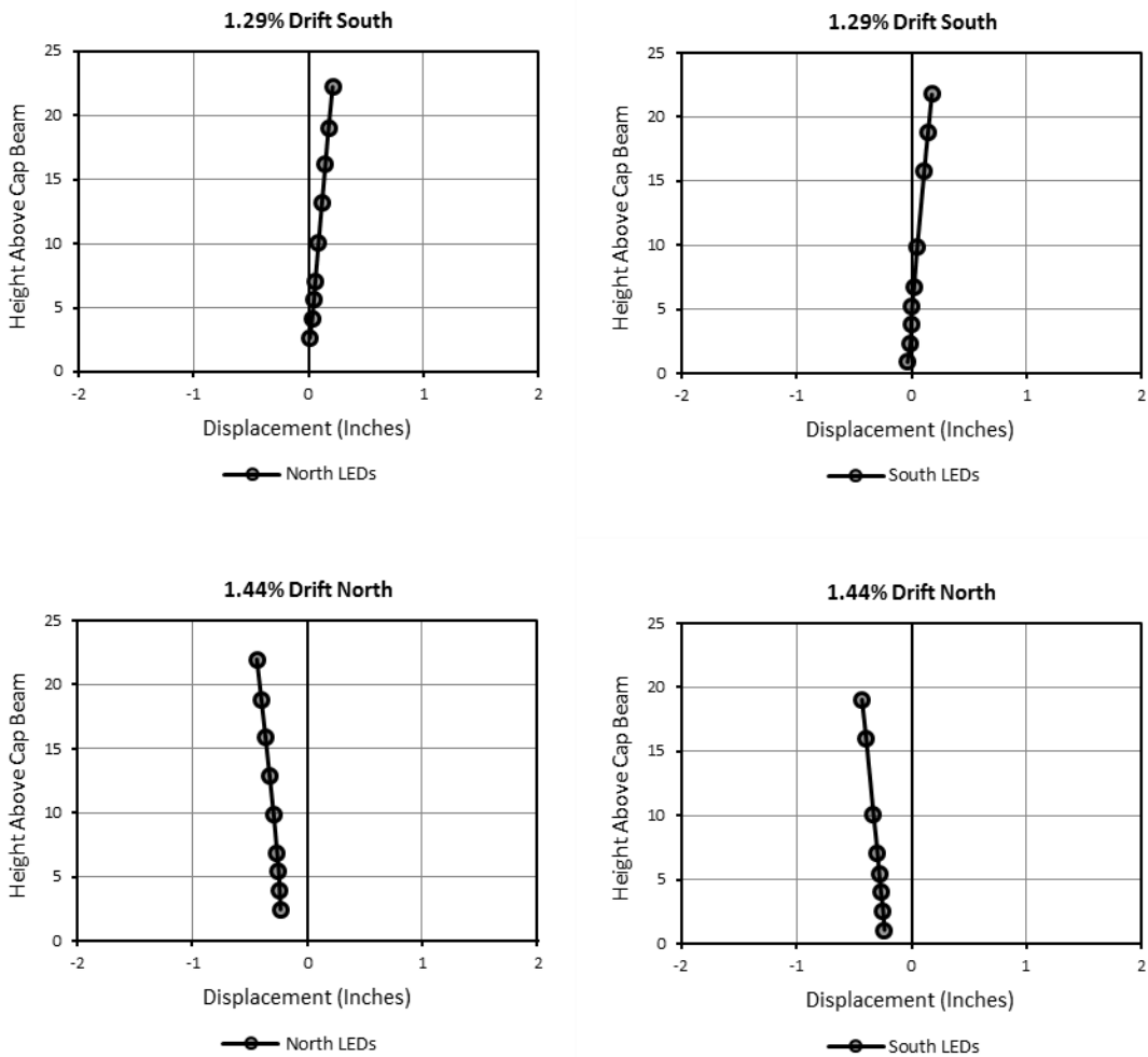
Figure 6.45: EMB96 Buckled Profile – Drift Set 8
