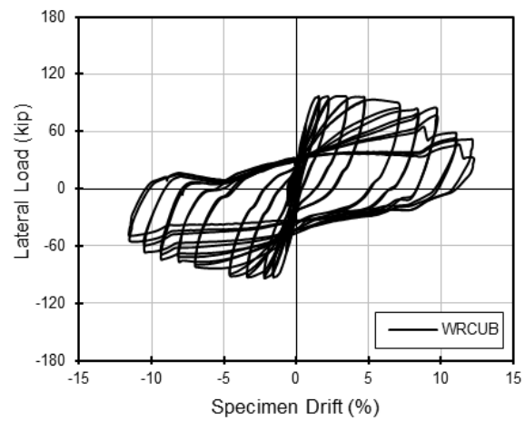
Figure 6.4: WRCUB Force-Drift Response
