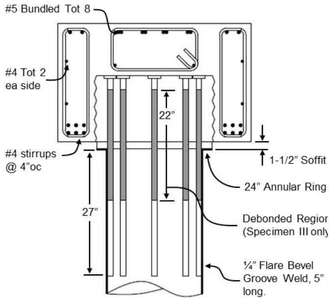
Figure 4.9: Specimens WRC, WRCUB, and RC Reinforcing Details
