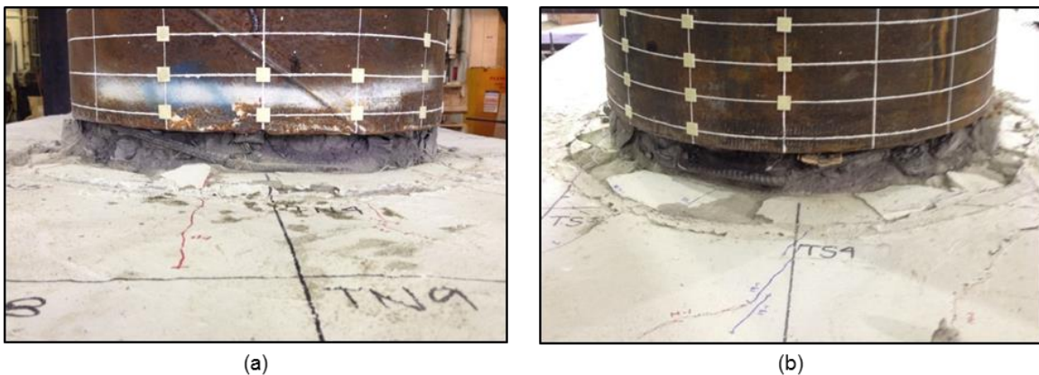
Figure 5.61: WRC(a) North and (b) South side of specimen after removal of spalled grout
