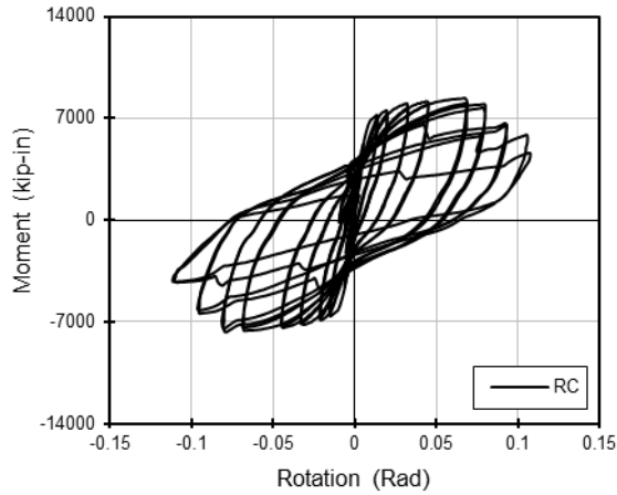
Figure 6.32: RC Moment-rotation response
