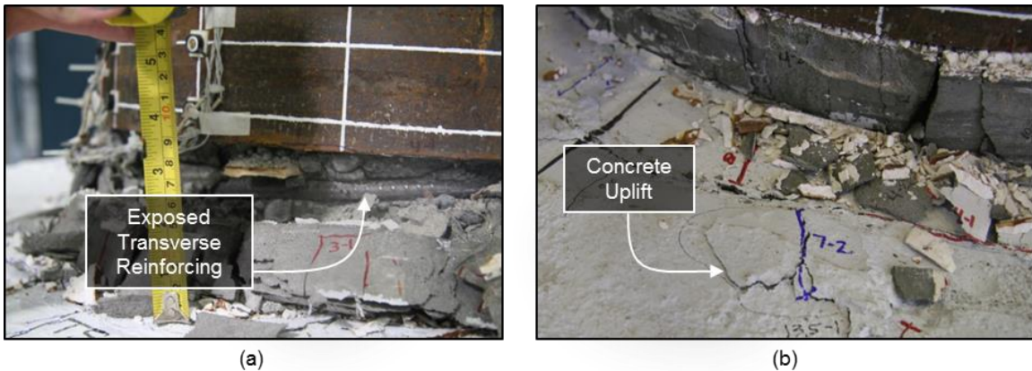
Figure 5.58: WRC (a) South transverse reinforcing, and (b) North concrete uplift at 8.15% drift
