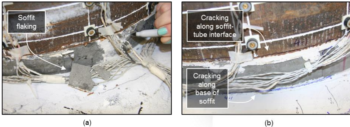
Figure 5.52: WRC (a) Soffit spalling at .28% drift, and (b) Soffit cracking at .44% drift
