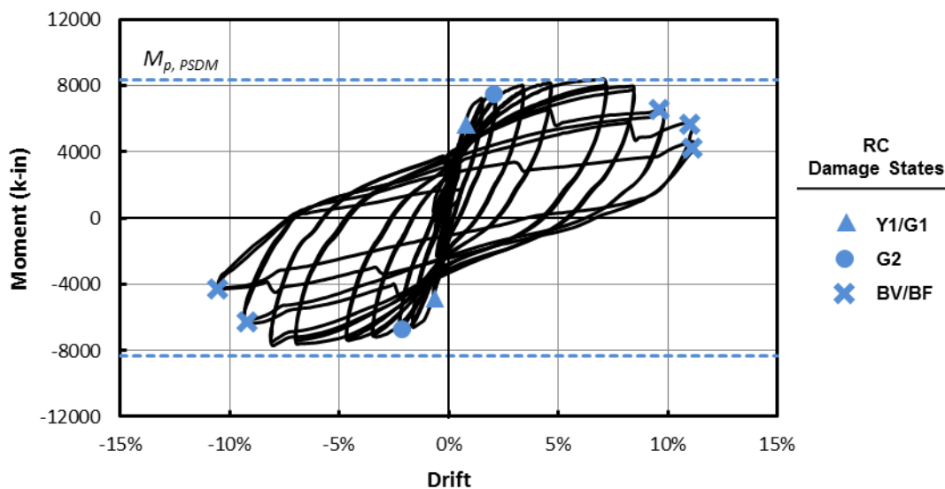
Figure 5.51: RC Moment-Drift Behavior
