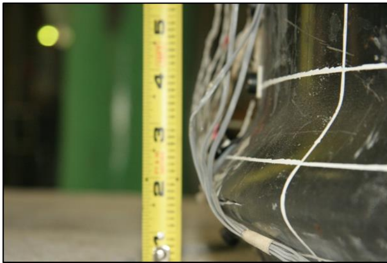
Figure 5.69: EMB96 Initiation of South tube tearing
