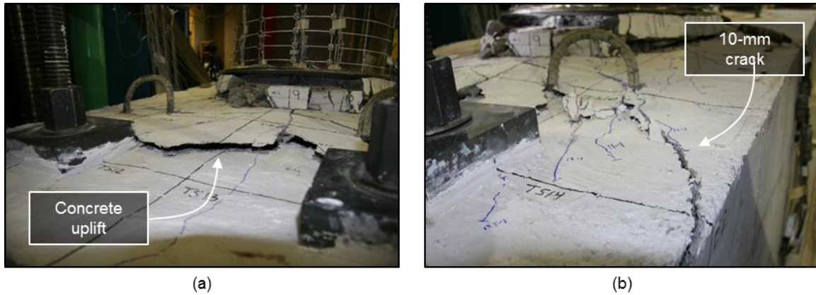
Figure 5.35: WRC South cap beam (a) uplift and (b) cracking at 11.01% drift North
