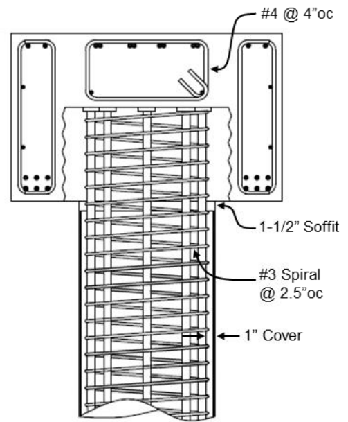
Figure 4.9: Specimens WRC, WRCUB, and RC Reinforcing Details
