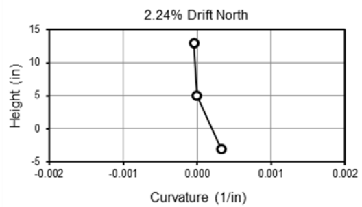
Figure 6.20: WRC Curvature profiles
