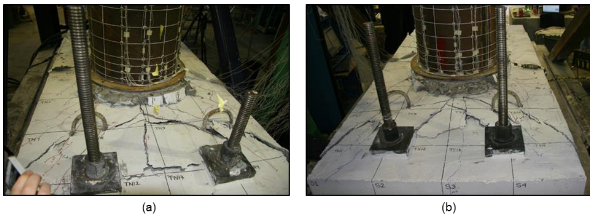
Figure 5.36: WRC (a) North, and (b) South cap beam damage after test termination
