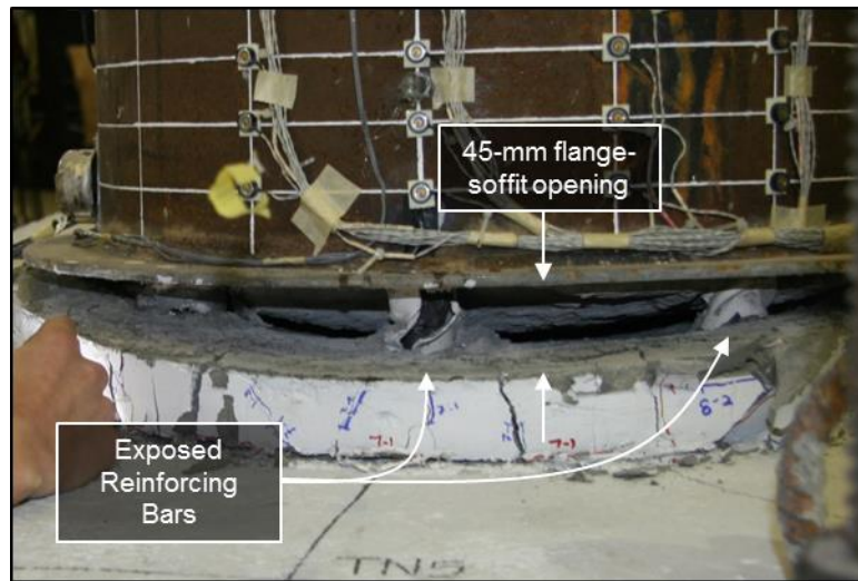
Figure 5.46: WRCUB North exposed reinforcing bars at 9.76% drift South
