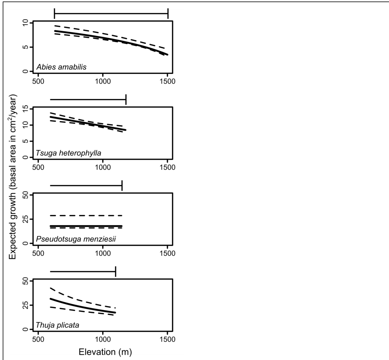
Figure 3. Relationship between elevation and growth for the four focal species. Solid lines show expected mean annual growth rates while dashed lines show the 95% bootstrap confidence interval. Bars above the graphs show the elevational range of the species within the study, with the “]” indicating that the range margin of the species in the study is near its range margin in the vicinity of Mount Rainier.
