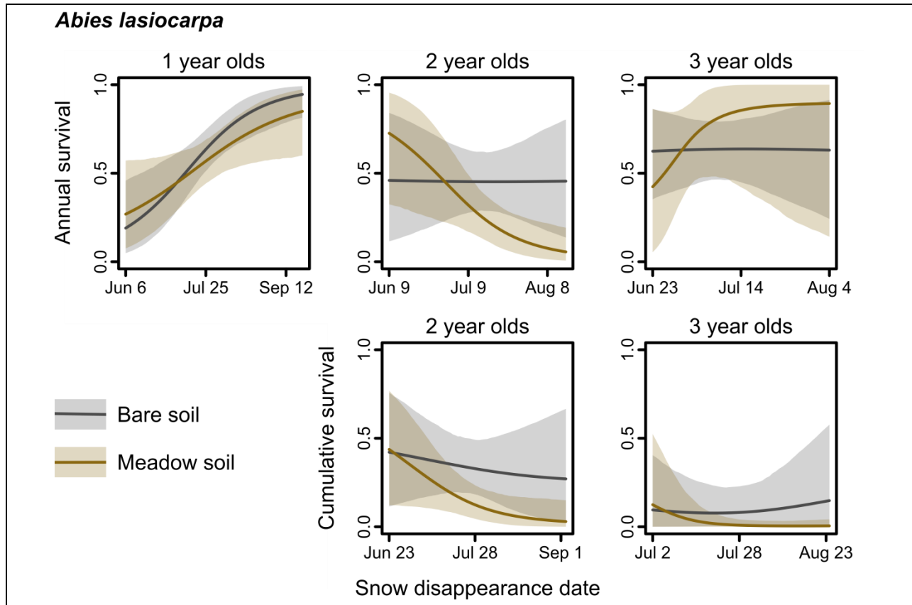
Figure 3. Annual and cumulative survival rates for 1, 2 and 3 year old Abies lasiocarpa seedlings for different microclimate and soil conditions. Lines show the expected mean survival rate and shading shows the 95% credible intervals across the range of snow disappearance dates observed for the given species in the two soil types.
