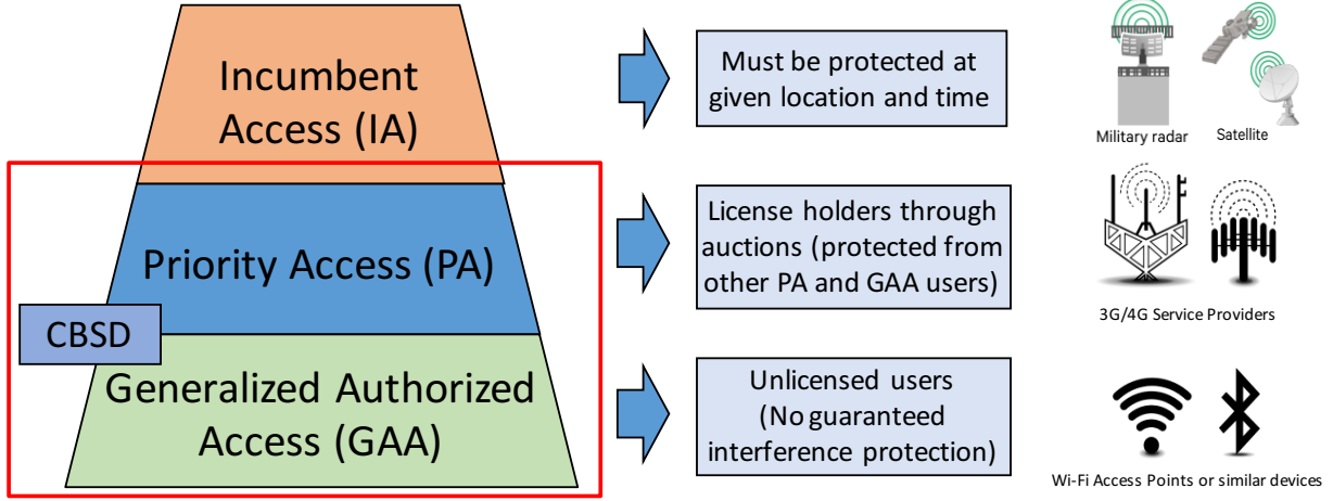
Figure 5.1: Three-tiered spectrum access framework in the 3.5 GHz CBRS band. Incumbents have the highest priority and must be protected at any given location and time. PA users obtain licenses via competitive bidding and are protected from other PA and GAA users. GAA users shall not expect any interference protection and are expected to coexist.
